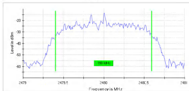
20 dB Bandwidth
