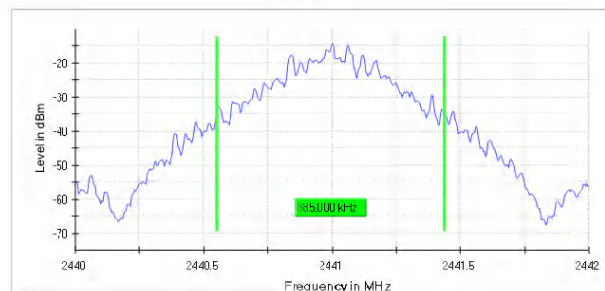
20 dB Bandwidth
