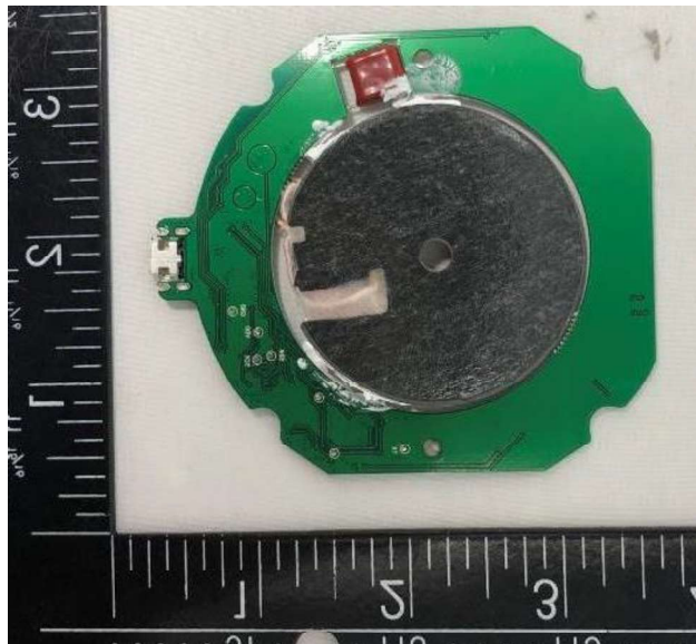
Fig 7. Internal View
