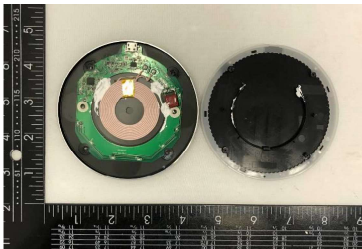
Fig 5. Internal View
