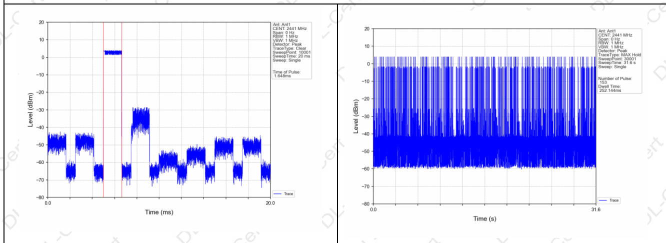
2-DH3
