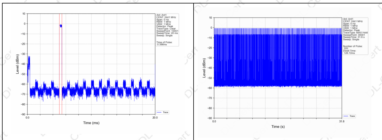
3-DH1
