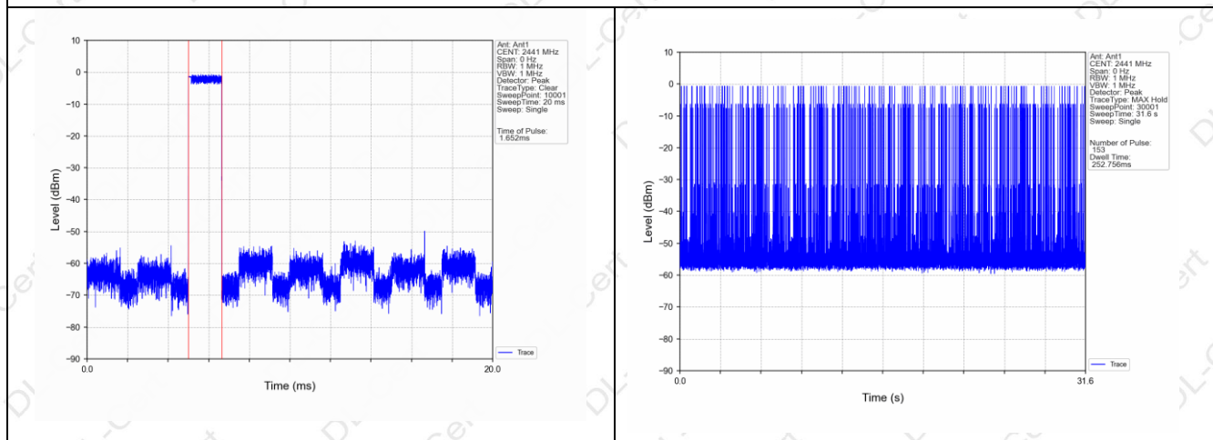
3-DH3
