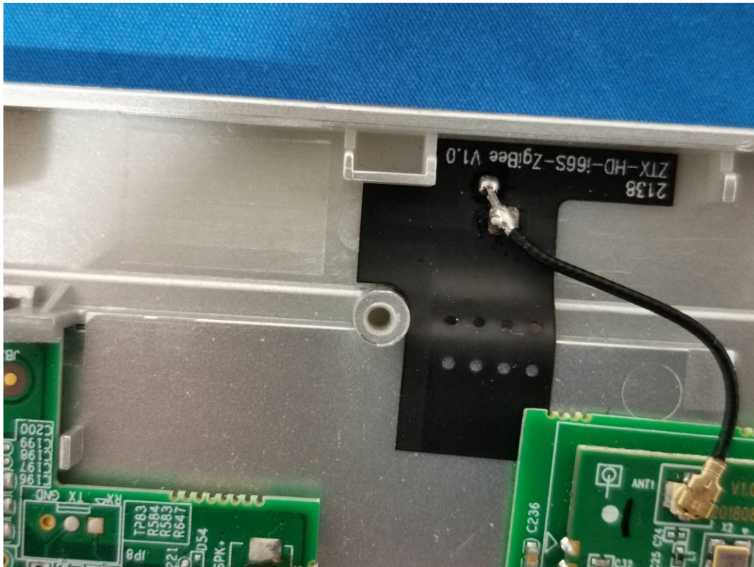
Zigbee Antenna
