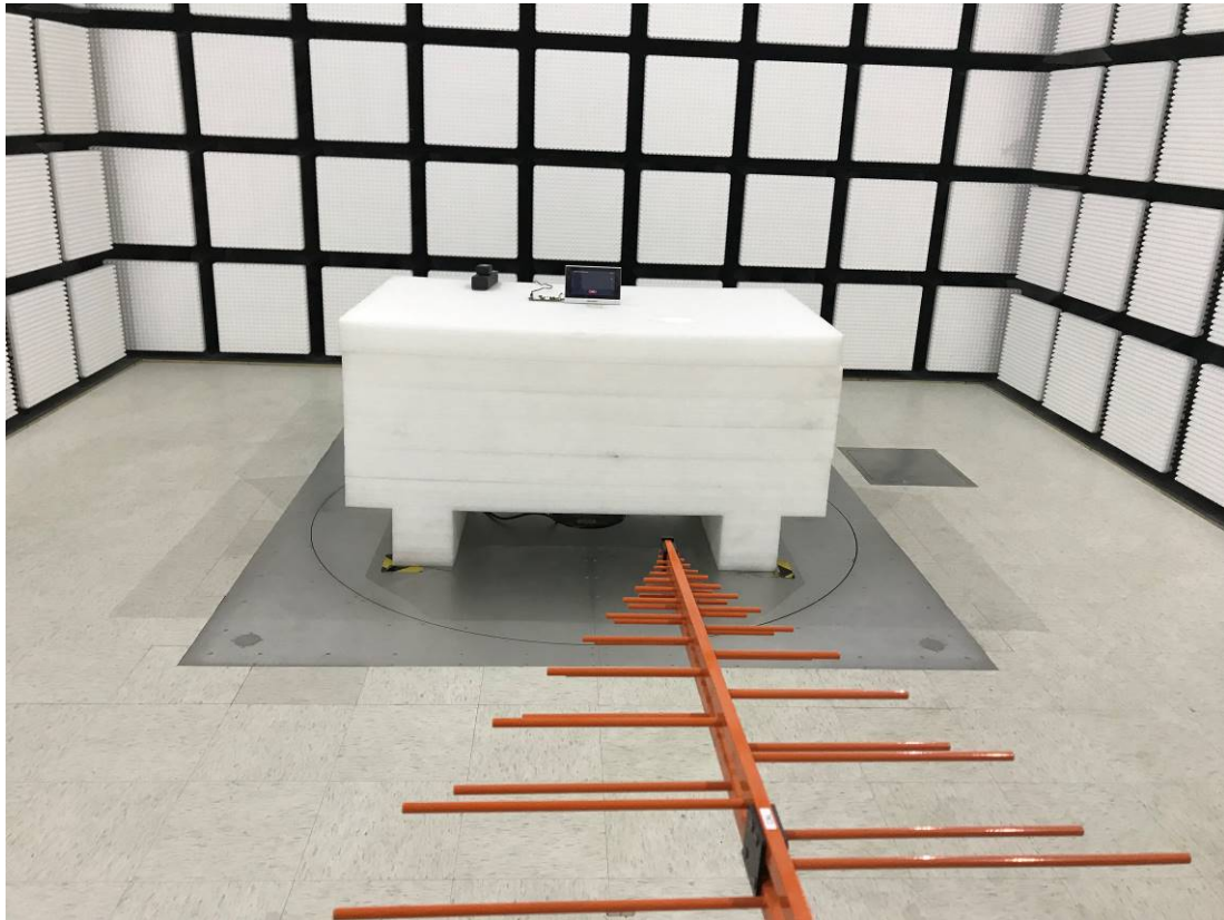
Radiated Emission Below 1GHz View- PoE power Supply mode
