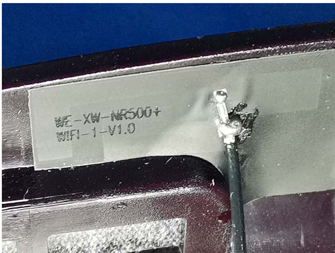
Wi-Fi Antenna 1
