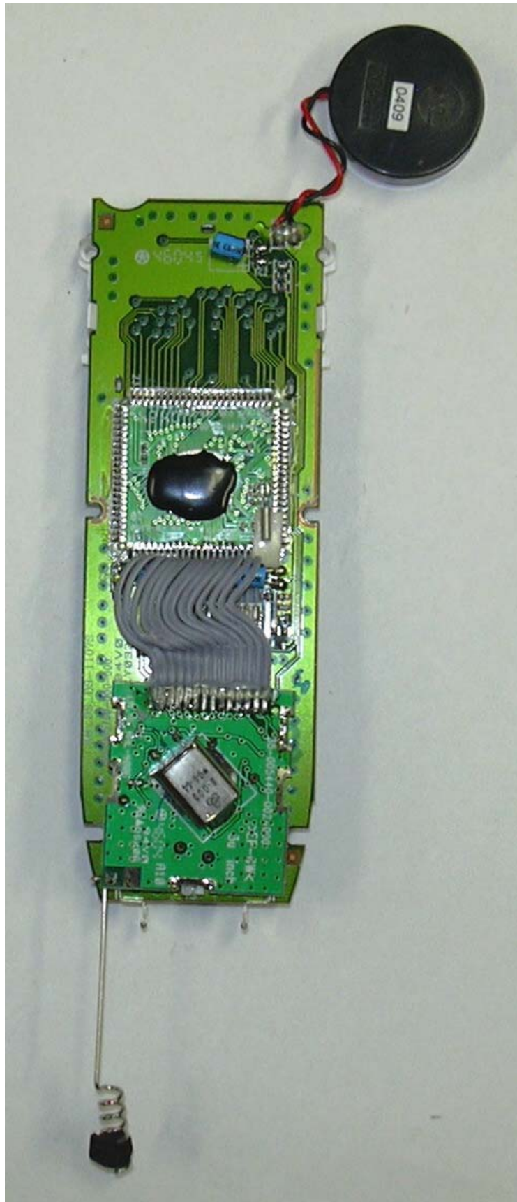
Vtech 2121 Handset PCB
