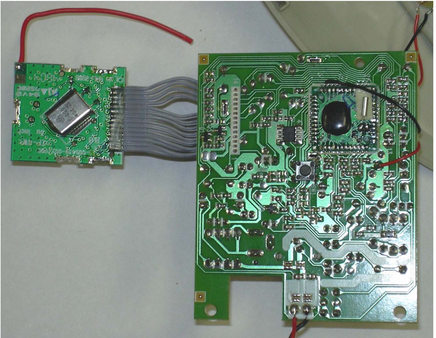
Vtech 2121 Base PCB
