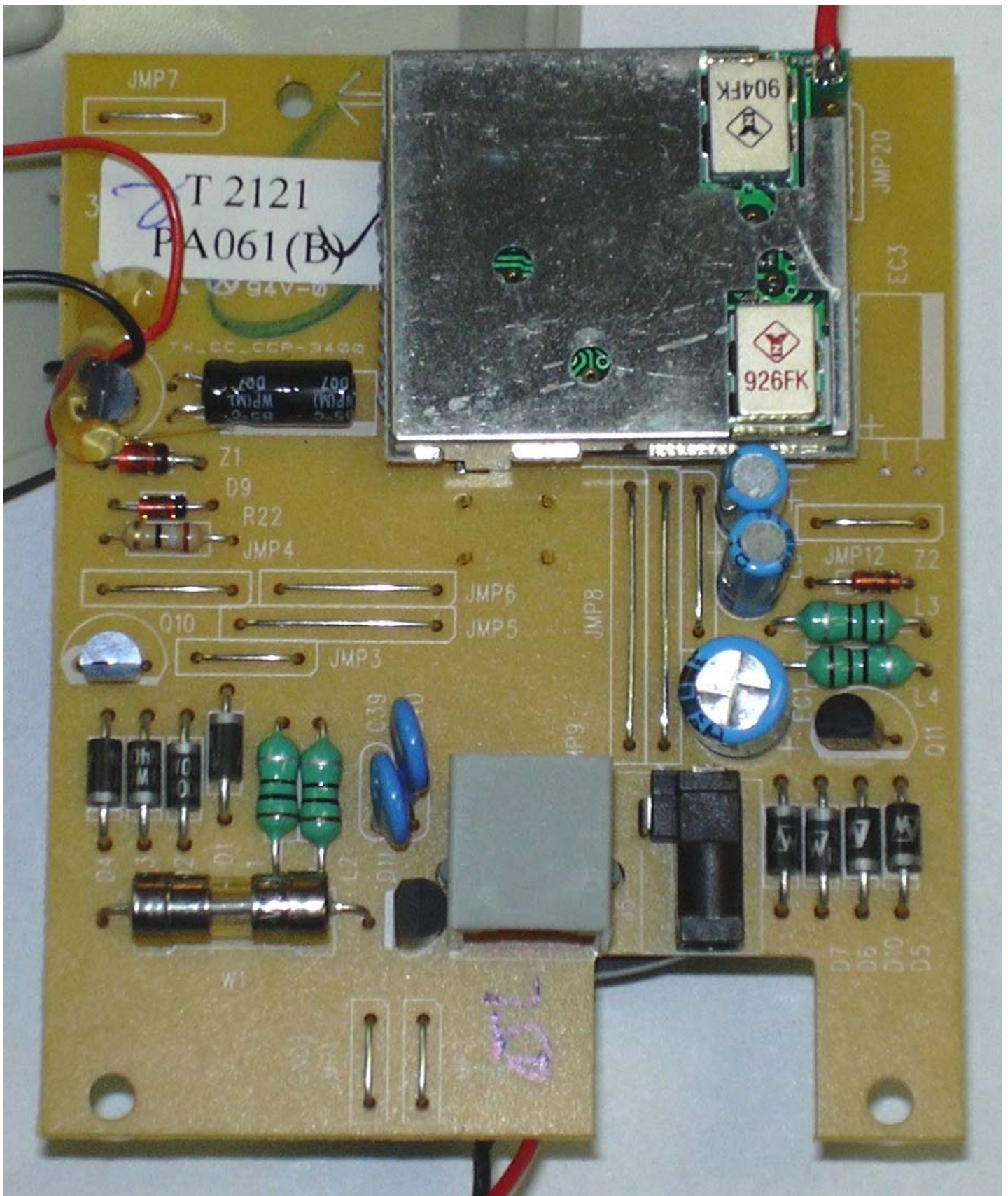
Vtech 2121 Base PCB
