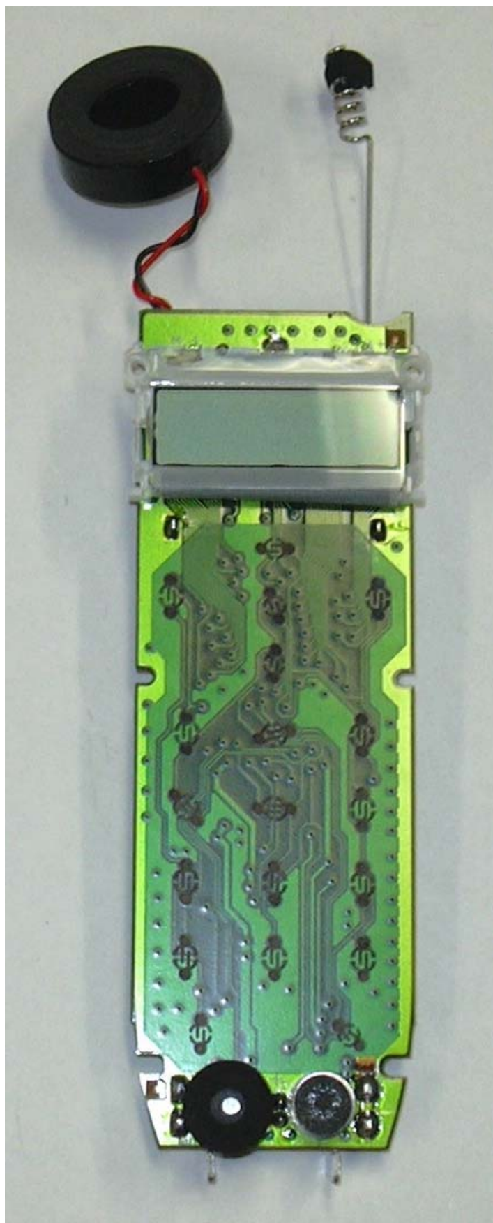
Vtech 2121 Handset PCB
