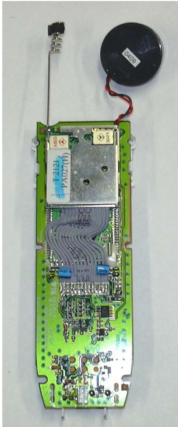
Vtech 2121 Handset PCB
