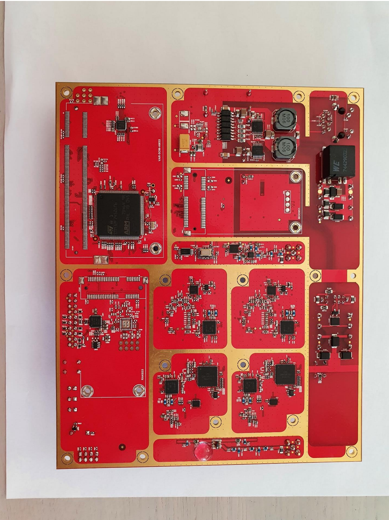
Bottom side of the Main Board PCBA without shields
