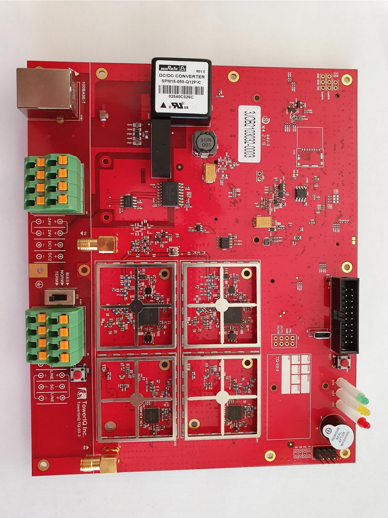
Top side of the Main Board PCBA without shields
