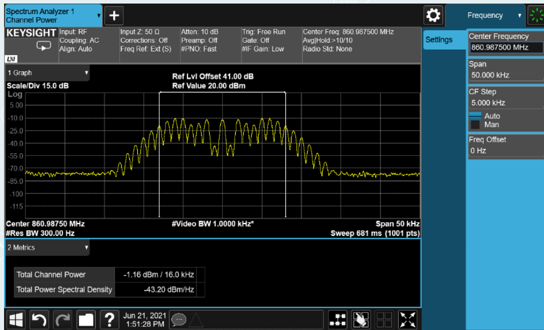
High Frequency: 860.9875MHz, Input occupied BW
