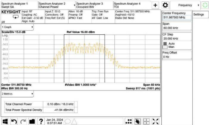
Input signal High Frequency: 511.9875MHz
