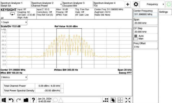
Input signal High Frequency: 511.99688MHz
