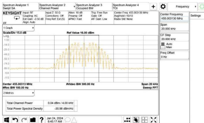
Input signal Low Frequency: 455.00313MHz
