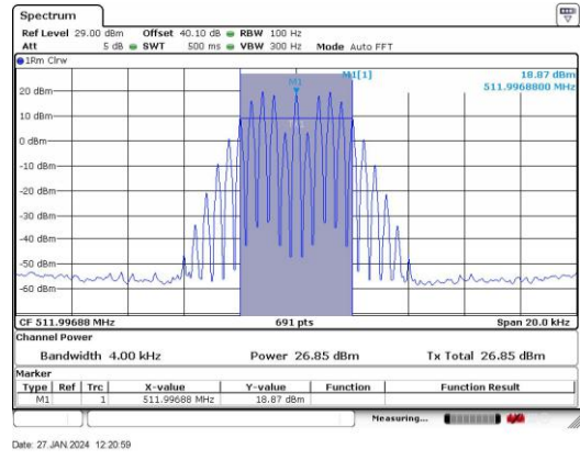
With the input signal amplitude set 3 dB above the AGC threshold High Frequency: 511.99688MHz
