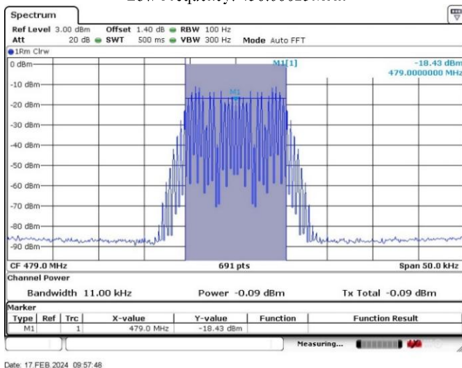
Input signal Middle Frequency: 479.0MHz
