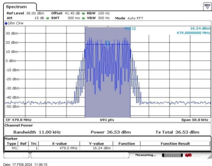
With the input signal amplitude set the AGC threshold Middle Frequency: 479.0MHz
