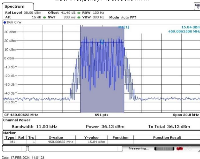
With the input signal amplitude set 3 dB above the AGC threshold Low Frequency: 450.00625MHz
