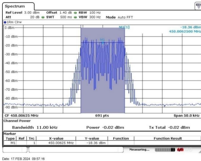
Input signal Low Frequency: 450.00625MHz
