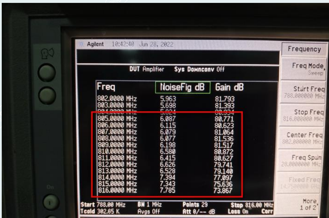
Uplink: 805MHz~816MHz
