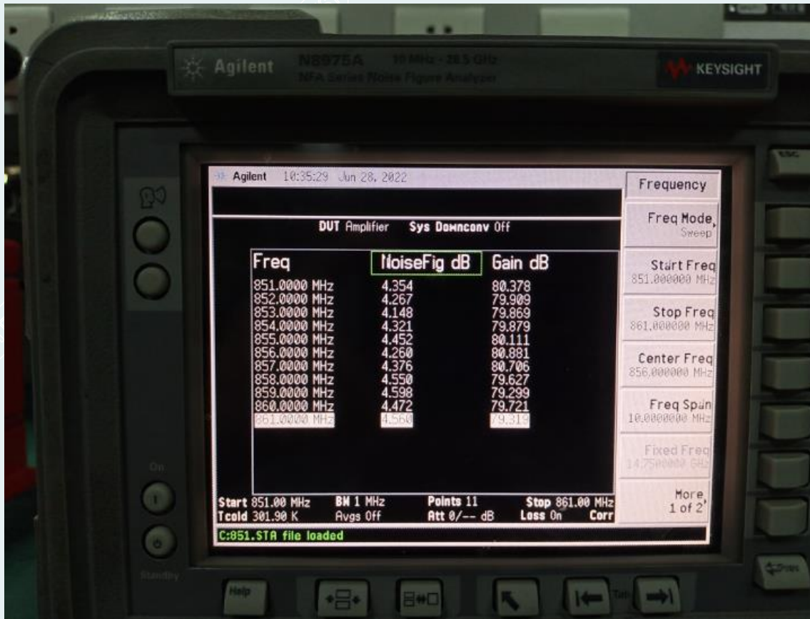
Downlink: 851MHz~861MHz
