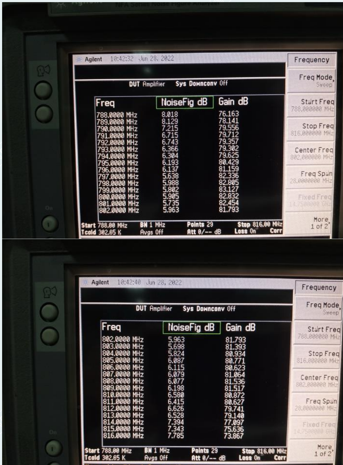
Uplink: 788MHz~805MHz
