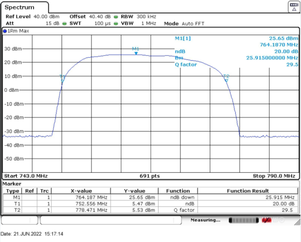
Downlink: 758MHz~775MHz
