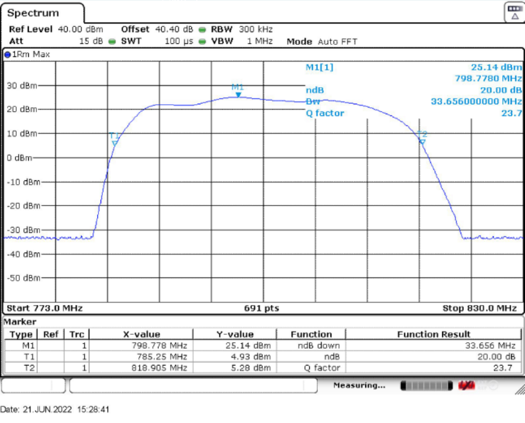
Uplink: 788MHz~816MHz
