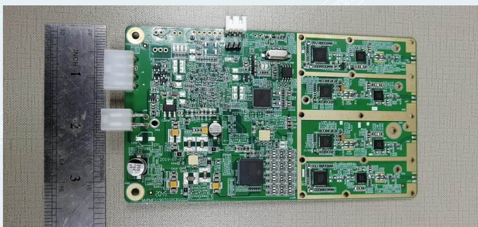
DIF Board-A
