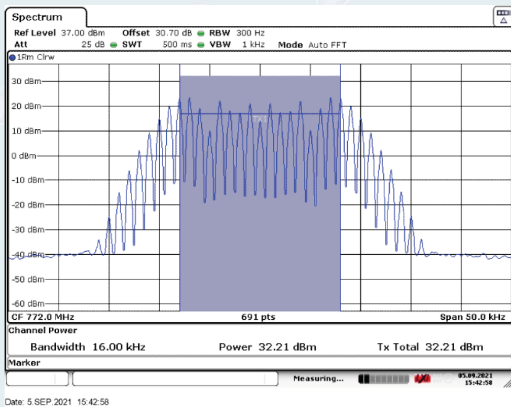
Middle Frequency: 772MHz, Output occupied BW (with the input signal amplitude set 3 dB above the AGC threshold)
