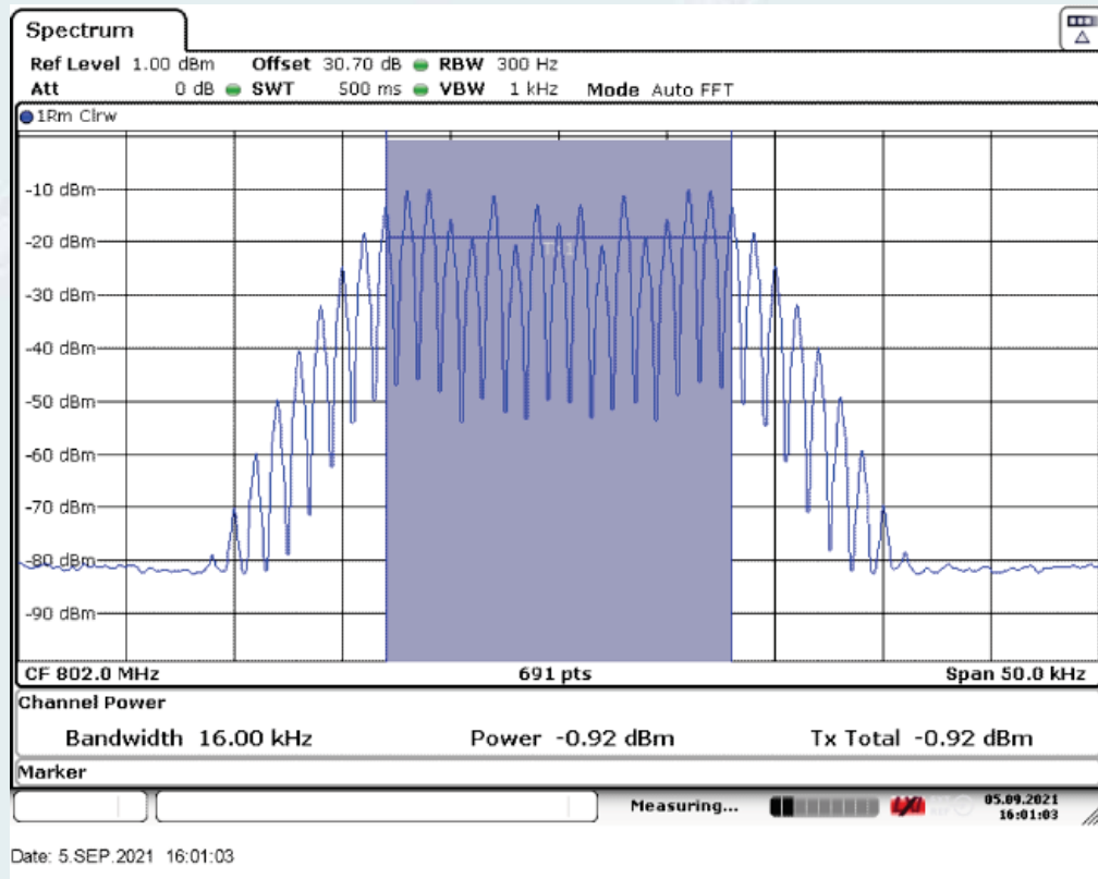
Middle Frequency: 802MHz, Input occupied BW
