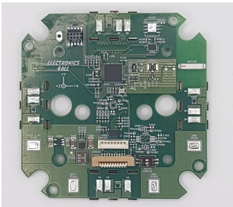
TP-400R8 Main Circuit Card Assembly Top
