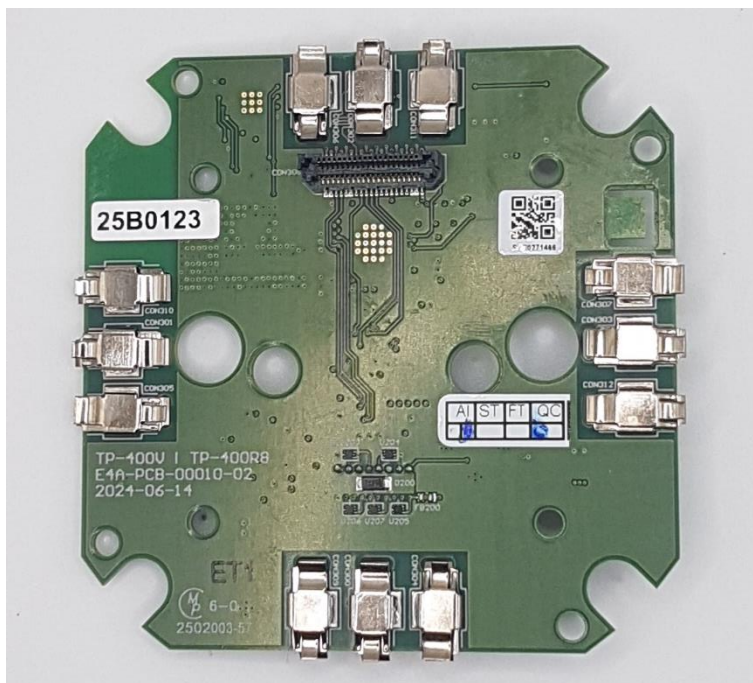
TP-400R8 Main Circuit Card Assembly Bottom
