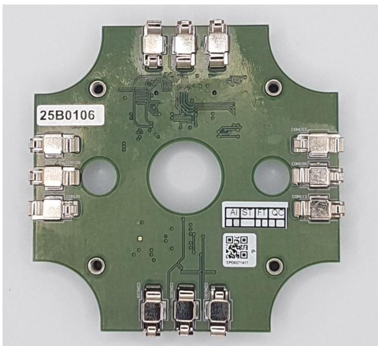
TP-400R8 Analog Daughter Circuit Card Assembly Bottom
