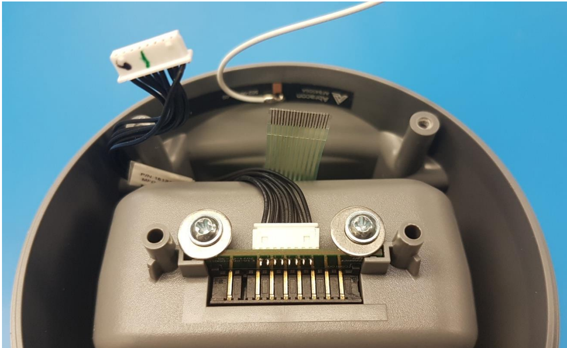
TP-400R8 Top Enclosure Interior View
