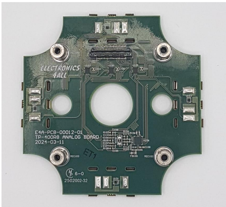
TP-400R8 Analog Daughter Circuit Card Assembly Top
