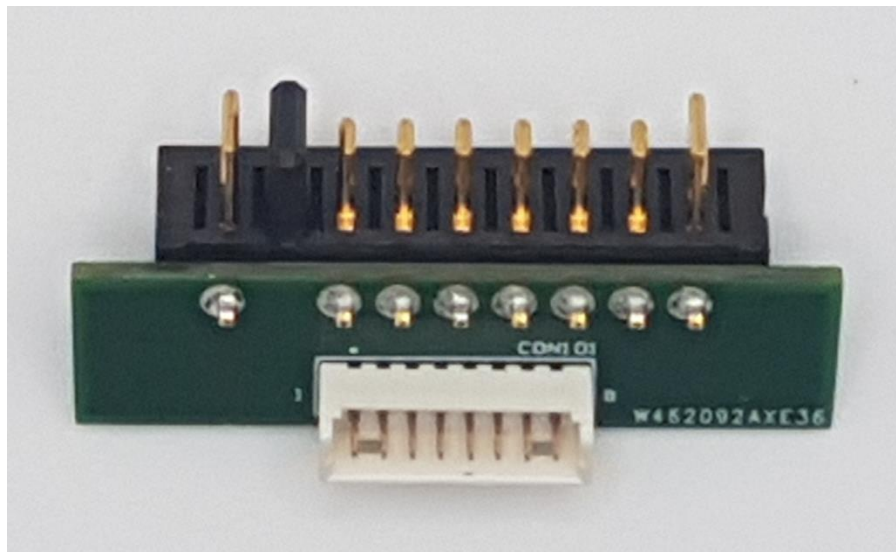
TP-400 Battery Connector Circuit Card Assembly Bottom
