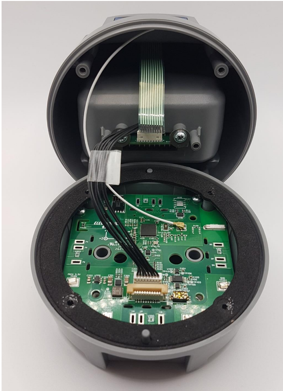
TP-400V Assembly with Top Enclosure Opened
