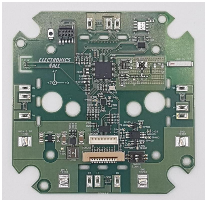
TP-400V Main Circuit Card Assembly Top
