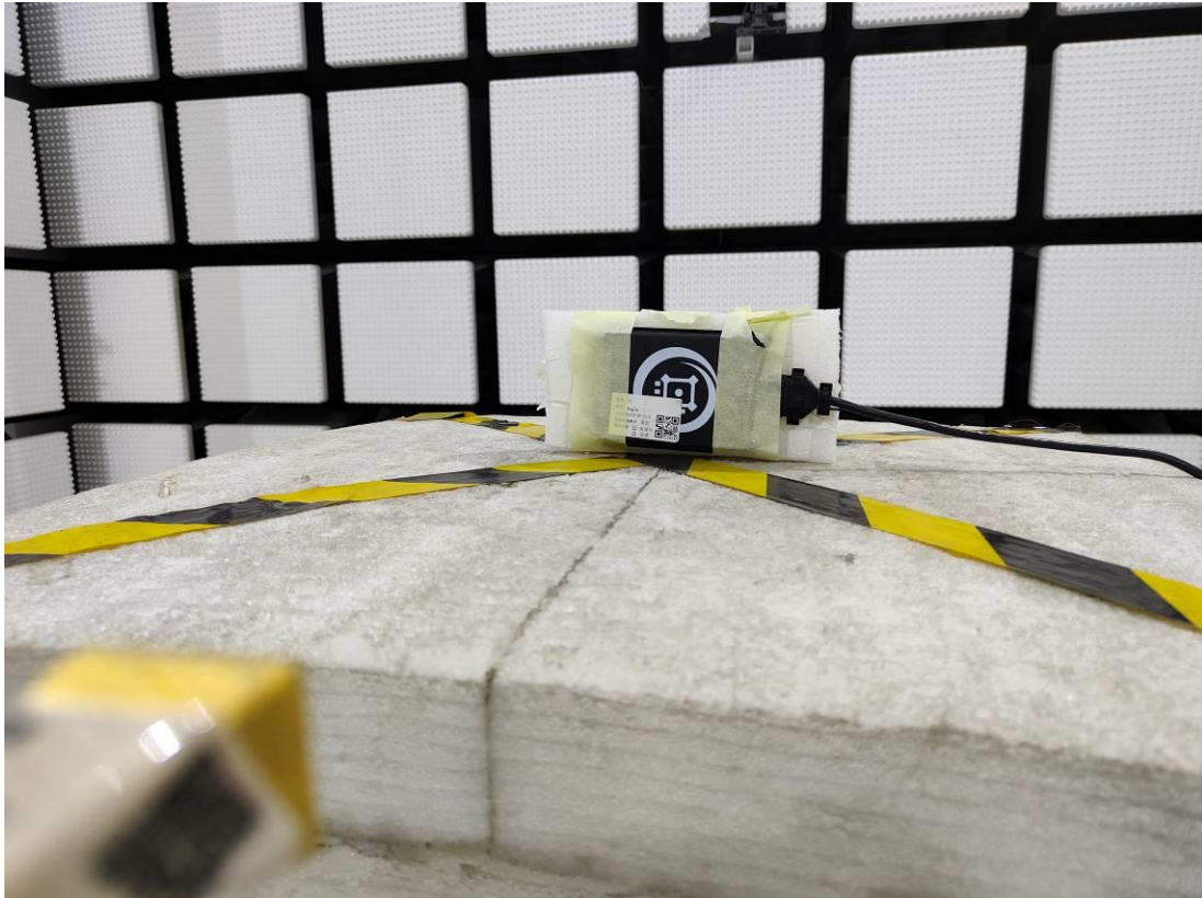
Radiated Emission 90GHz - 140GHz View
