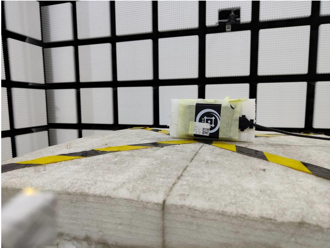
Radiated Emission 220GHz - 231GHz View
