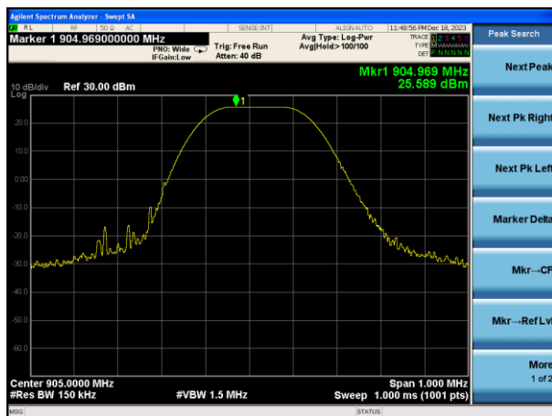
Peak output Power plot on channel 00
