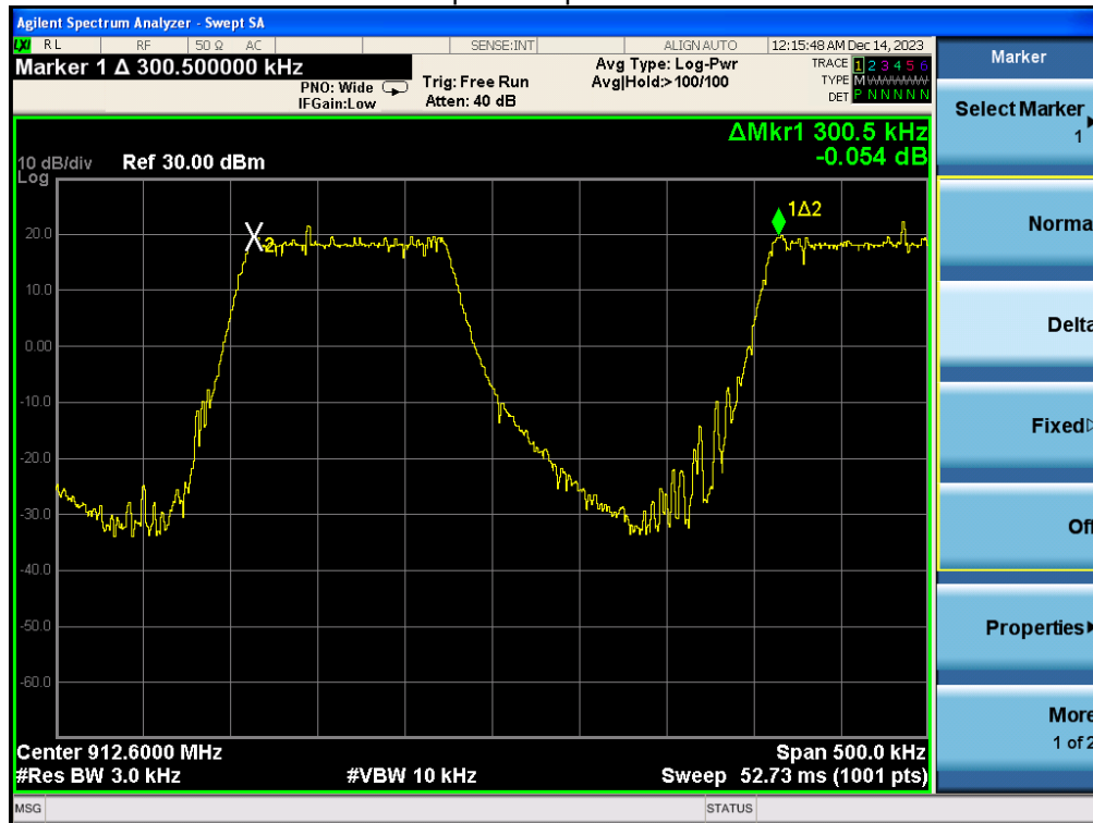
Channel Separation plot on channel 48-49
