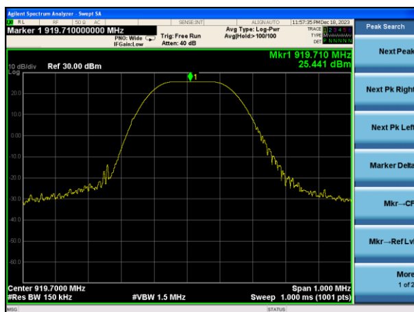
Peak output Power plot on channel 49
