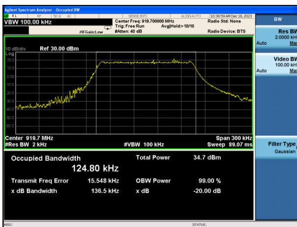
20dB Bandwidth plot on channel 49
