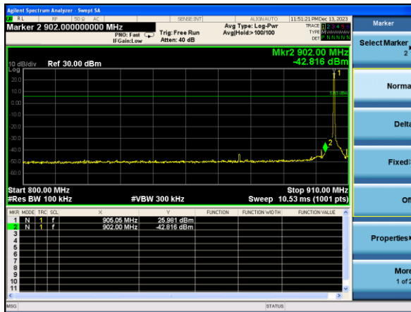
LORA: Band Edge-Low Channel
