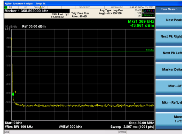
LORA on channel 00
