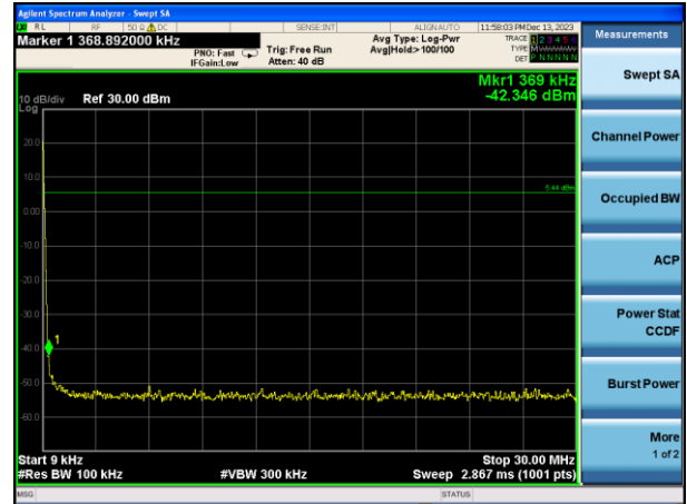
LORA on channel 49
