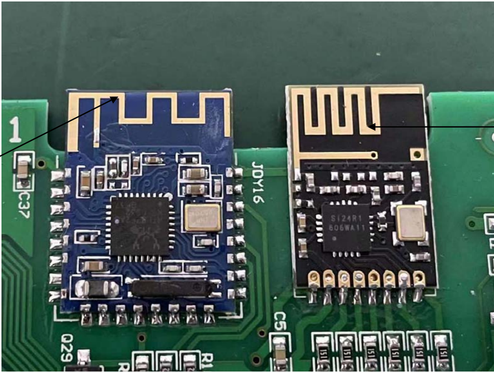
2.4G SRD antenna
