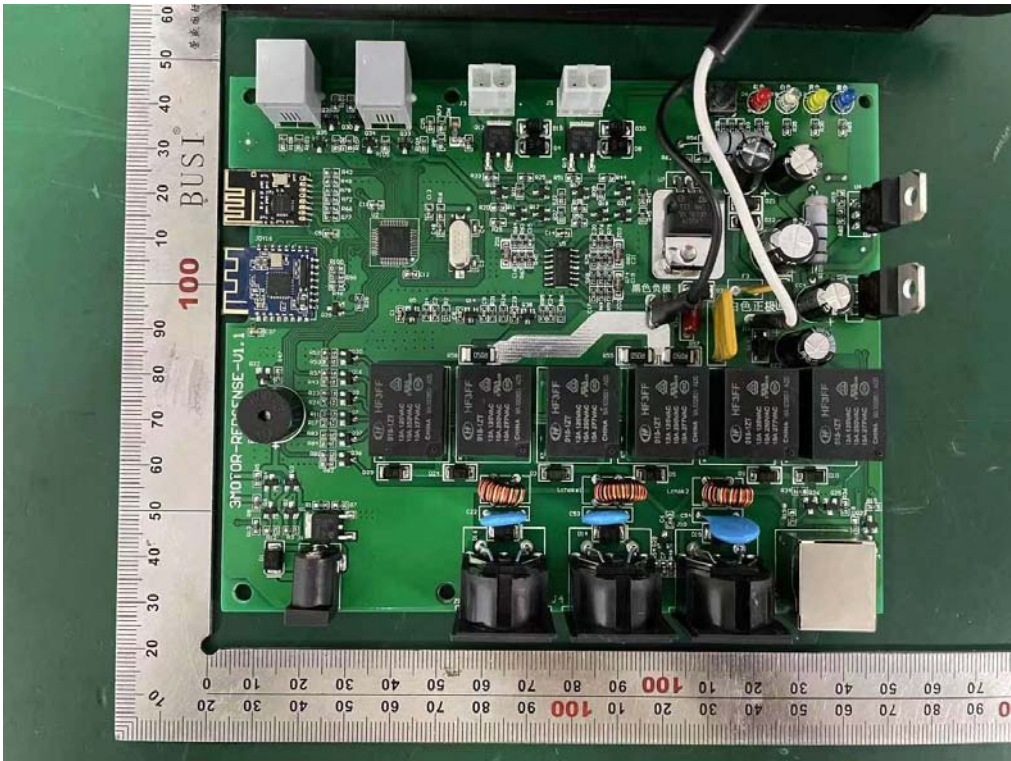
Internal photos M/N: S3A
