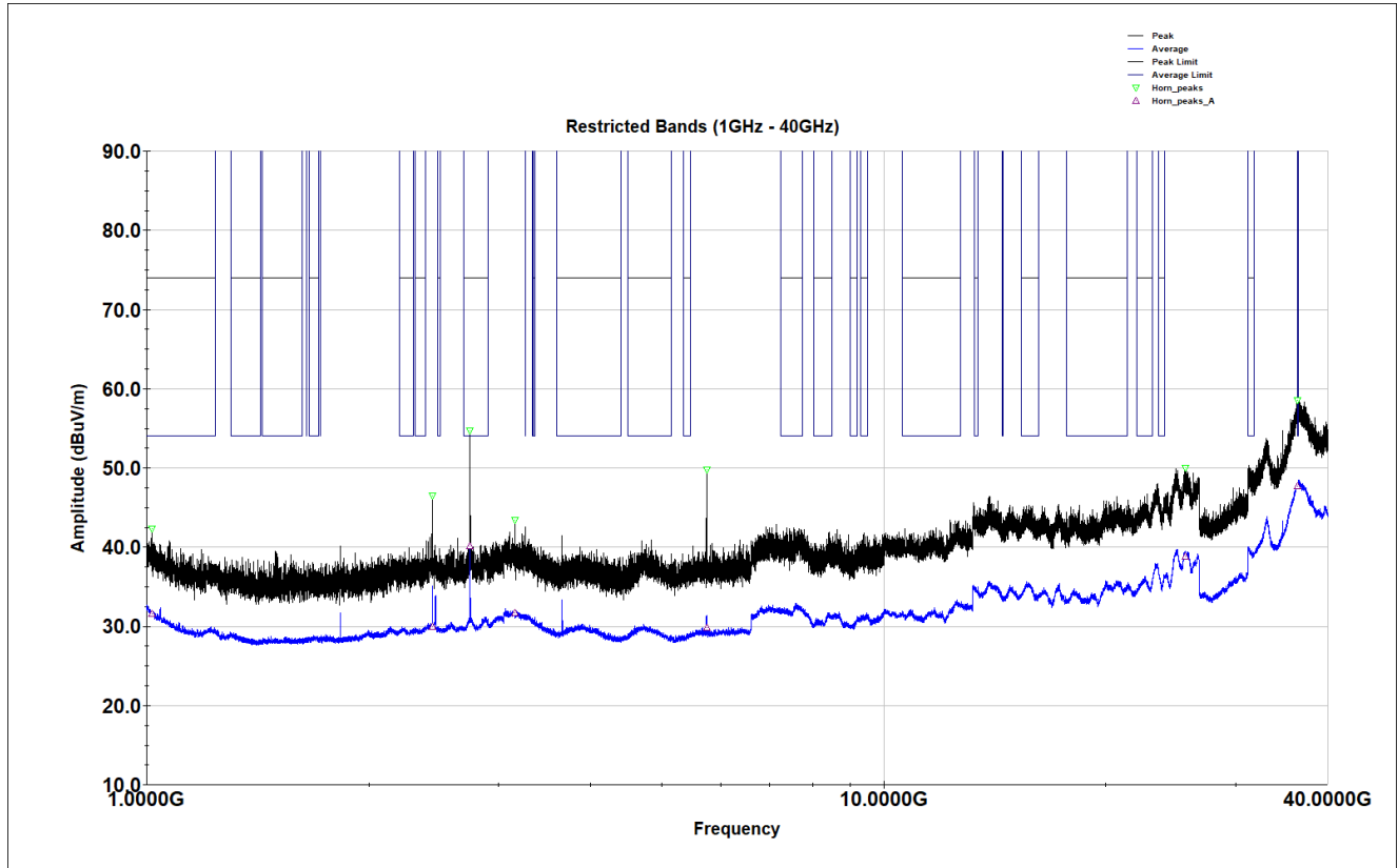
Figure 17. Middle Channel, 1GHz – 40GHz Restricted Band Spurious Emissions
