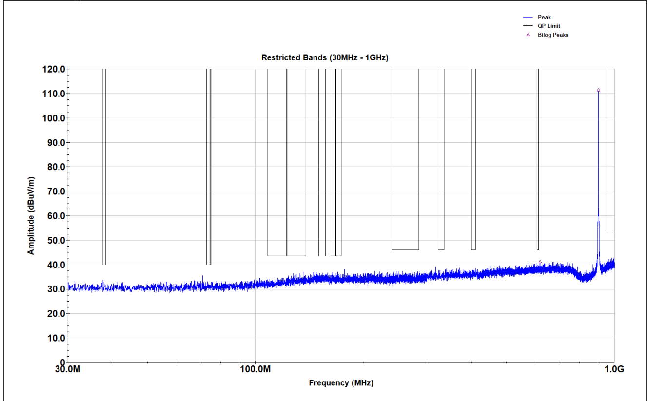
Figure 14. Low Channel, 30MHz – 1GHz Restricted Band Spurious Emissions
