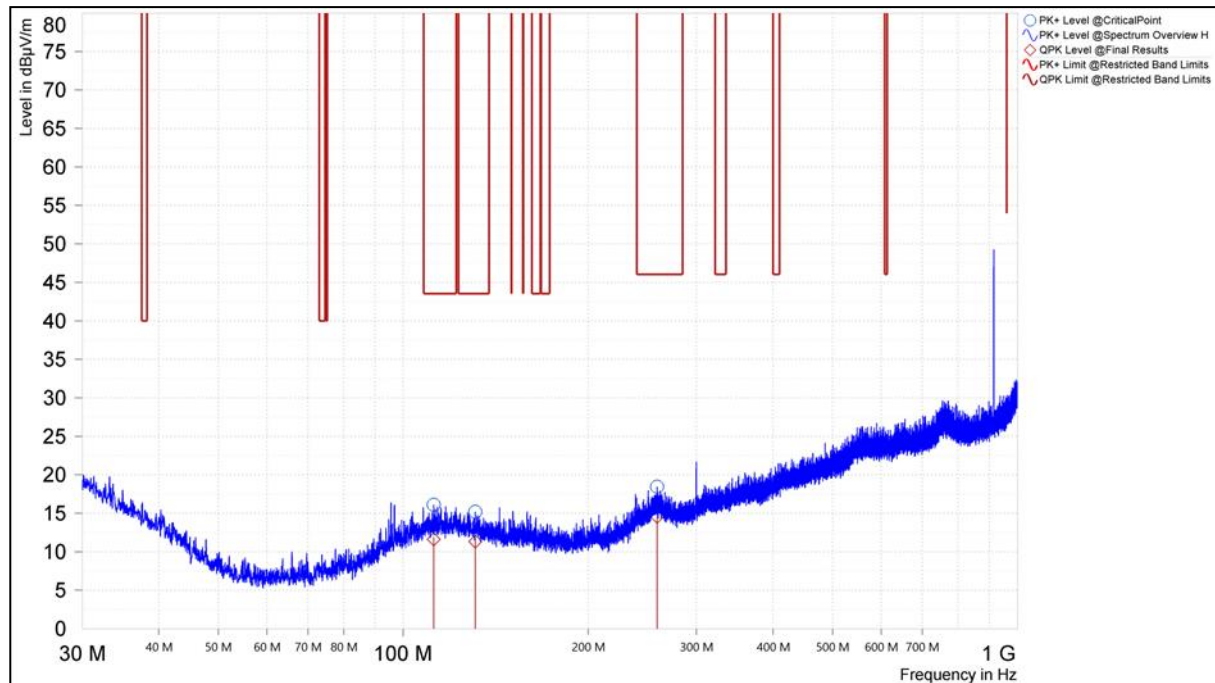
Figure 25. Worst Case Cabinet Radiation, 30MHz – 1GHz, Horizontal Polarity
