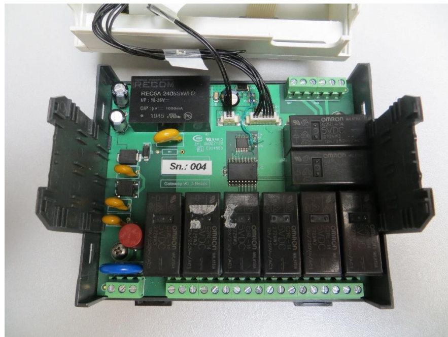
PCB relay top
