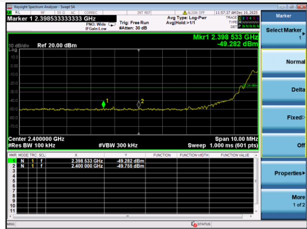
GFSK (1Mbps) LOW CHANNEL, BAND EDGE
