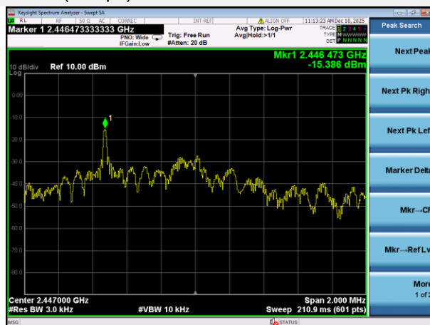
GFSK (2Mbps) MIDDLE CHANNEL
