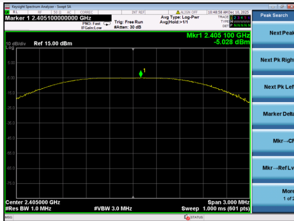
GFSK (1Mbps) LOW CHANNEL
