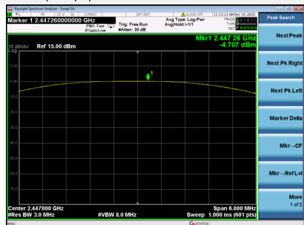
GFSK (2Mbps) MIDDLE CHANNEL
