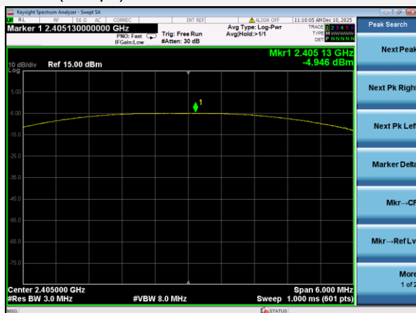
GFSK (2Mbps) LOW CHANNEL
