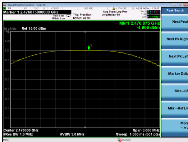
GFSK (1Mbps) HIGH CHANNEL
