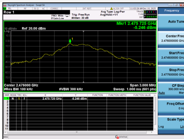
GFSK (1Mbps) HIGH CHANNEL, CARRIER LEVEL
