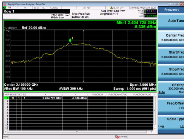
GFSK (1Mbps) LOW CHANNEL, CARRIER LEVEL
