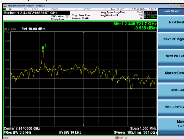
GFSK (1Mbps) MIDDLE CHANNEL
