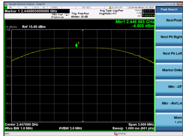
GFSK (1Mbps) MIDDLE CHANNEL
