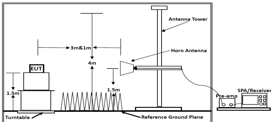
Above 1GHz
