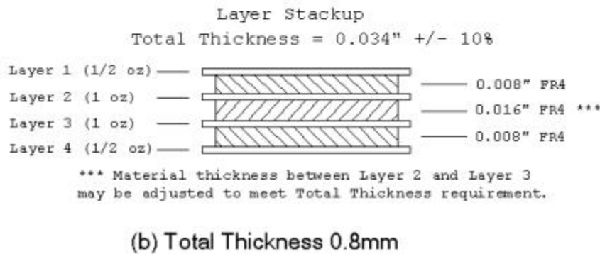
Figure 2.2. Board Stackup
