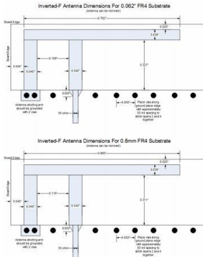
Figure 2.1. Antenna Dimensions
