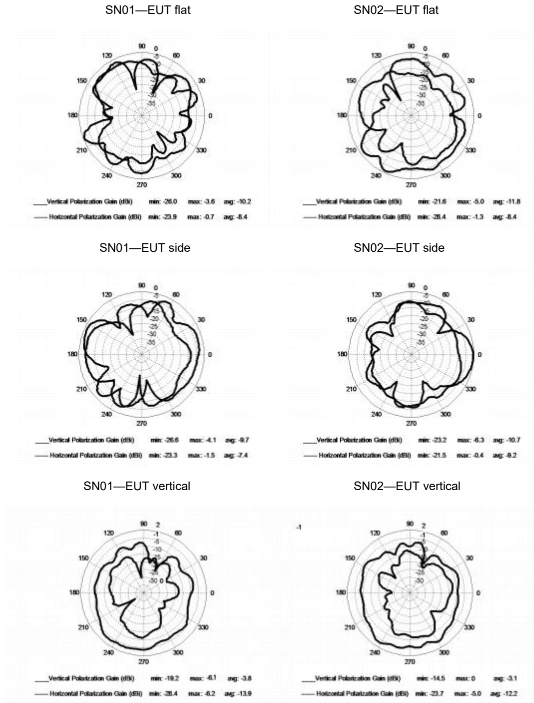
Figure 4.4. Measured Antenna Patterns for EM250 62 mil Boards
