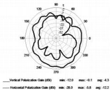
Figure 4.6. Measured Antenna Patterns for EM250 0.8 mm Boards
