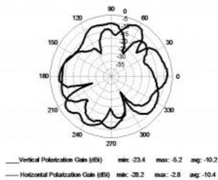
SN02—EUT vertical
