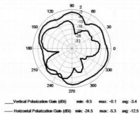
Figure 4.5. Measured Antenna Patterns for EM260 62 mil Boards
