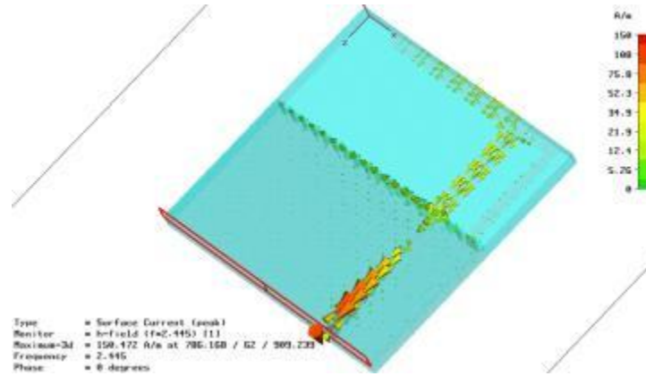
Figure 3.1. Surface Current
