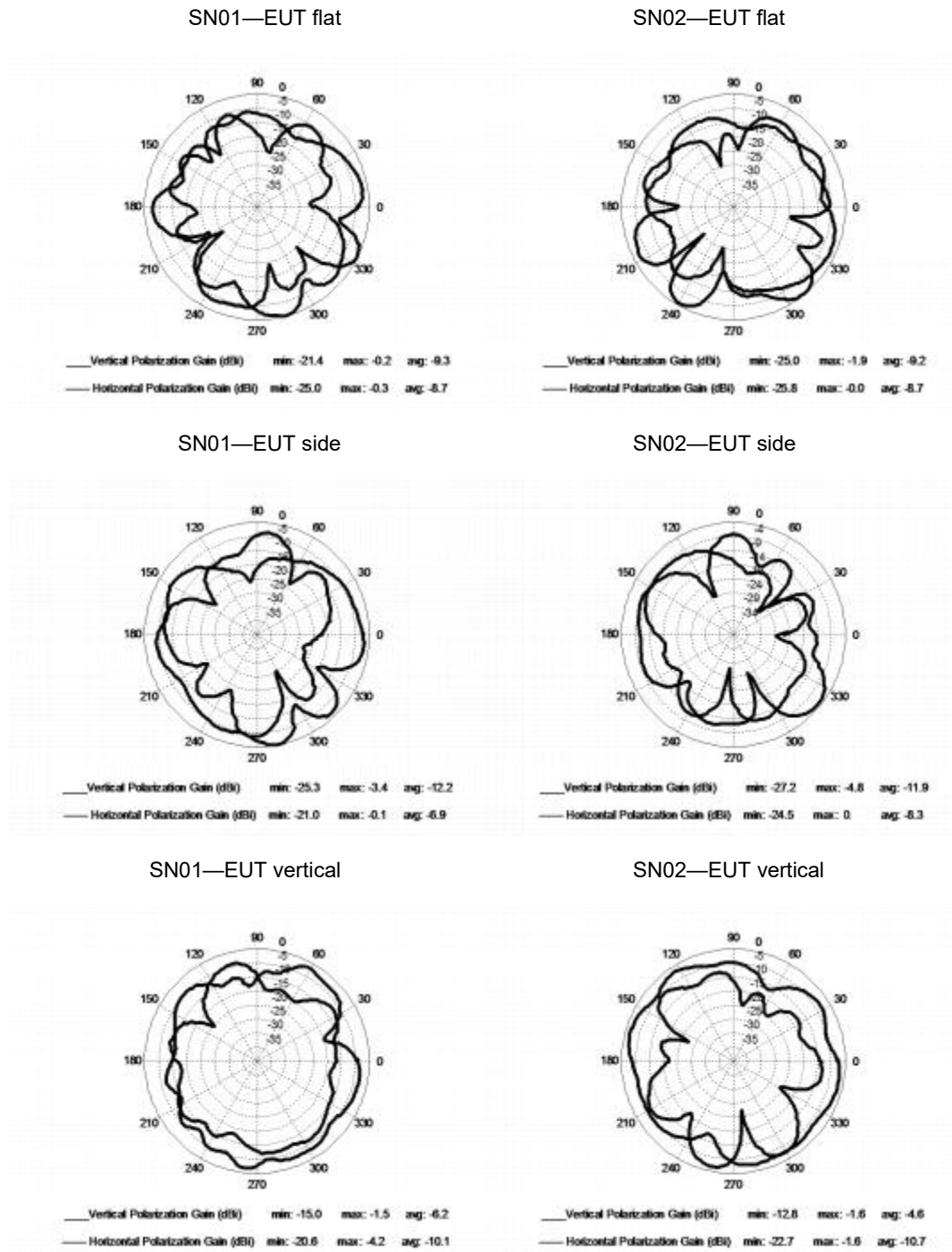
Figure 4.7. Measured Antenna Patterns for EM260 0.8 mm Boards
