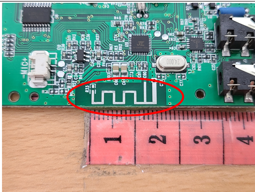
FMT Antenna
