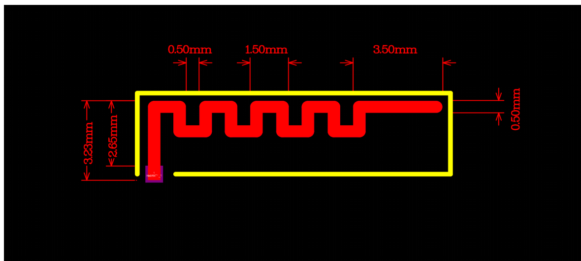
Antenna Photo &amp; Length (mm)
