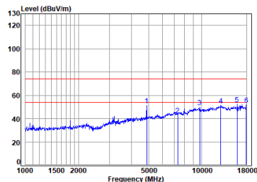
BT_3DH5_TX_CH_39_Vertical
