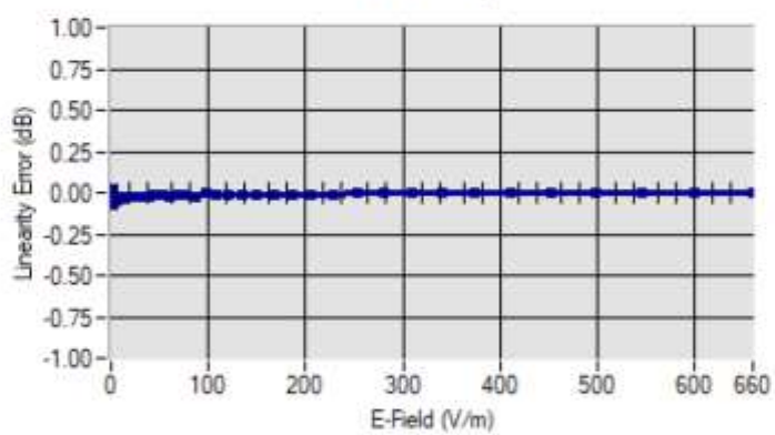
Linearity
