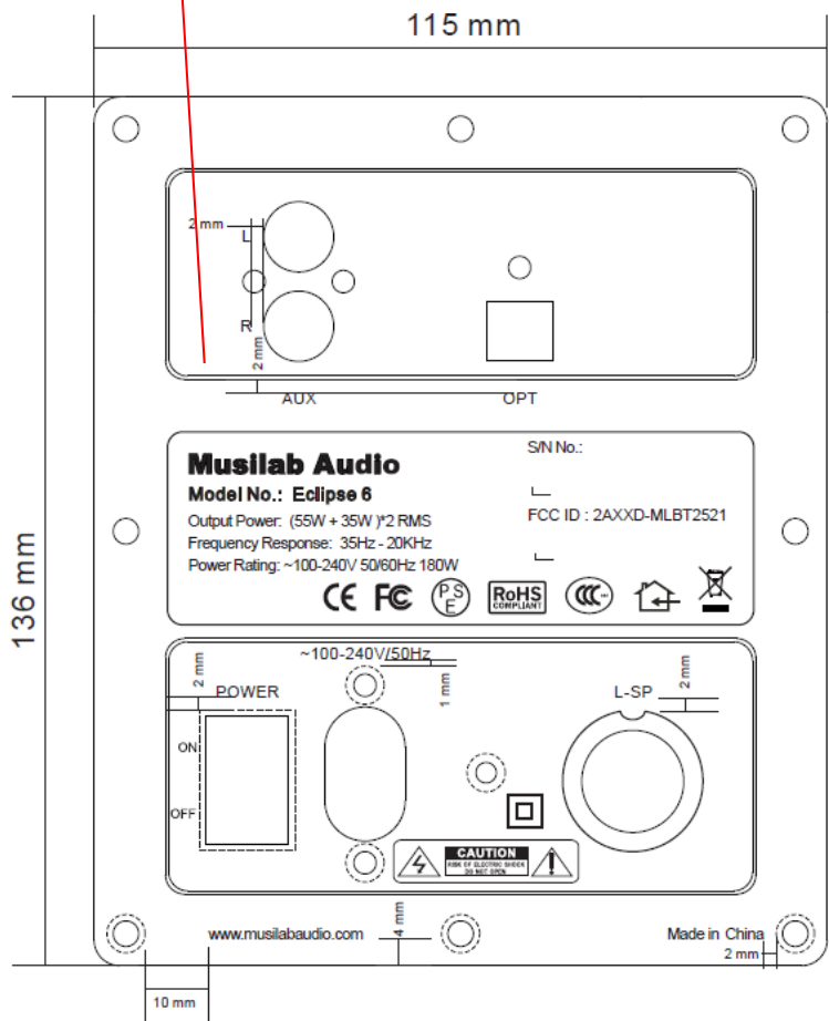
Label Location
