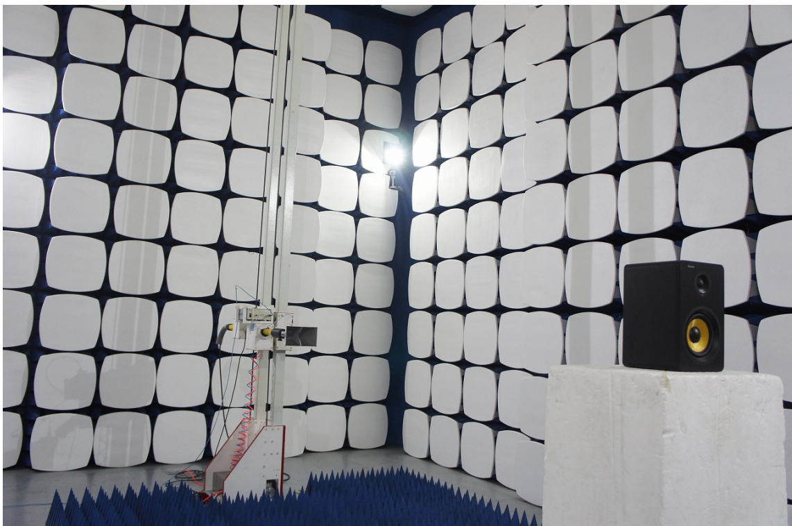
Radiated Setup photo (Above 1G)
