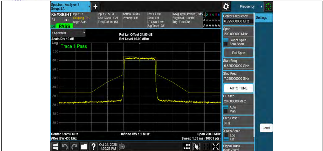
NTNV-11AX40MIMO-Ant3-6925-PASS
