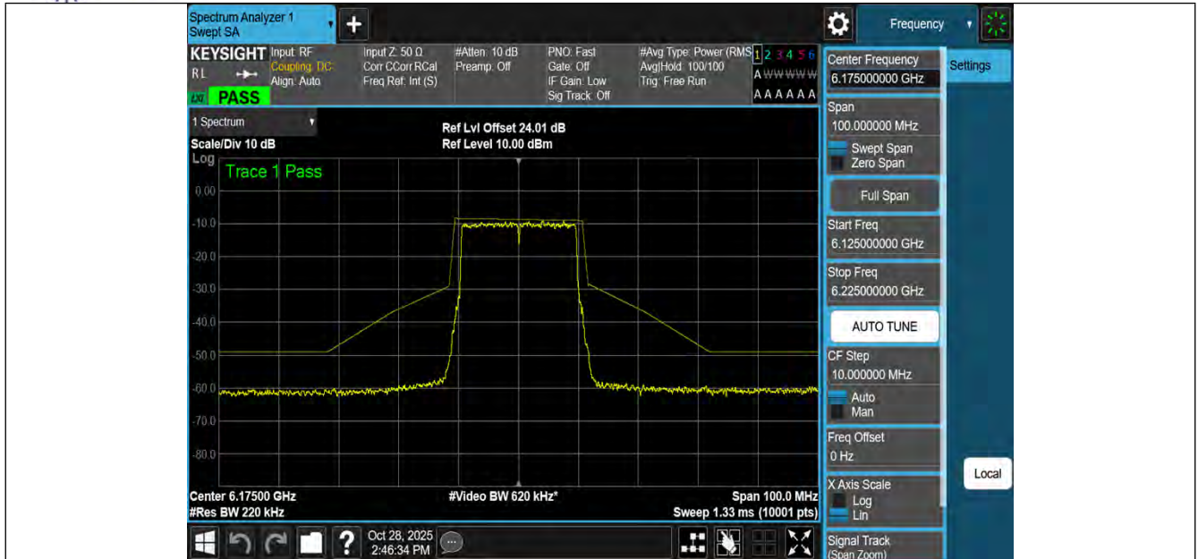
NTNV-11BE20MIMO-Ant3-6175-PASS
