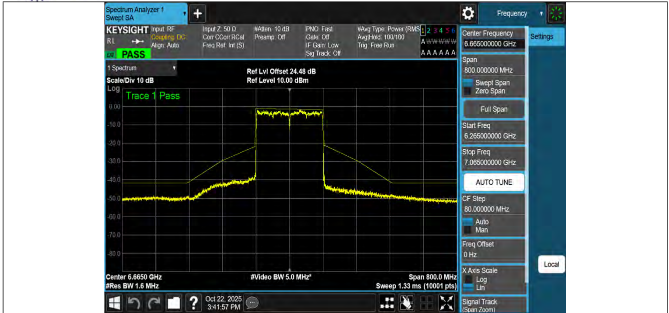
NTVN-11AX160MIMO-Ant3-6665-PASS
