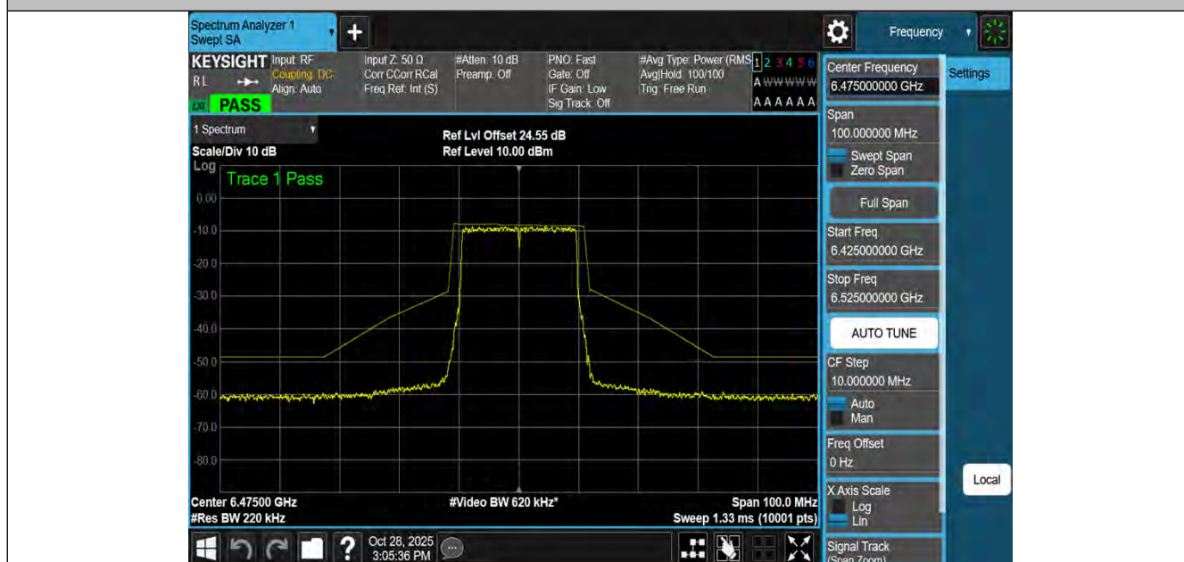
NTNV-11BE20MIMO-Ant4-6475-PASS
