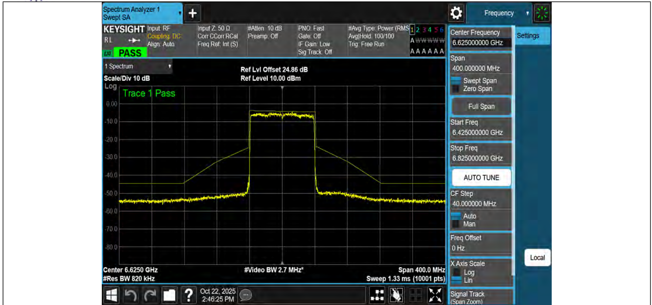
NTNV-11AX80MIMO-Ant3-6625-PASS
