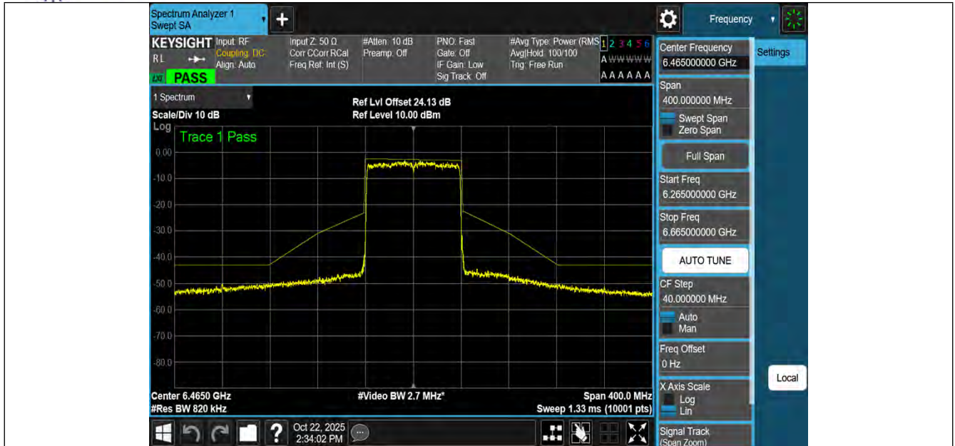
NTNV-11AX80MIMO-Ant1-6465-PASS
