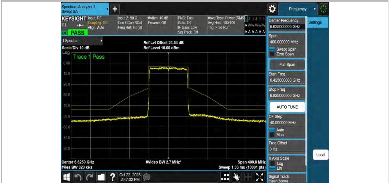
NTNV-11AX80MIMO-Ant4-6625-PASS
