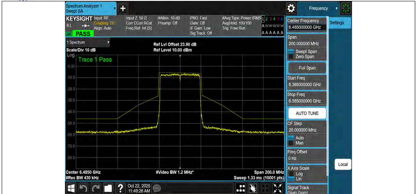
NTNV-11AX40MIMO-Ant1-6485-PASS
