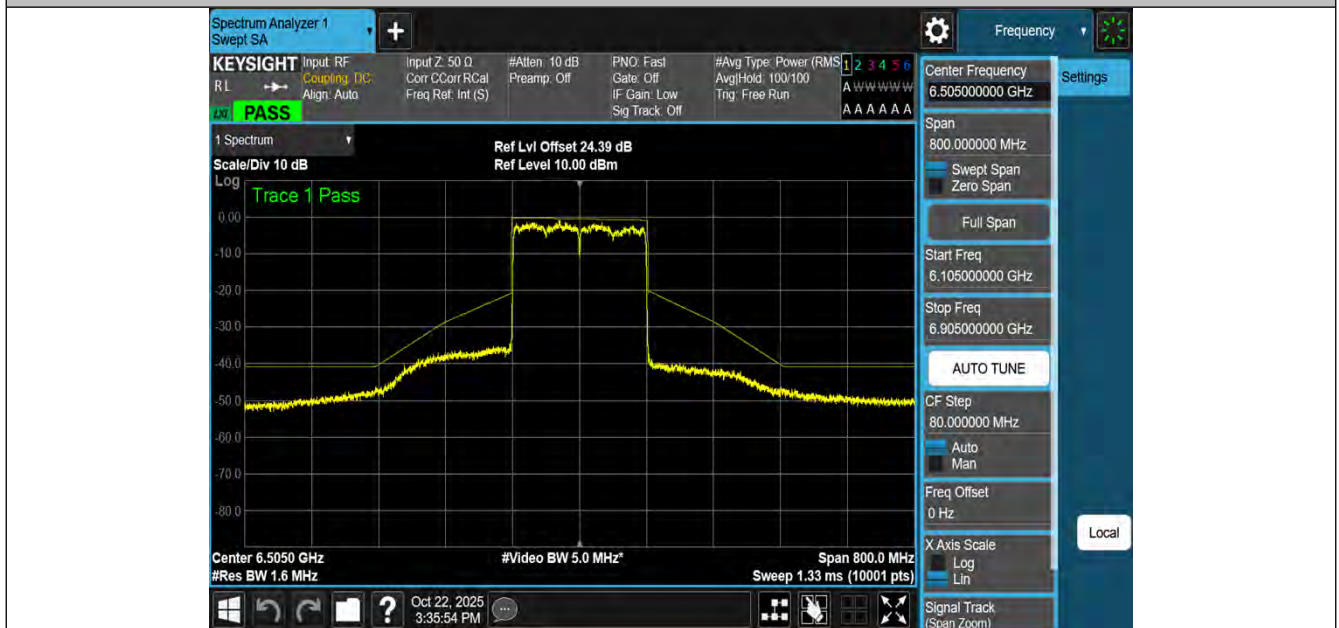
NTNV-11AX160MIMO-Ant2-6505-PASS
