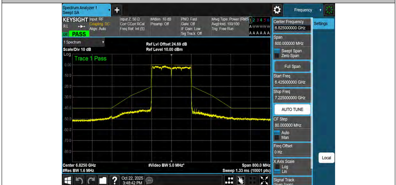
NTVN-11AX160MIMO-Ant4-6825-PASS
