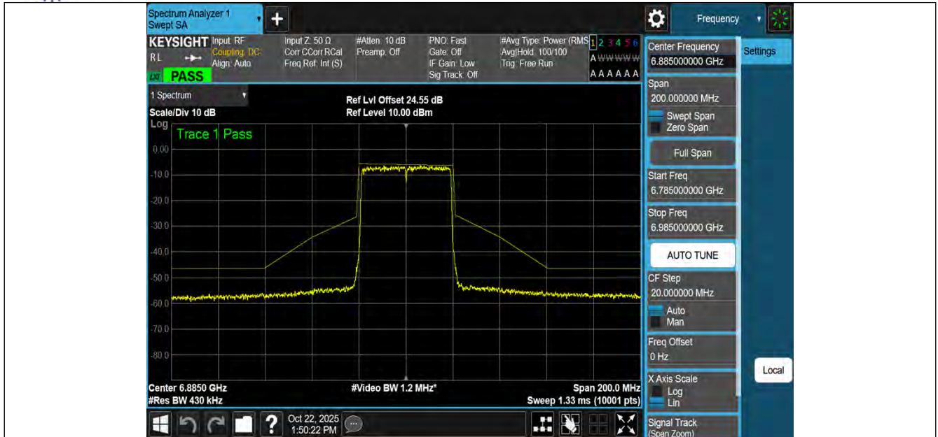
NTNV-11AX40MIMO-Ant3-6885-PASS
