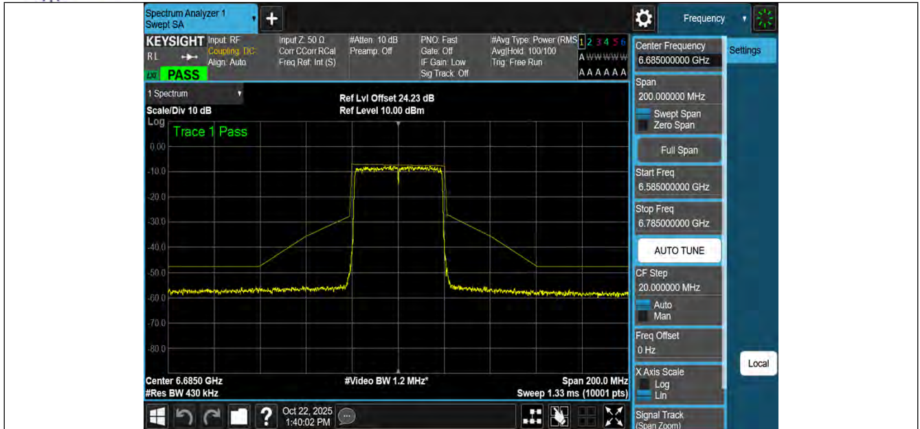
NTNV-11AX40MIMO-Ant3-6685-PASS
