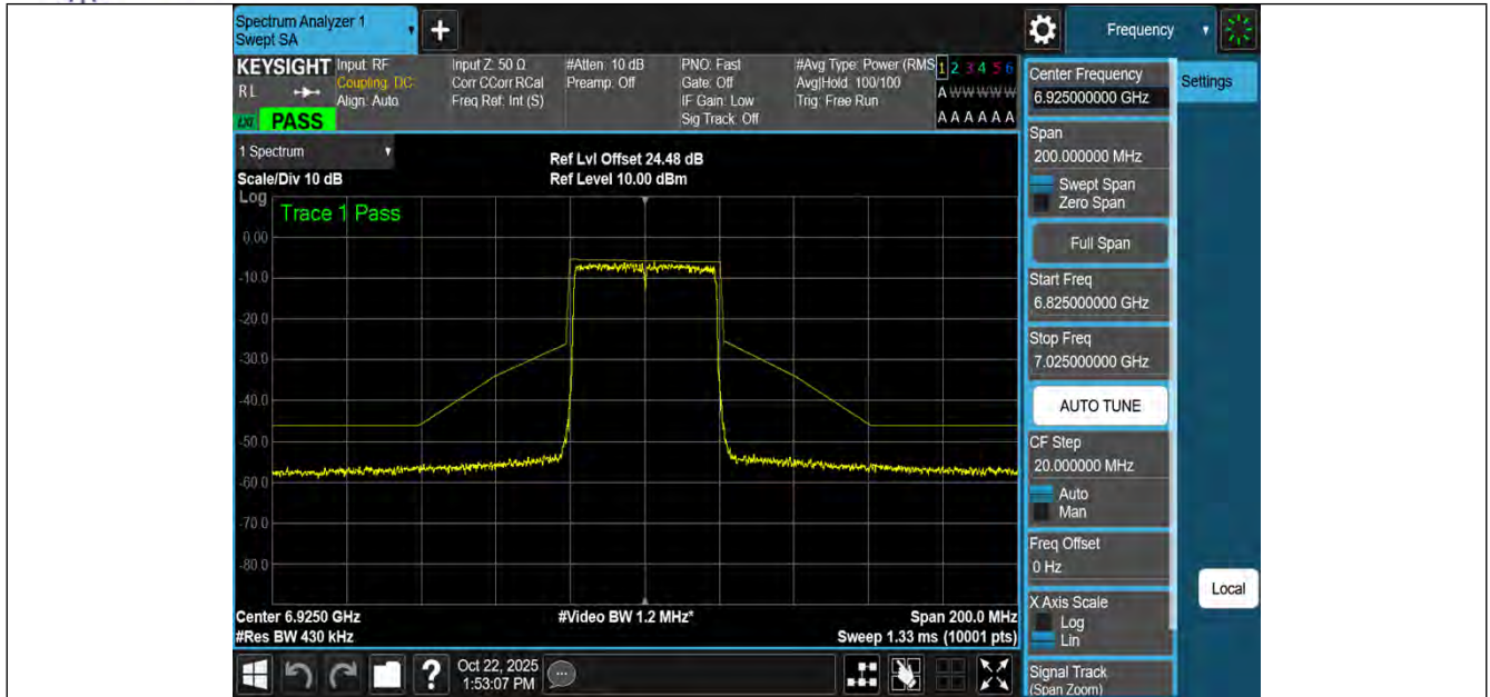
NTNV-11AX40MIMO-Ant1-6925-PASS
