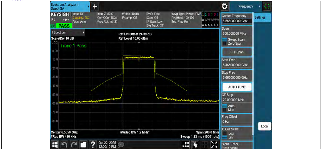
NTNV-11AX40MIMO-Ant1-6565-PASS
