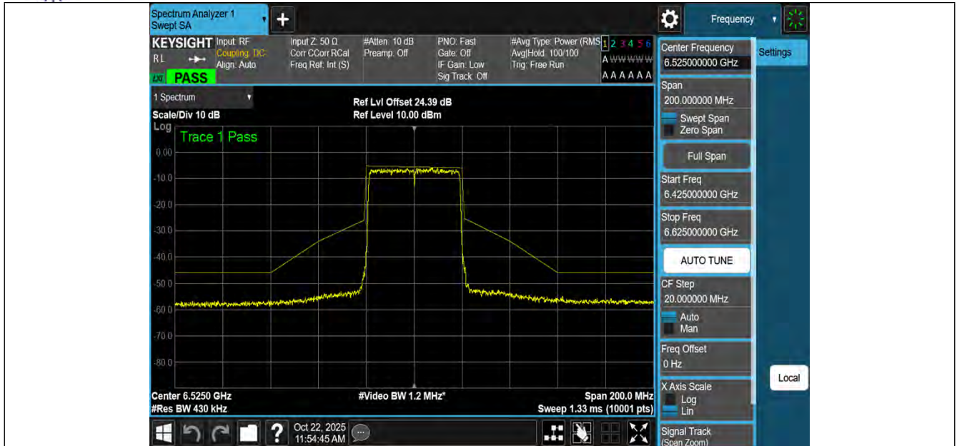
NTNV-11AX40MIMO-Ant1-6525-PASS
