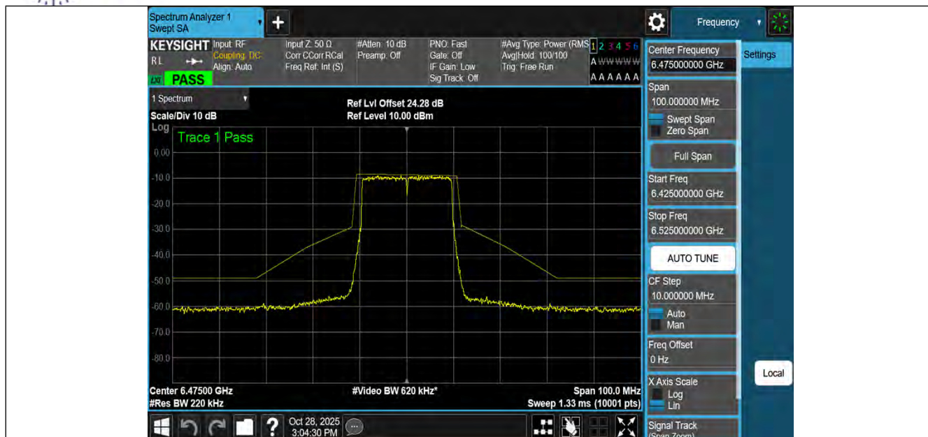
NTNV-11BE20MIMO-Ant3-6475-PASS
