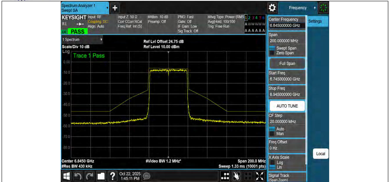
NTNV-11AX40MIMO-Ant3-6845-PASS
