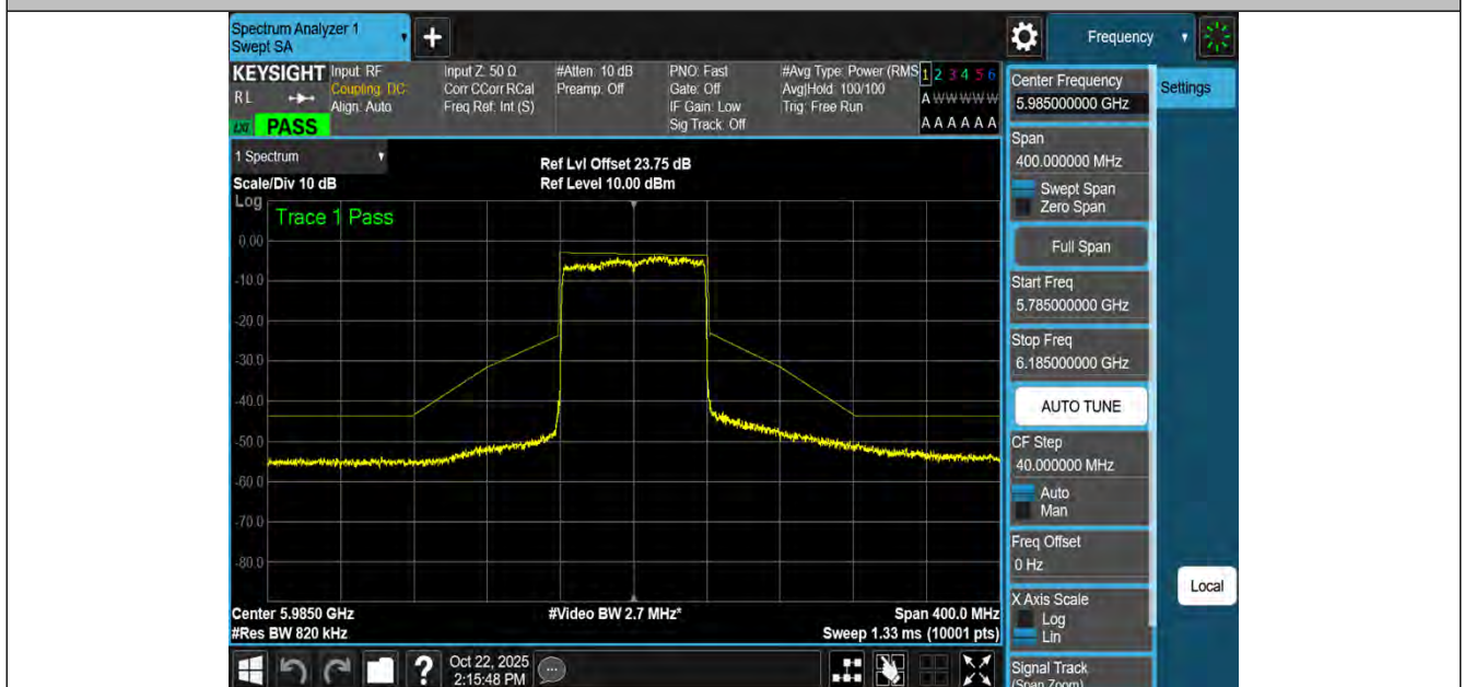
NTNV-11AX80MIMO-Ant4-5985-PASS
