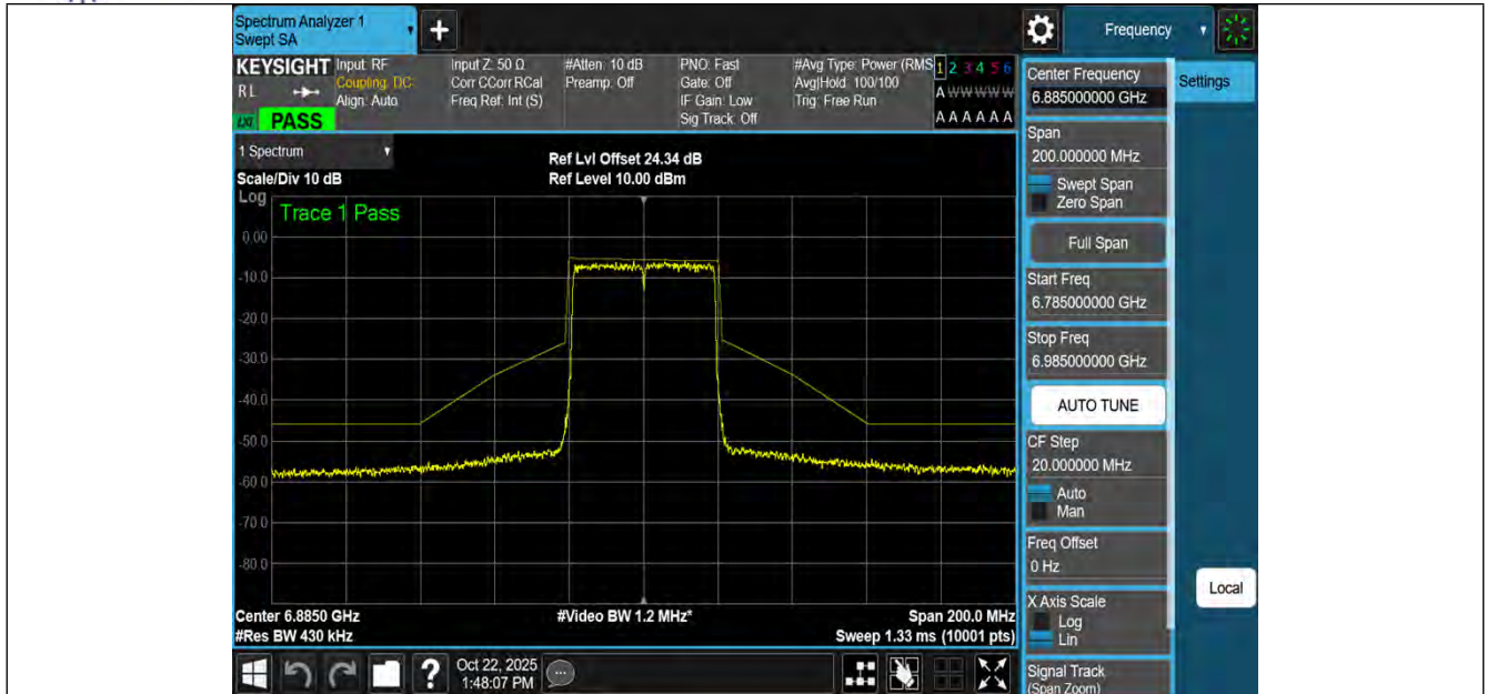
NTNV-11AX40MIMO-Ant1-6885-PASS
