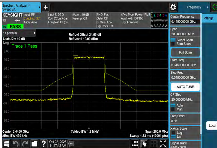
NTNV-11AX40MIMO-Ant4-6445-PASS
