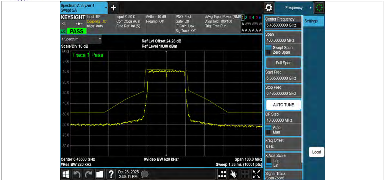
NTNV-11BE20MIMO-Ant3-6435-PASS
