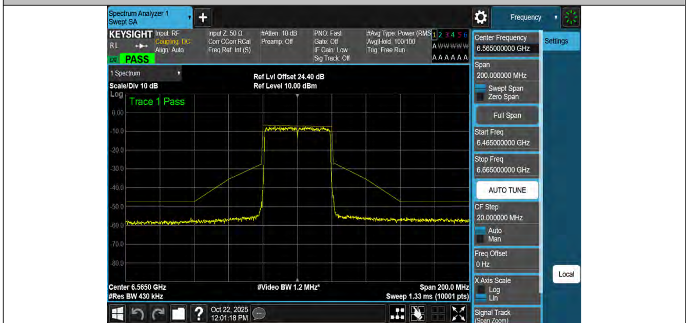
NTNV-11AX40MIMO-Ant2-6565-PASS
