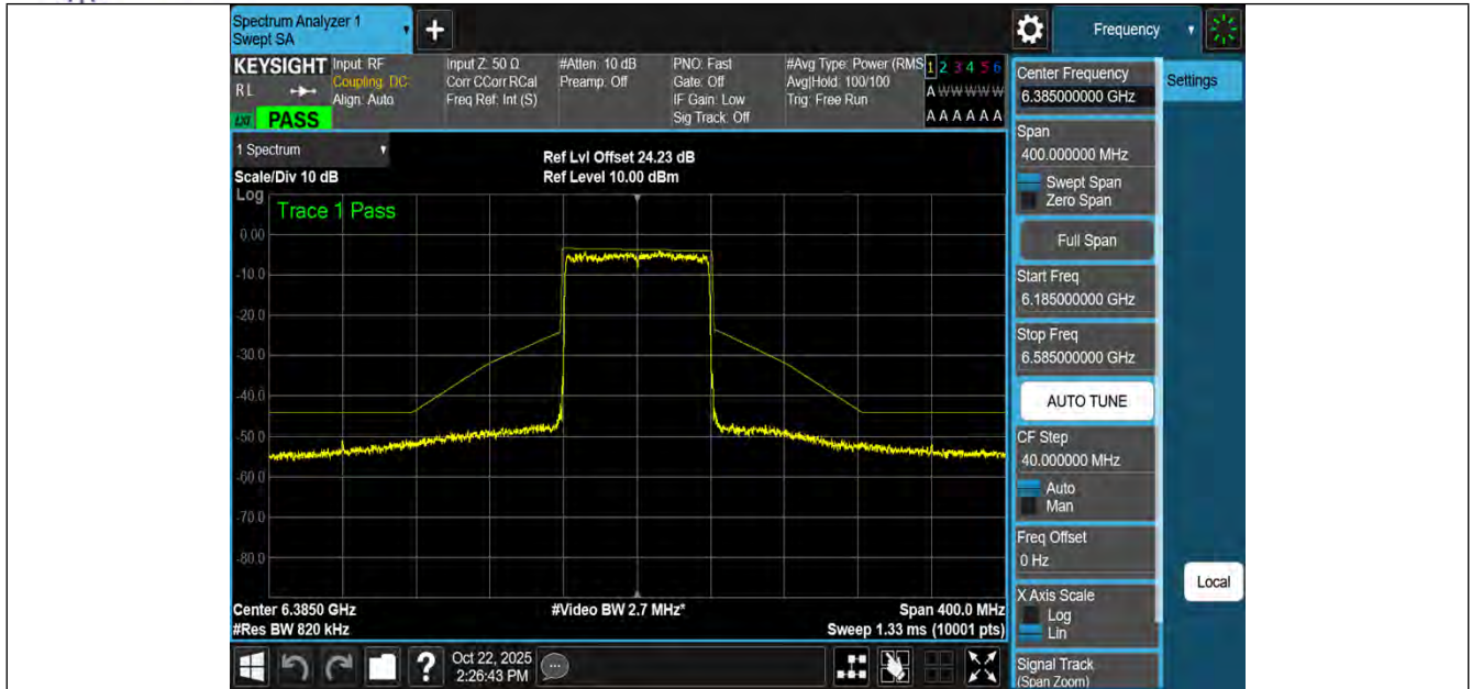
NTNV-11AX80MIMO-Ant1-6385-PASS
