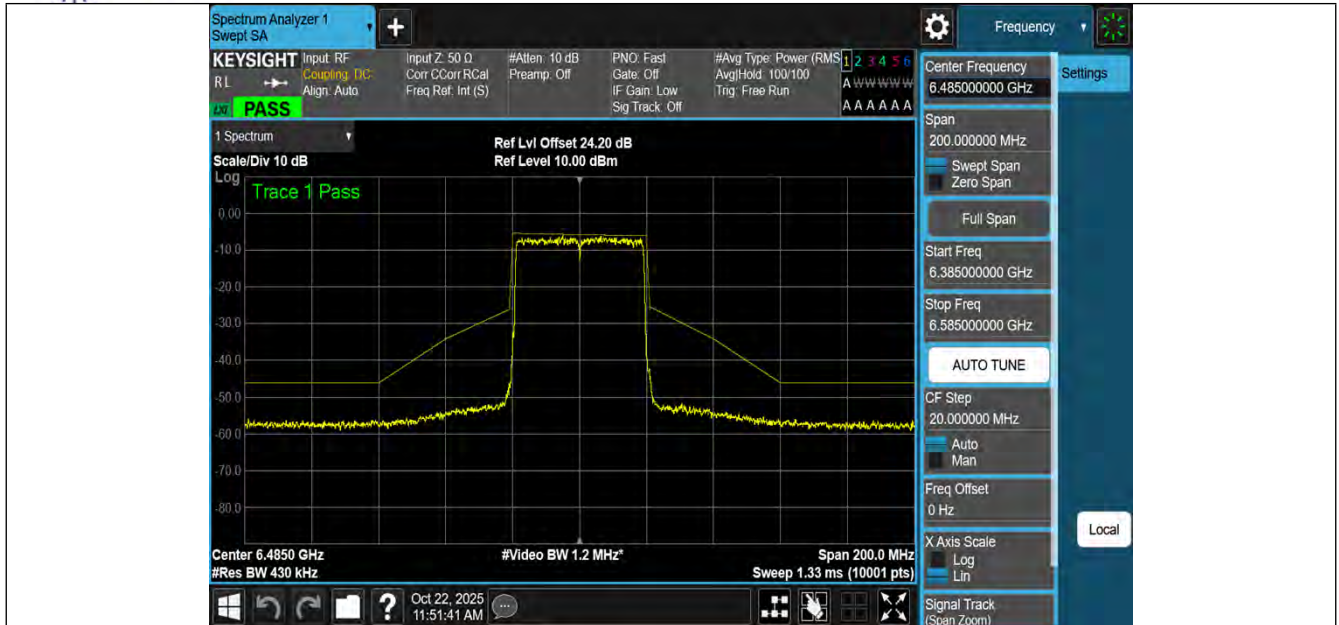
NTNV-11AX40MIMO-Ant3-6485-PASS
