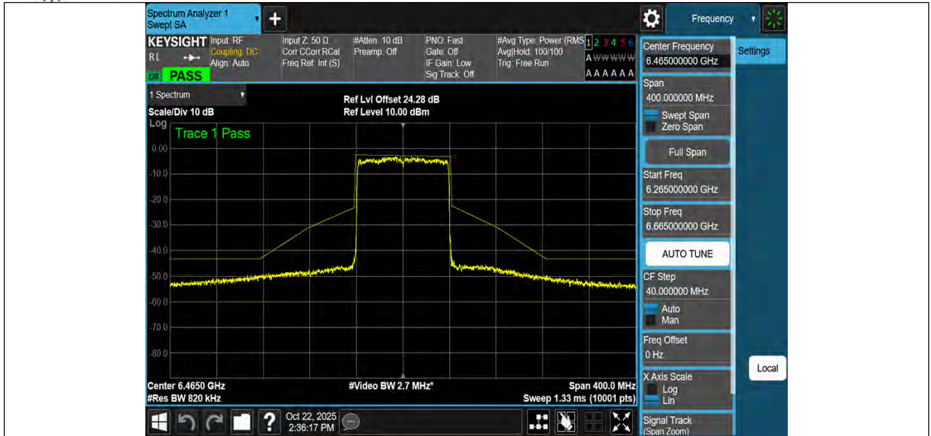
NTNV-11AX80MIMO-Ant3-6465-PASS
