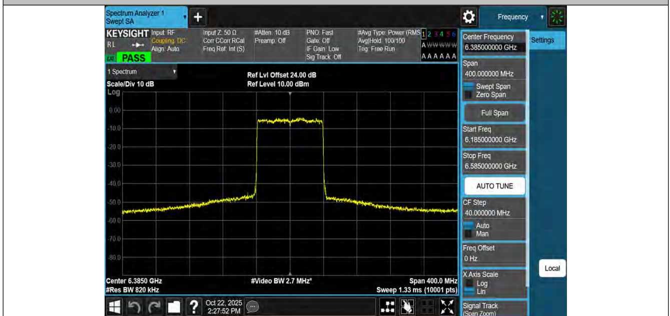
NTNV-11AX80MIMO-Ant2-6385-PASS
