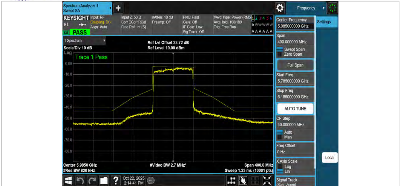
NTNV-11AX80MIMO-Ant3-5985-PASS
