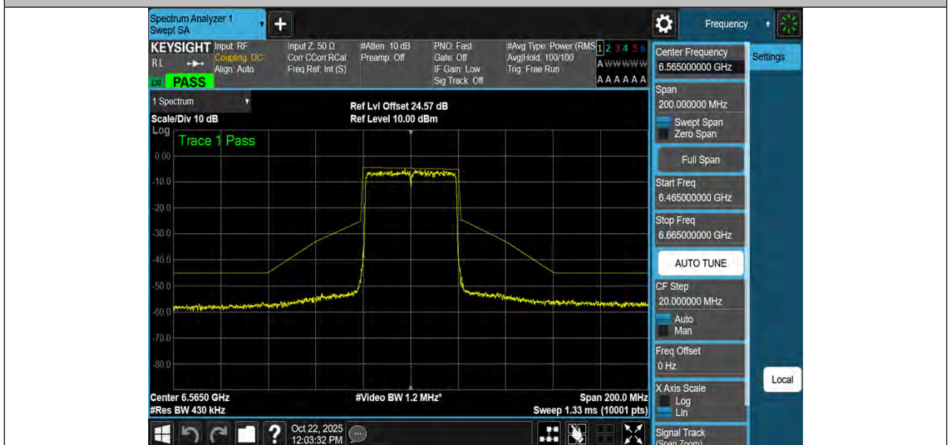
NTNV-11AX40MIMO-Ant4-6565-PASS
