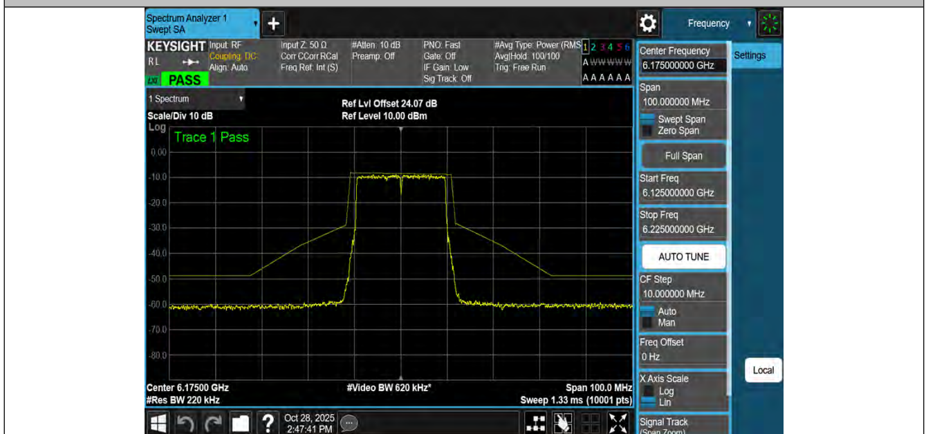
NTNV-11BE20MIMO-Ant4-6175-PASS
