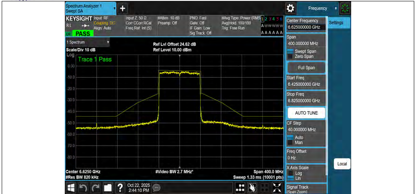
NTNV-11AX80MIMO-Ant1-6625-PASS
