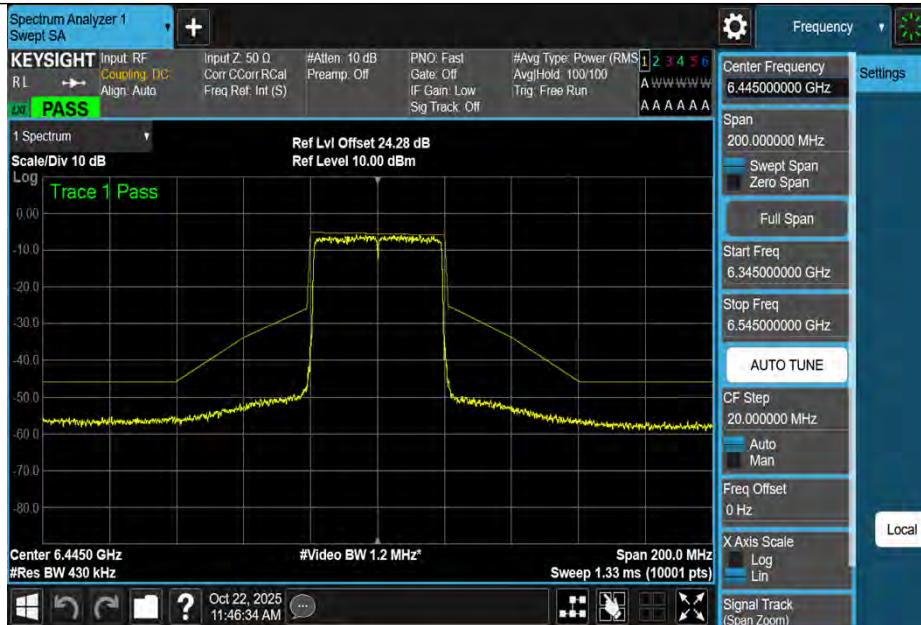
NTNV-11AX40MIMO-Ant3-6445-PASS
