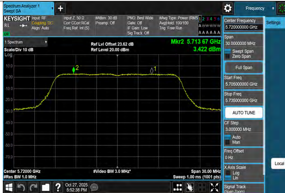
11N20MIMO-Ant1-5720_UNII-2C-PASS
