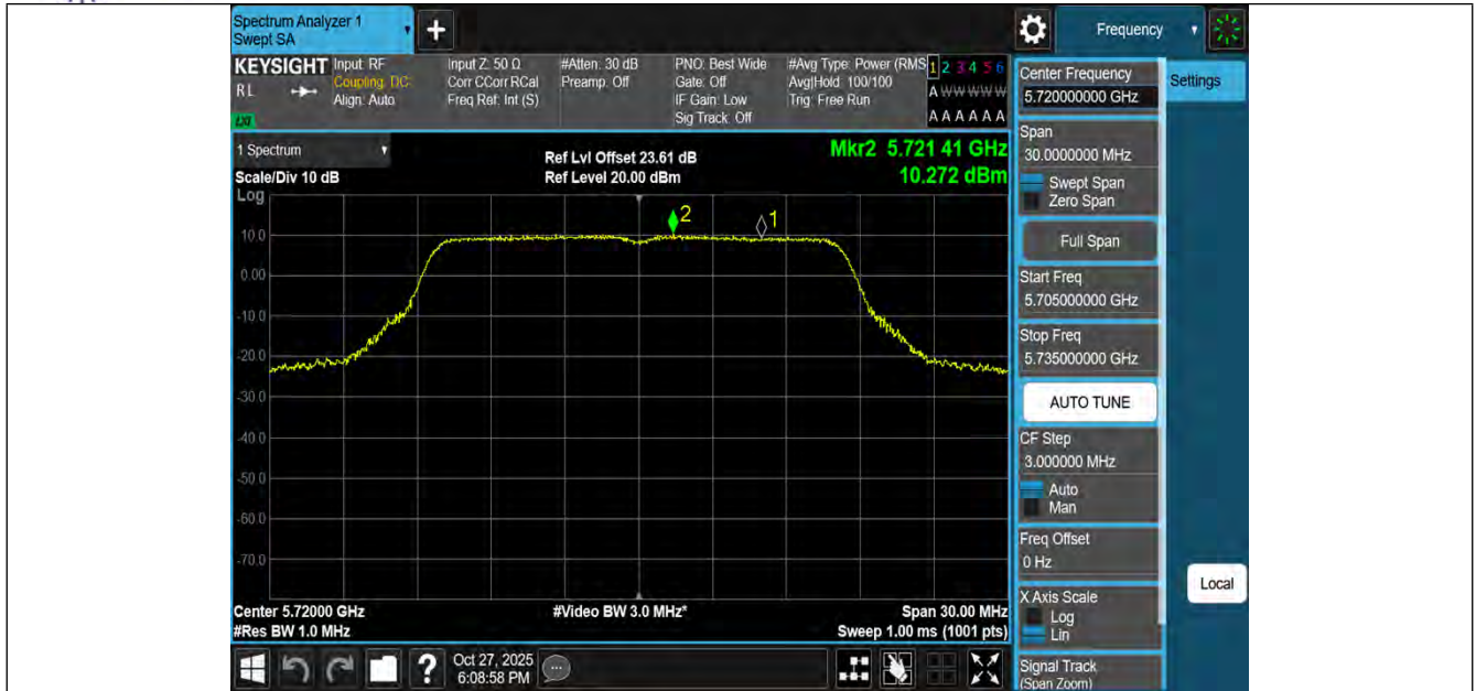
11A-Ant1-5720_UNII-2C-PASS
