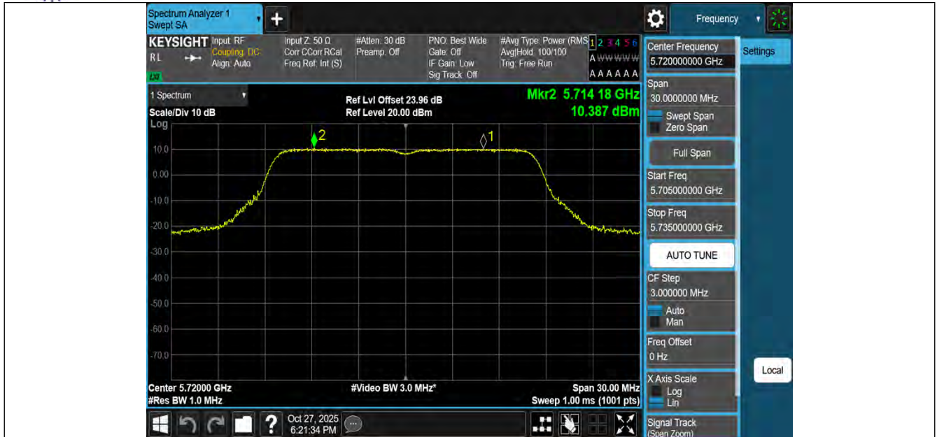
11A-Ant3-5720_UNII-2C-PASS
