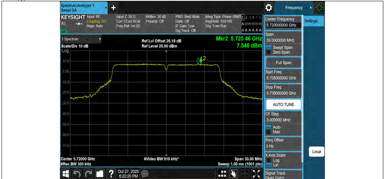
11A-Ant3-5720_UNII-3-PASS
