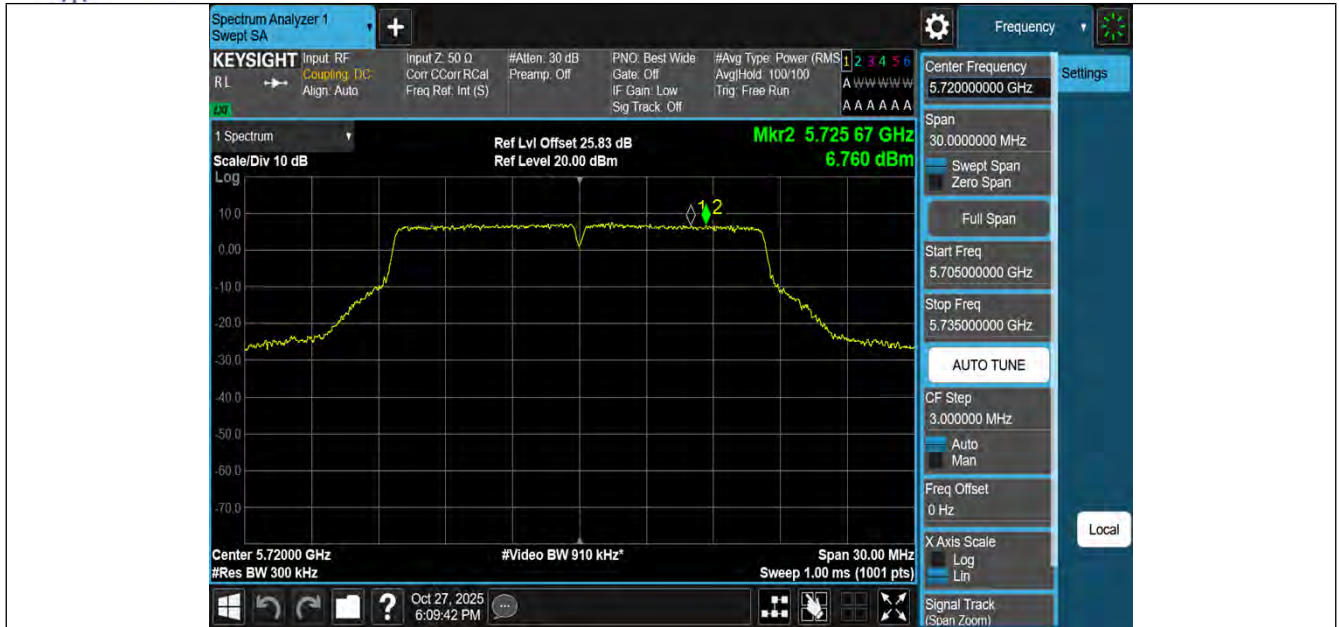
11A-Ant1-5720_UNII-3-PASS
