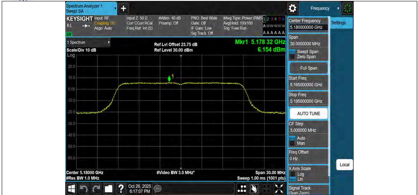
11N20MIMO-Ant3-5180-PASS
