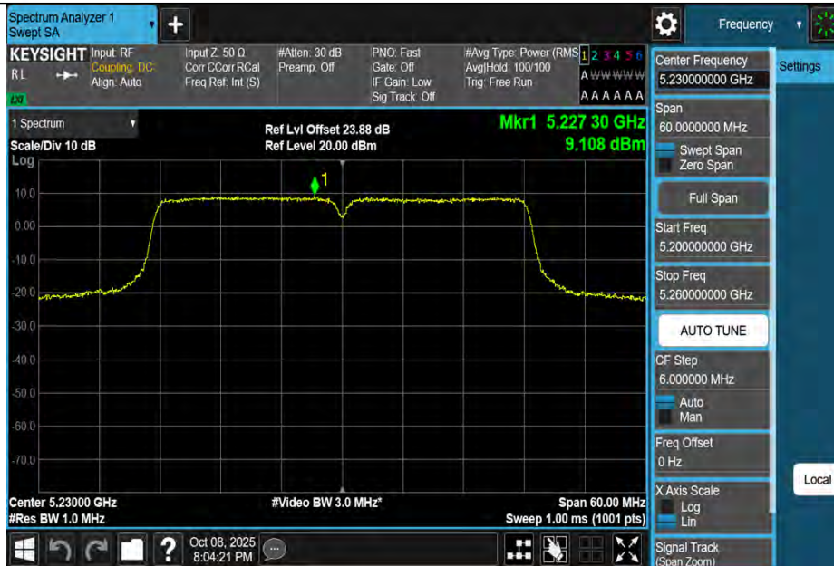
11N40MIMO-Ant1-5230-PASS
