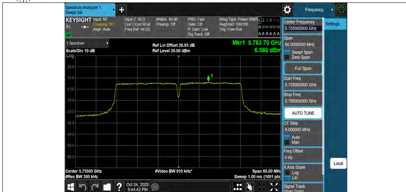
11N40MIMO-Ant3-5755-PASS
