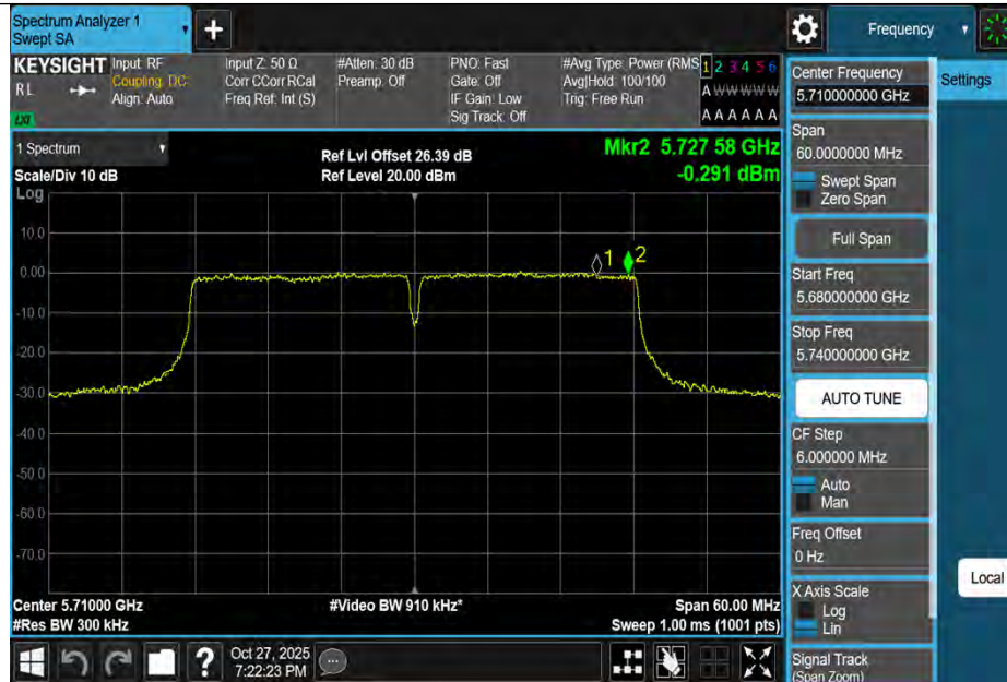
11N40MIMO-Ant3-5710_UNII-3-PASS
