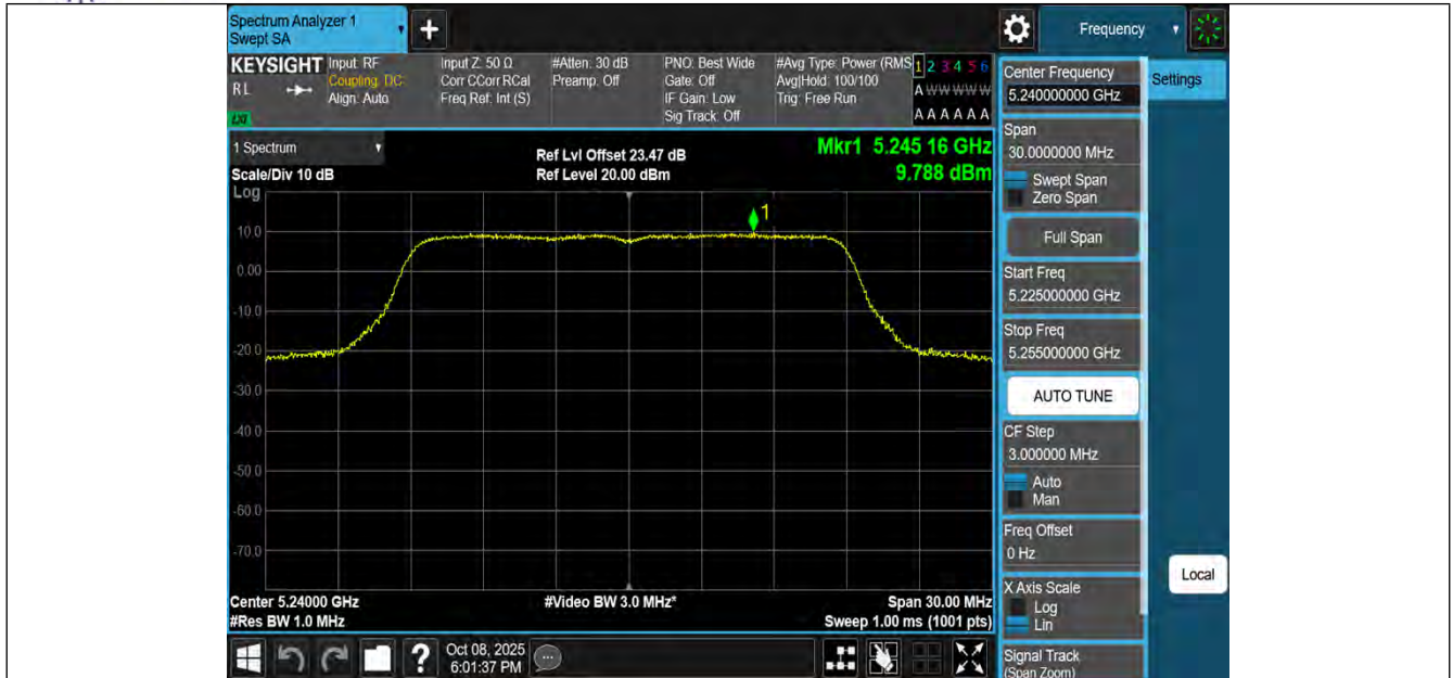
11N20MIMO-Ant3-5240-PASS
