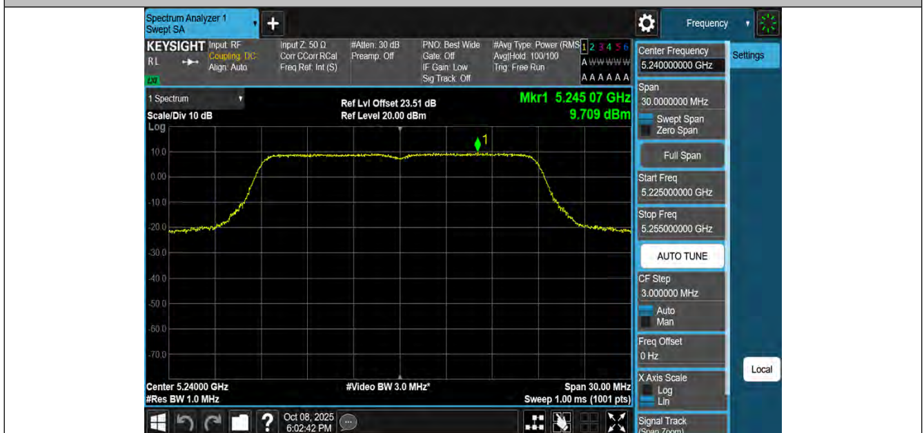
11N20MIMO-Ant4-5240-PASS
