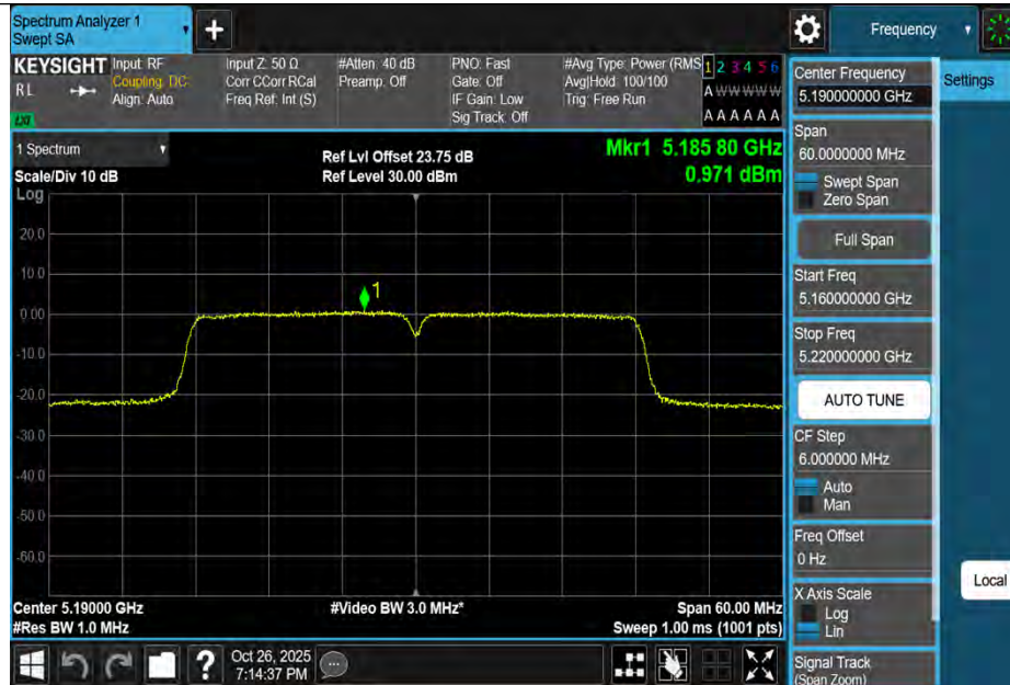
11N40MIMO-Ant1-5190-PASS
