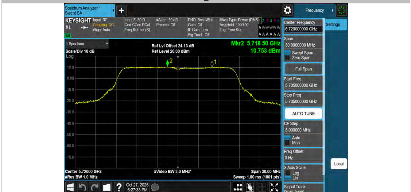
11A-Ant4-5720_UNII-2C-PASS
