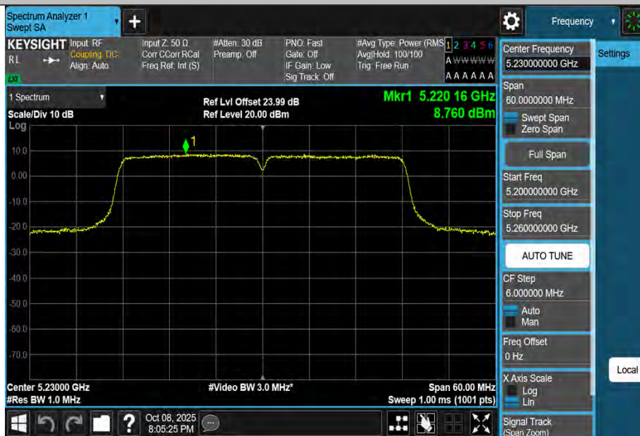
11N40MIMO-Ant2-5230-PASS
