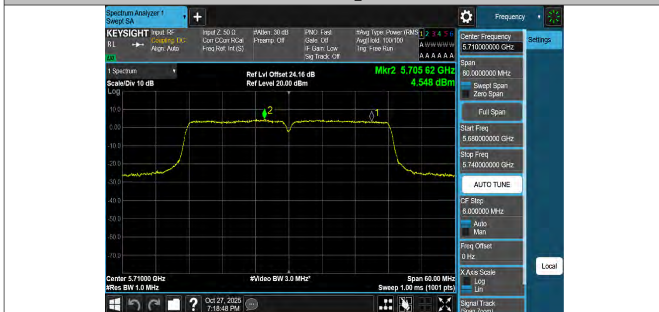
11N40MIMO-Ant2-5710_UNII-2C-PASS
