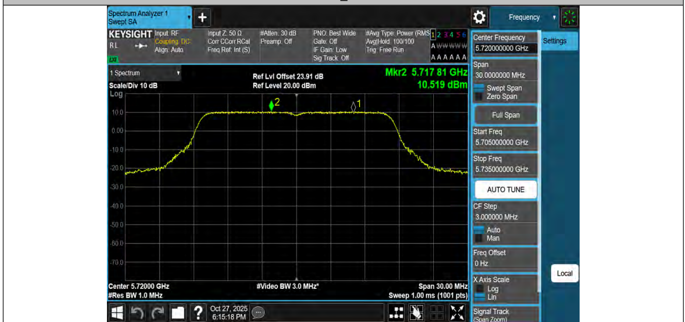
11A-Ant2-5720_UNII-2C-PASS
