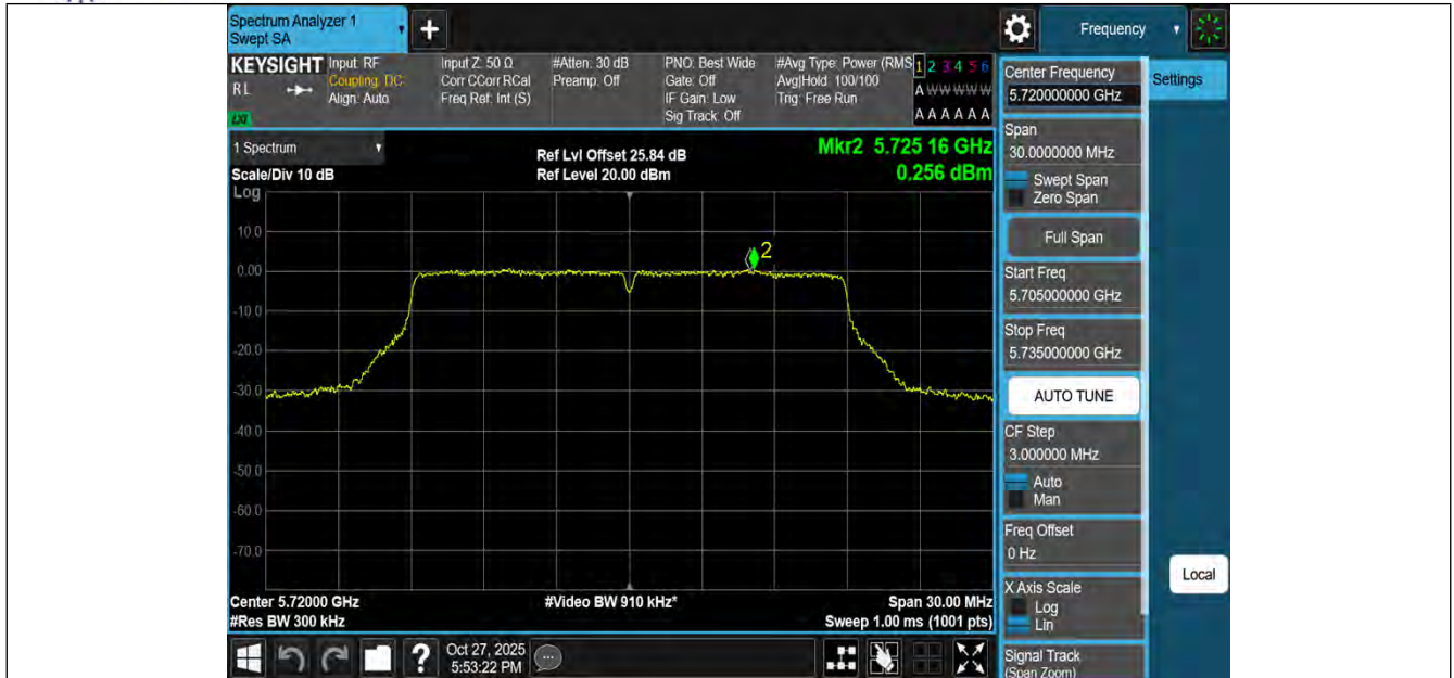
11N20MIMO-Ant1-5720_UNII-3-PASS
