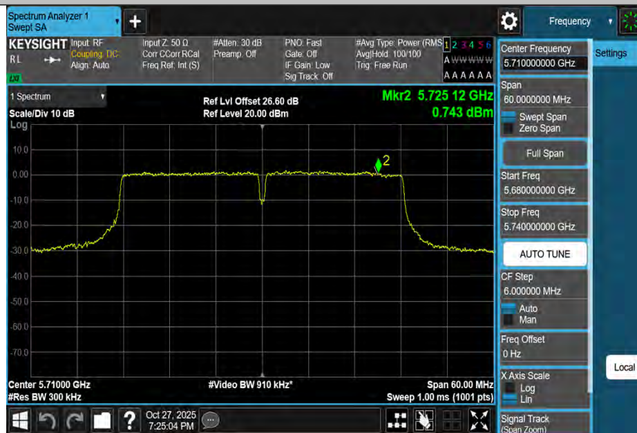
11N40MIMO-Ant4-5710_UNII-3-PASS
