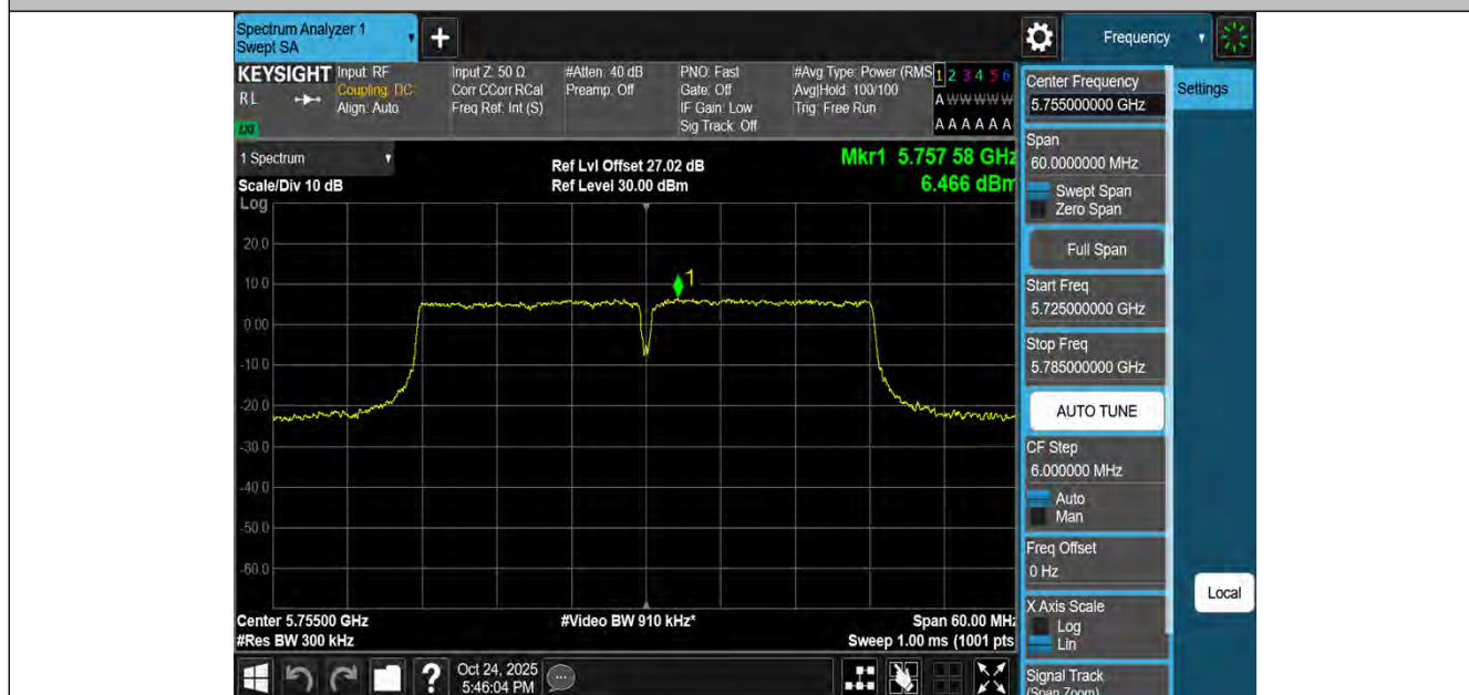
11N40MIMO-Ant4-5755-PASS
