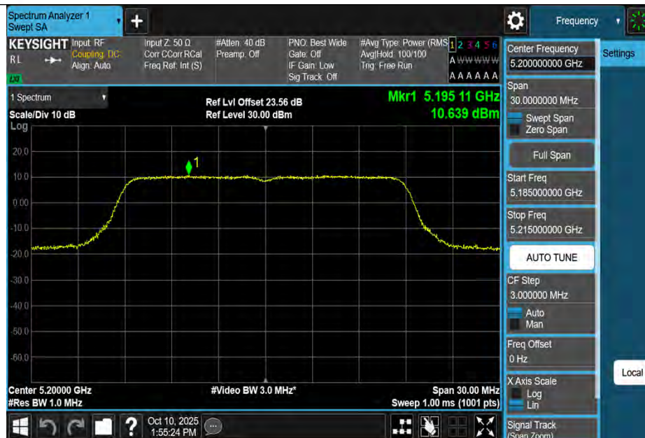
11AC20MIMO-Ant3-5200-PASS
