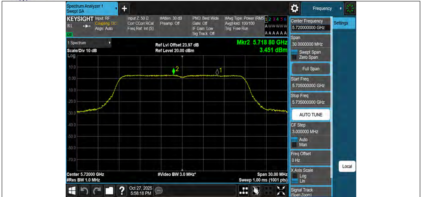
11N20MIMO-Ant3-5720_UNII-2C-PASS
