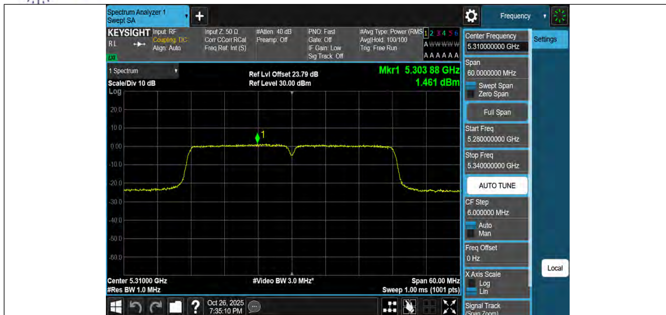
11N40MIMO-Ant1-5310-PASS
