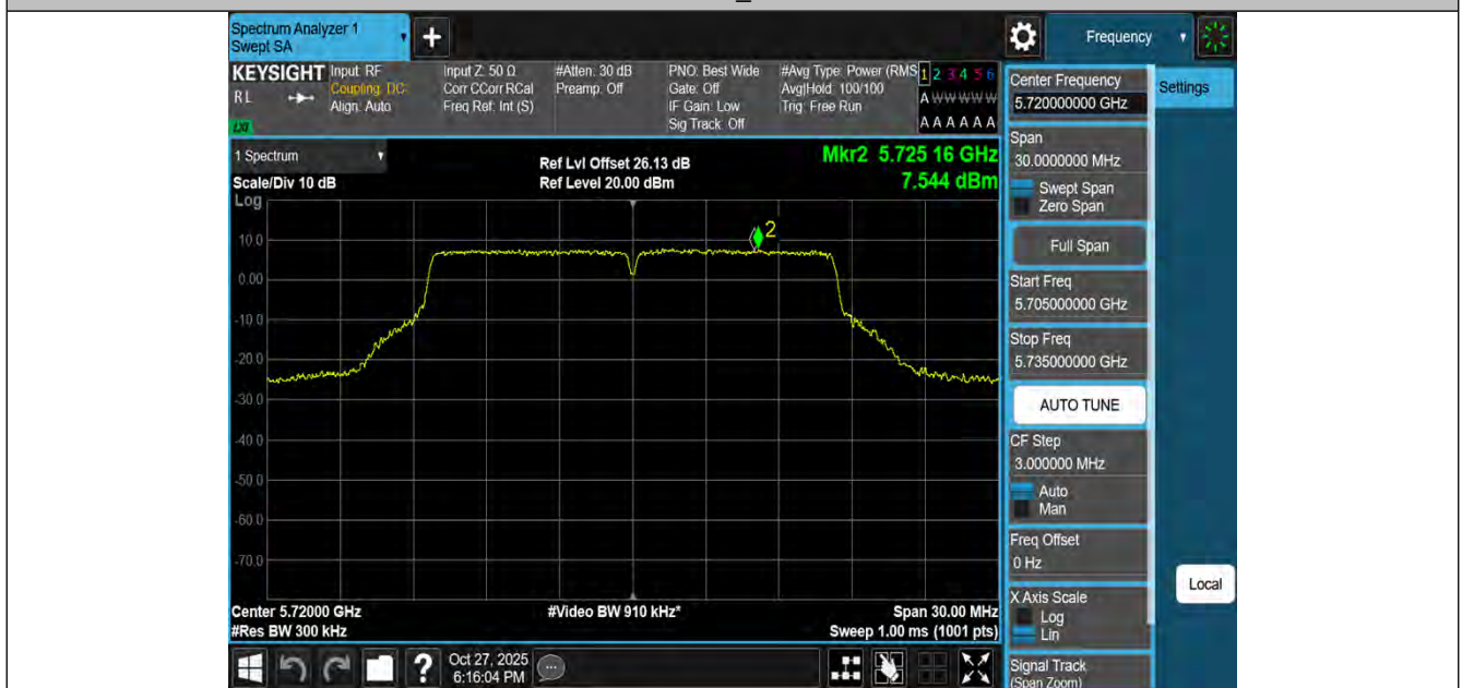
11A-Ant2-5720_UNII-3-PASS
