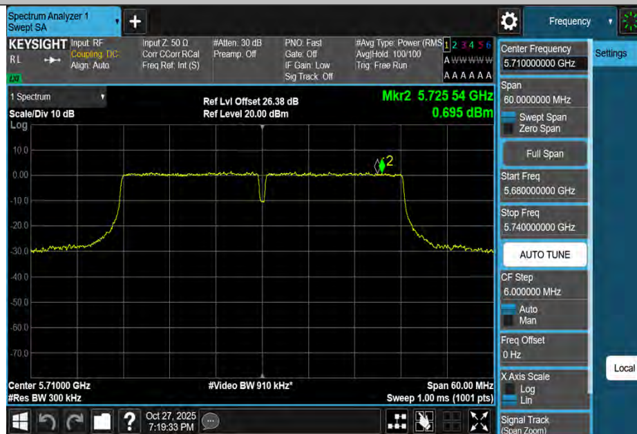
11N40MIMO-Ant2-5710_UNII-3-PASS
