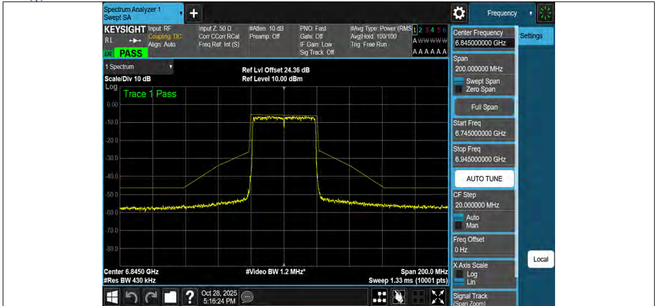
NTNV-11BE40MIMO-Ant1-6845-PASS
