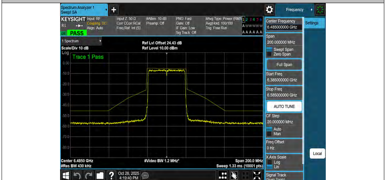
NTNV-11BE40MIMO-Ant4-6485-PASS
