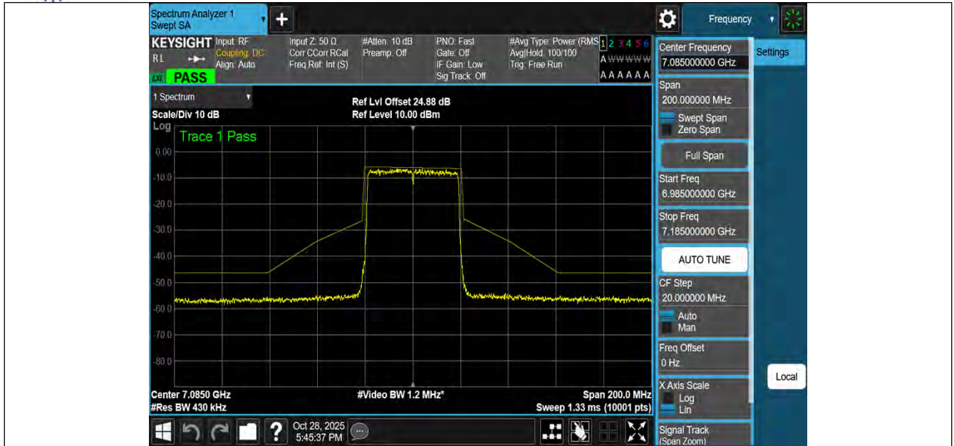
NTNV-11BE40MIMO-Ant3-7085-PASS
