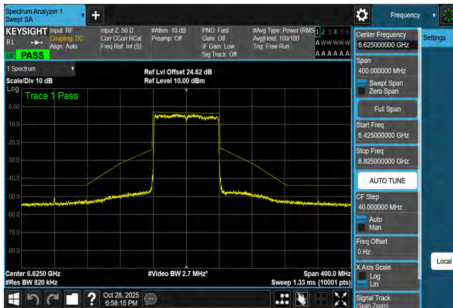
NTNV-11BE80MIMO-Ant1-6625-PASS
