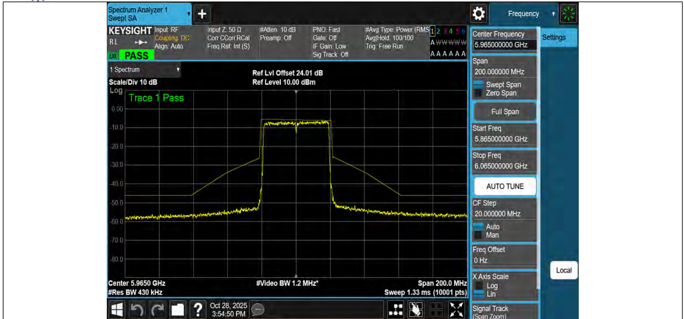
NTNV-11BE40MIMO-Ant1-5965-PASS
