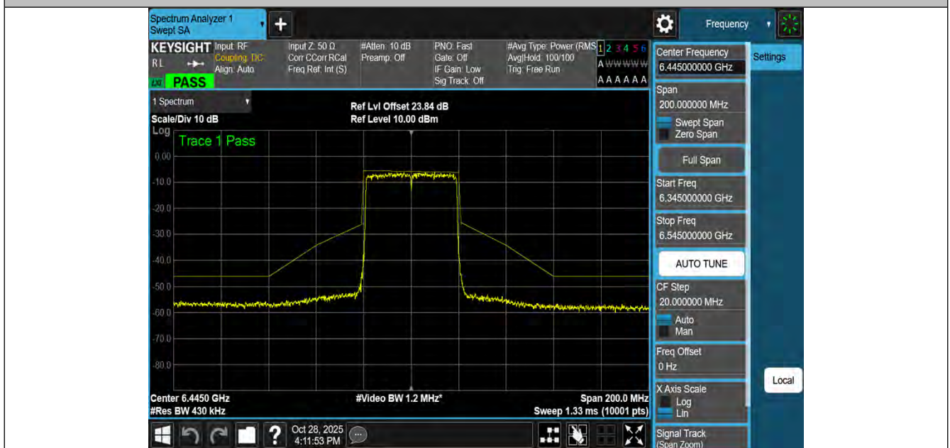
NTNV-11BE40MIMO-Ant2-6445-PASS
