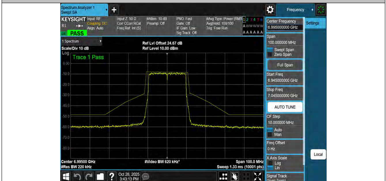
NTNV-11BE20MIMO-Ant4-6995-PASS
