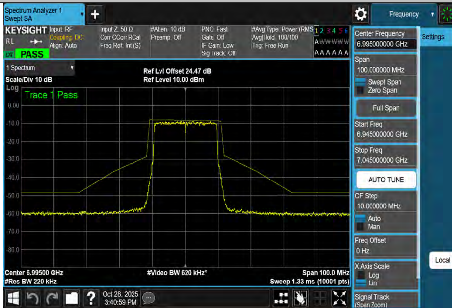
NTNV-11BE20MIMO-Ant2-6995-PASS
