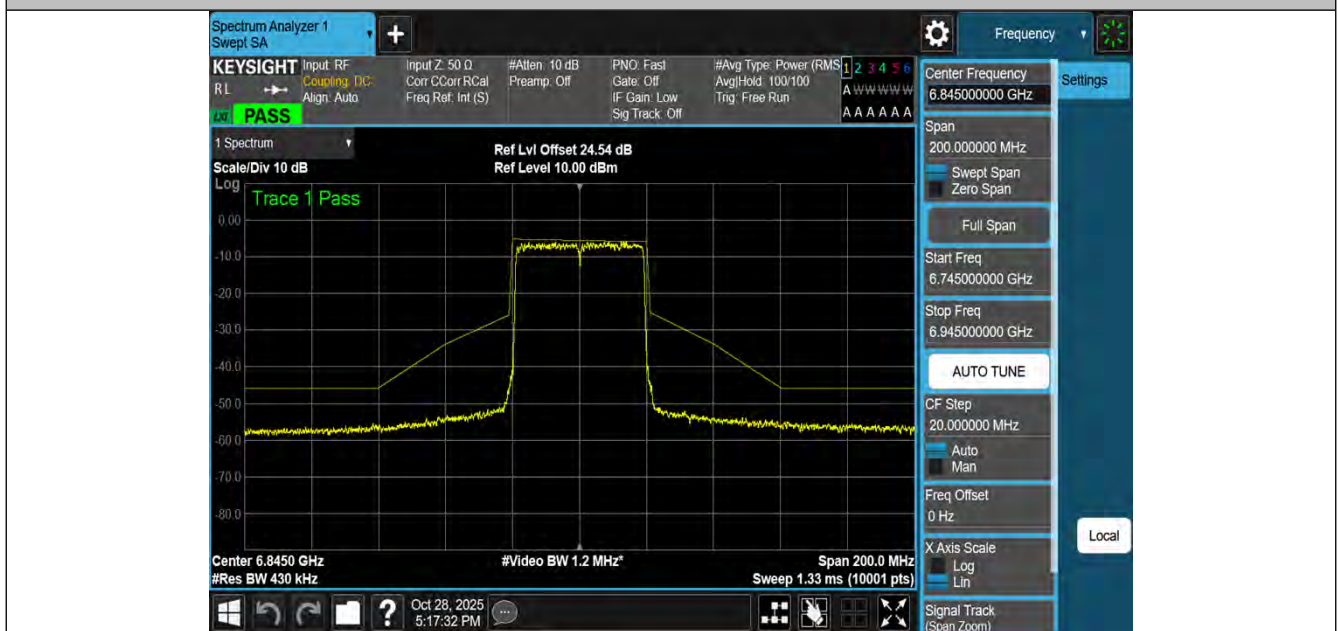
NTNV-11BE40MIMO-Ant2-6845-PASS
