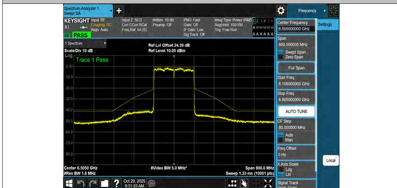
NTVN-11BE160MIMO-Ant2-6505-PASS
