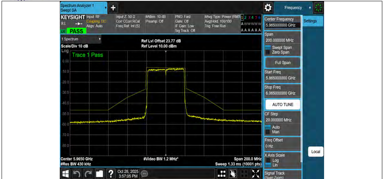
NTNV-11BE40MIMO-Ant3-5965-PASS
