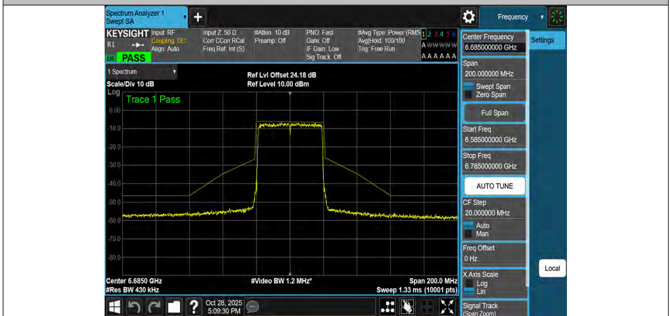
NTNV-11BE40MIMO-Ant2-6685-PASS
