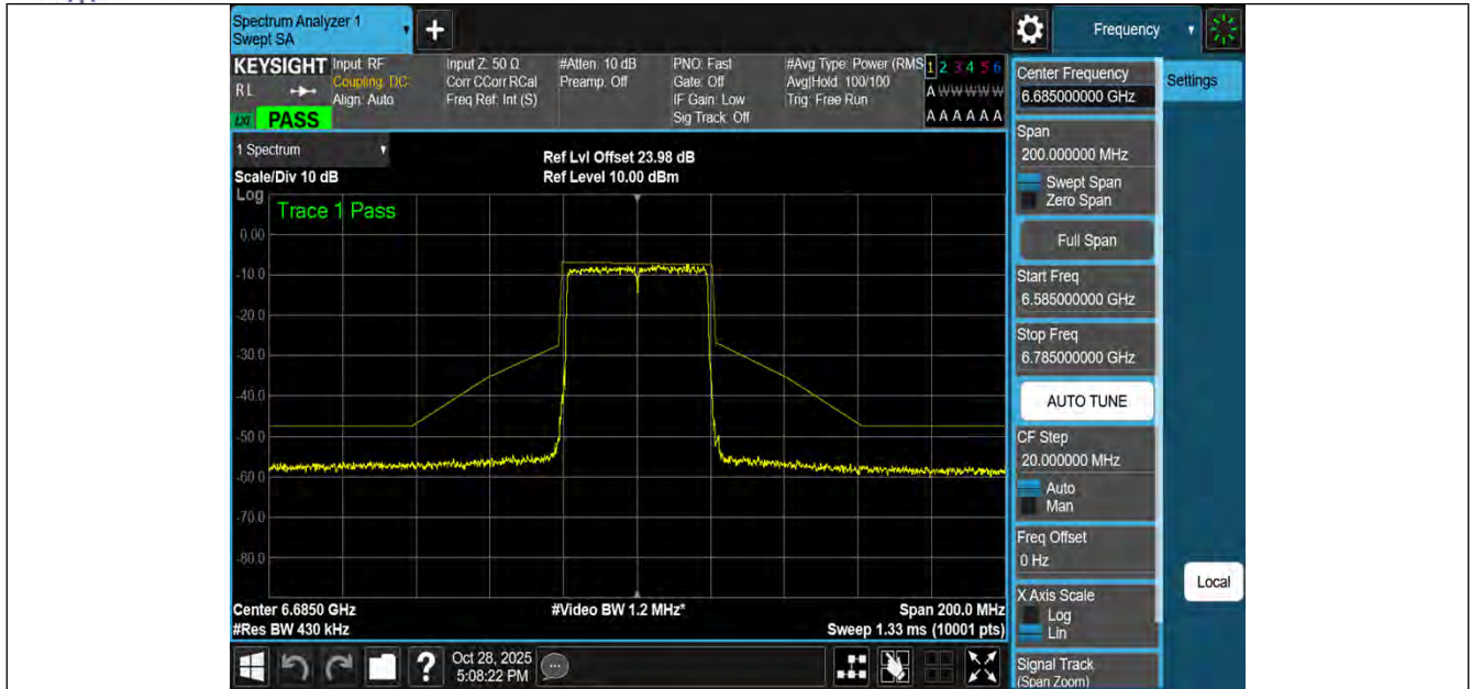
NTNV-11BE40MIMO-Ant1-6685-PASS
