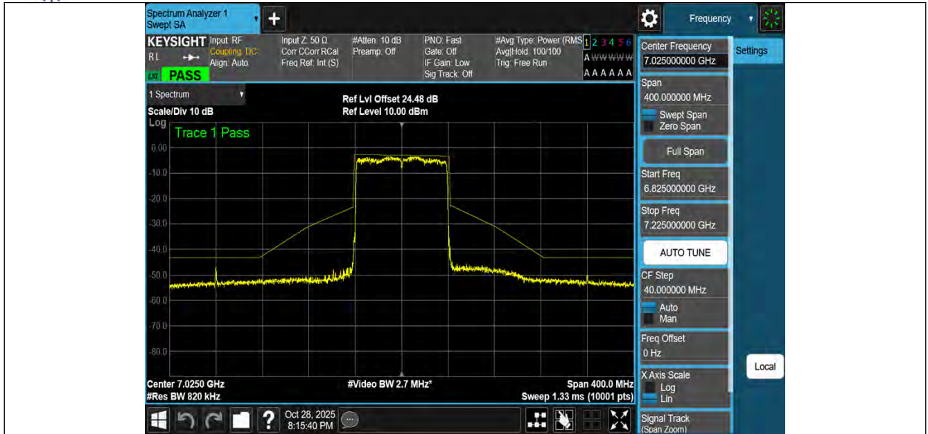
NTNV-11BE80MIMO-Ant1-7025-PASS
