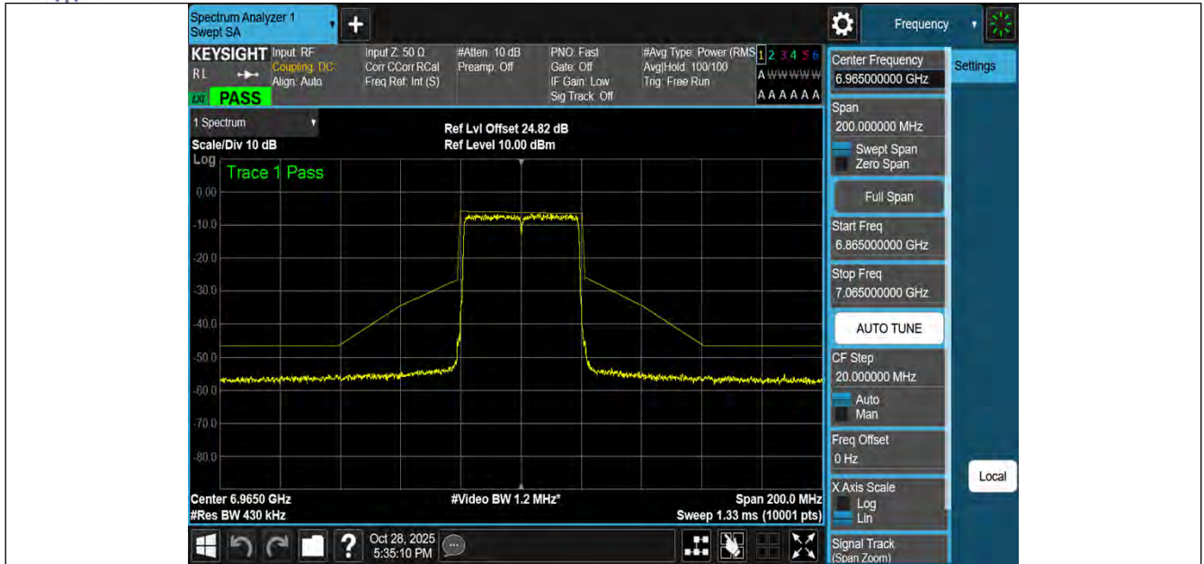
NTNV-11BE40MIMO-Ant1-6965-PASS
