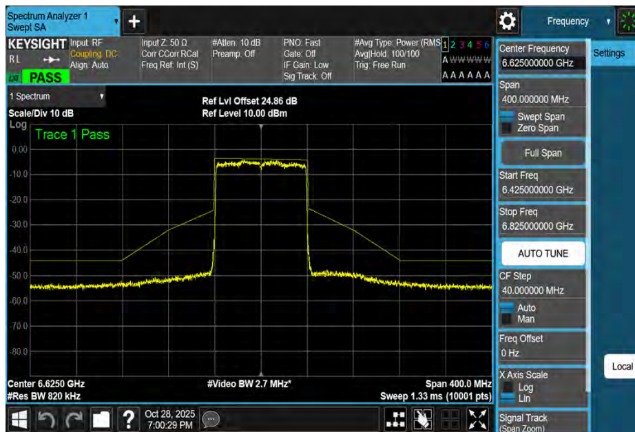
NTNV-11BE80MIMO-Ant3-6625-PASS
