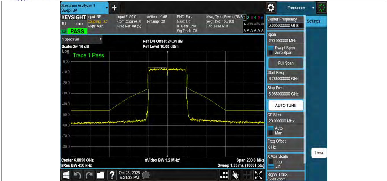
NTNV-11BE40MIMO-Ant1-6885-PASS
