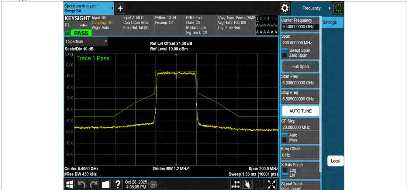
NTNV-11BE40MIMO-Ant3-6405-PASS
