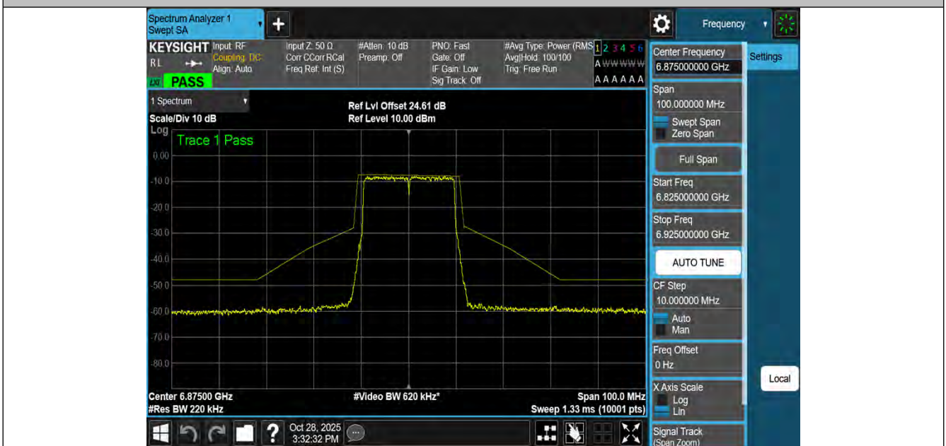
NTNV-11BE20MIMO-Ant4-6875-PASS
