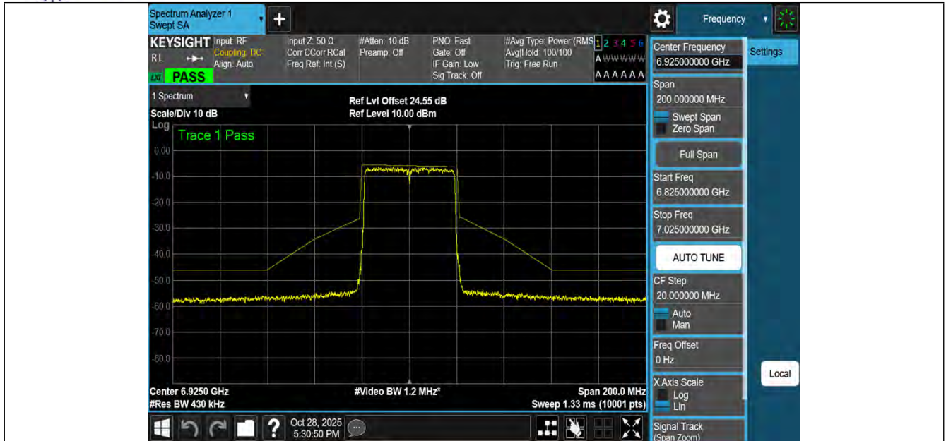
NTNV-11BE40MIMO-Ant3-6925-PASS
