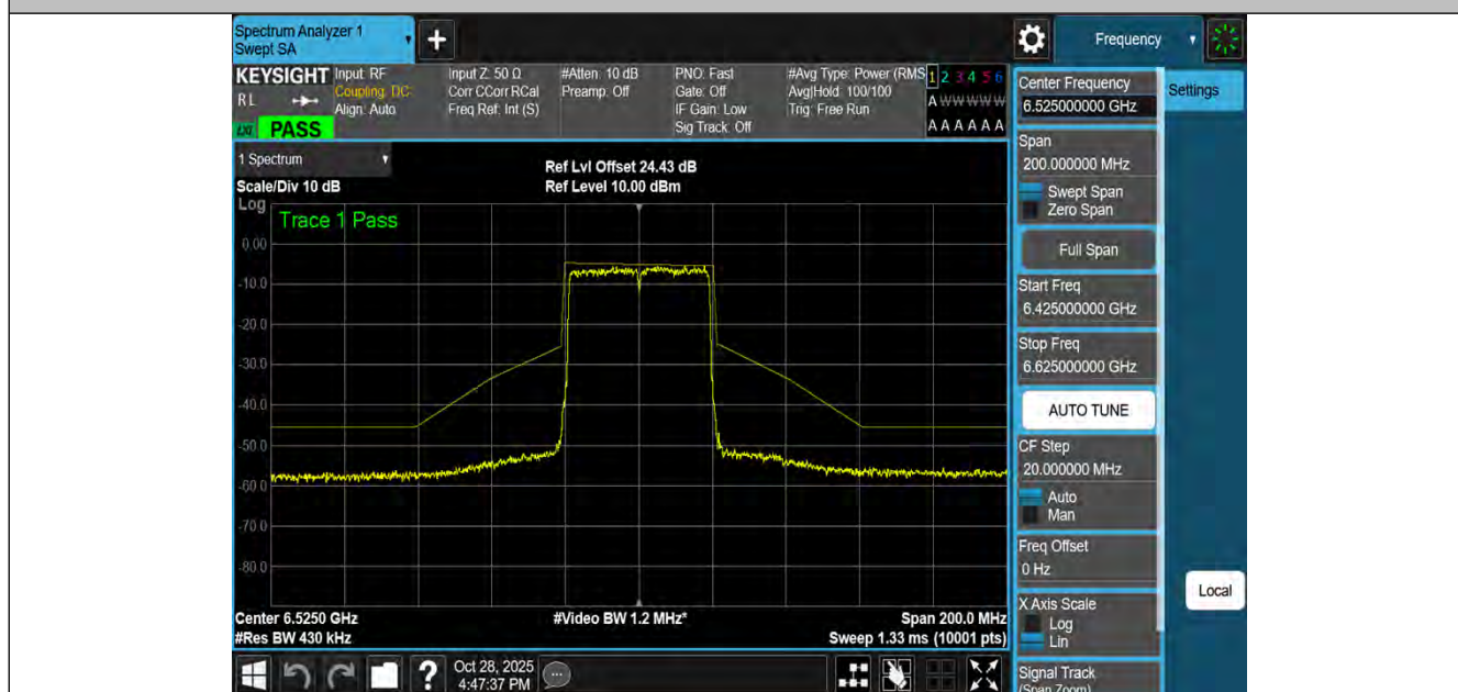
NTNV-11BE40MIMO-Ant4-6525-PASS
