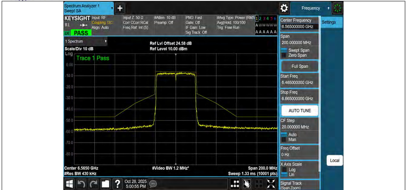
NTNV-11BE40MIMO-Ant3-6565-PASS
