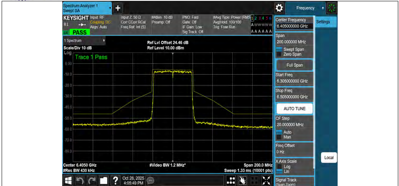
NTNV-11BE40MIMO-Ant1-6405-PASS
