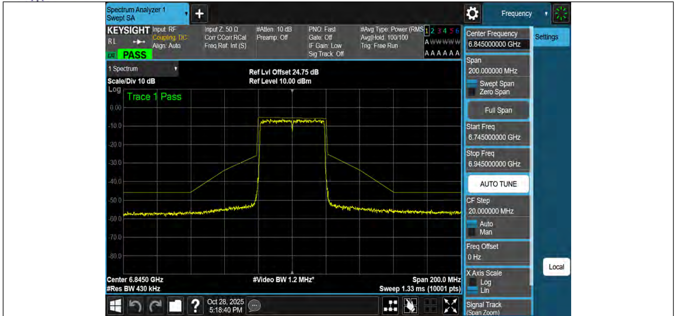
NTNV-11BE40MIMO-Ant3-6845-PASS
