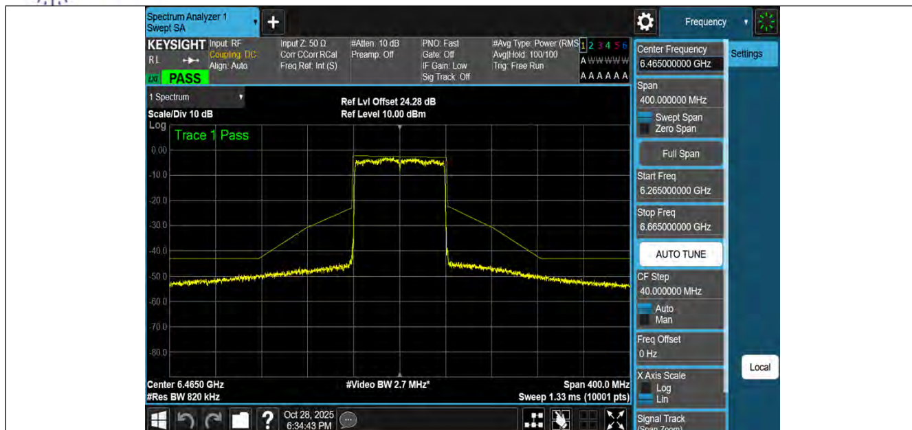
NTNV-11BE80MIMO-Ant3-6465-PASS
