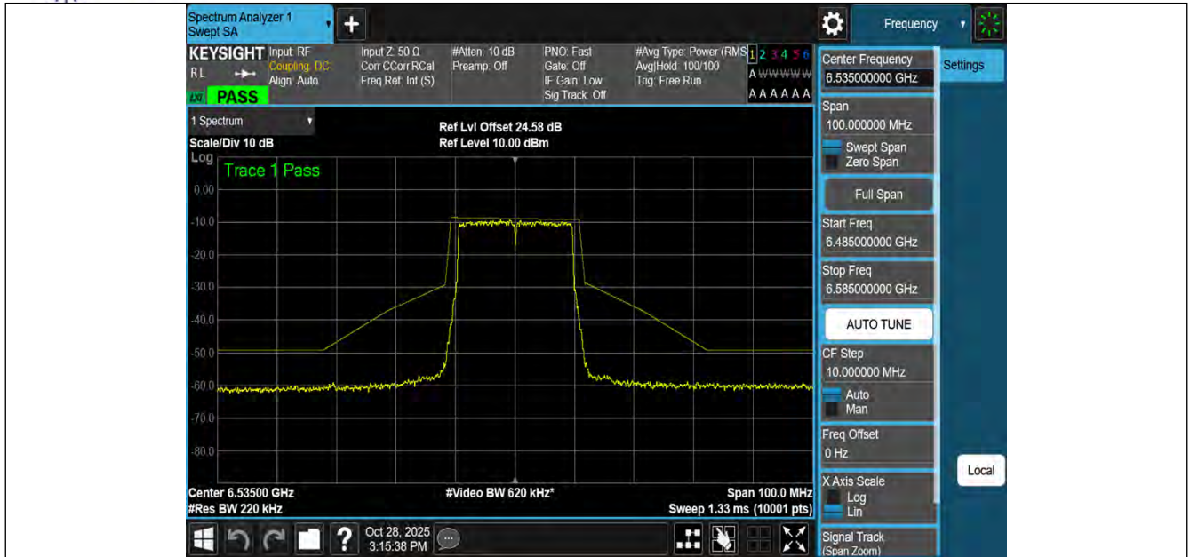
NTNV-11BE20MIMO-Ant3-6535-PASS
