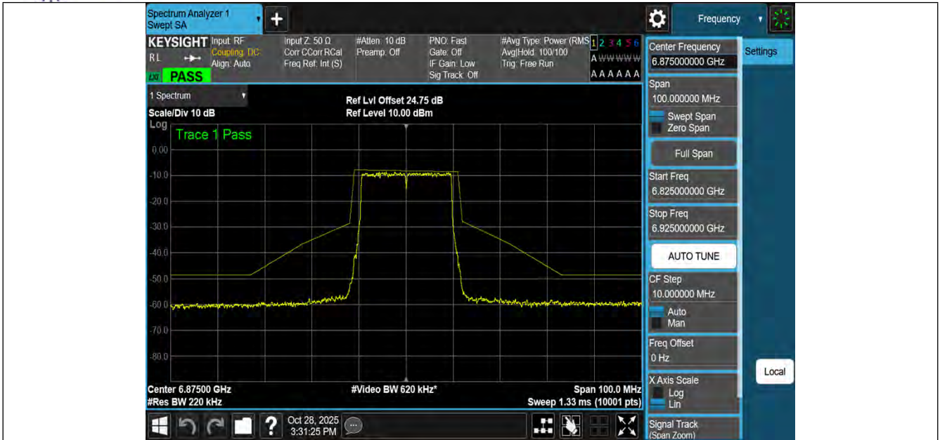
NTNV-11BE20MIMO-Ant3-6875-PASS
