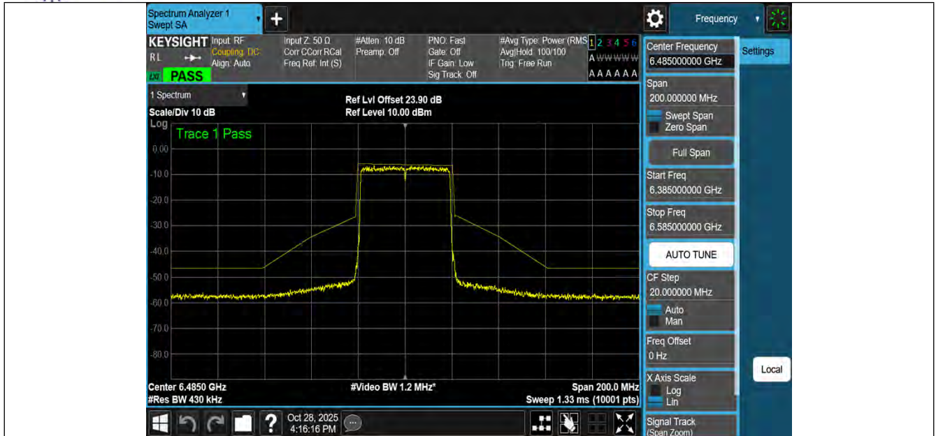
NTNV-11BE40MIMO-Ant1-6485-PASS
