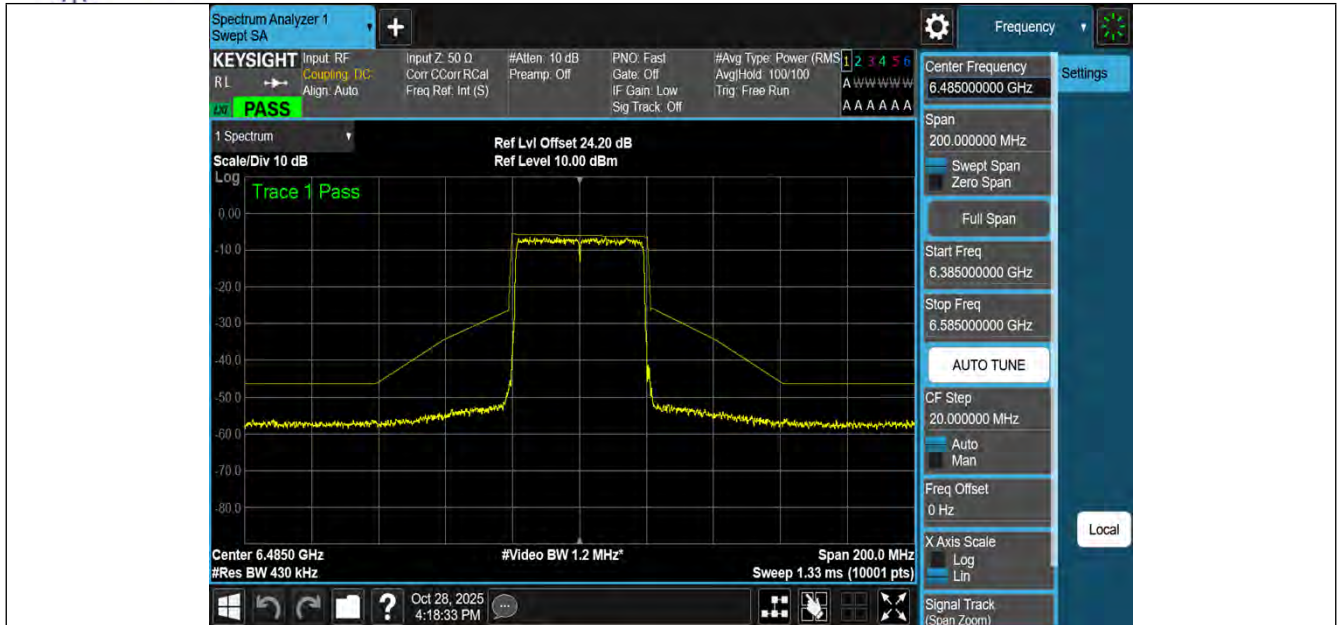
NTNV-11BE40MIMO-Ant3-6485-PASS
