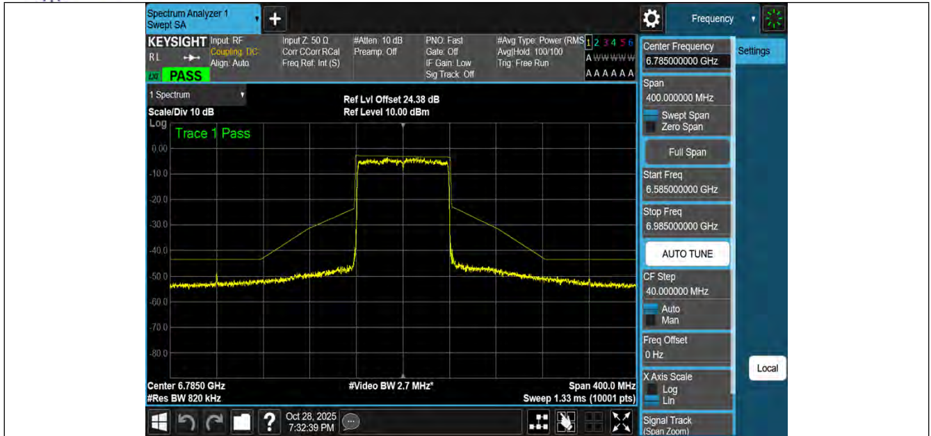
NTNV-11BE80MIMO-Ant1-6785-PASS
