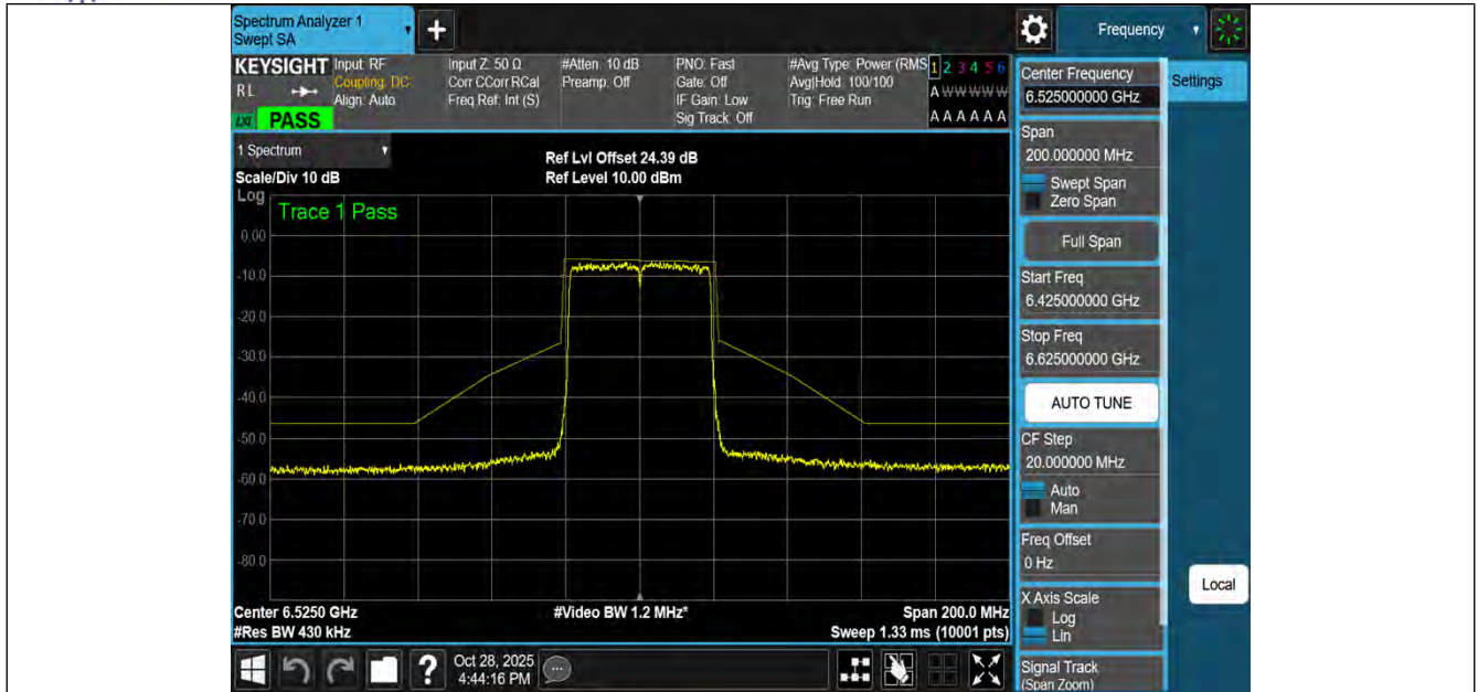
NTNV-11BE40MIMO-Ant1-6525-PASS
