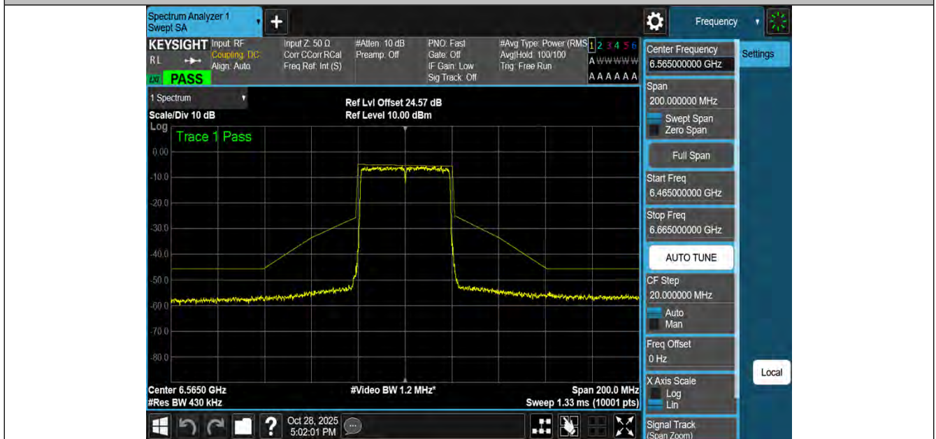
NTNV-11BE40MIMO-Ant4-6565-PASS
