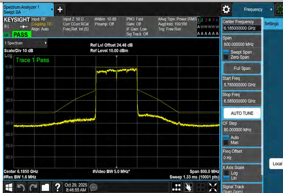
NTNV-11BE160MIMO-Ant2-6185-PASS
