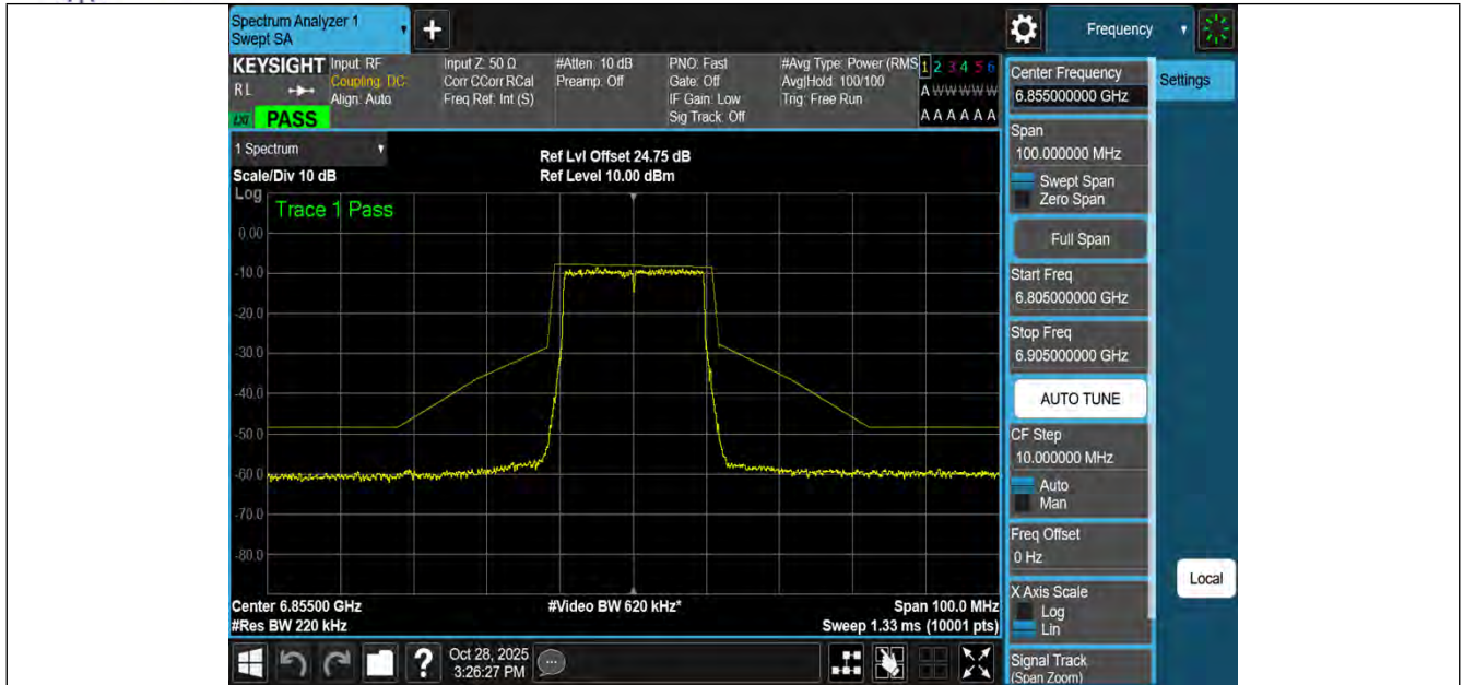
NTNV-11BE20MIMO-Ant3-6855-PASS
