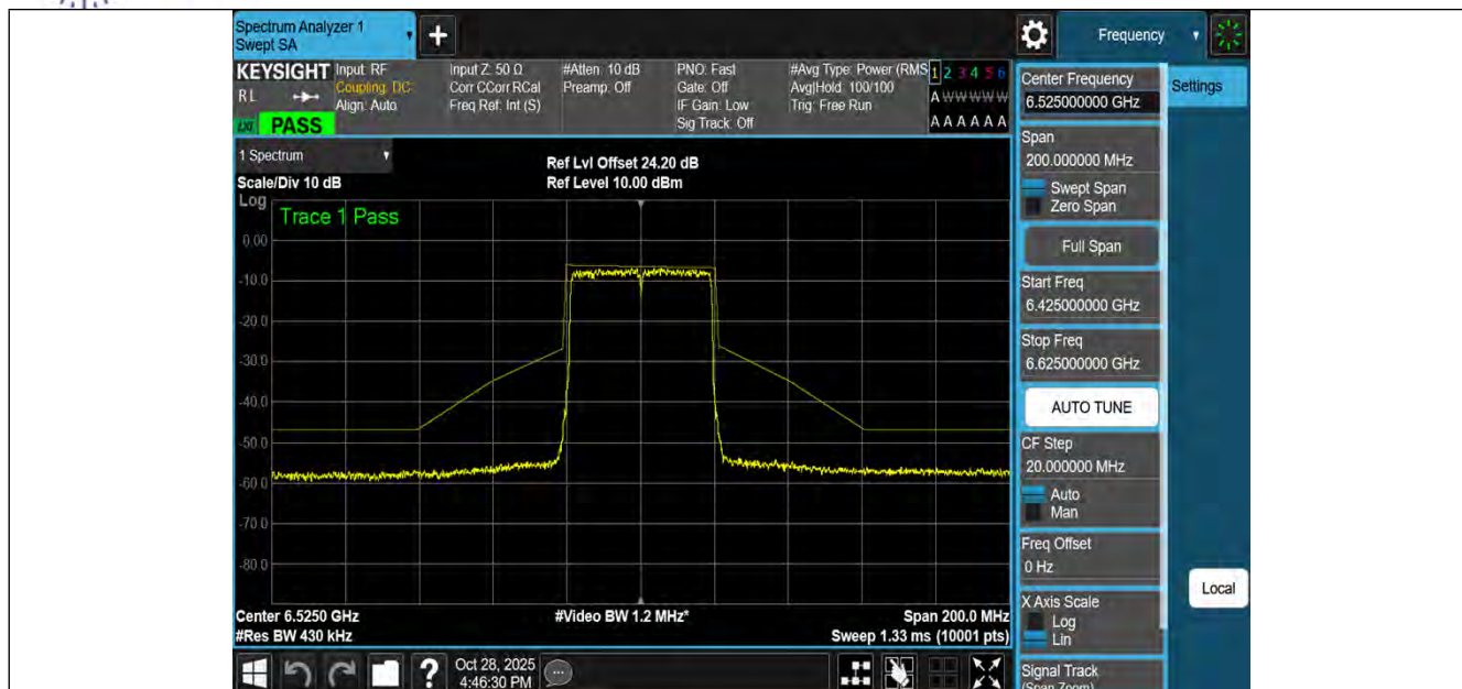
NTNV-11BE40MIMO-Ant3-6525-PASS
