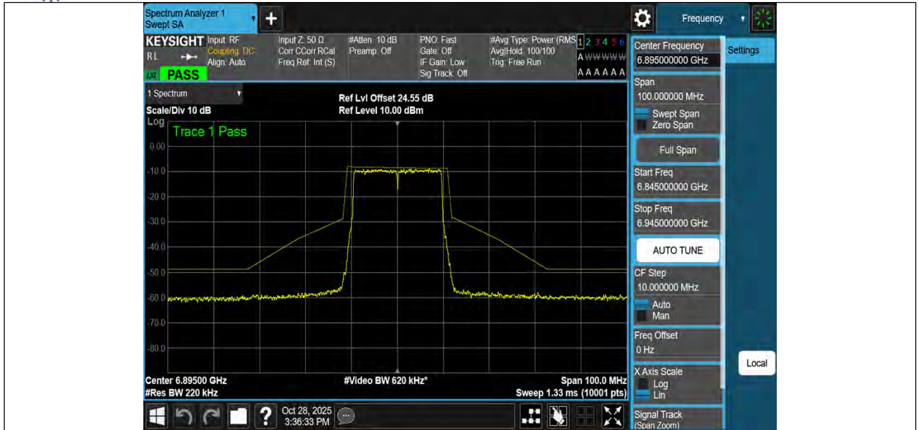
NTNV-11BE20MIMO-Ant3-6895-PASS
