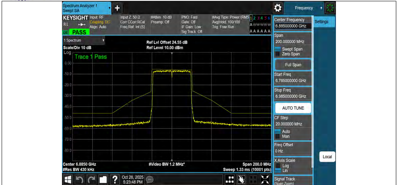
NTNV-11BE40MIMO-Ant3-6885-PASS
