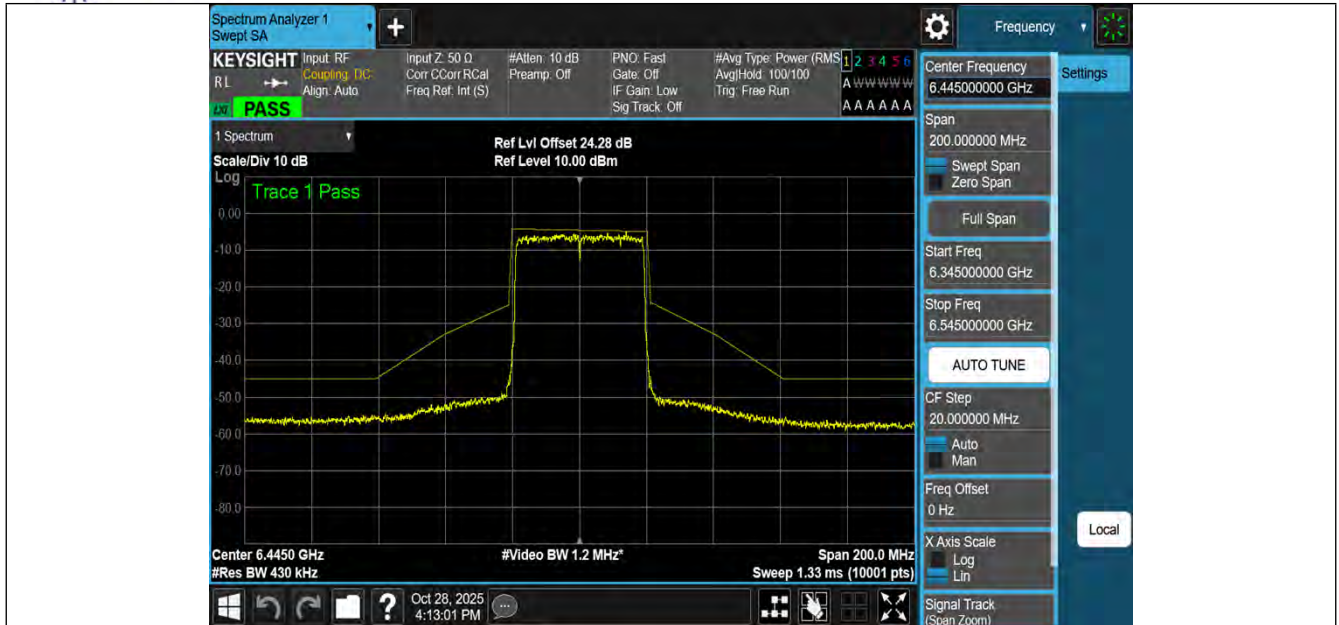
NTNV-11BE40MIMO-Ant3-6445-PASS
