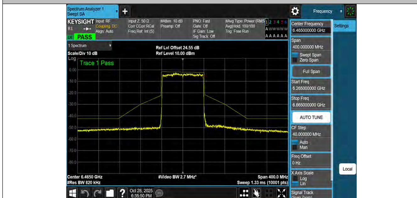
NTNV-11BE80MIMO-Ant4-6465-PASS
