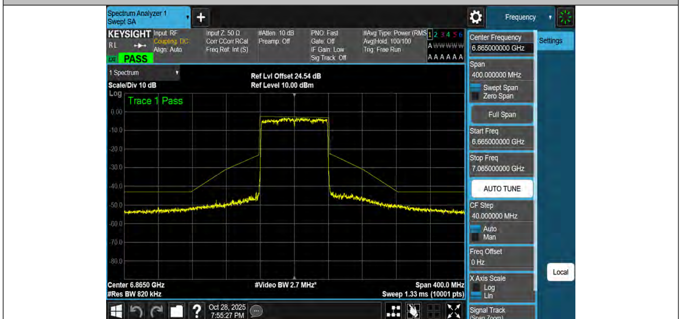
NTNV-11BE80MIMO-Ant2-6865-PASS
