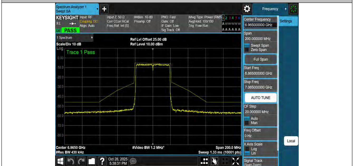
NTNV-11BE40MIMO-Ant4-6965-PASS
