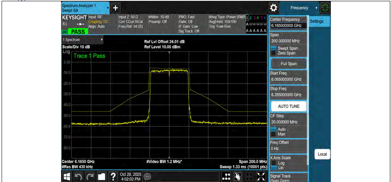
NTNV-11BE40MIMO-Ant3-6165-PASS
