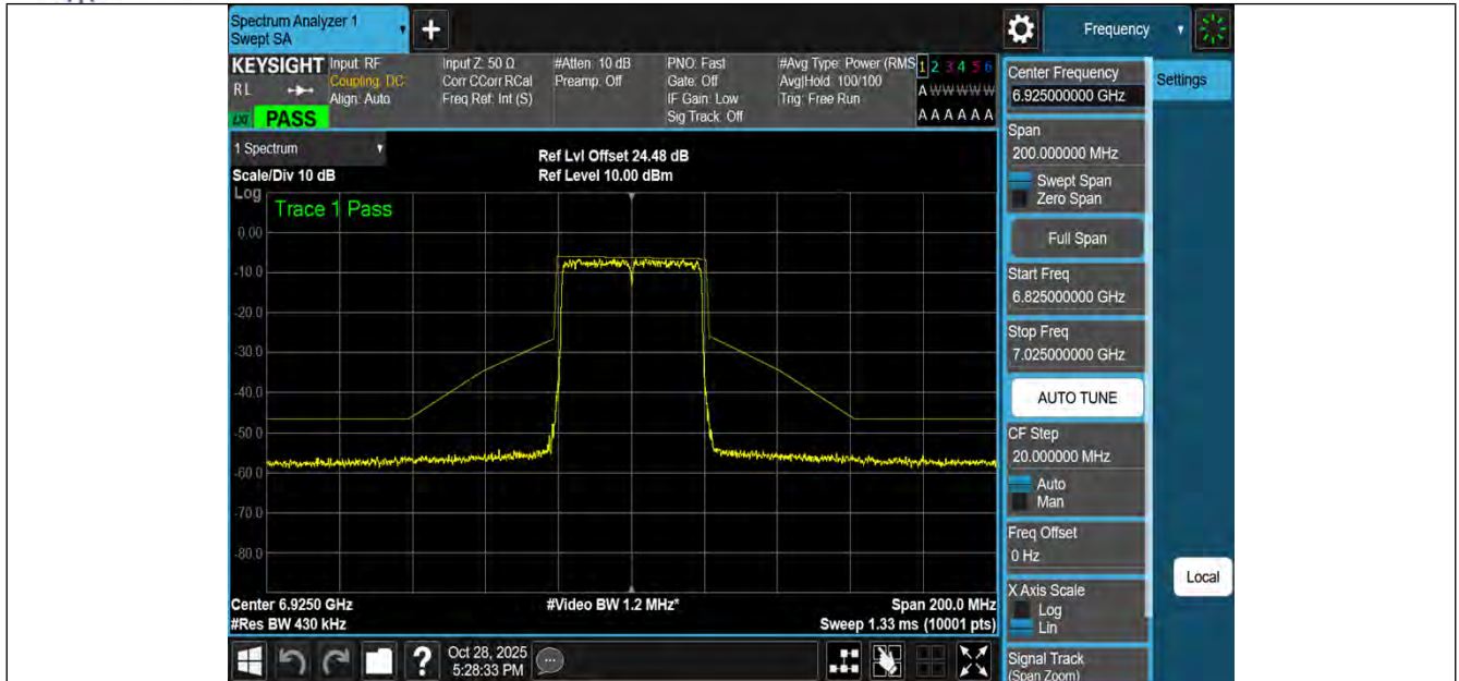
NTNV-11BE40MIMO-Ant1-6925-PASS
