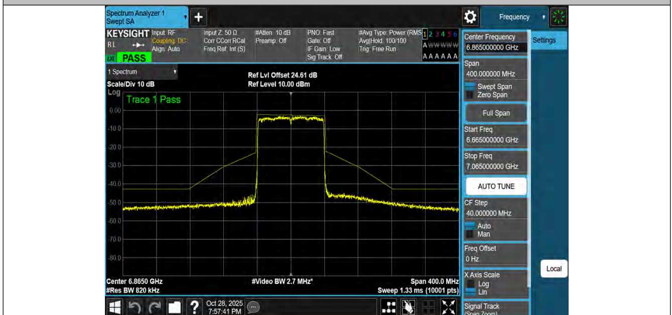
NTNV-11BE80MIMO-Ant4-6865-PASS
