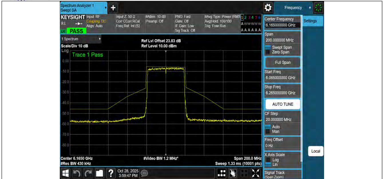
NTNV-11BE40MIMO-Ant1-6165-PASS
