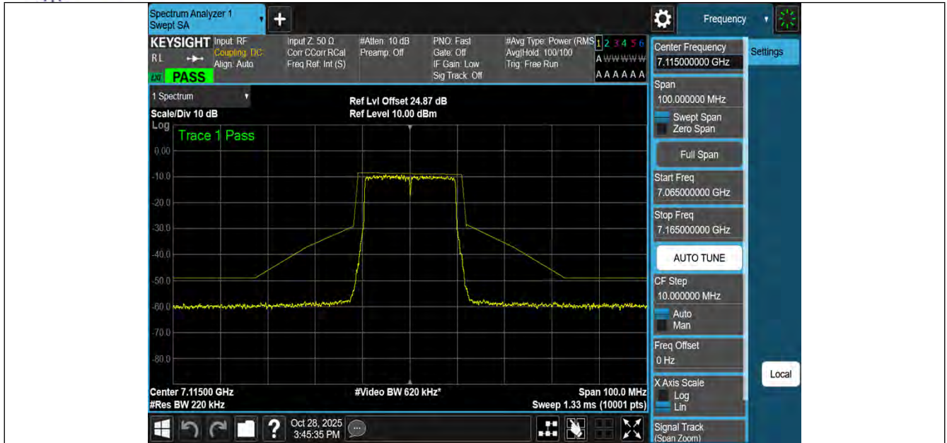
NTNV-11BE20MIMO-Ant1-7115-PASS
