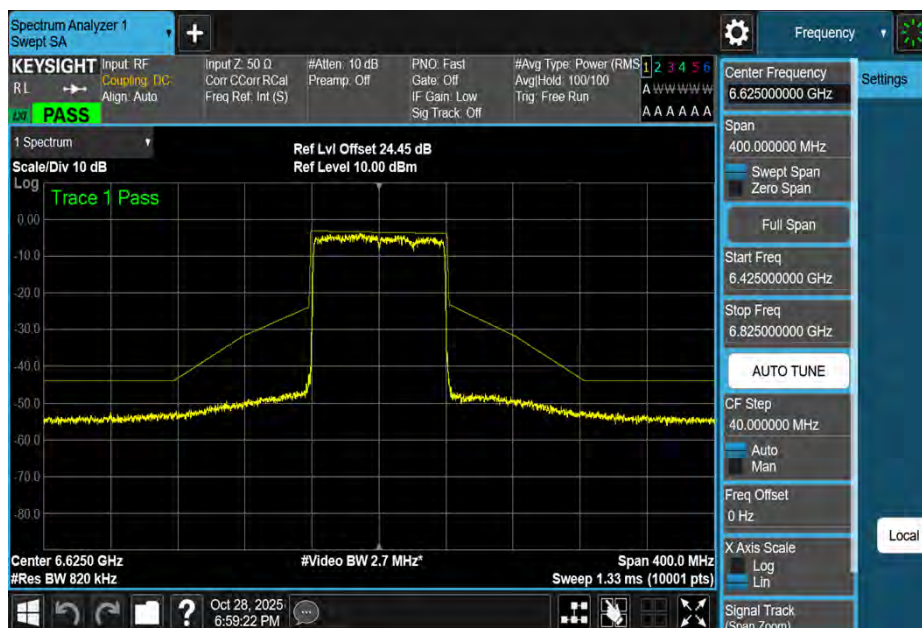
NTNV-11BE80MIMO-Ant2-6625-PASS
