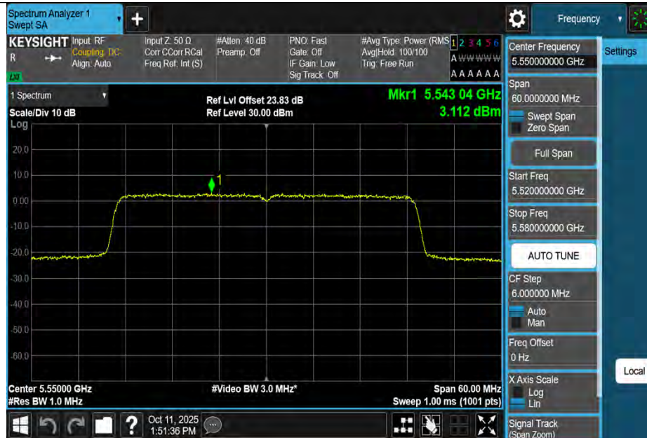
11AX40MIMO-Ant1-5550-PASS
