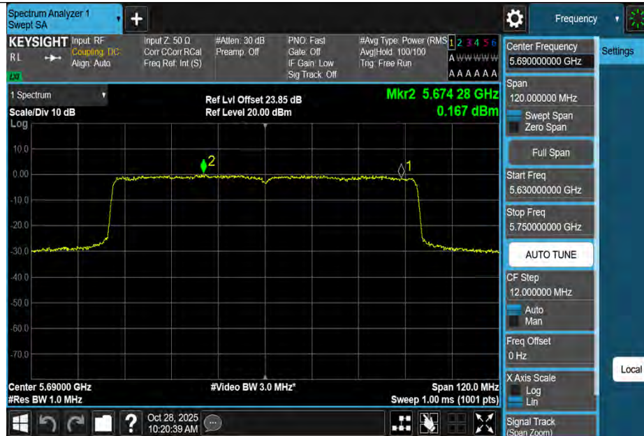
11AX80MIMO-Ant1-5690_UNII-2C-PASS
