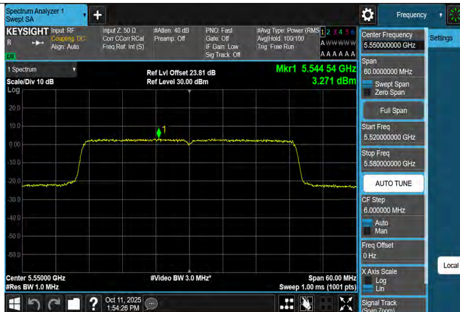
11AX40MIMO-Ant3-5550-PASS
