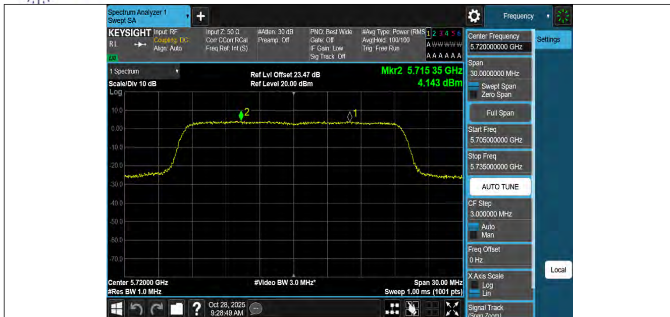
11AX20MIMO-Ant1-5720_UNII-2C-PASS
