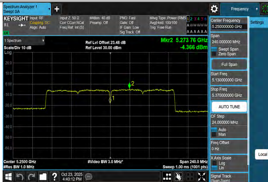
11AX160MIMO-Ant2-5250_UNII-2A-PASS
