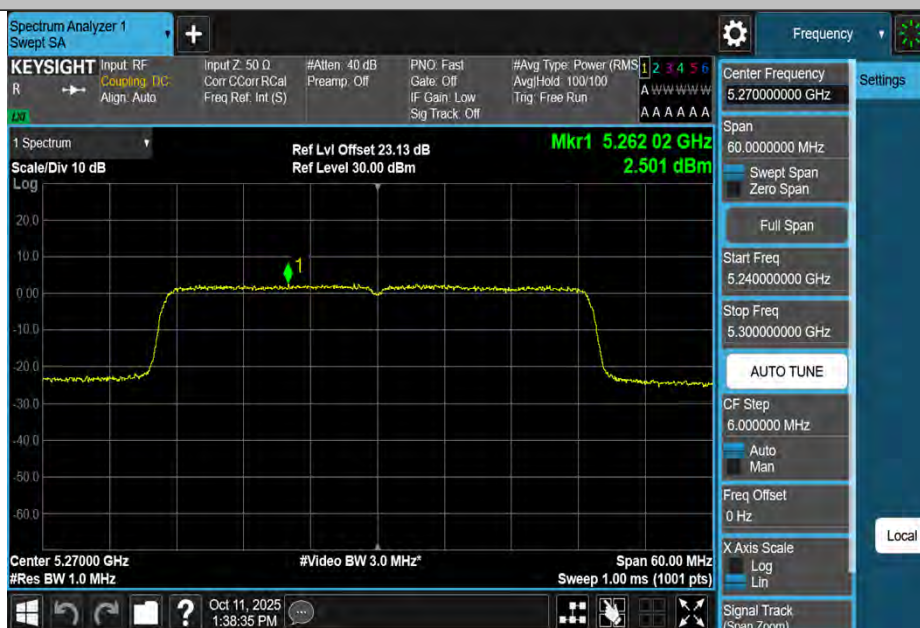
11AX40MIMO-Ant2-5270-PASS
