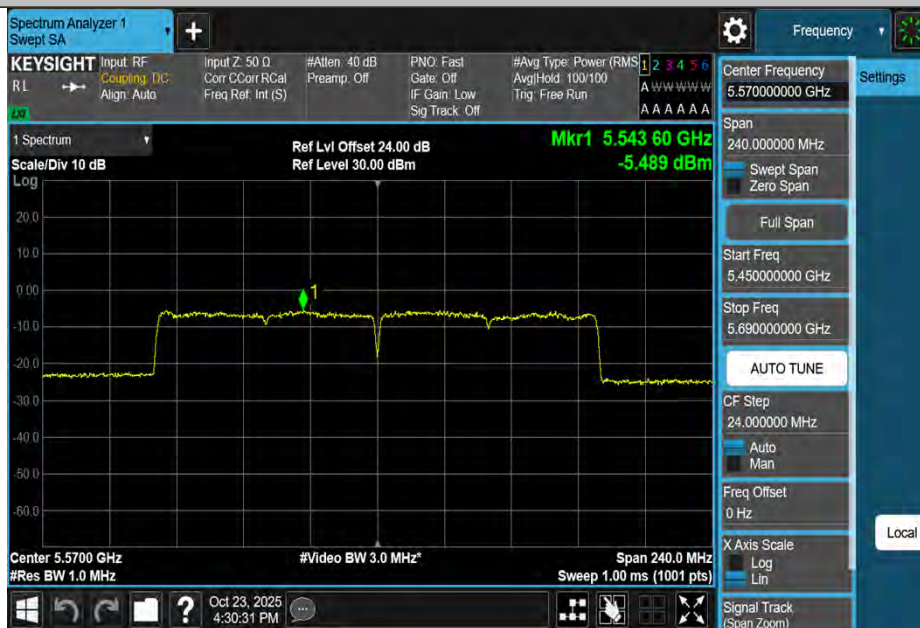
11AX160MIMO-Ant2-5570-PASS
