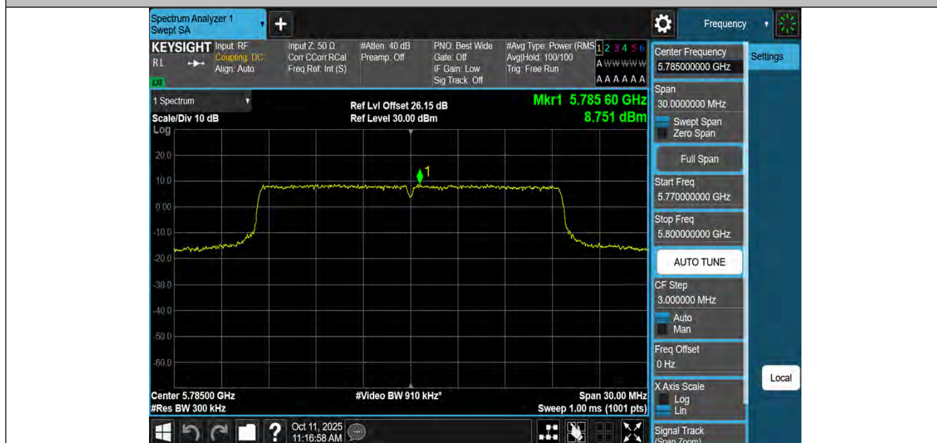
11AX20MIMO-Ant2-5785-PASS
