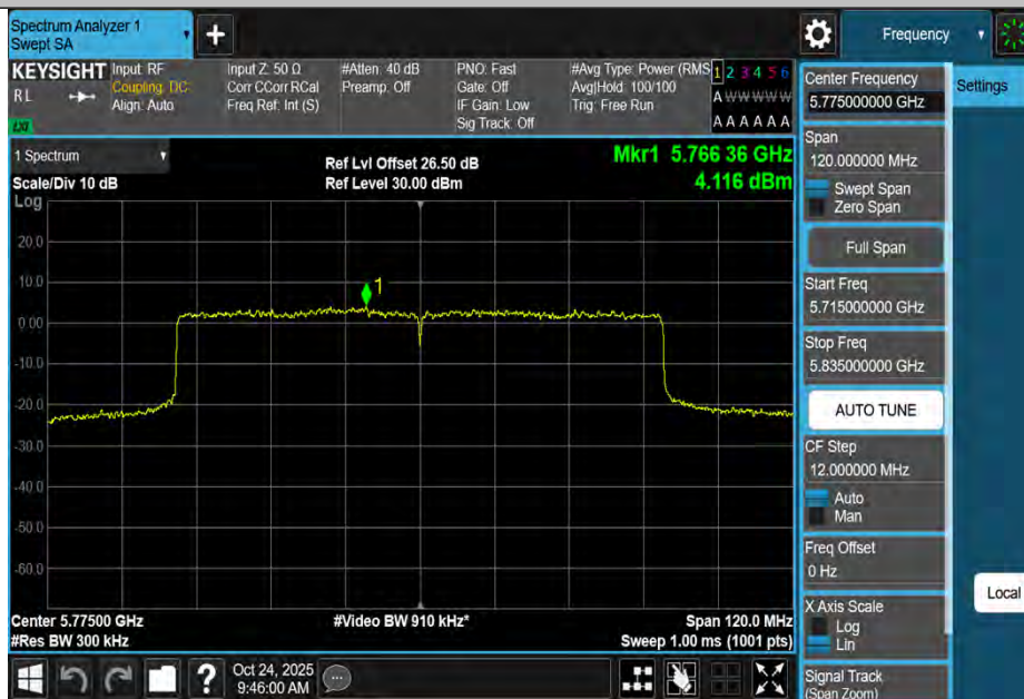
11AX80MIMO-Ant2-5775-PASS
