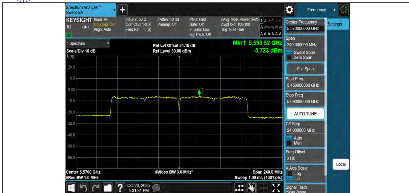
11AX160MIMO-Ant3-5570-PASS
