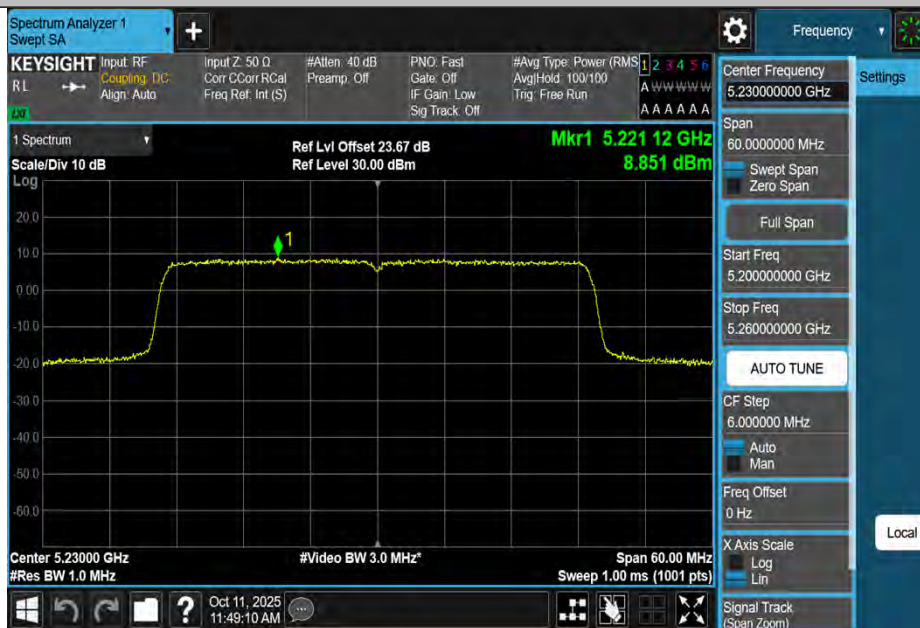
11AX40MIMO-Ant2-5230-PASS
