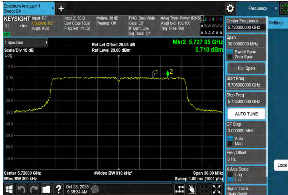
11AX20MIMO-Ant3-5720_UNII-3-PASS
