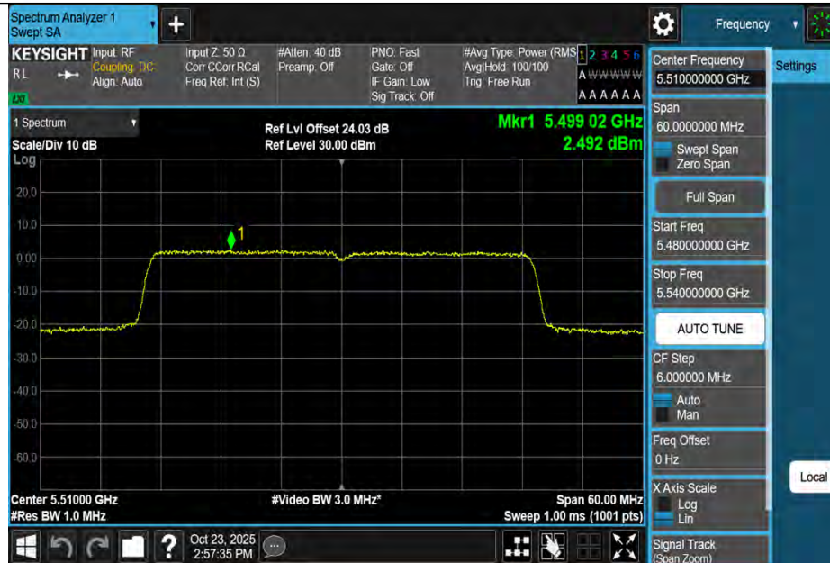
11AX40MIMO-Ant3-5510-PASS
