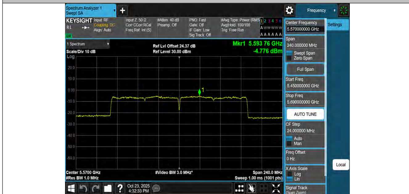
11AX160MIMO-Ant4-5570-PASS
