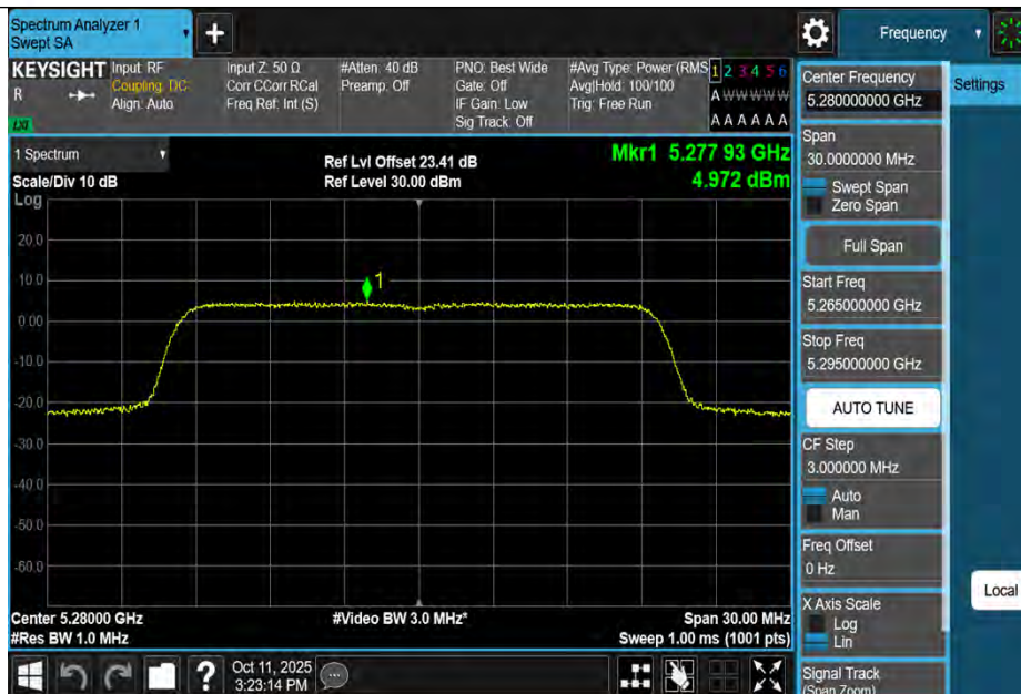
11BE20MIMO-Ant1-5280-PASS
