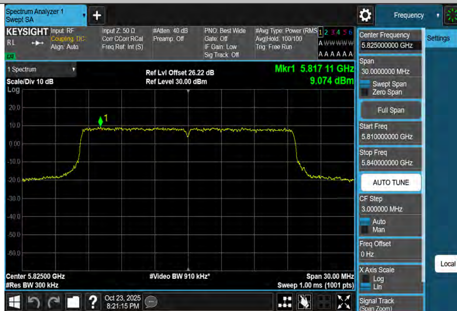
11AX20MIMO-Ant4-5825-PASS
