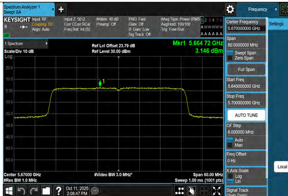
11AX40MIMO-Ant3-5670-PASS
