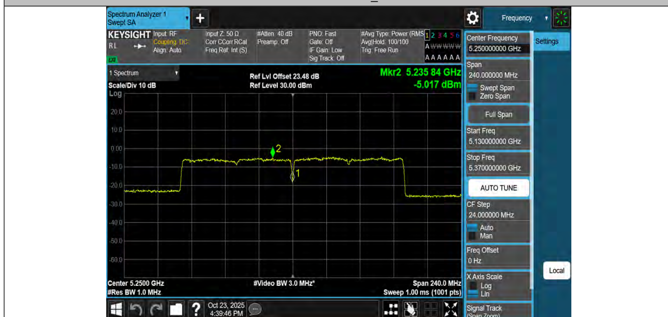
11AX160MIMO-Ant2-5250_UNII-1-PASS
