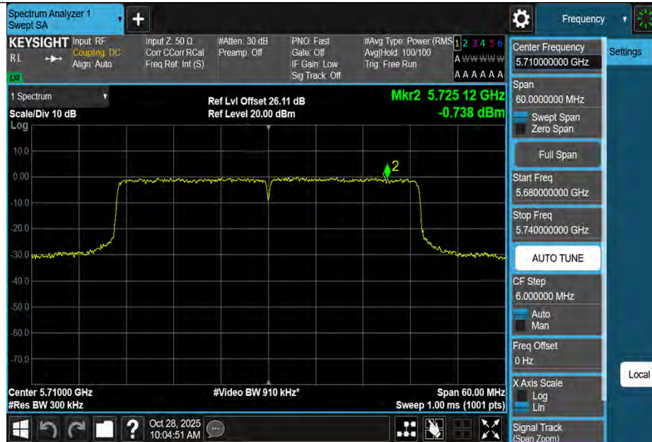
11AX40MIMO-Ant3-5710_UNII-3-PASS
