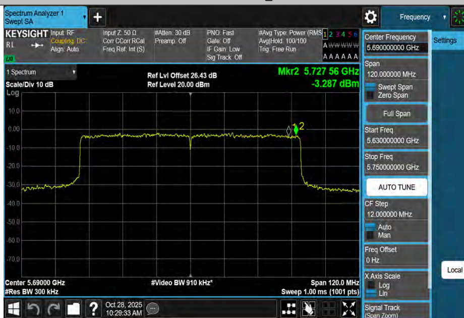
11AX80MIMO-Ant4-5690_UNII-3-PASS
