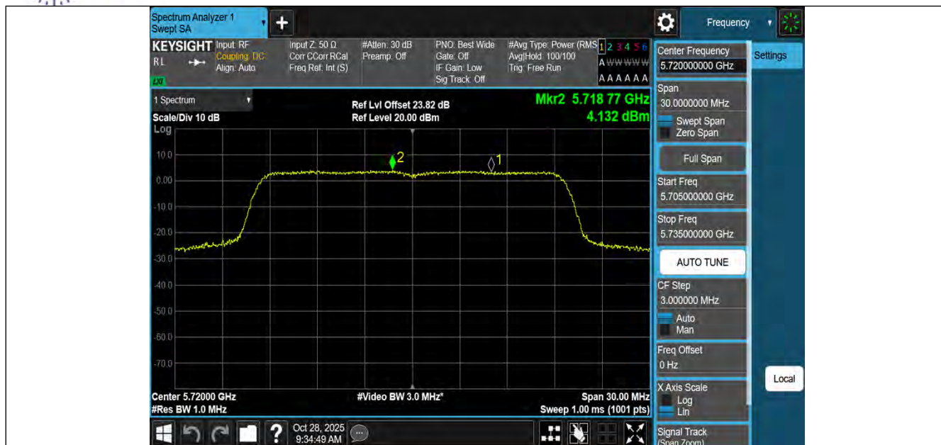
11AX20MIMO-Ant3-5720_UNII-2C-PASS
