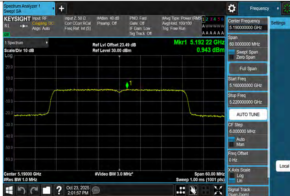
11AX40MIMO-Ant1-5190-PASS
