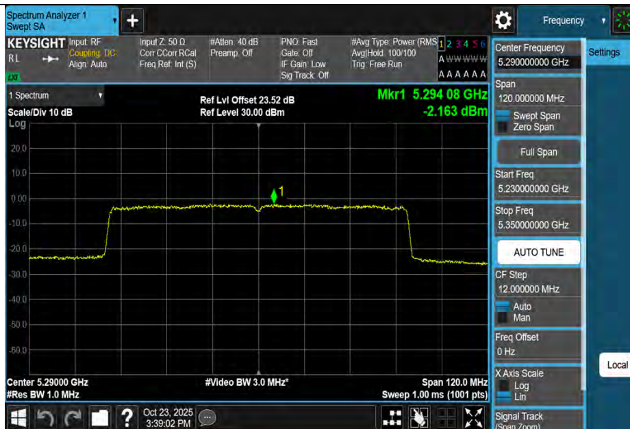
11AX80MIMO-Ant1-5290-PASS
