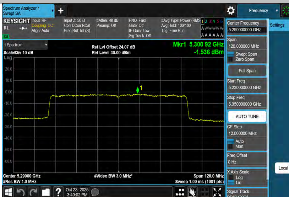
11AX80MIMO-Ant2-5290-PASS
