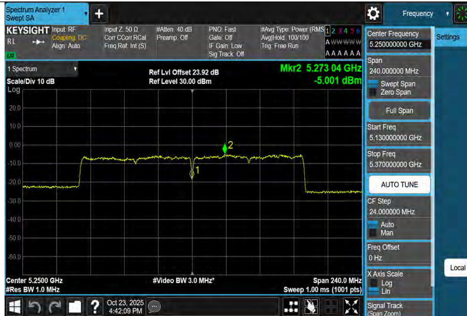
11AX160MIMO-Ant3-5250_UNII-2A-PASS
