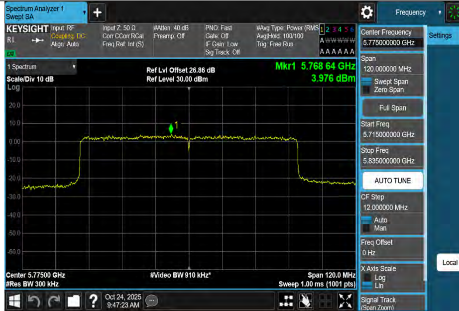
11AX80MIMO-Ant3-5775-PASS
