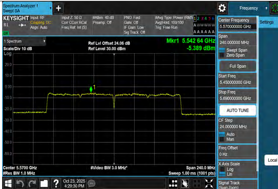
11AX160MIMO-Ant1-5570-PASS
