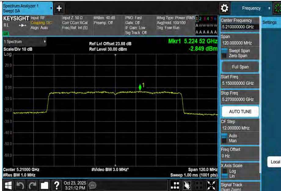
11AX80MIMO-Ant3-5210-PASS
