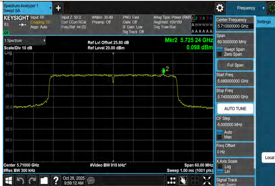
11AX40MIMO-Ant1-5710_UNII-3-PASS
