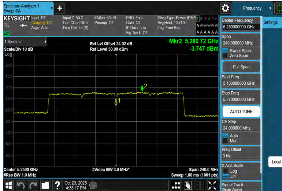
11AX160MIMO-Ant1-5250_UNII-2A-PASS
