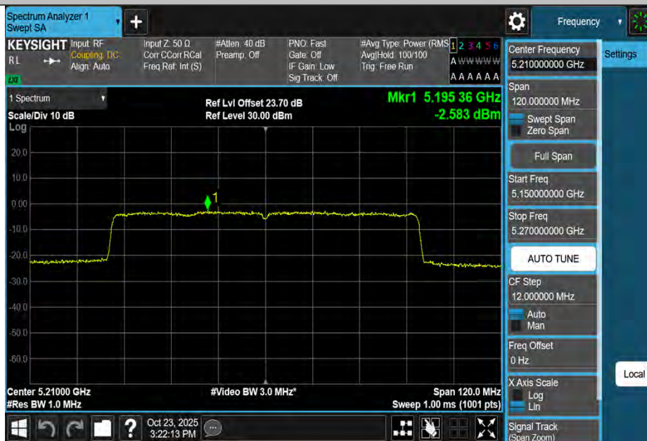
11AX80MIMO-Ant4-5210-PASS
