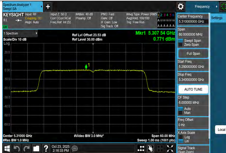
11AX40MIMO-Ant1-5310-PASS
