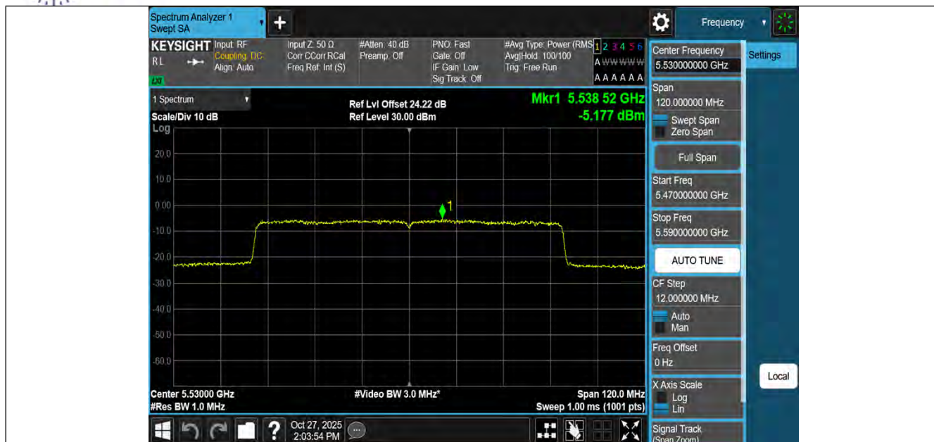
11AX80MIMO-Ant3-5530-PASS
