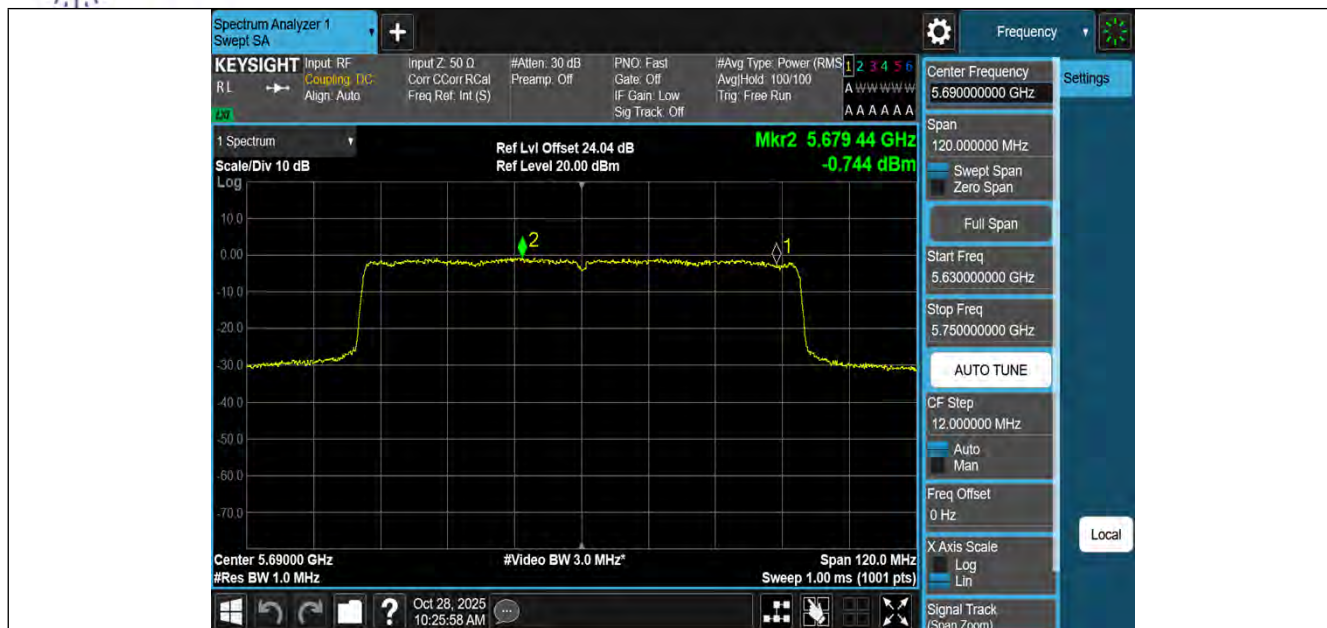
11AX80MIMO-Ant3-5690_UNII-2C-PASS
