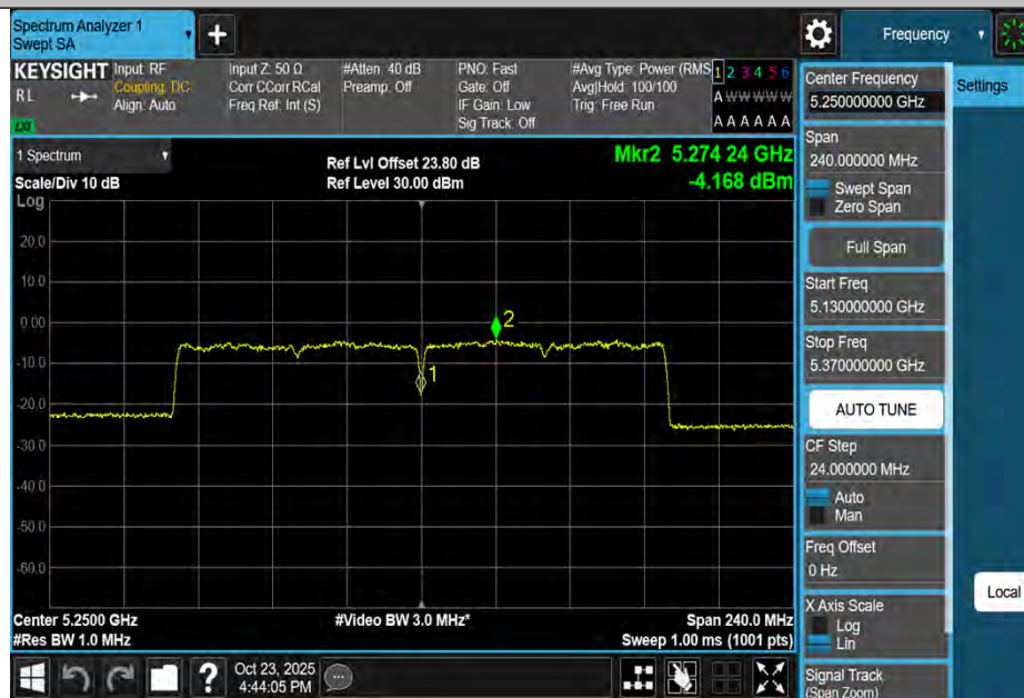
11AX160MIMO-Ant4-5250_UNII-2A-PASS
