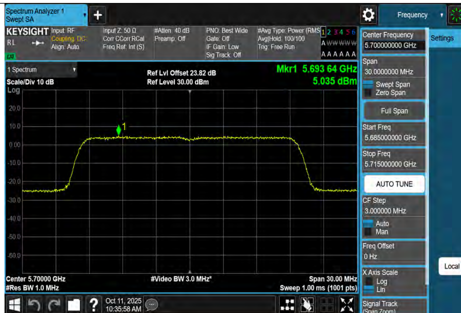
11AX20MIMO-Ant3-5700-PASS
