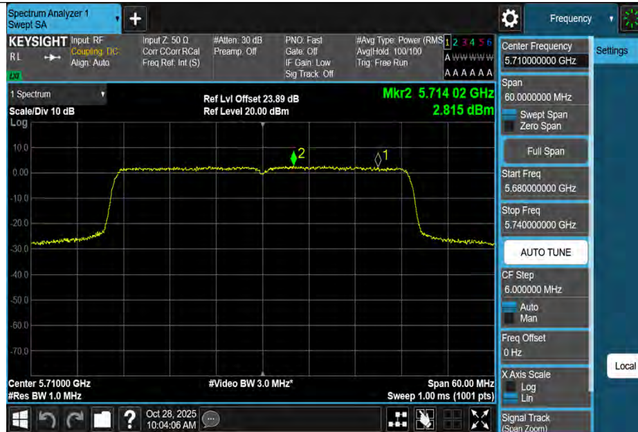
11AX40MIMO-Ant3-5710_UNII-2C-PASS
