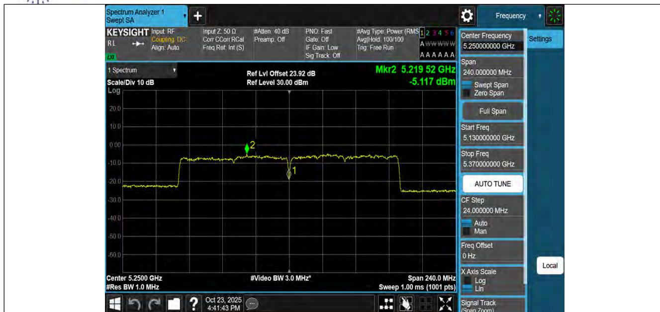
11AX160MIMO-Ant3-5250_UNII-1-PASS
