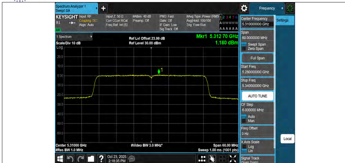
11AX40MIMO-Ant3-5310-PASS
