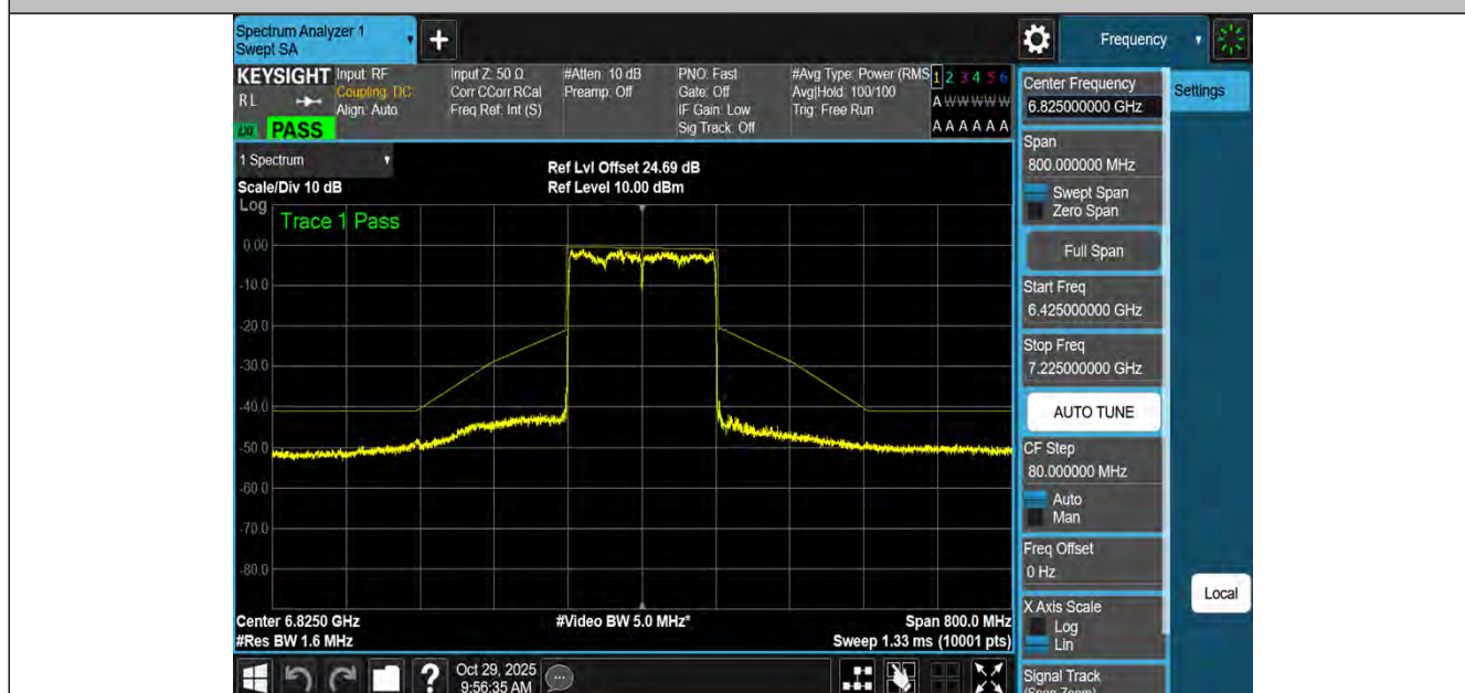
NTNV-11BE160MIMO-Ant4-6825-PASS
