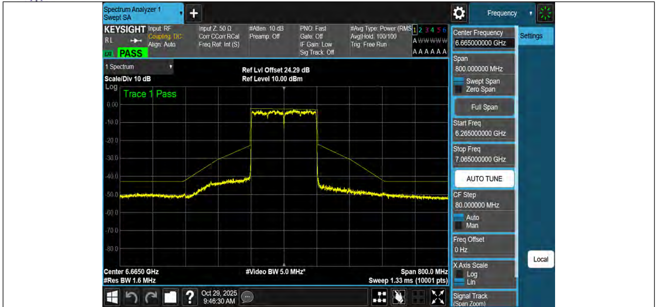
NTNV-11BE160MIMO-Ant1-6665-PASS
