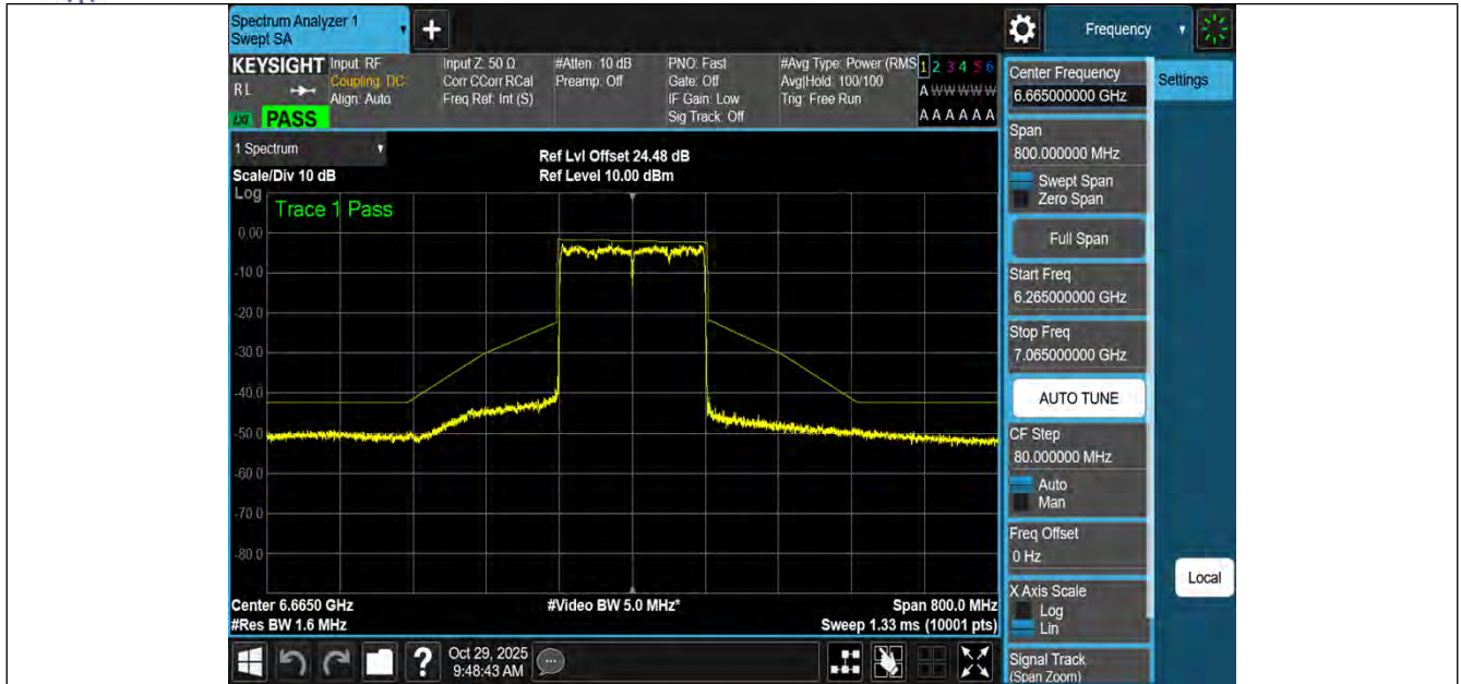
NTNV-11BE160MIMO-Ant3-6665-PASS
