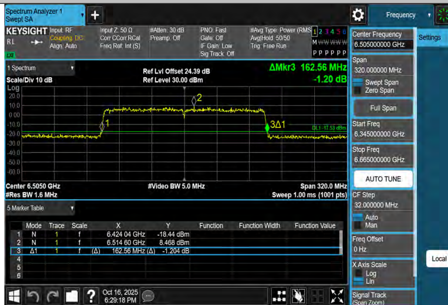
11AX160MIMO-Ant2-6505
