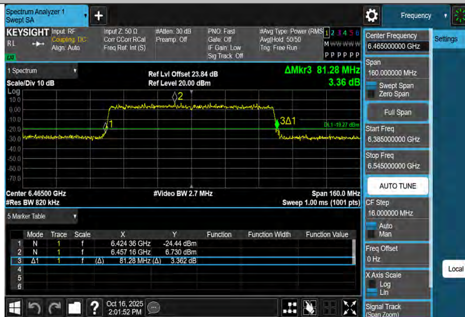
11AX80MIMO-Ant2-6465
