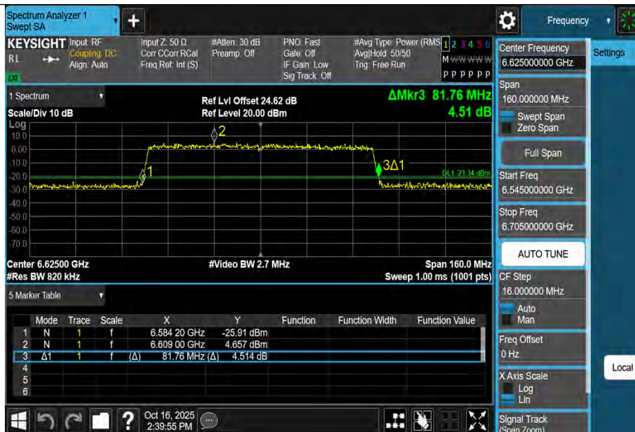
11AX80MIMO-Ant1-6625
