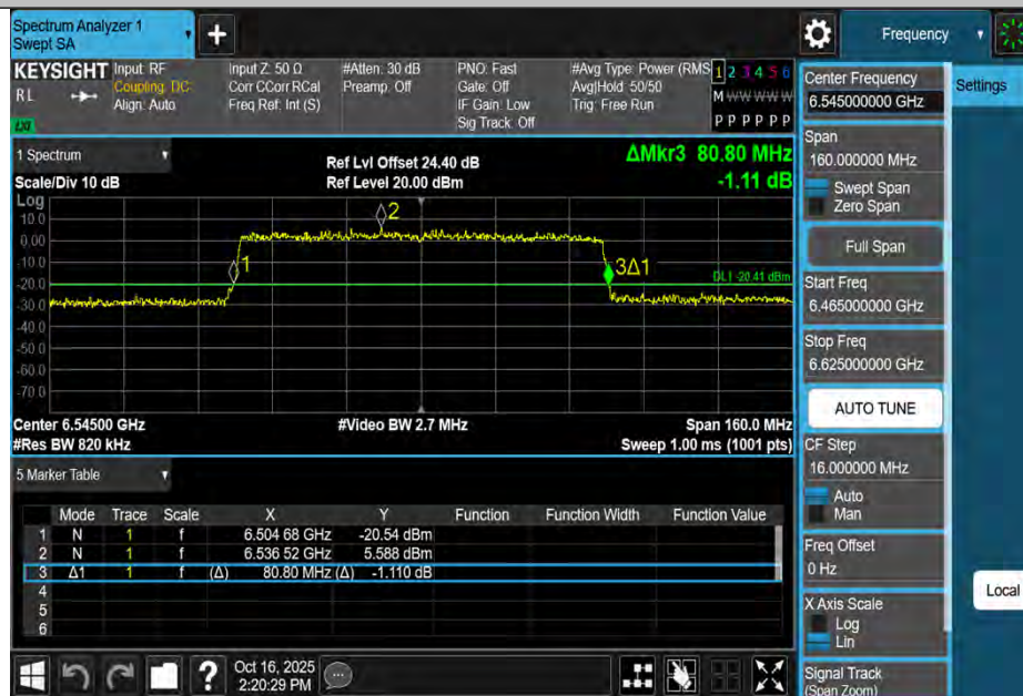
11AX80MIMO-Ant2-6545
