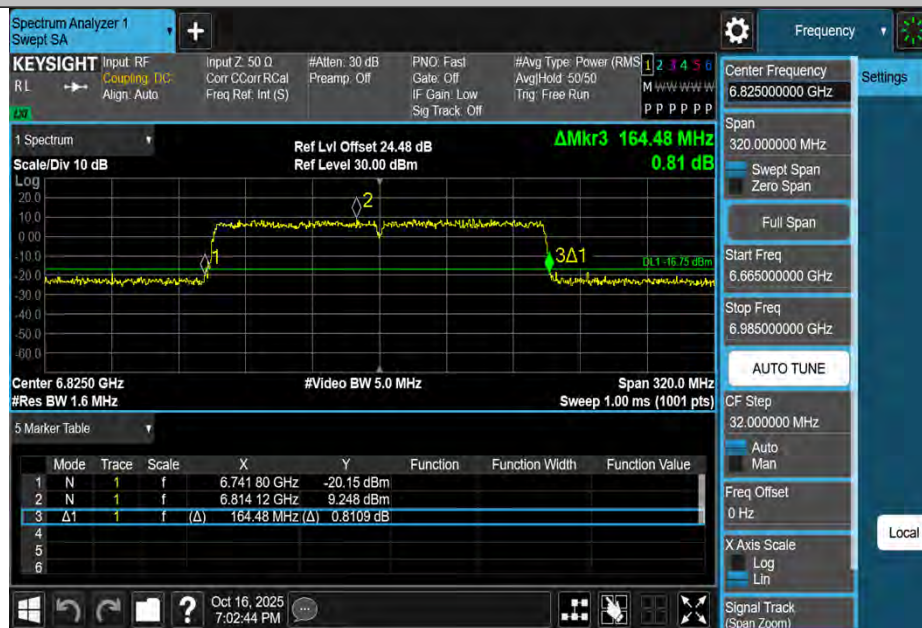
11AX160MIMO-Ant2-6825
