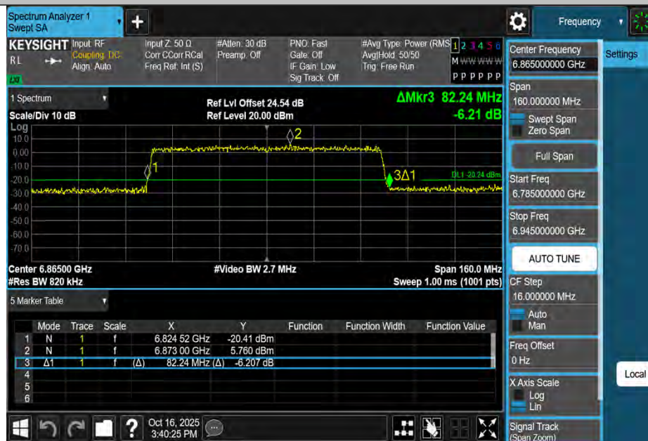
11AX80MIMO-Ant2-6865
