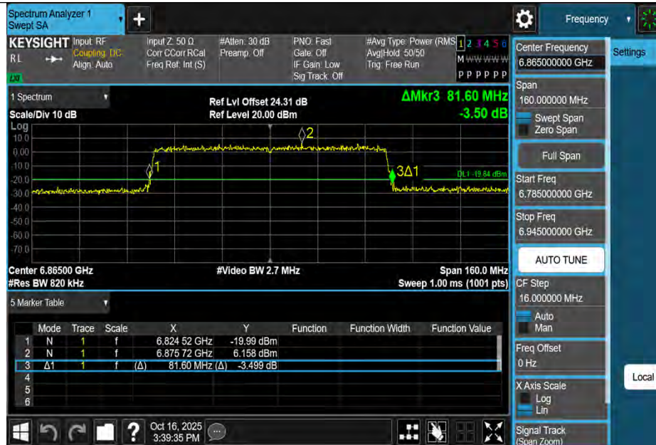
11AX80MIMO-Ant1-6865
