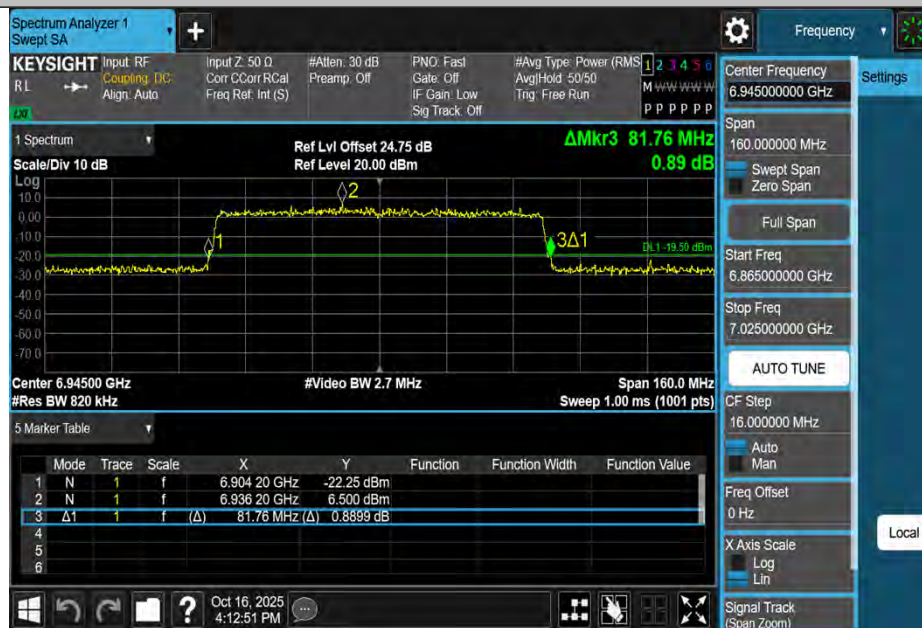
11AX80MIMO-Ant2-6945
