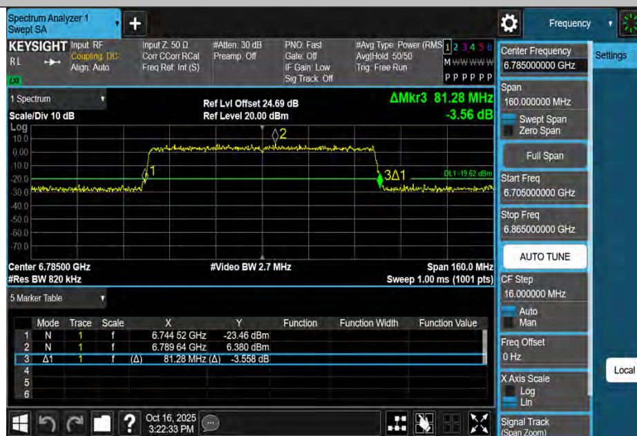
11AX80MIMO-Ant4-6785
