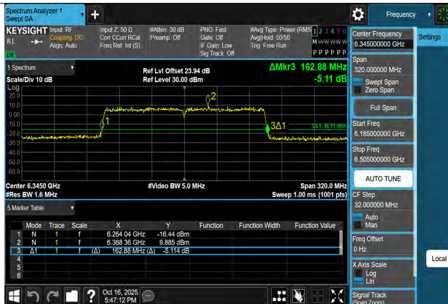
11AX160MIMO-Ant1-6345
