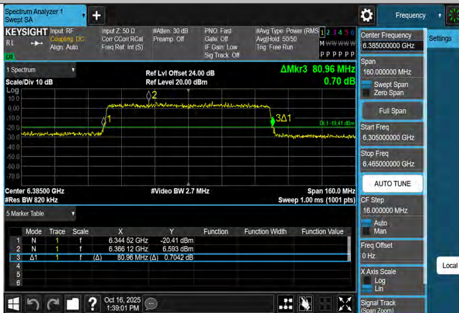
11AX80MIMO-Ant2-6385
