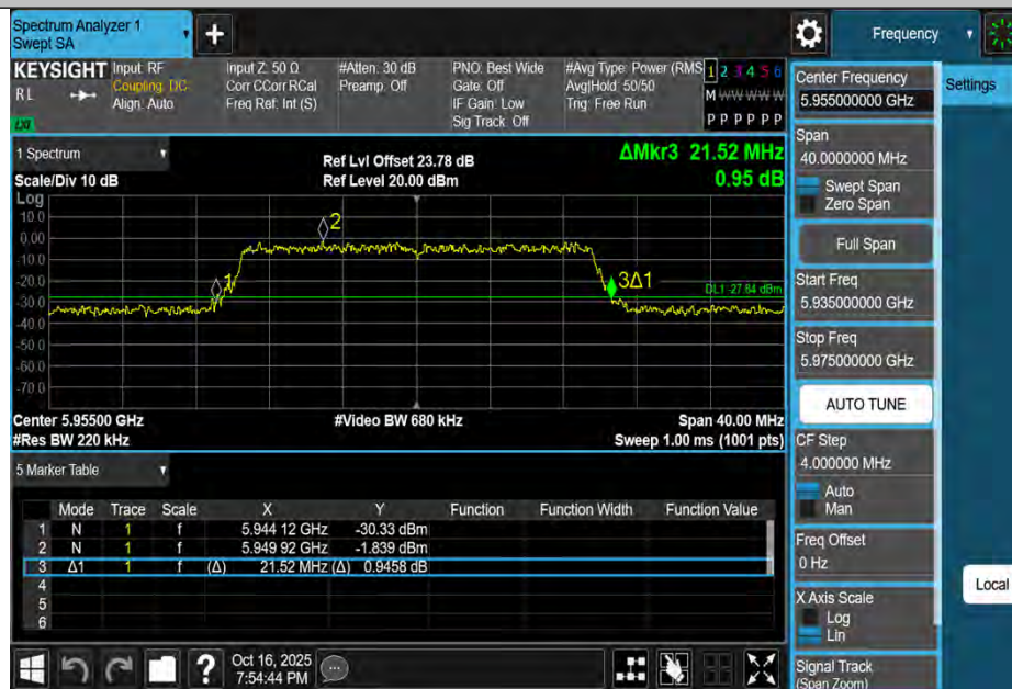
11BE20MIMO-Ant2-5955
