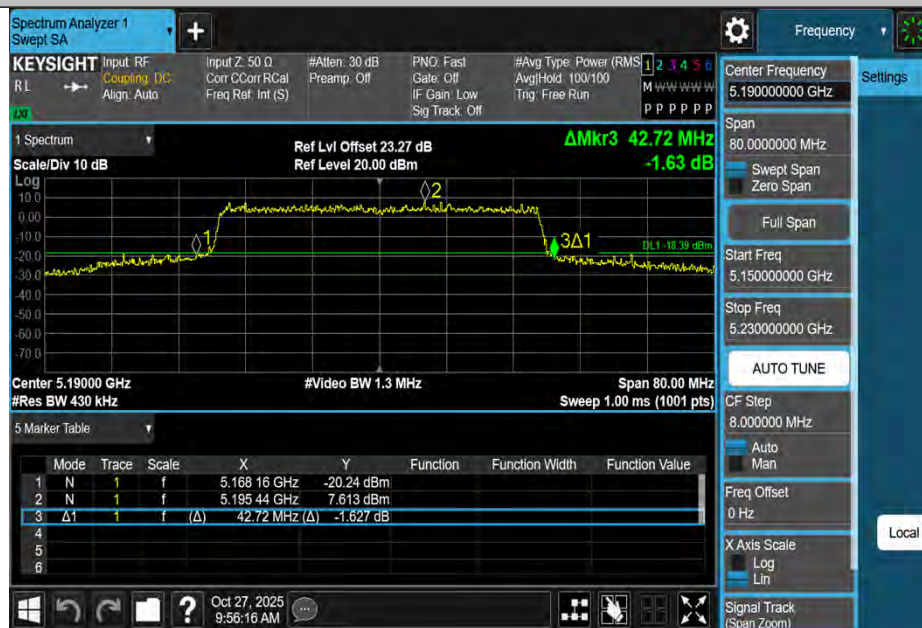
11AC40MIMO-Ant1-5190
