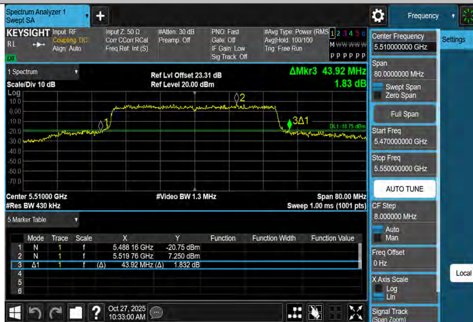
11AC40MIMO-Ant2-5510
