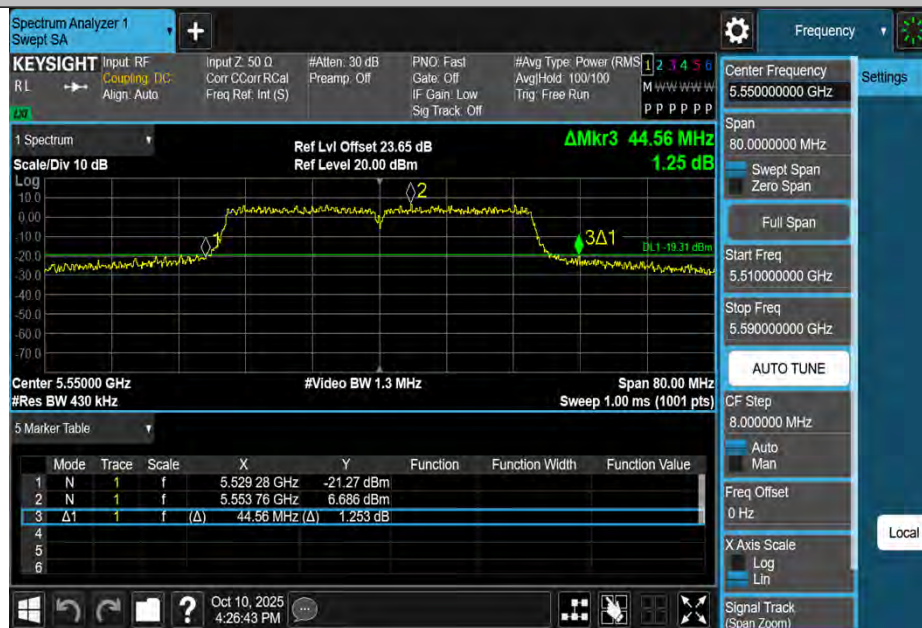
11AC40MIMO-Ant3-5550
