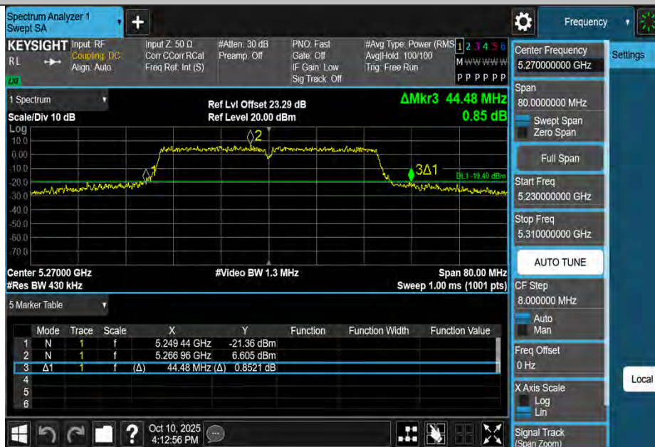
11AC40MIMO-Ant4-5270
