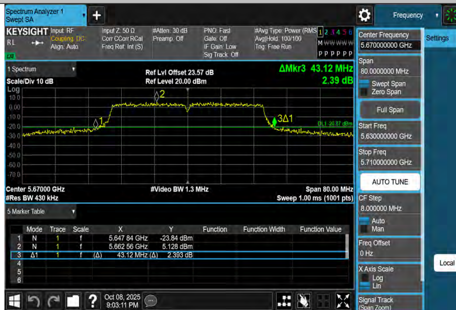
11N40MIMO-Ant3-5670
