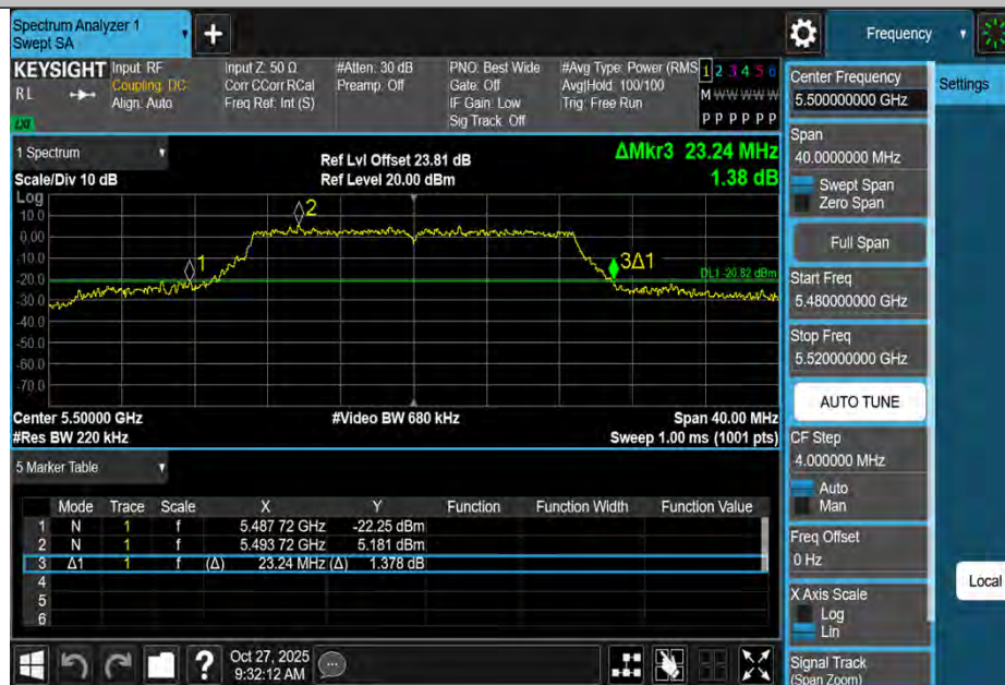
11AC20MIMO-Ant3-5500
