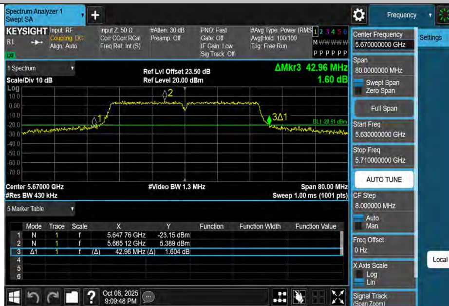
11N40MIMO-Ant1-5670
