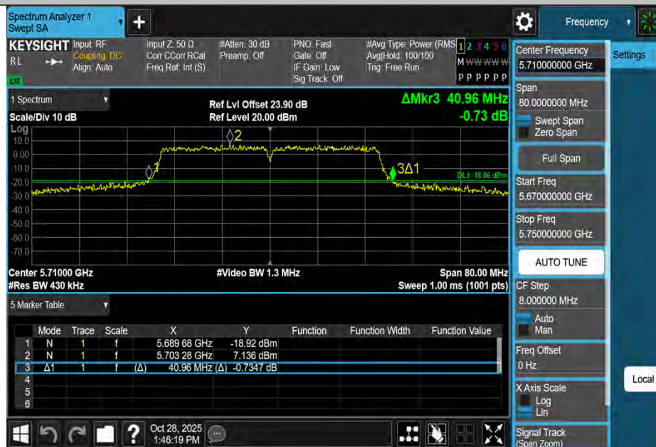
11N40MIMO-Ant4-5710
