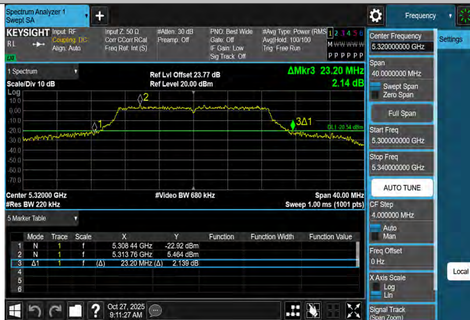
11AC20MIMO-Ant3-5320
