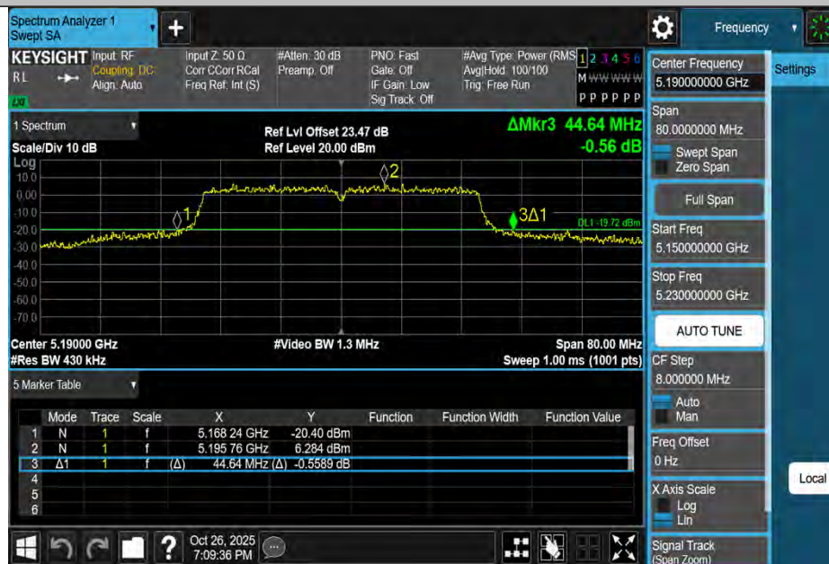
11N40MIMO-Ant3-5190
