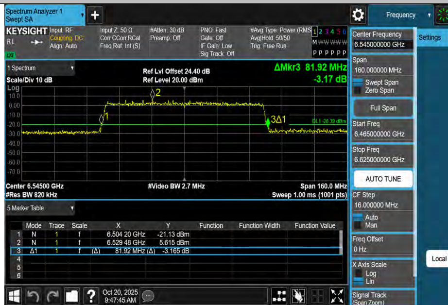
11BE80MIMO-Ant2-6545
