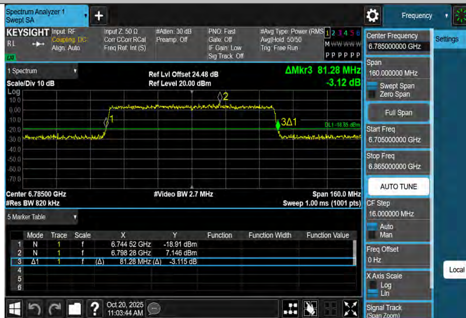
11BE80MIMO-Ant2-6785
