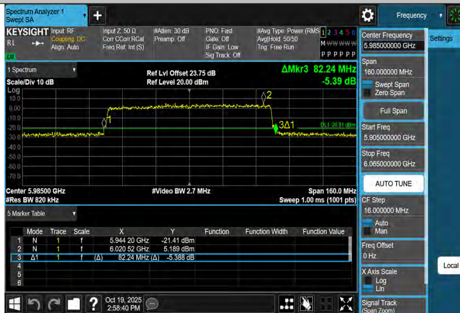
11BE80MIMO-Ant4-5985
