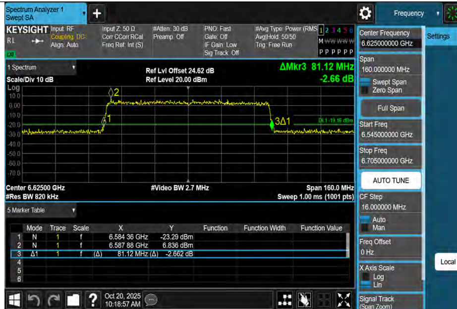
11BE80MIMO-Ant1-6625
