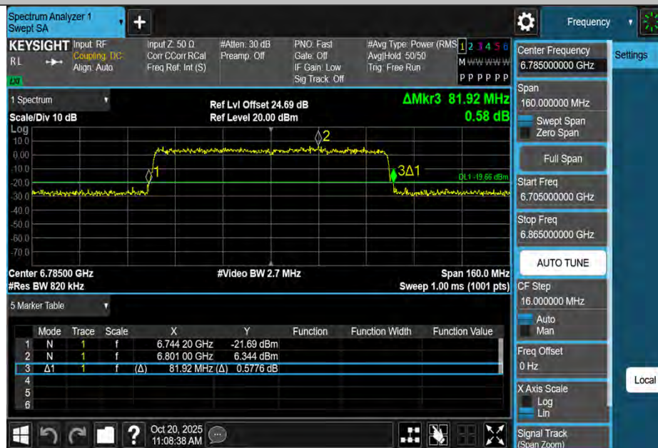
11BE80MIMO-Ant4-6785
