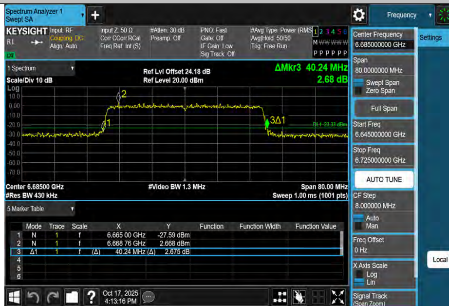
11BE40MIMO-Ant2-6685
