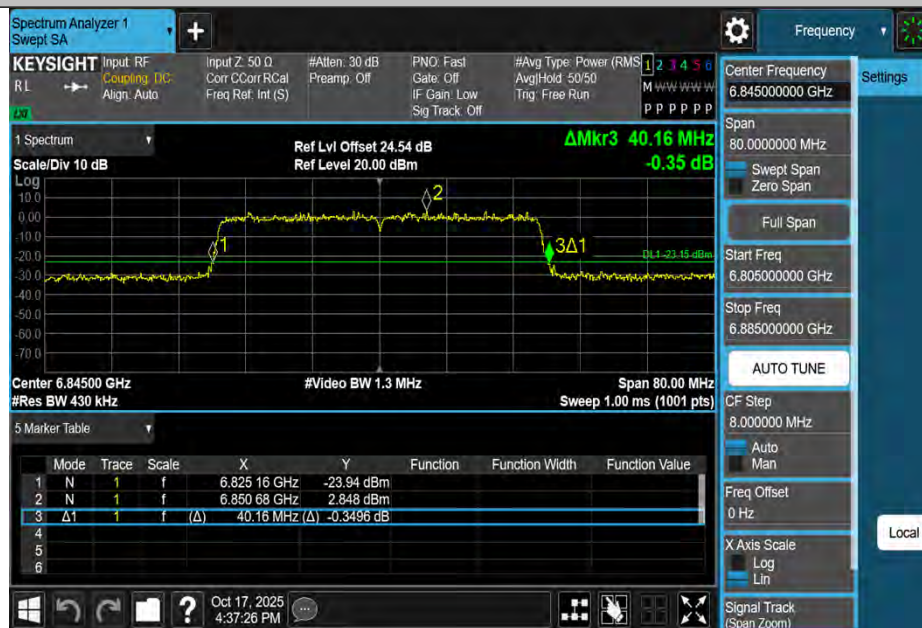
11BE40MIMO-Ant2-6845
