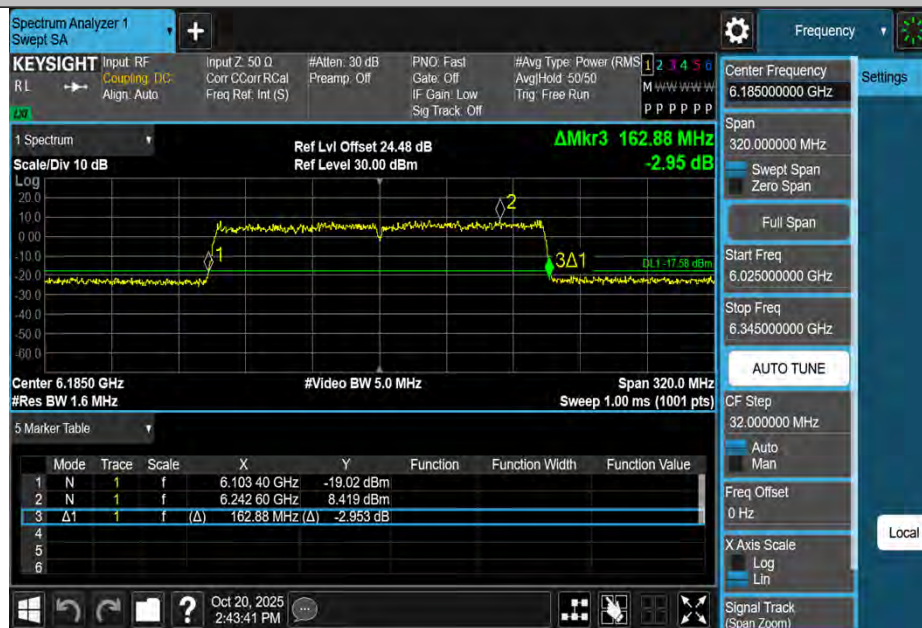
11BE160MIMO-Ant2-6185
