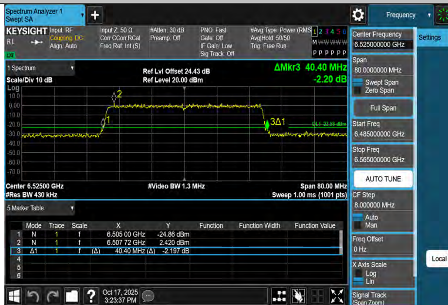
11BE40MIMO-Ant4-6525
