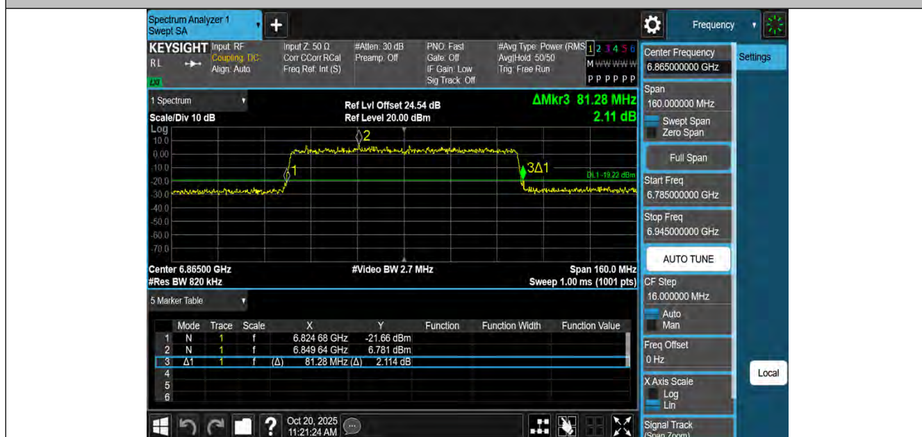
11BE80MIMO-Ant2-6865
