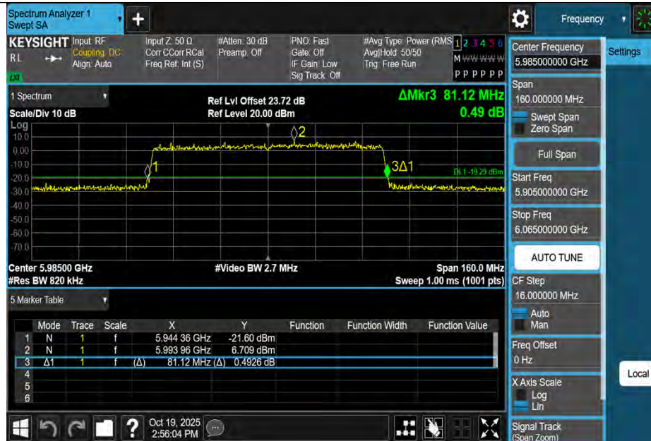
11BE80MIMO-Ant3-5985
