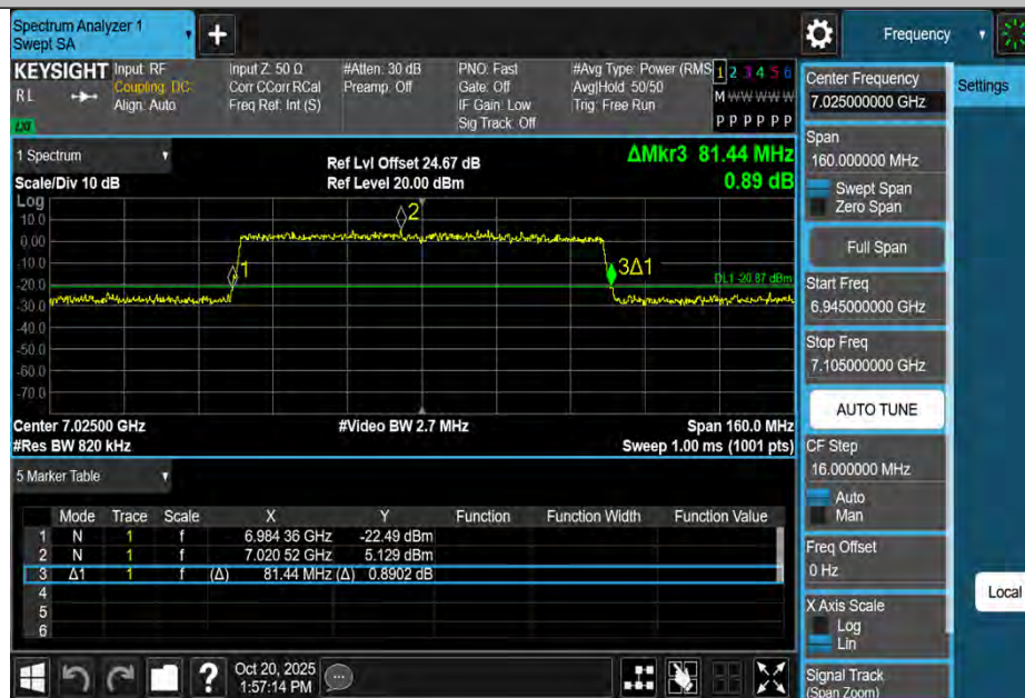
11BE80MIMO-Ant4-7025
