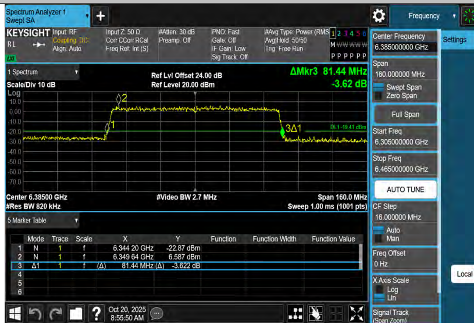
11BE80MIMO-Ant2-6385
