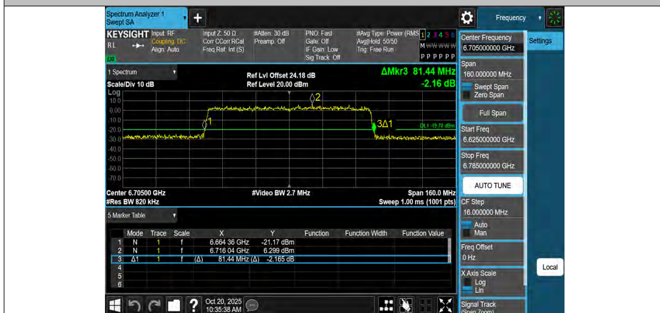
11BE80MIMO-Ant2-6705
