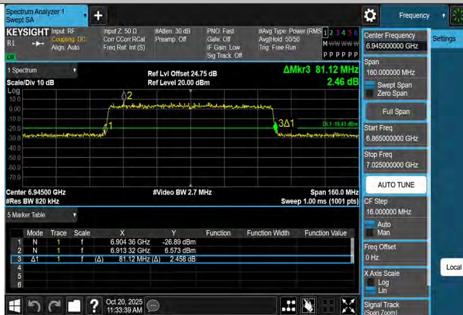
11BE80MIMO-Ant2-6945
