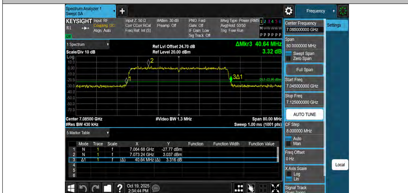
11BE40MIMO-Ant2-7085
