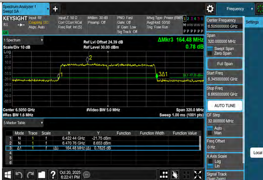
11BE160MIMO-Ant2-6505
