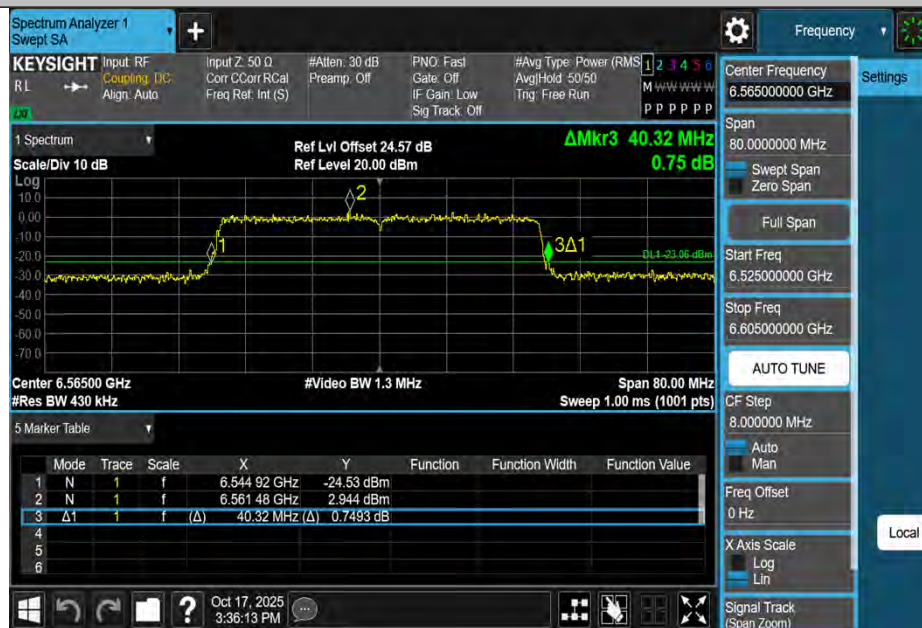
11BE40MIMO-Ant4-6565
