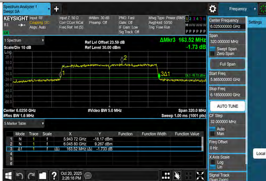
11BE160MIMO-Ant2-6025
