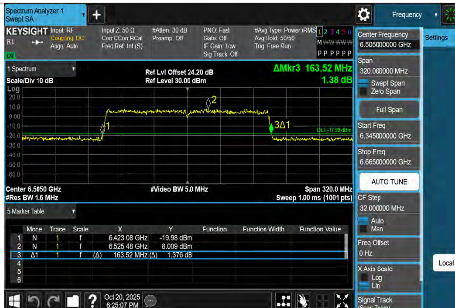
11BE160MIMO-Ant3-6505
