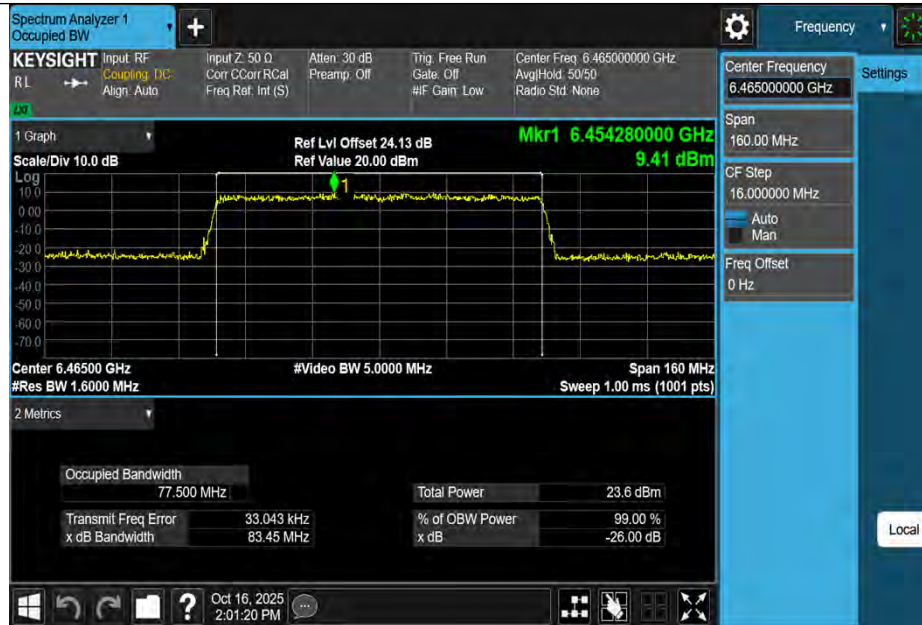
11AX80MIMO-Ant1-6465-PASS
