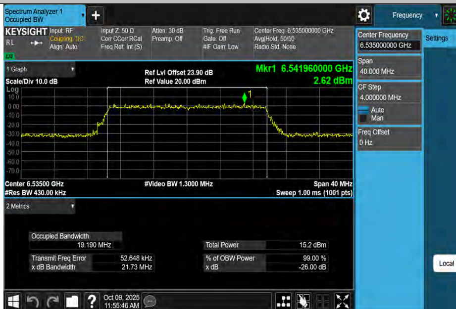
11AX20MIMO-Ant2-6535-PASS
