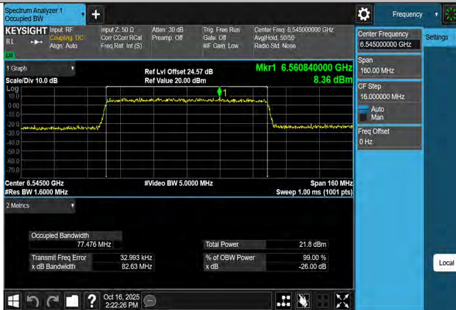
11AX80MIMO-Ant4-6545-PASS
