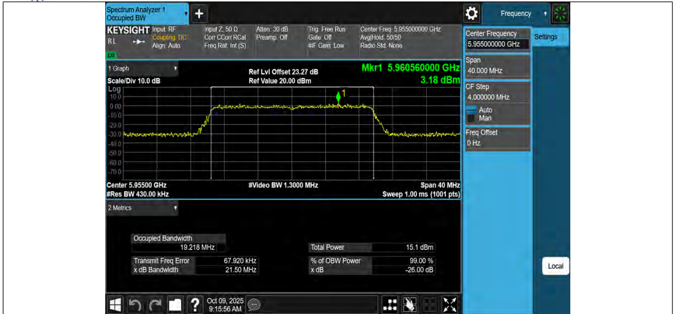
11AX20MIMO-Ant3-5955-PASS
