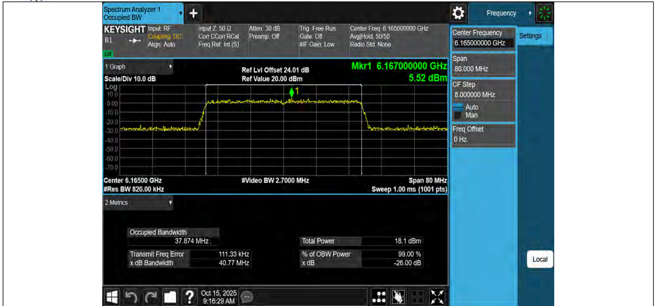
11AX40MIMO-Ant3-6165-PASS
