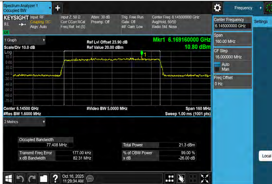
11AX80MIMO-Ant1-6145-PASS
