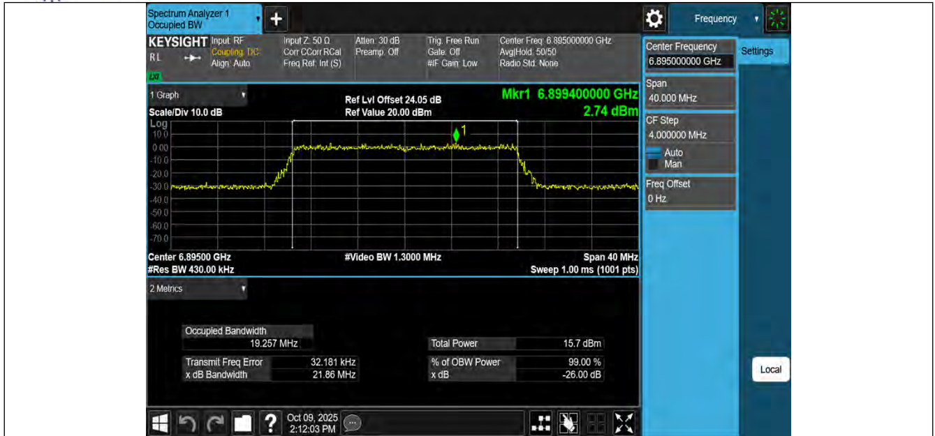
11AX20MIMO-Ant3-6895-PASS
