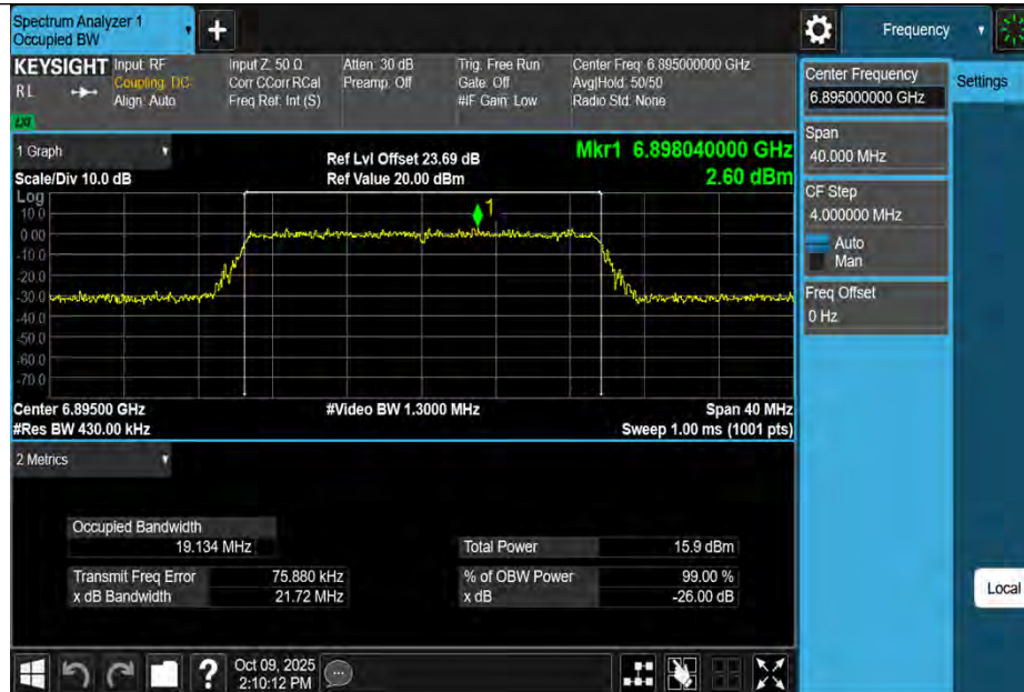
11AX20MIMO-Ant1-6895-PASS
