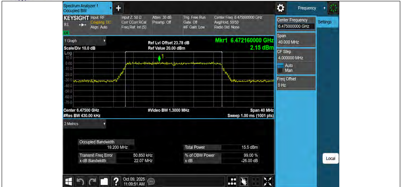
11AX20MIMO-Ant3-6475-PASS
