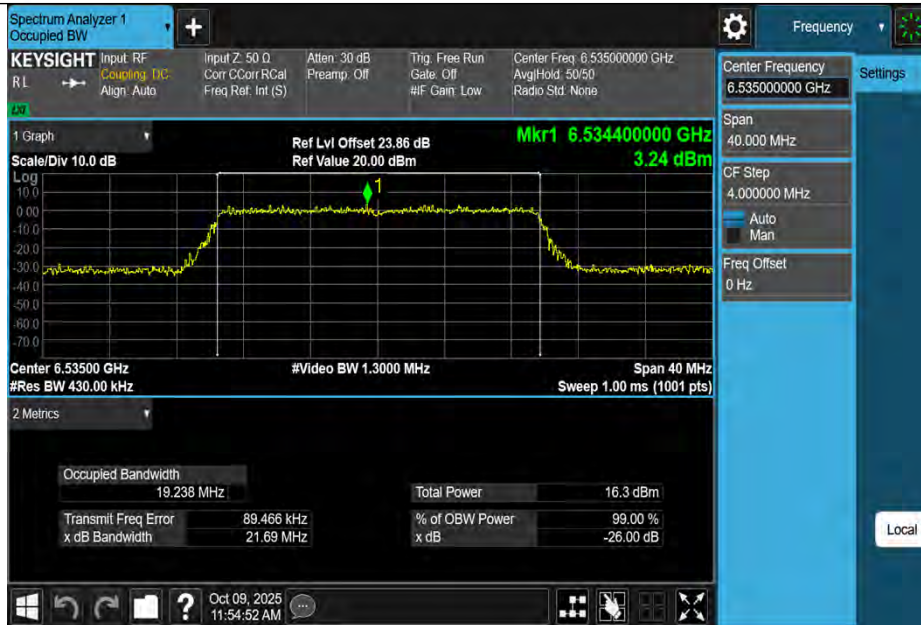
11AX20MIMO-Ant1-6535-PASS
