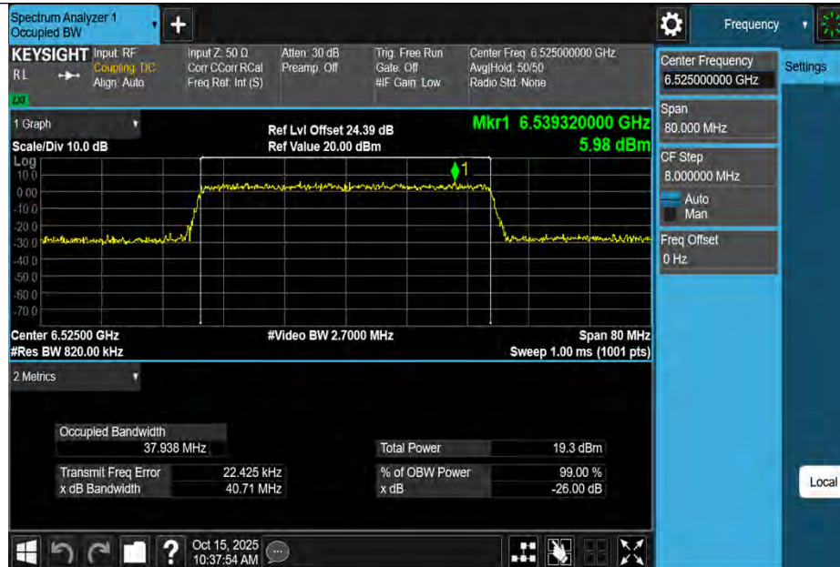
11AX40MIMO-Ant1-6525-PASS
