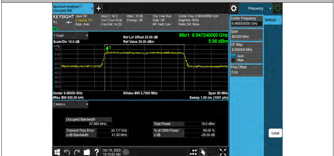
11AX40MIMO-Ant4-6965-PASS
