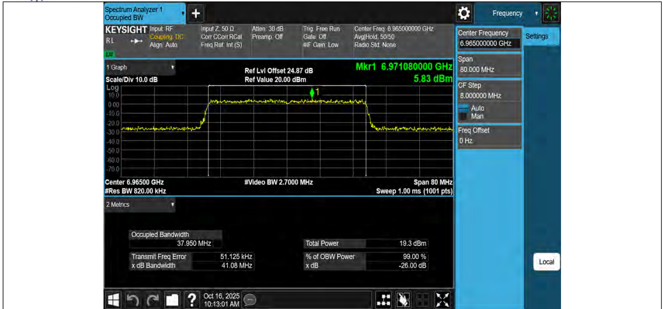
11AX40MIMO-Ant3-6965-PASS
