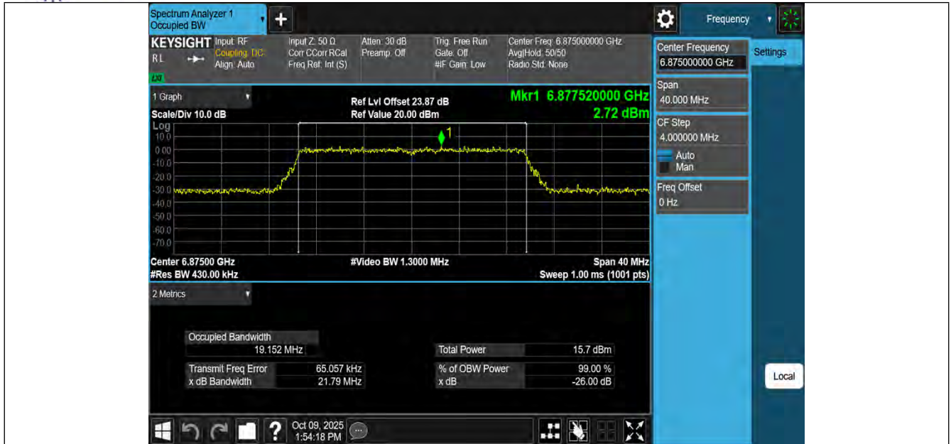
11AX20MIMO-Ant1-6875-PASS
