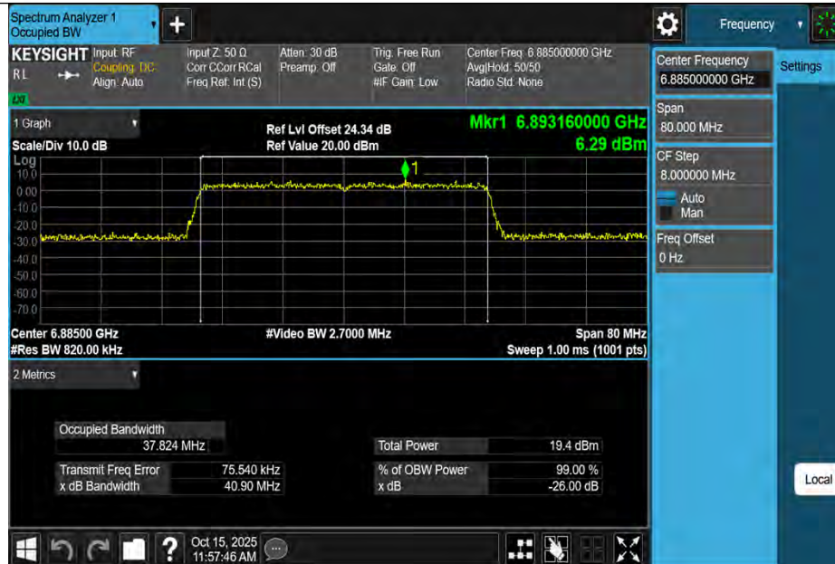
11AX40MIMO-Ant1-6885-PASS
