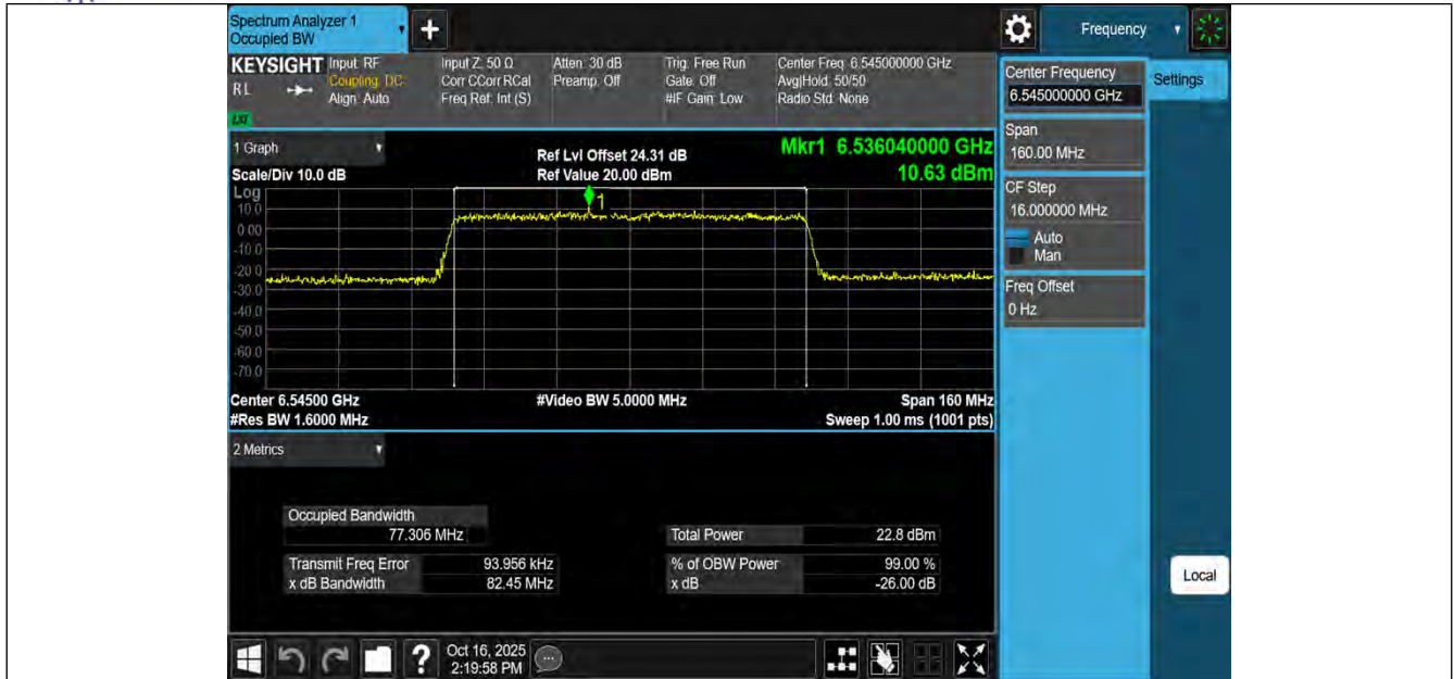
11AX80MIMO-Ant1-6545-PASS
