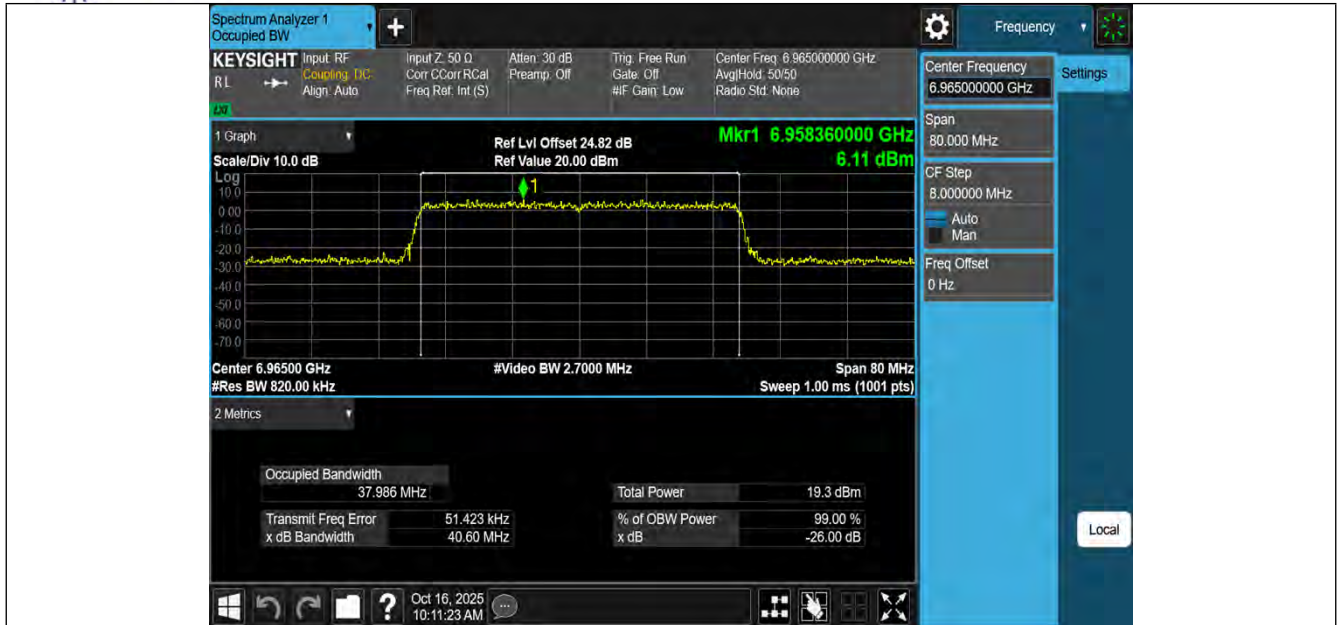
11AX40MIMO-Ant1-6965-PASS
