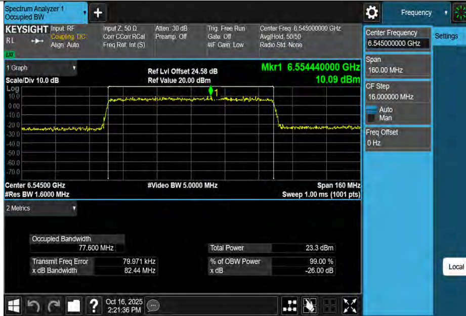
11AX80MIMO-Ant3-6545-PASS
