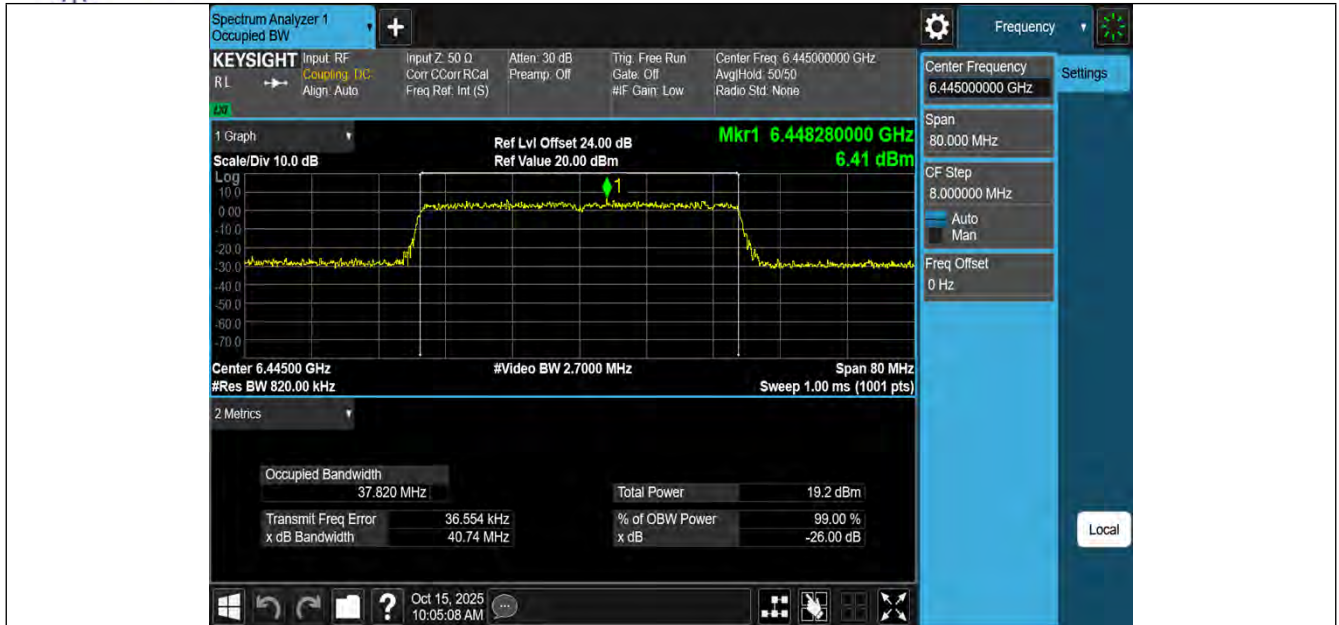
11AX40MIMO-Ant1-6445-PASS
