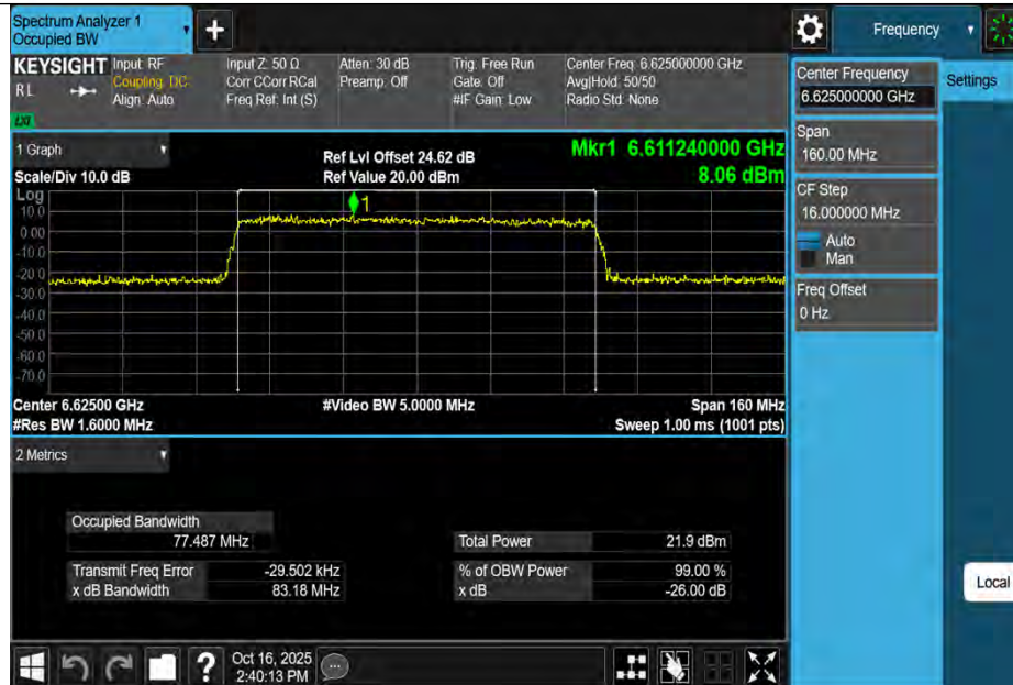
11AX80MIMO-Ant1-6625-PASS
