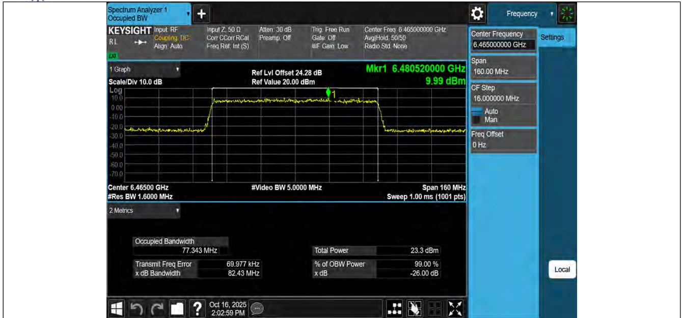
11AX80MIMO-Ant3-6465-PASS
