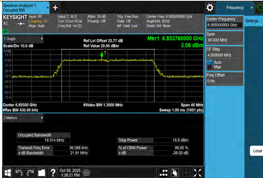
11AX20MIMO-Ant1-6855-PASS
