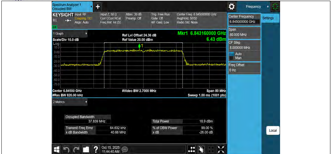
11AX40MIMO-Ant1-6845-PASS
