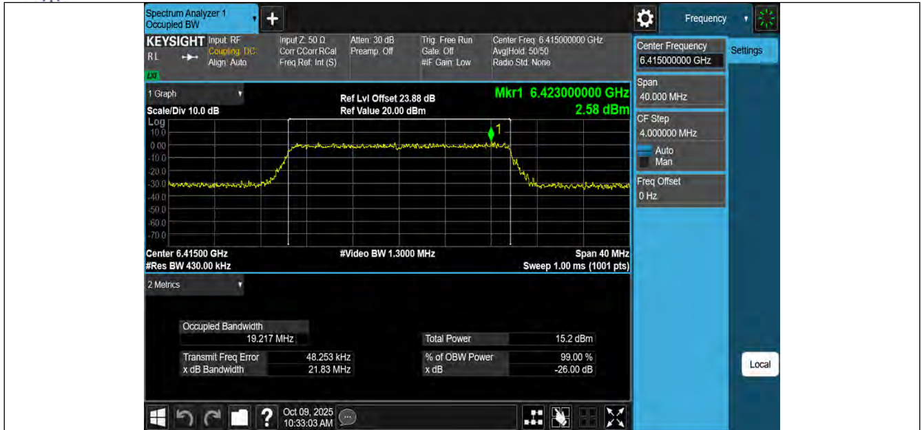
11AX20MIMO-Ant3-6415-PASS
