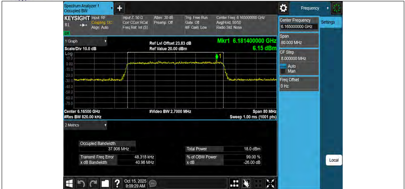
11AX40MIMO-Ant1-6165-PASS
