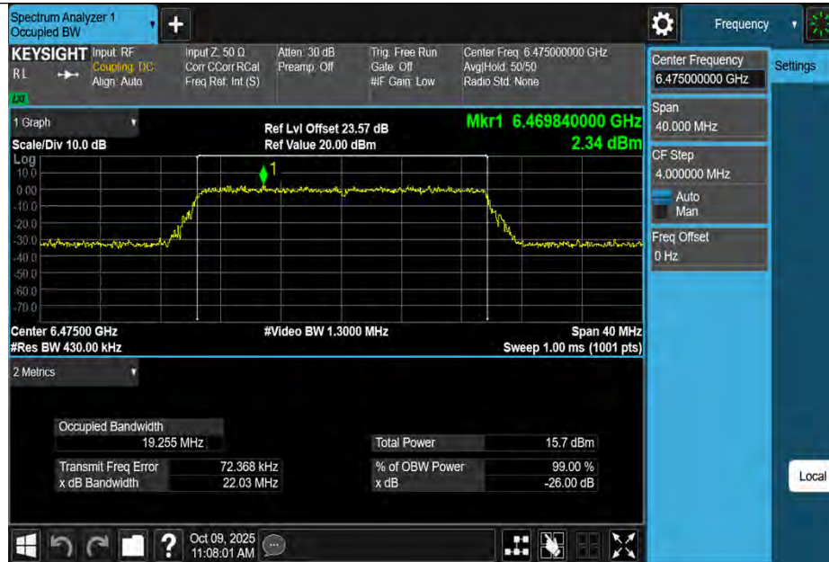
11AX20MIMO-Ant1-6475-PASS
