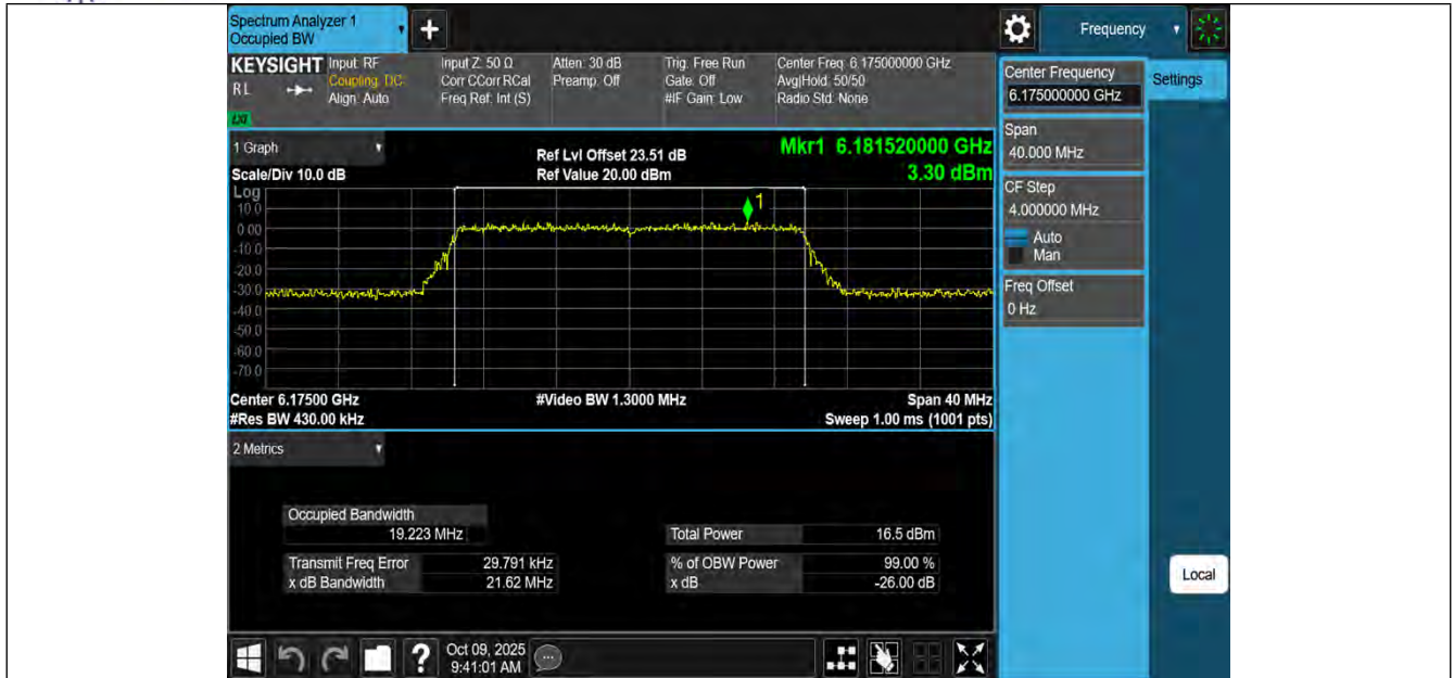
11AX20MIMO-Ant3-6175-PASS
