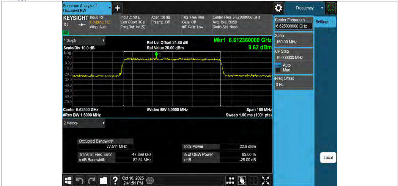
11AX80MIMO-Ant3-6625-PASS
