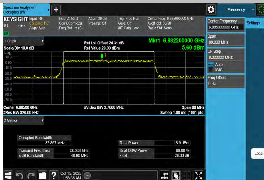
11AX40MIMO-Ant2-6885-PASS
