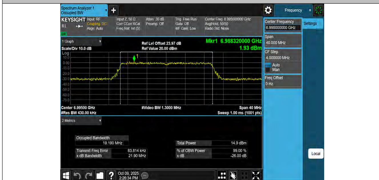
11AX20MIMO-Ant2-6995-PASS
