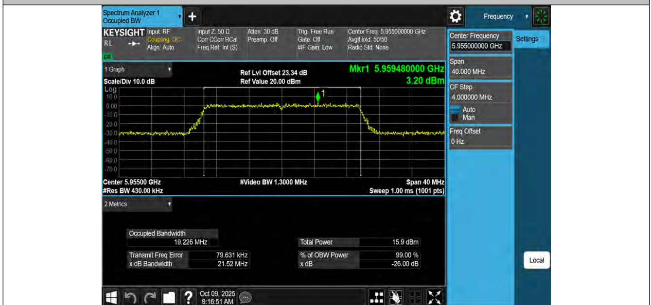
11AX20MIMO-Ant4-5955-PASS
