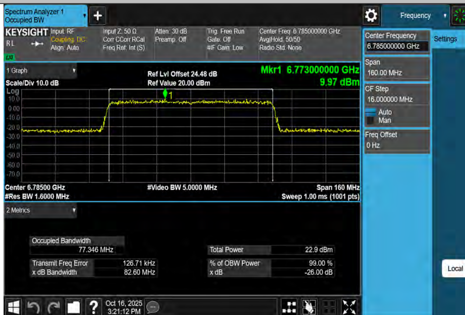
11AX80MIMO-Ant2-6785-PASS
