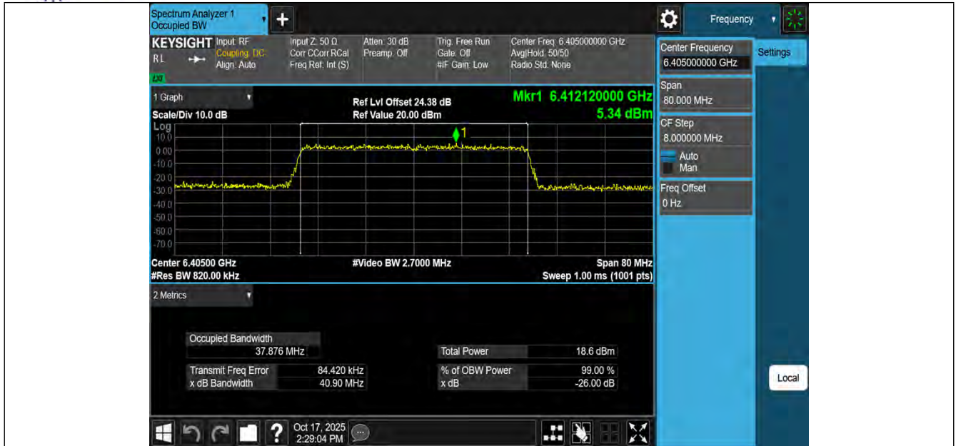
11BE40MIMO-Ant3-6405-PASS
