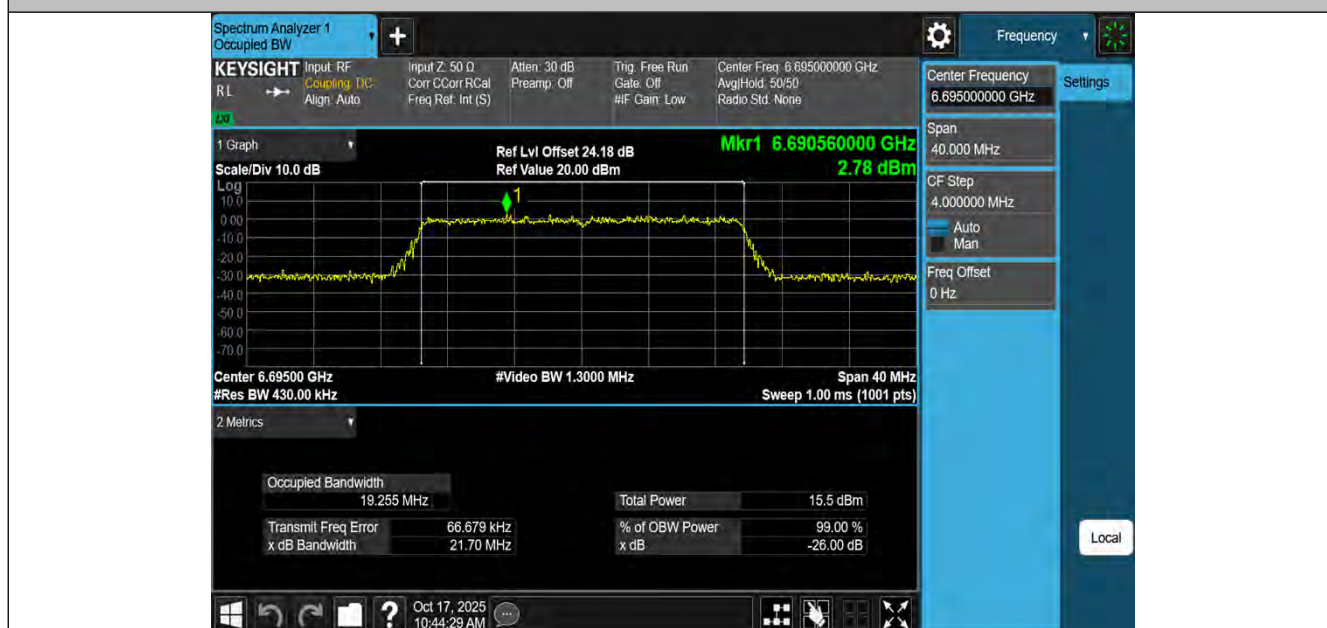
11BE20MIMO-Ant2-6695-PASS
