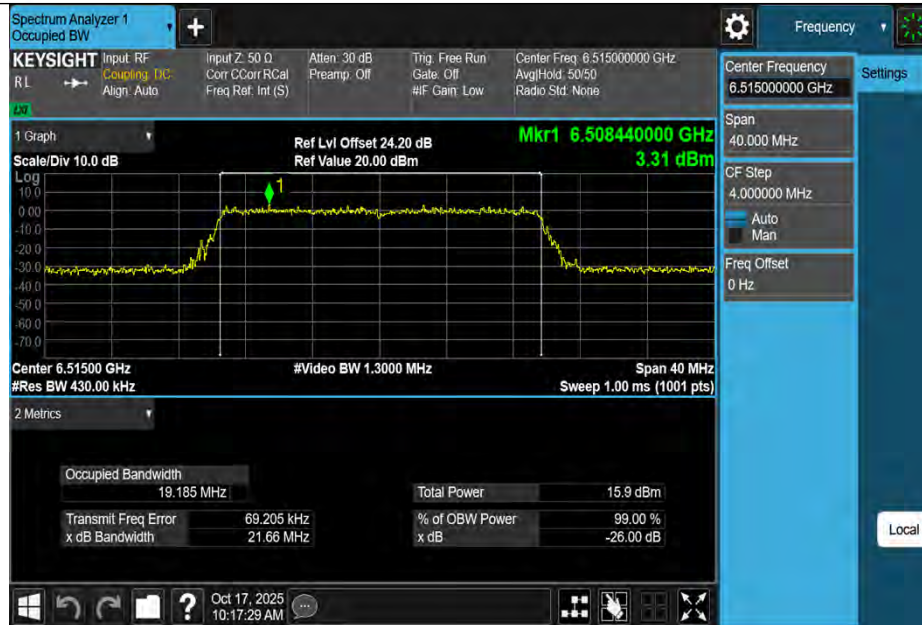
11BE20MIMO-Ant3-6515-PASS
