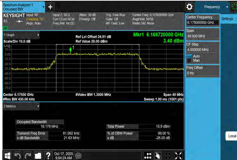
11BE20MIMO-Ant3-6175-PASS
