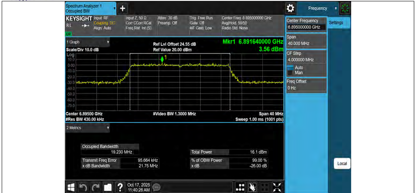
11BE20MIMO-Ant3-6895-PASS
