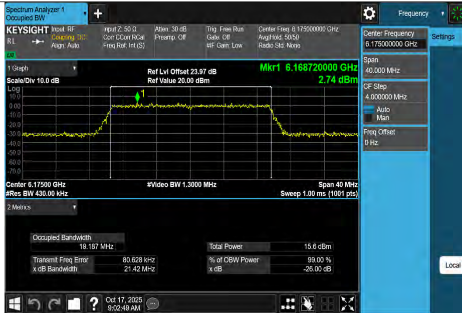
11BE20MIMO-Ant1-6175-PASS
