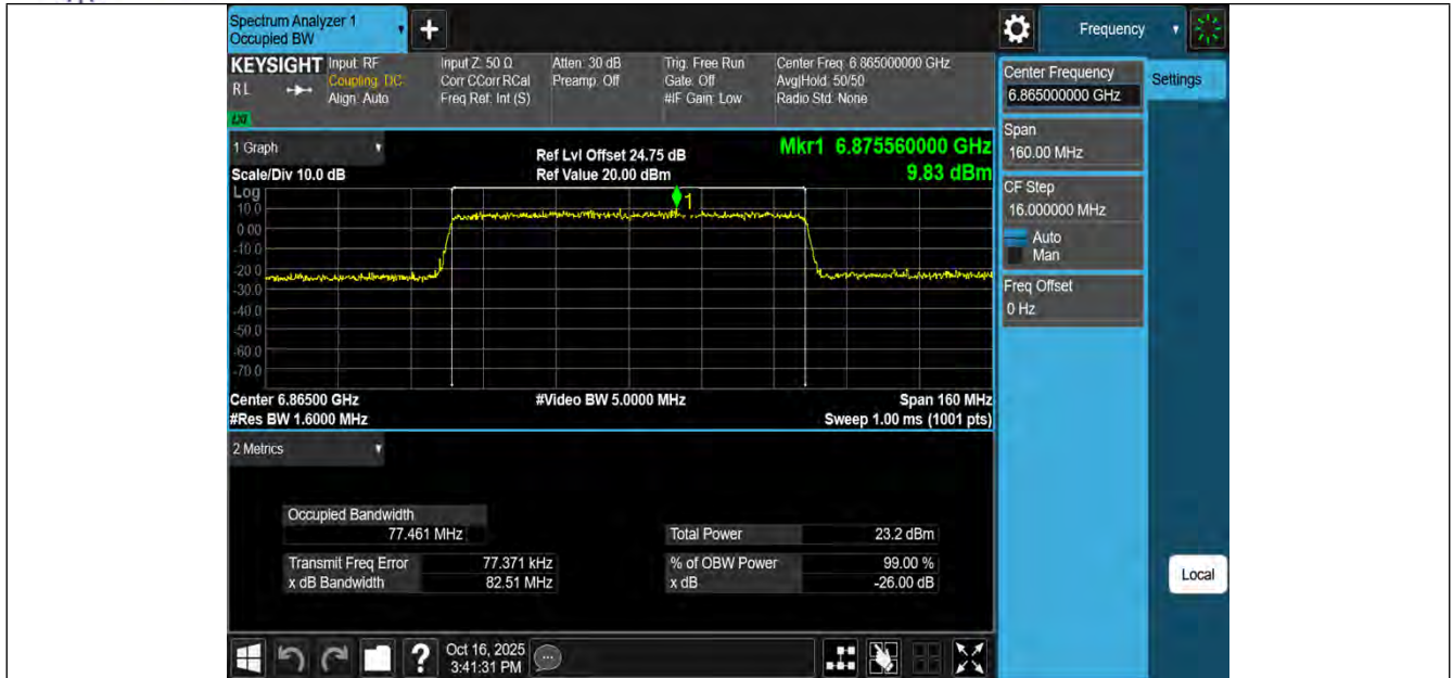
11AX80MIMO-Ant3-6865-PASS
