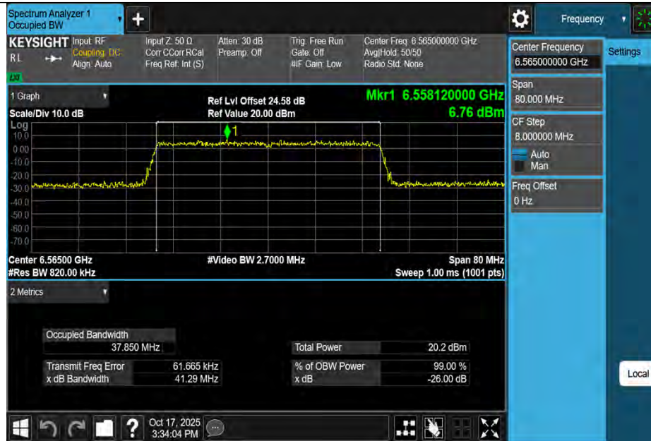
11BE40MIMO-Ant3-6565-PASS
