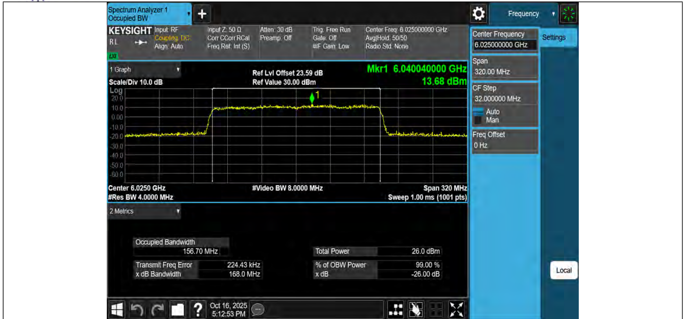
11AX160MIMO-Ant1-6025-PASS
