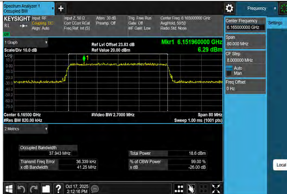
11BE40MIMO-Ant1-6165-PASS
