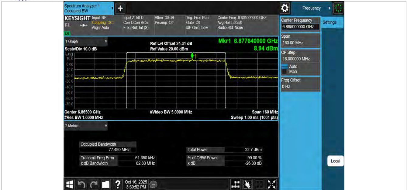
11AX80MIMO-Ant1-6865-PASS
