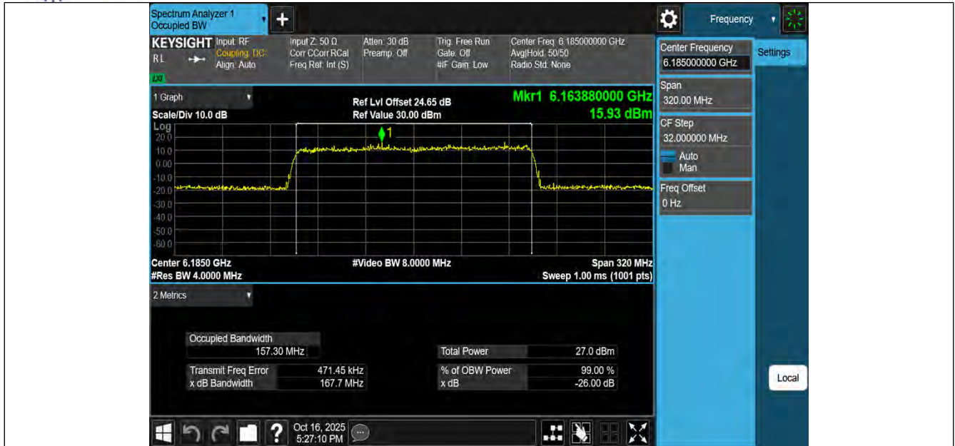
11AX160MIMO-Ant3-6185-PASS
