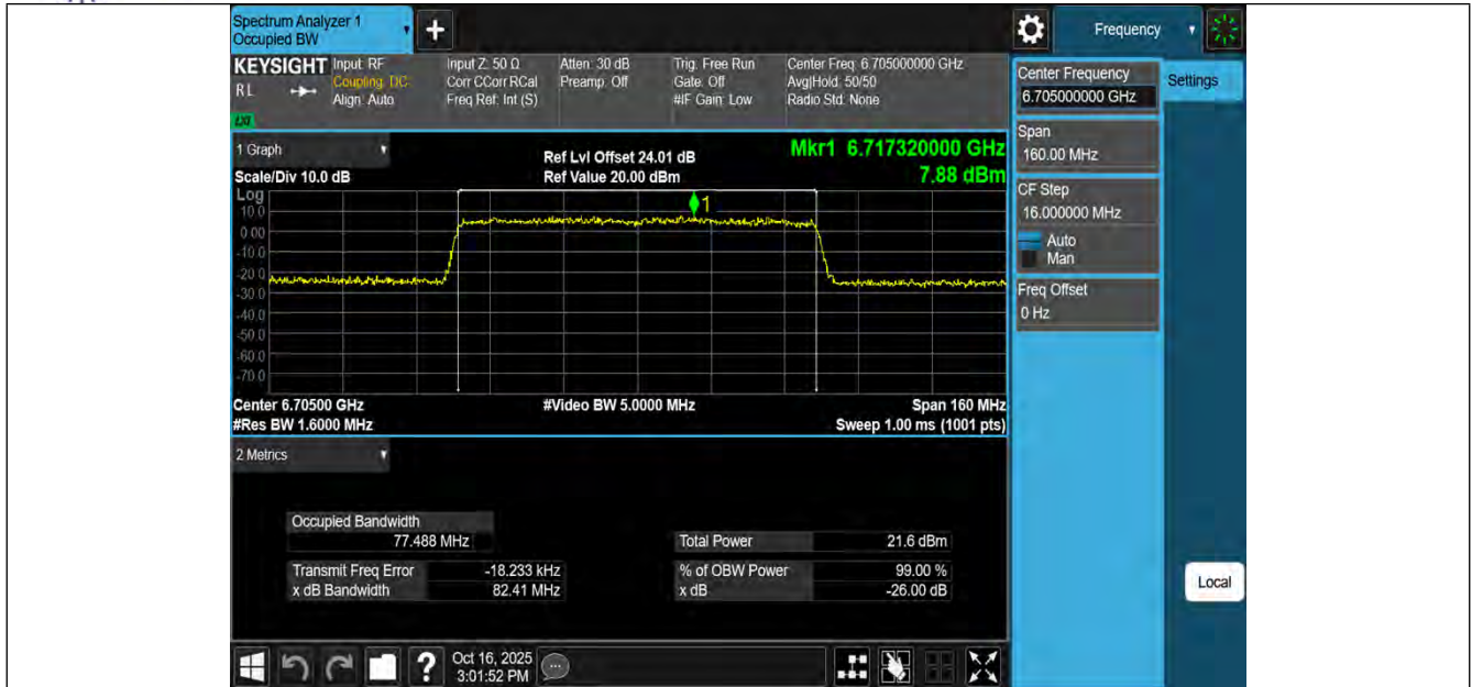
11AX80MIMO-Ant1-6705-PASS
