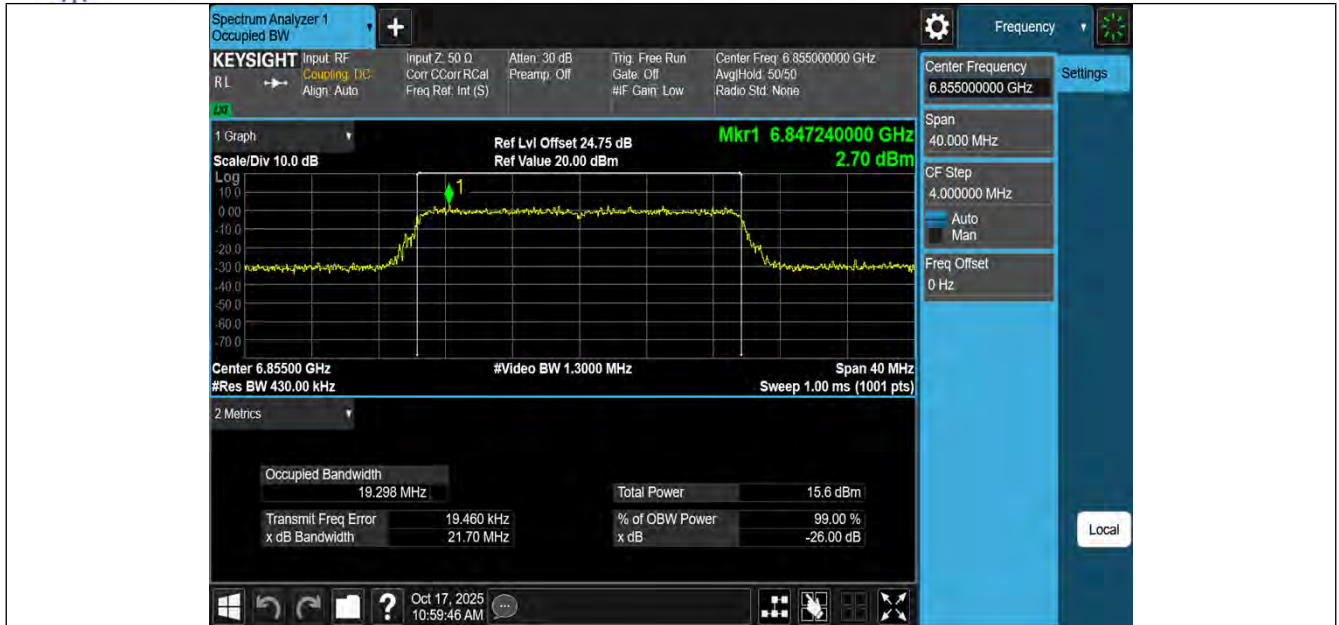
11BE20MIMO-Ant3-6855-PASS
