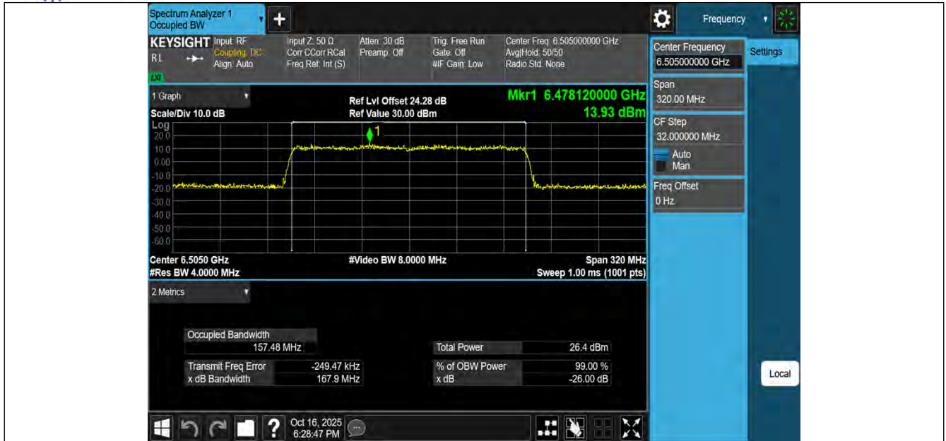
11AX160MIMO-Ant1-6505-PASS
