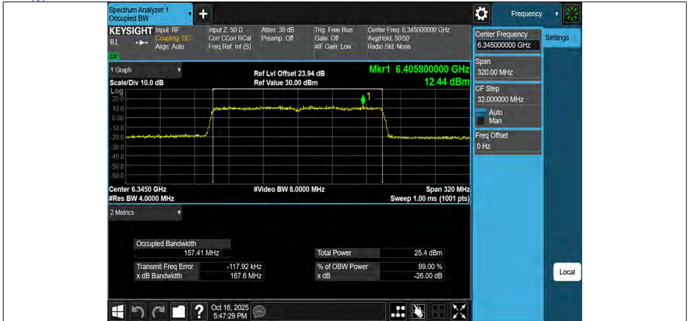
11AX160MIMO-Ant1-6345-PASS
