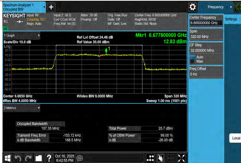
11AX160MIMO-Ant3-6665-PASS
