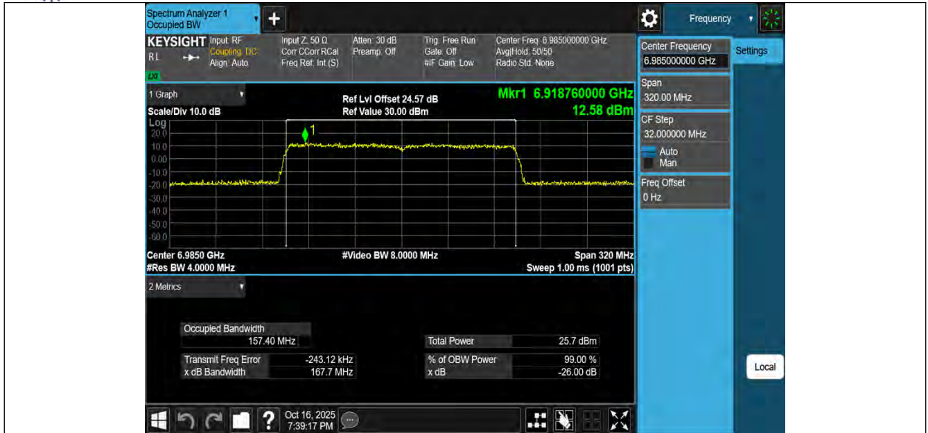
11AX160MIMO-Ant1-6985-PASS
