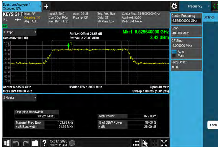
11BE20MIMO-Ant3-6535-PASS
