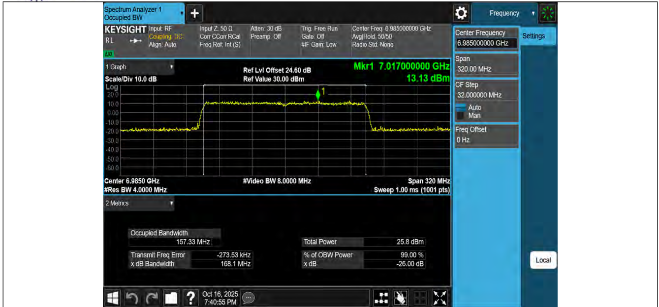
11AX160MIMO-Ant3-6985-PASS
