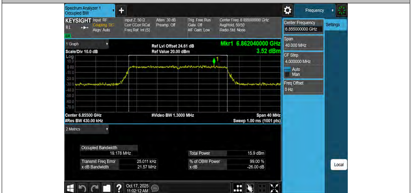
11BE20MIMO-Ant4-6855-PASS
