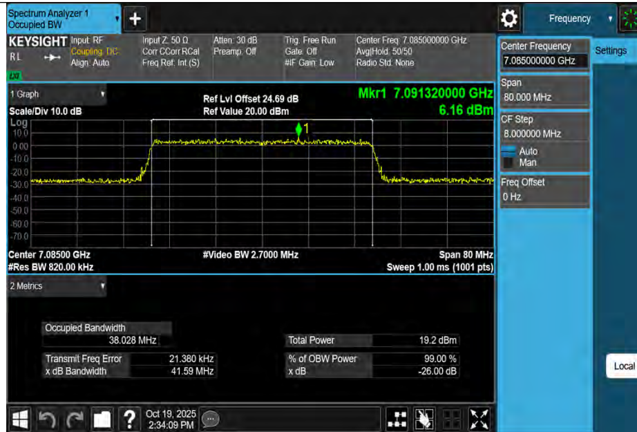
11BE40MIMO-Ant1-7085-PASS
