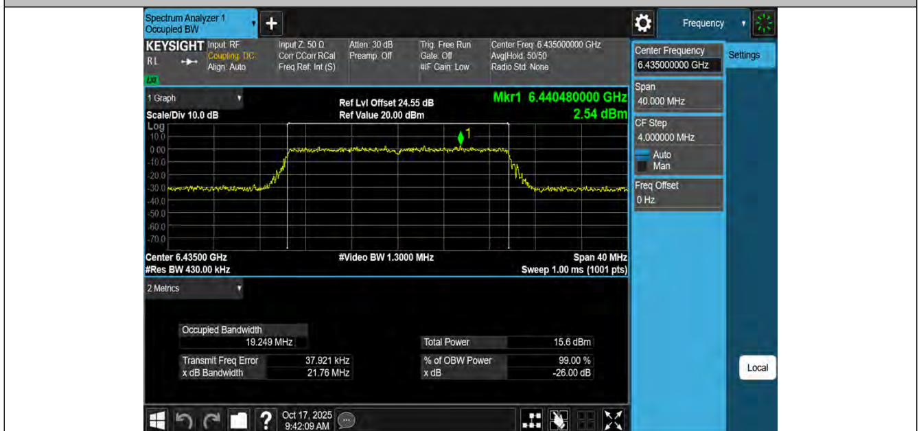
11BE20MIMO-Ant4-6435-PASS
