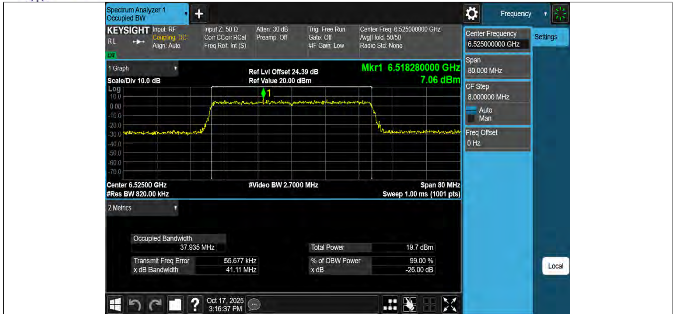
11BE40MIMO-Ant1-6525-PASS
