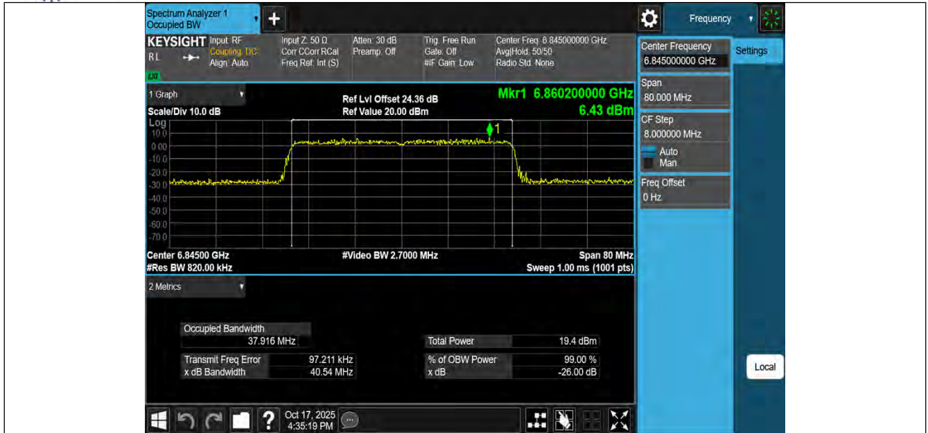
11BE40MIMO-Ant1-6845-PASS
