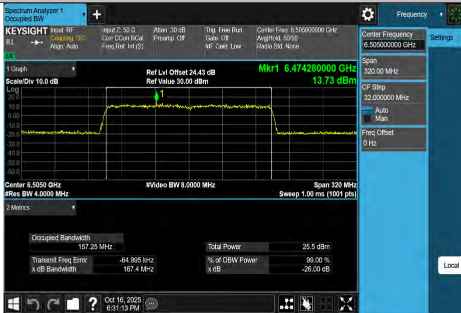
11AX160MIMO-Ant4-6505-PASS
