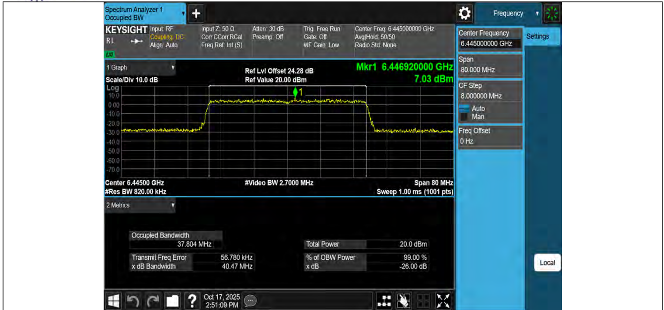
11BE40MIMO-Ant3-6445-PASS
