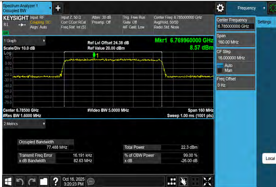
11AX80MIMO-Ant1-6785-PASS
