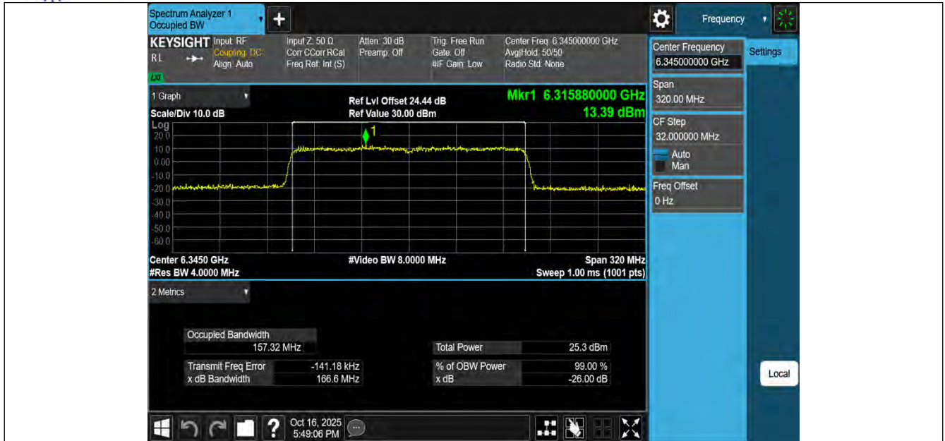
11AX160MIMO-Ant3-6345-PASS
