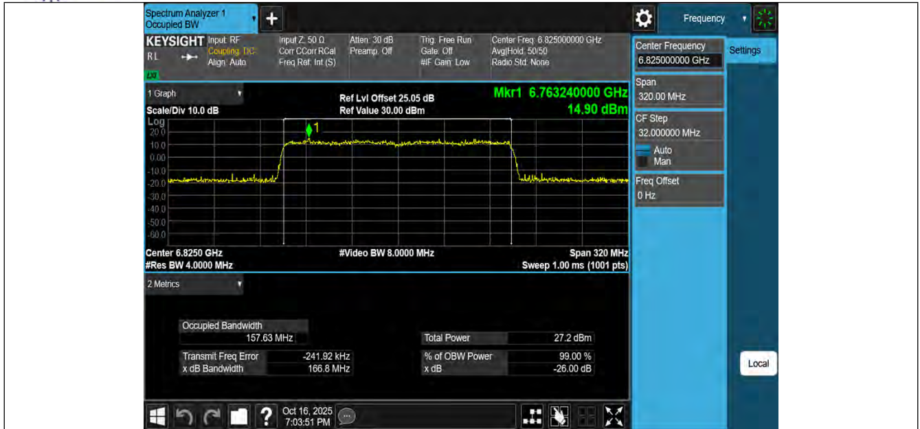
11AX160MIMO-Ant3-6825-PASS
