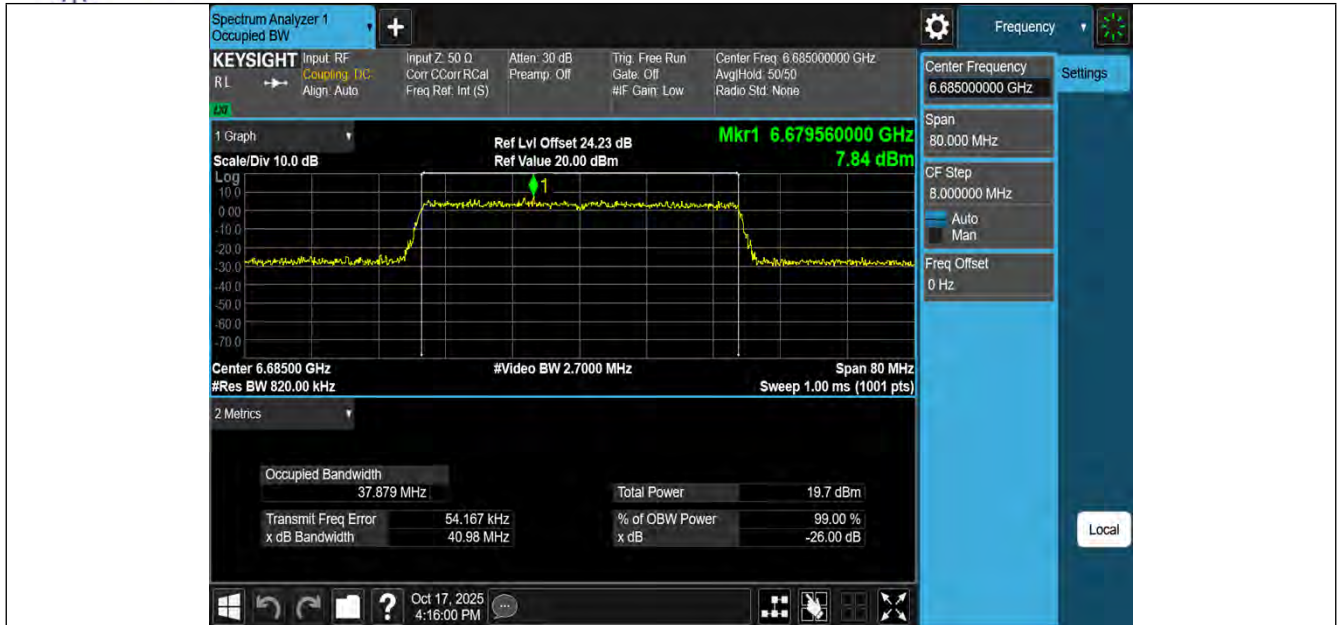
11BE40MIMO-Ant3-6685-PASS
