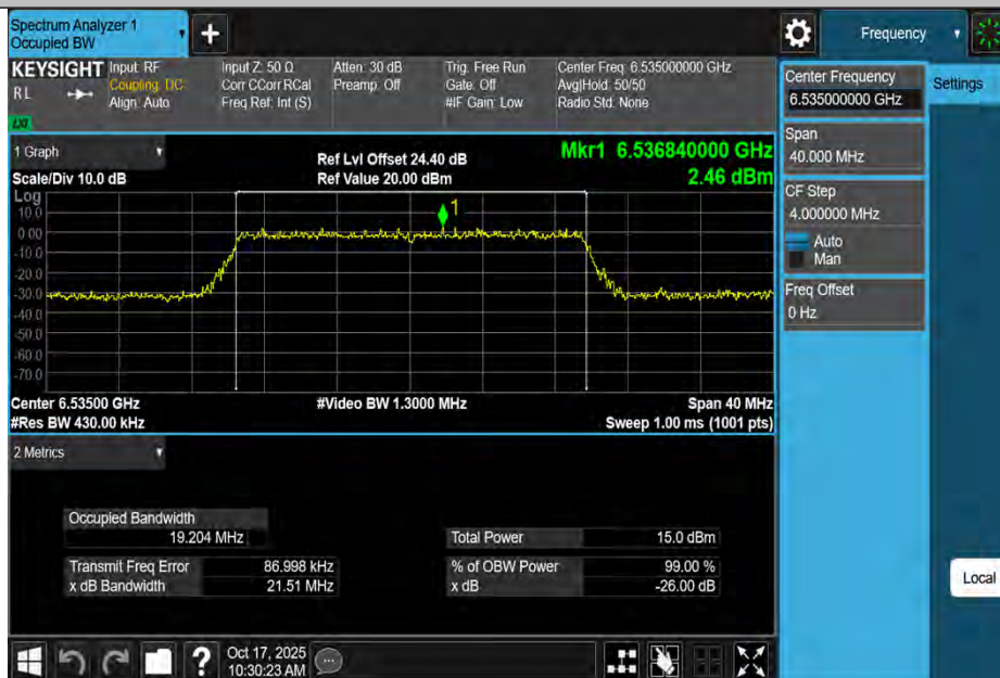
11BE20MIMO-Ant2-6535-PASS
