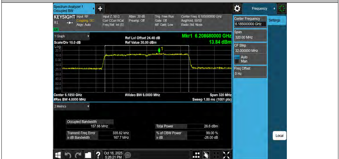
11AX160MIMO-Ant2-6185-PASS
