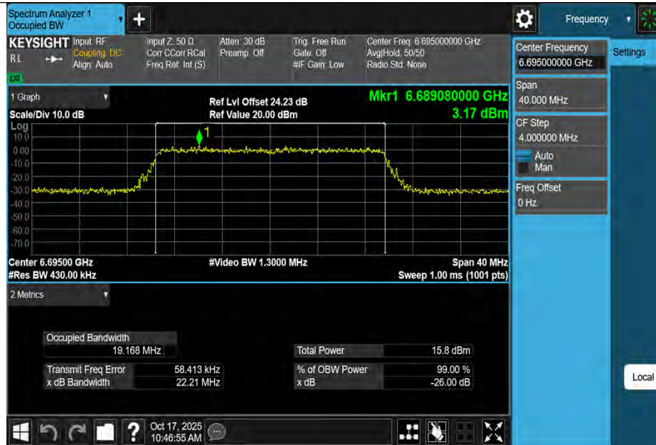
11BE20MIMO-Ant3-6695-PASS
