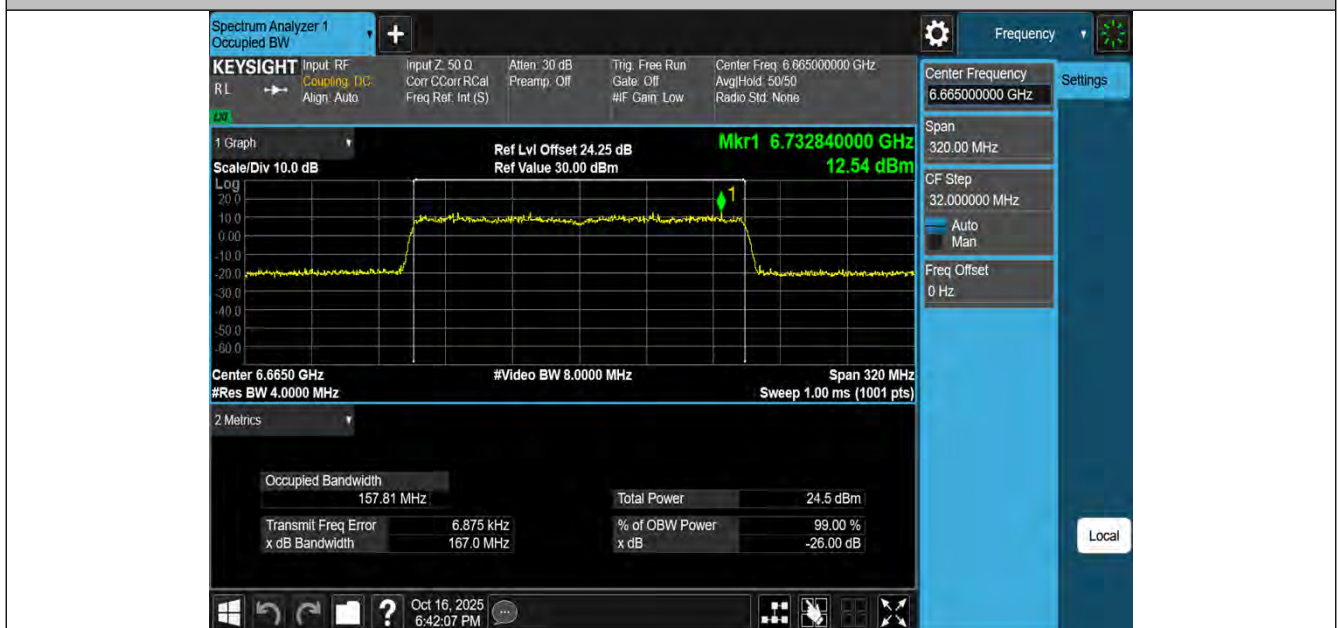
11AX160MIMO-Ant2-6665-PASS
