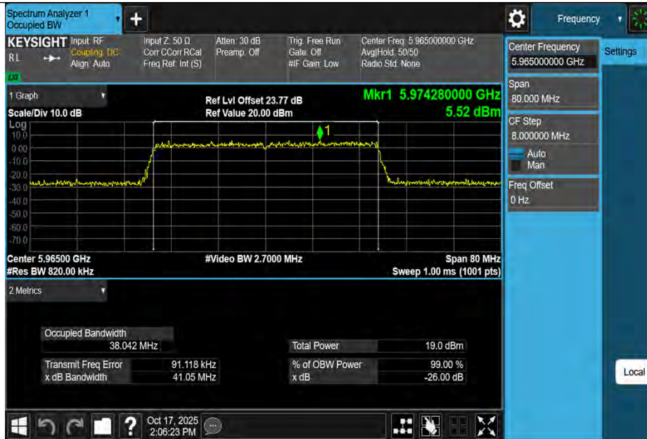
11BE40MIMO-Ant3-5965-PASS
