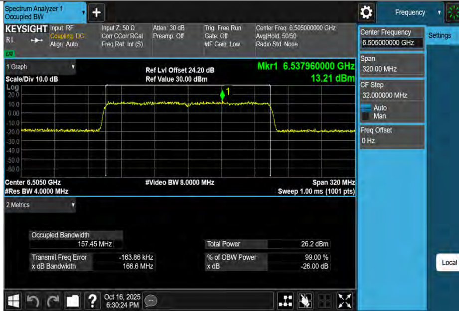
11AX160MIMO-Ant3-6505-PASS
