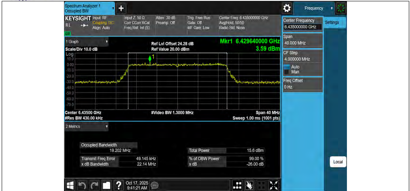
11BE20MIMO-Ant3-6435-PASS
