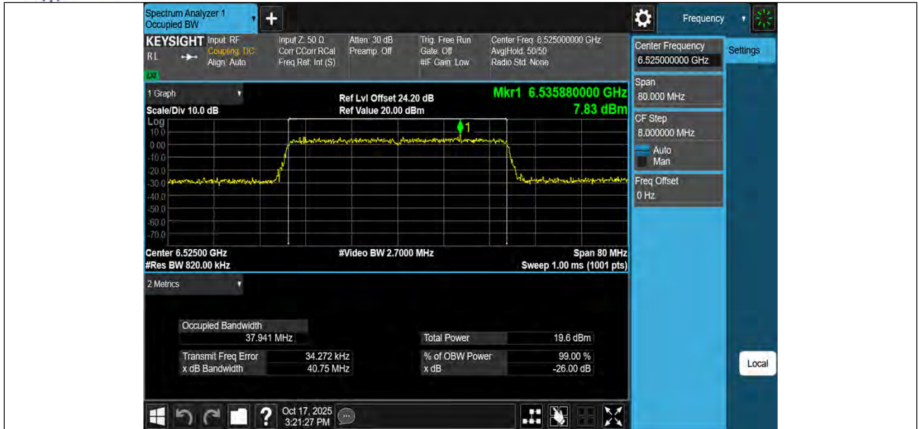
11BE40MIMO-Ant3-6525-PASS
