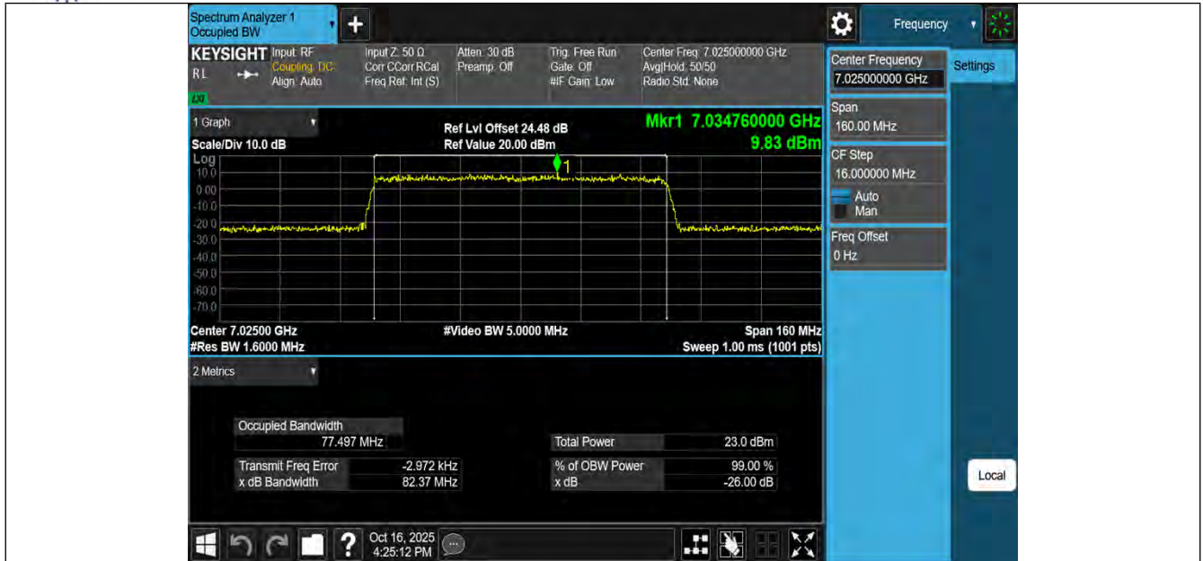
11AX80MIMO-Ant1-7025-PASS
