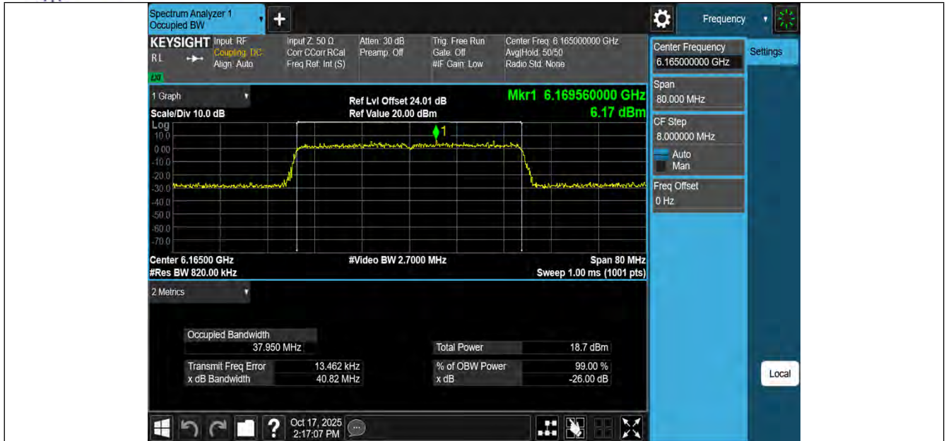
11BE40MIMO-Ant3-6165-PASS
