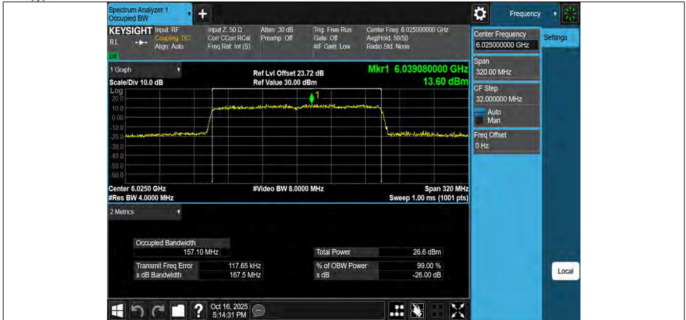
11AX160MIMO-Ant3-6025-PASS
