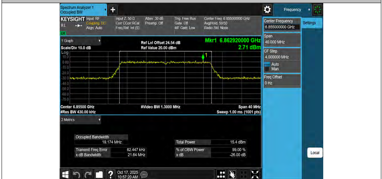
11BE20MIMO-Ant2-6855-PASS
