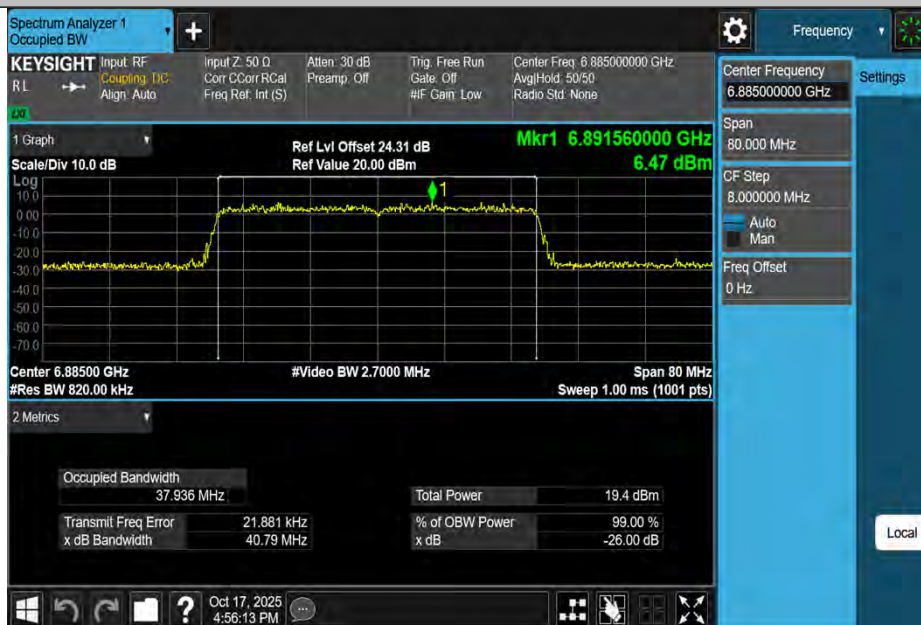
11BE40MIMO-Ant2-6885-PASS
