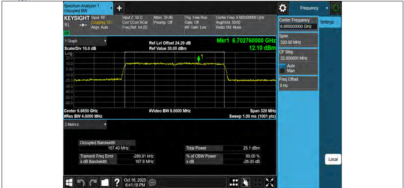
11AX160MIMO-Ant1-6665-PASS
