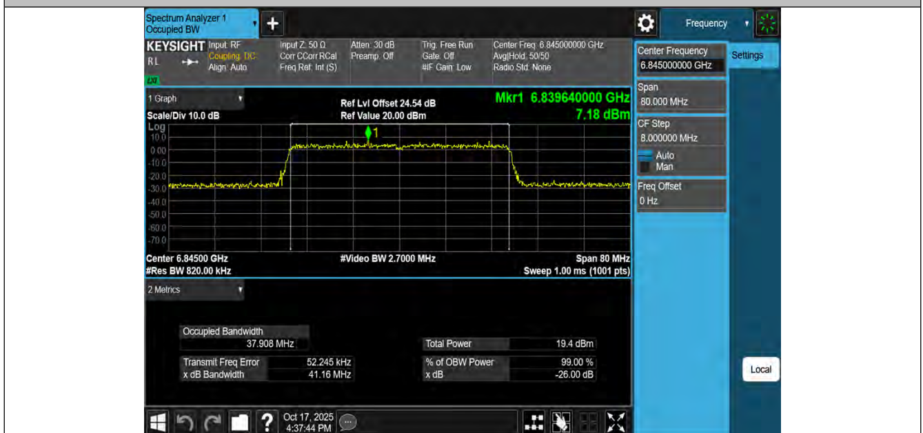
11BE40MIMO-Ant2-6845-PASS
