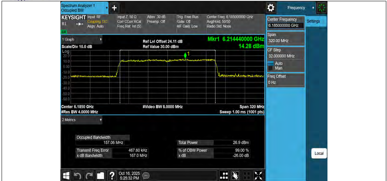
11AX160MIMO-Ant1-6185-PASS
