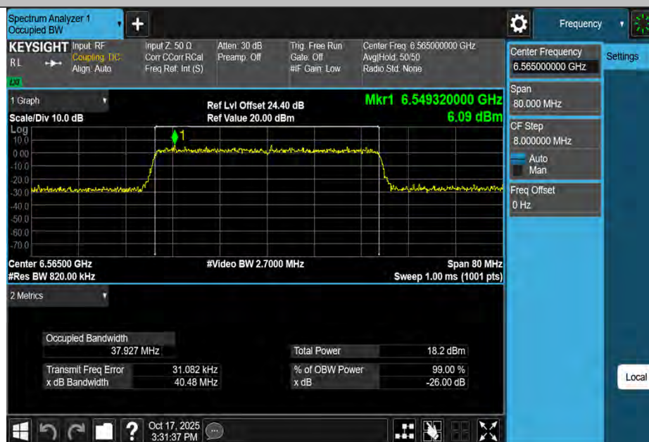
11BE40MIMO-Ant2-6565-PASS
