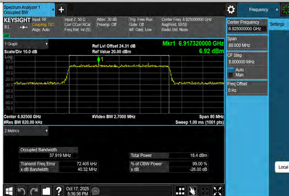
11BE40MIMO-Ant2-6925-PASS
