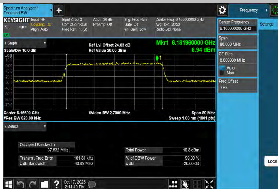
11BE40MIMO-Ant2-6165-PASS
