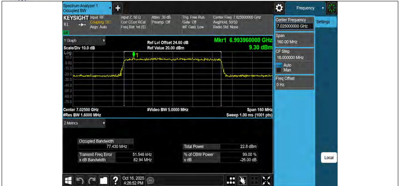
11AX80MIMO-Ant3-7025-PASS
