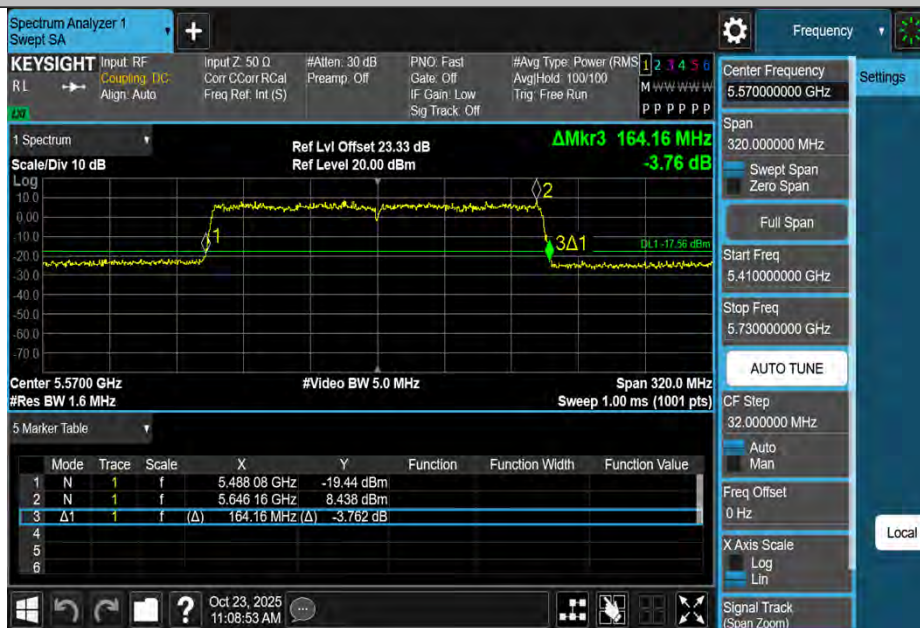
11BE160MIMO-Ant2-5570
