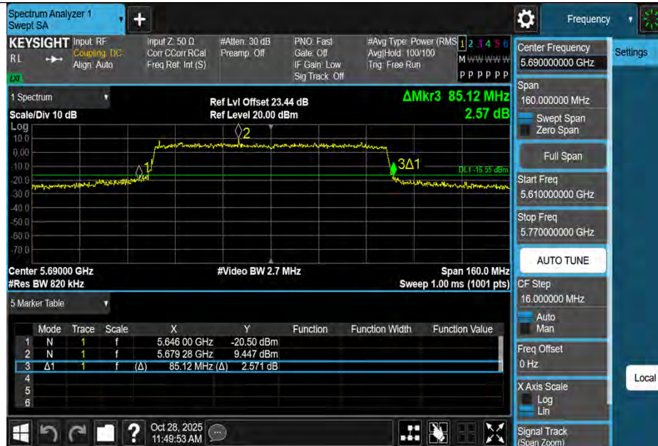
11BE80MIMO-Ant1-5690
