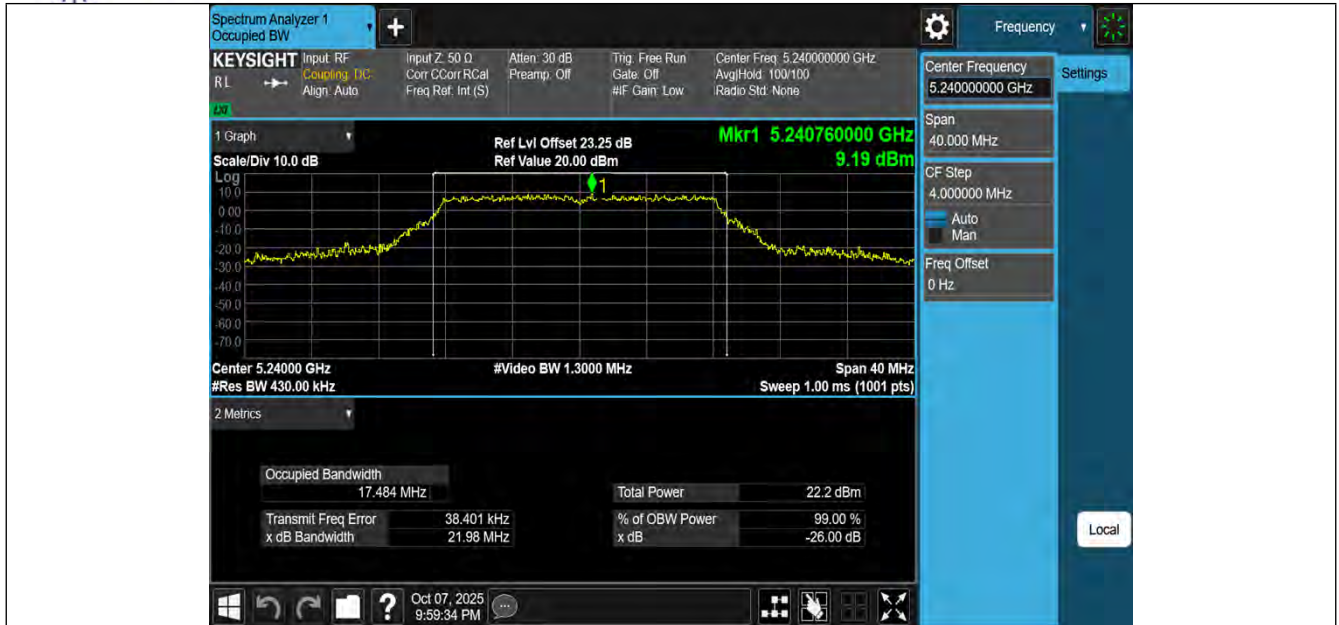
11A-Ant3-5240
