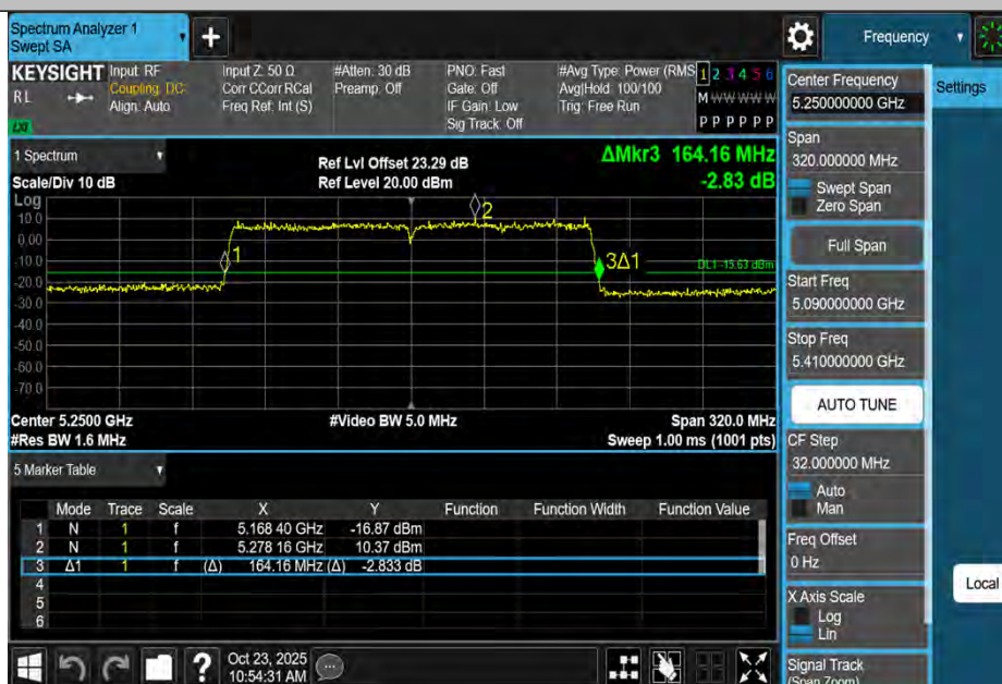
11BE160MIMO-Ant4-5250
