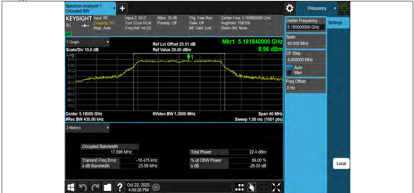
11A-Ant3-5180
