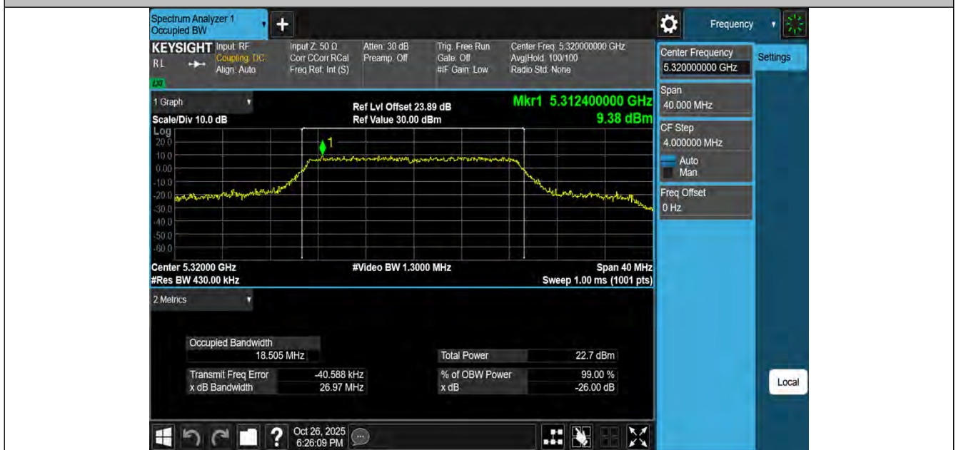
11N20MIMO-Ant4-5320
