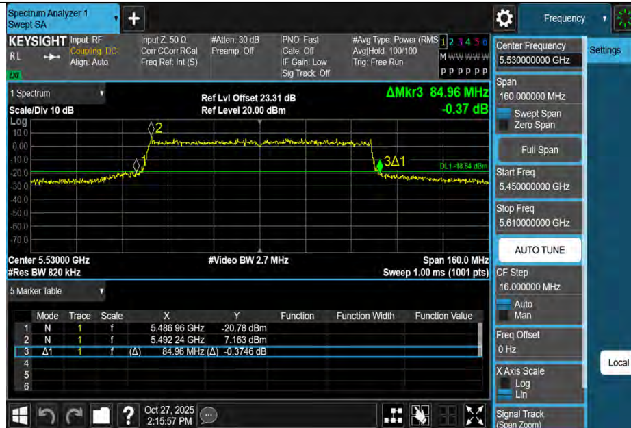
11BE80MIMO-Ant2-5530
