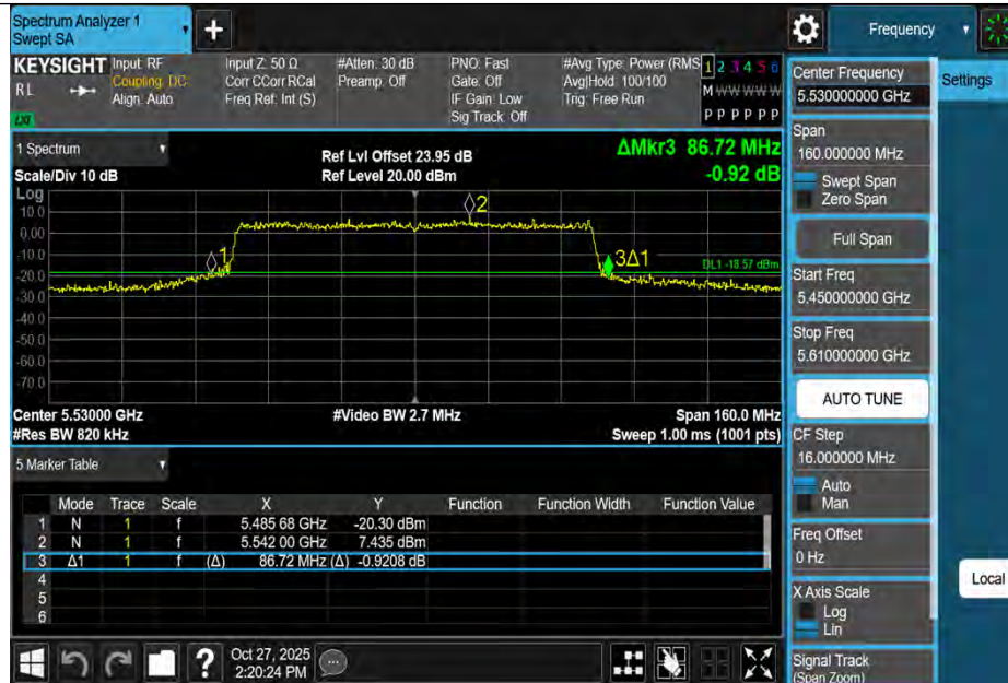
11BE80MIMO-Ant4-5530
