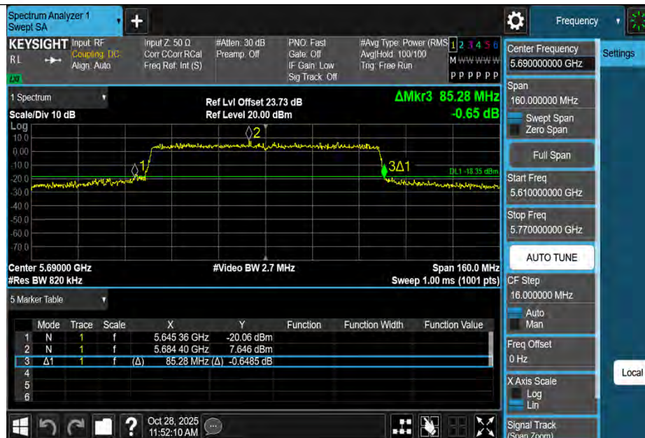
11BE80MIMO-Ant3-5690
