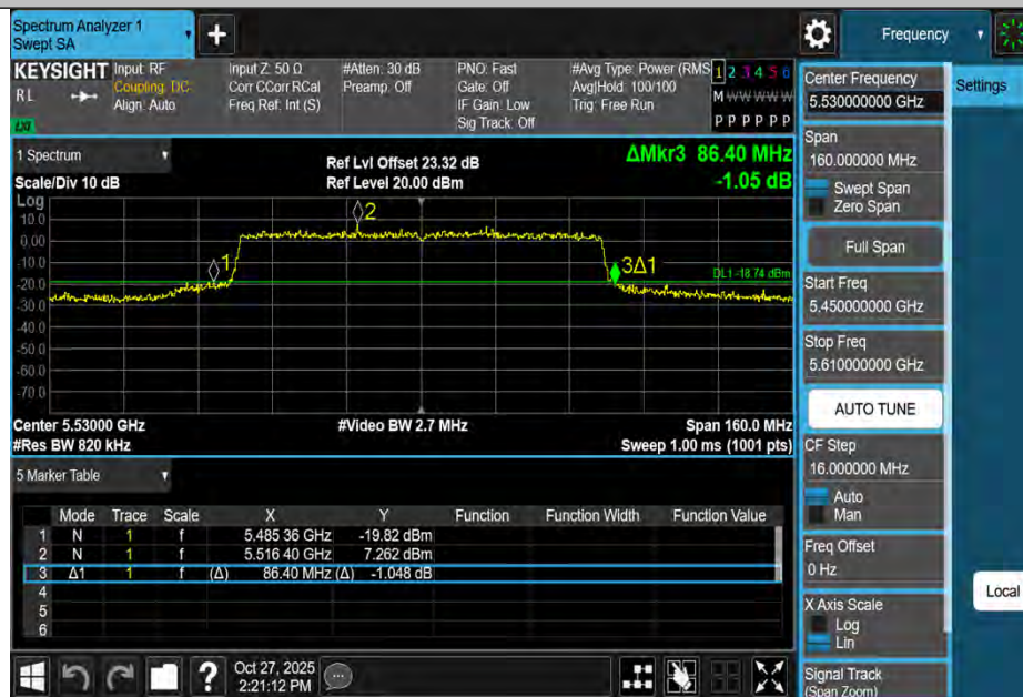
11BE80MIMO-Ant1-5530
