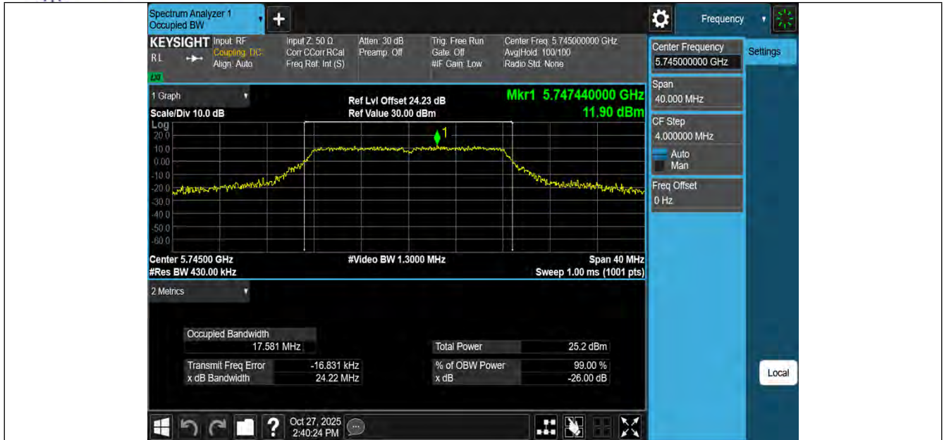
11A-Ant3-5745
