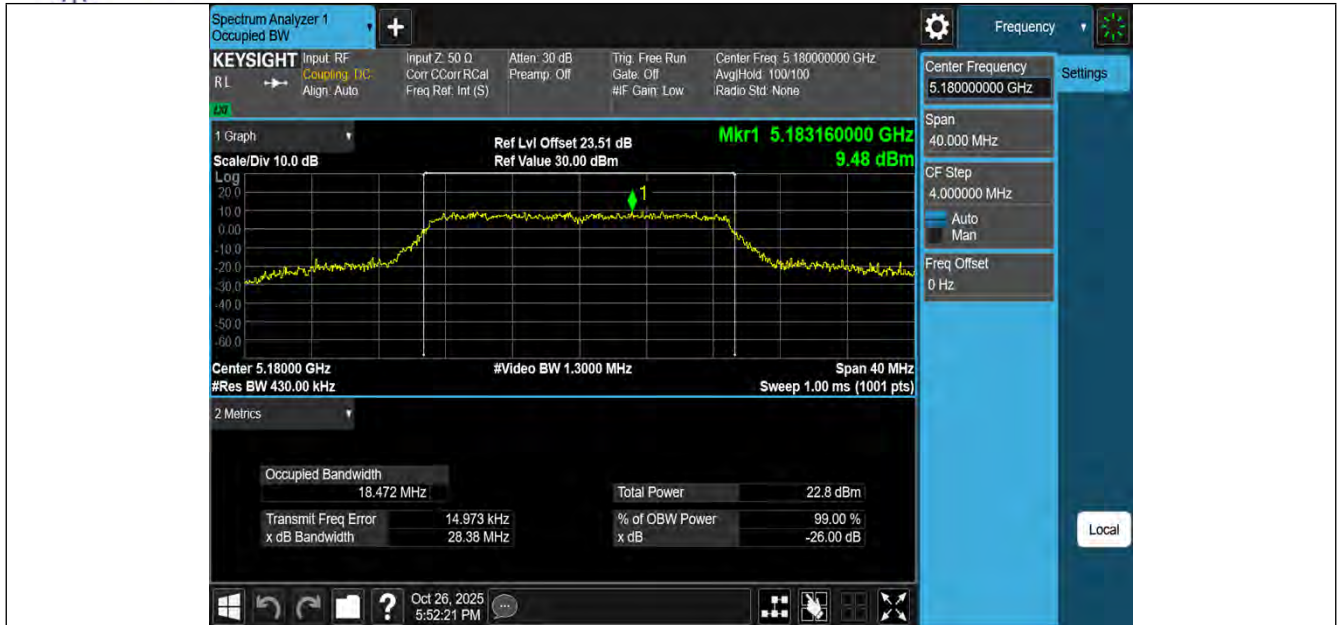
11N20MIMO-Ant3-5180
