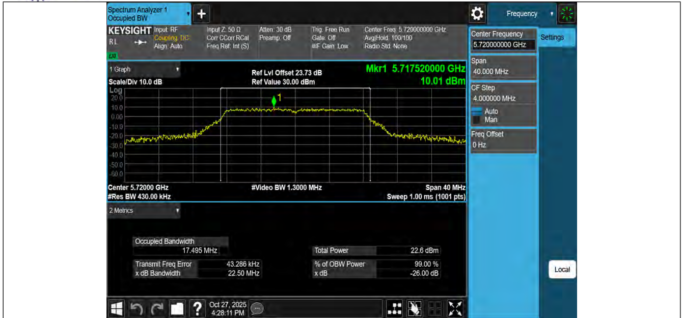
11A-Ant3-5720
