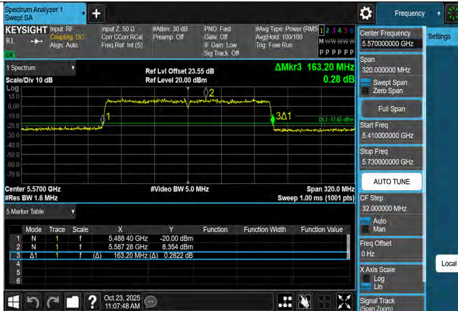
11BE160MIMO-Ant1-5570
