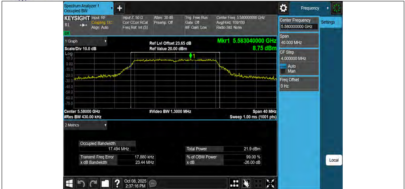
11A-Ant3-5580
