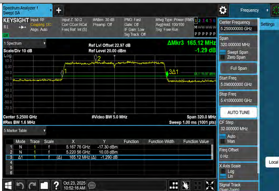
11BE160MIMO-Ant2-5250
