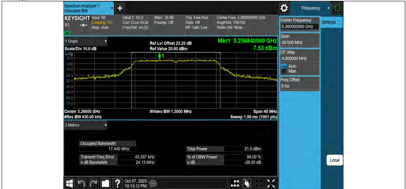
11A-Ant3-5260
