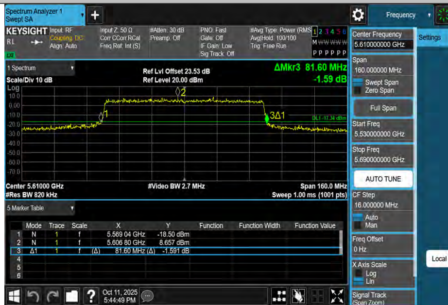
11BE80MIMO-Ant3-5610
