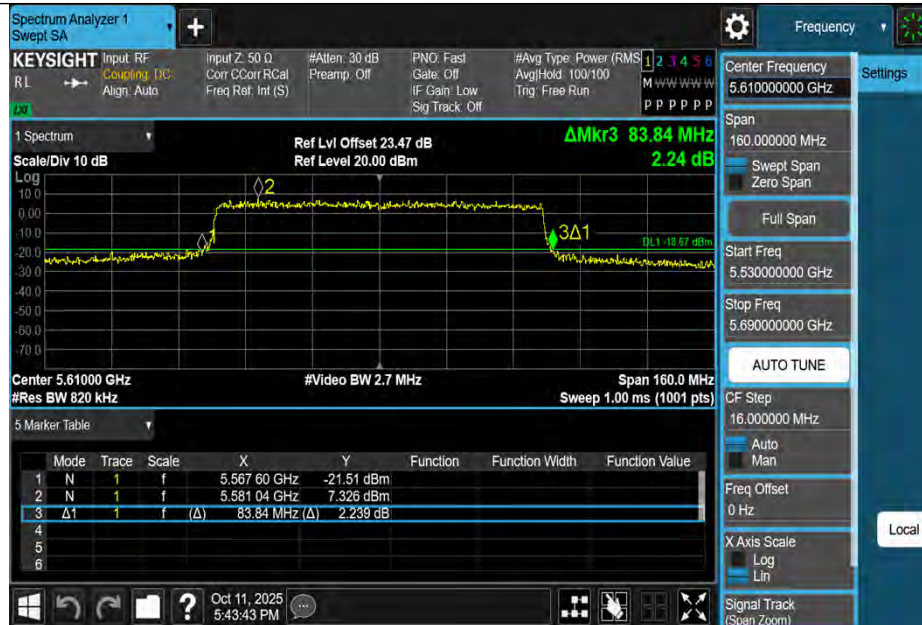
11BE80MIMO-Ant2-5610
