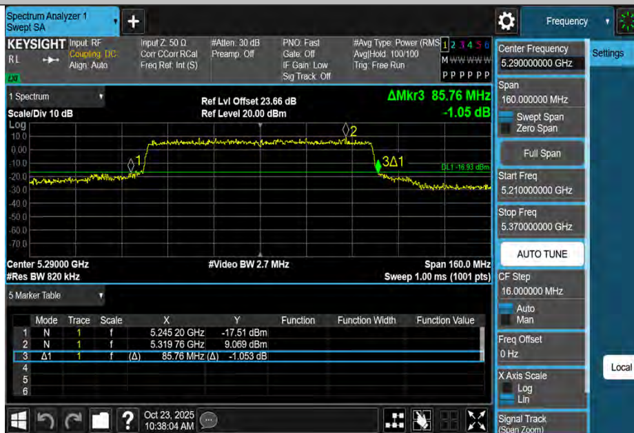
11BE80MIMO-Ant2-5290
