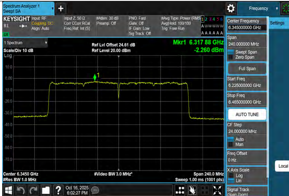
11AX160MIMO-Ant1-6345-PASS
