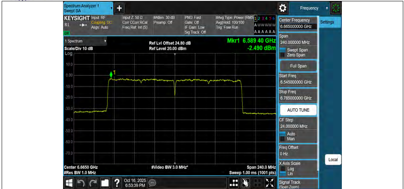
11AX160MIMO-Ant1-6665-PASS
