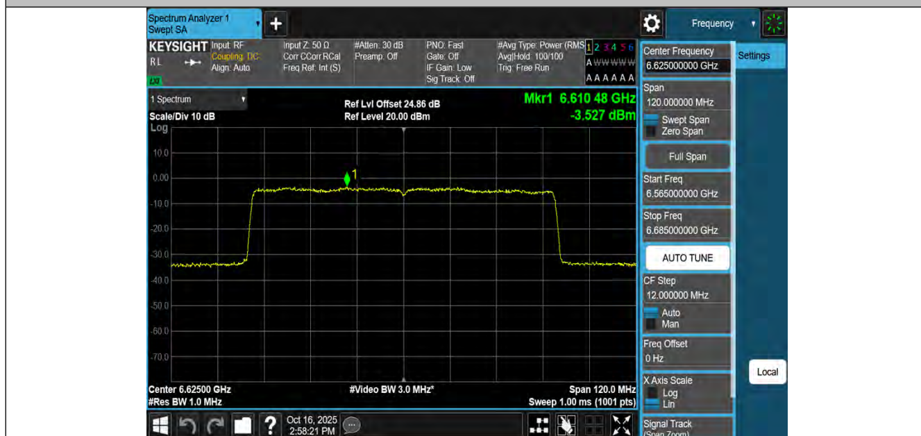
11AX80MIMO-Ant2-6625-PASS
