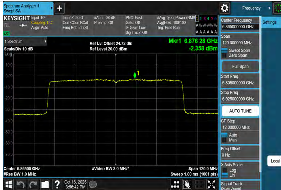
11AX80MIMO-Ant1-6865-PASS
