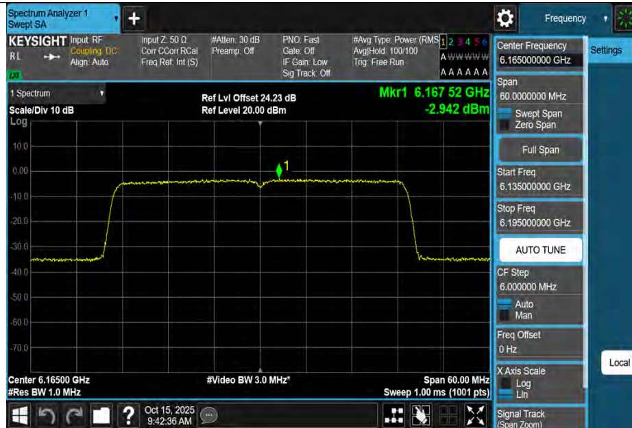
11AX40MIMO-Ant3-6165-PASS
