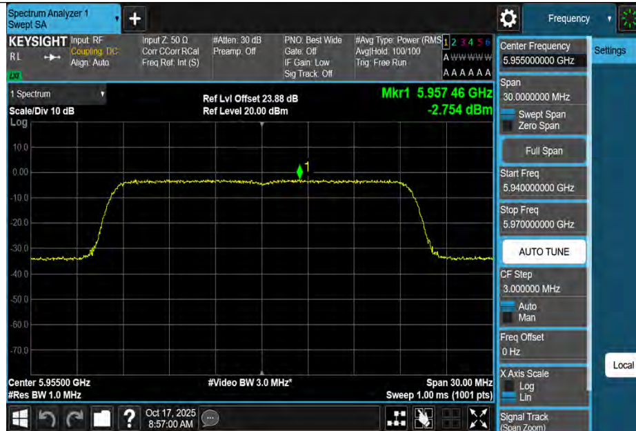
11BE20MIMO-Ant3-5955-PASS
