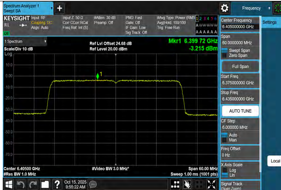
11AX40MIMO-Ant1-6405-PASS
