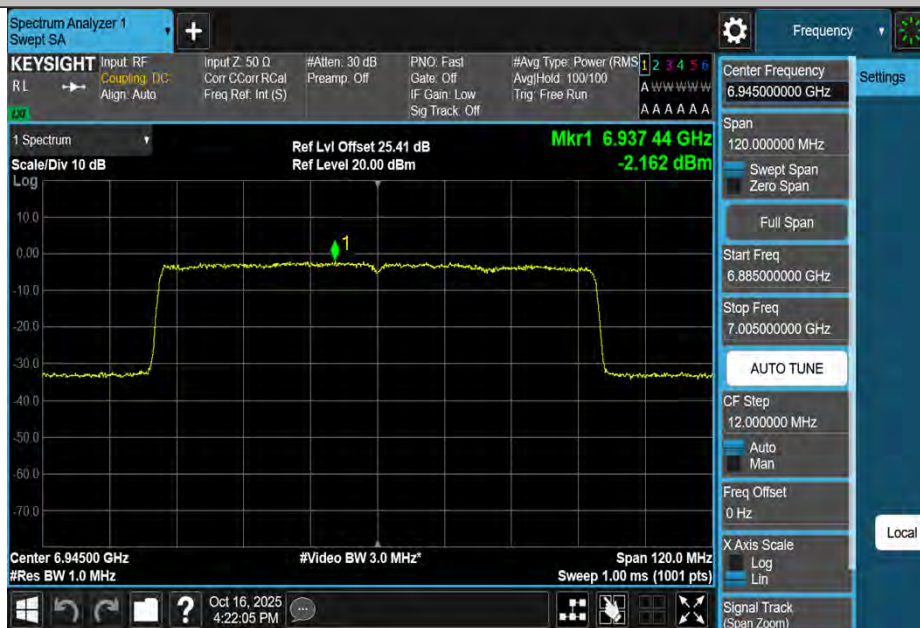
11AX80MIMO-Ant4-6945-PASS
