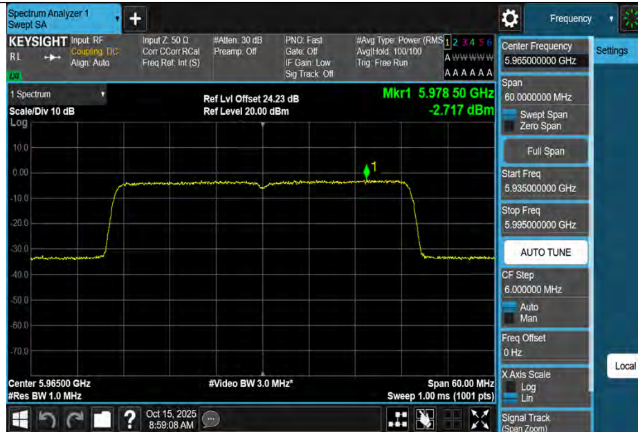
11AX40MIMO-Ant1-5965-PASS
