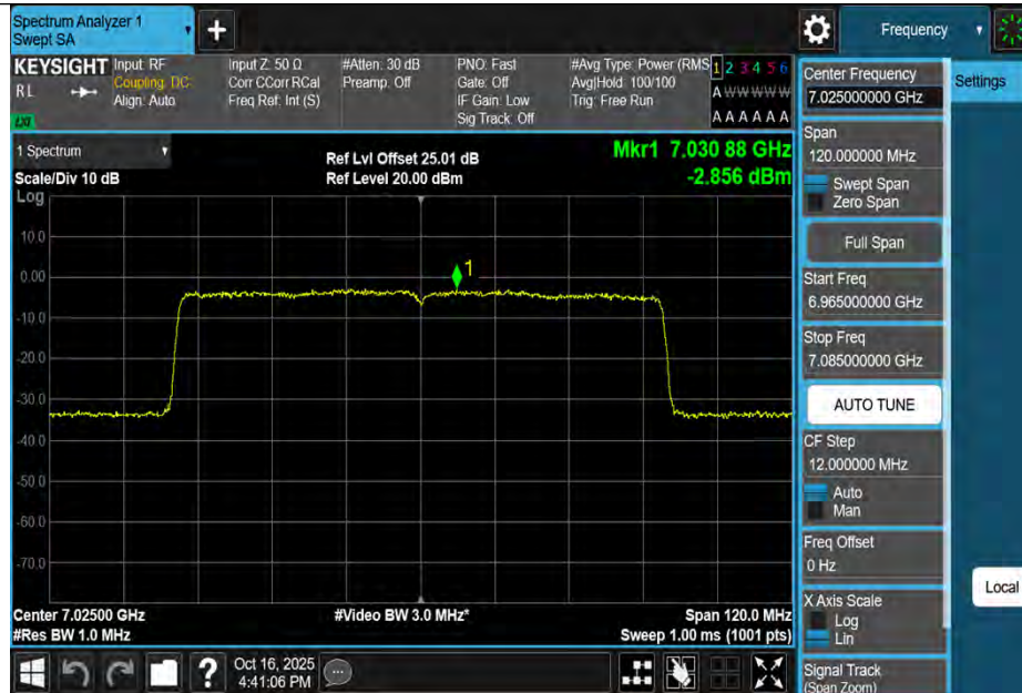
11AX80MIMO-Ant3-7025-PASS
