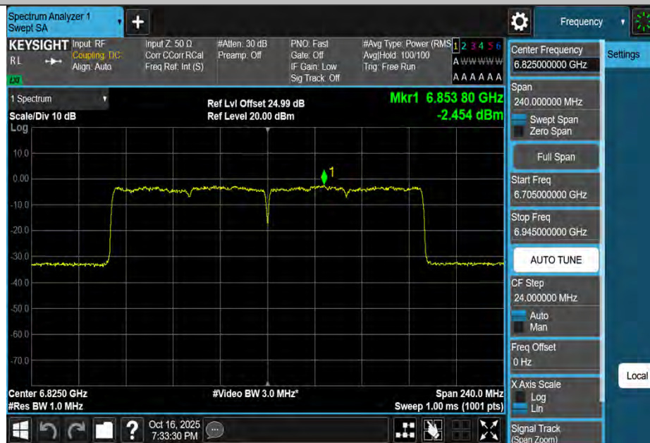
11AX160MIMO-Ant2-6825-PASS
