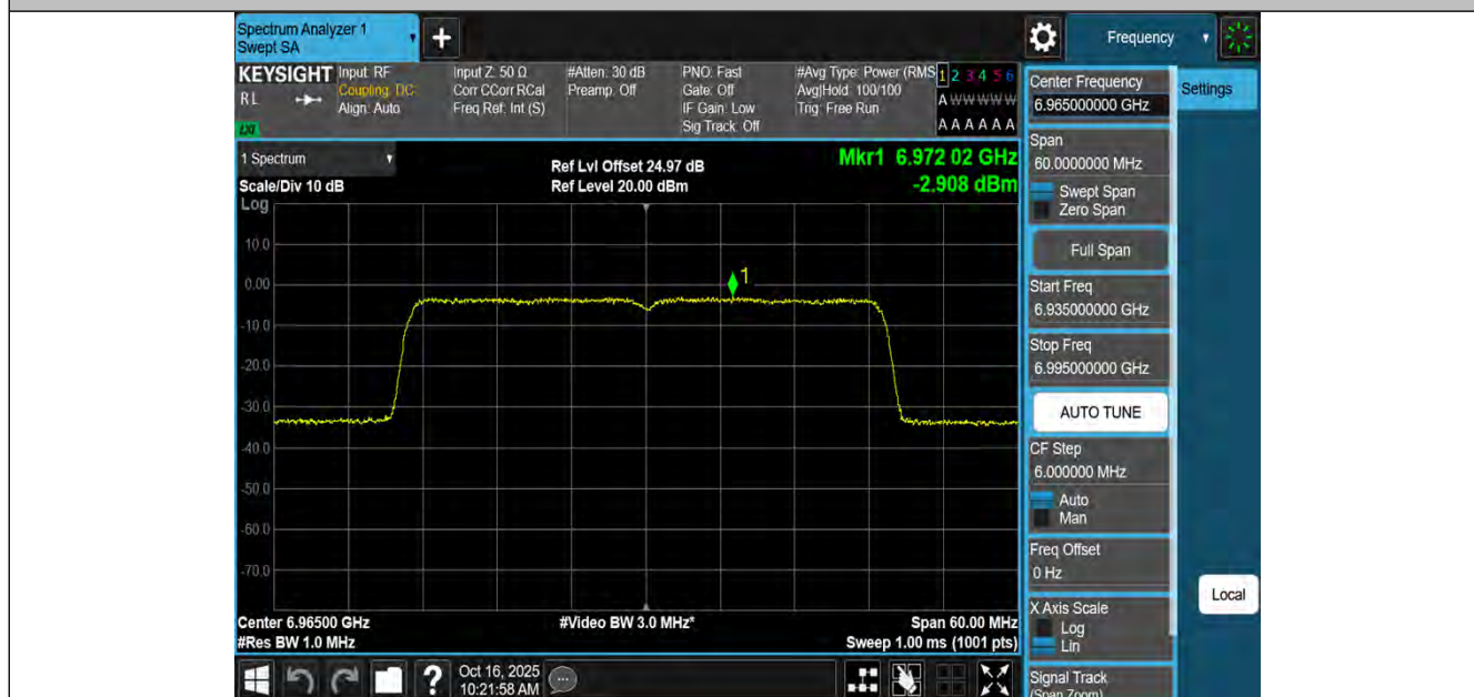
11AX40MIMO-Ant2-6965-PASS
