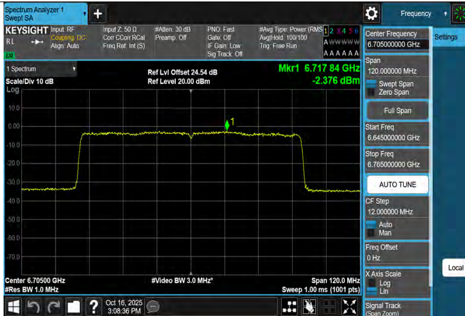
11AX80MIMO-Ant3-6705-PASS
