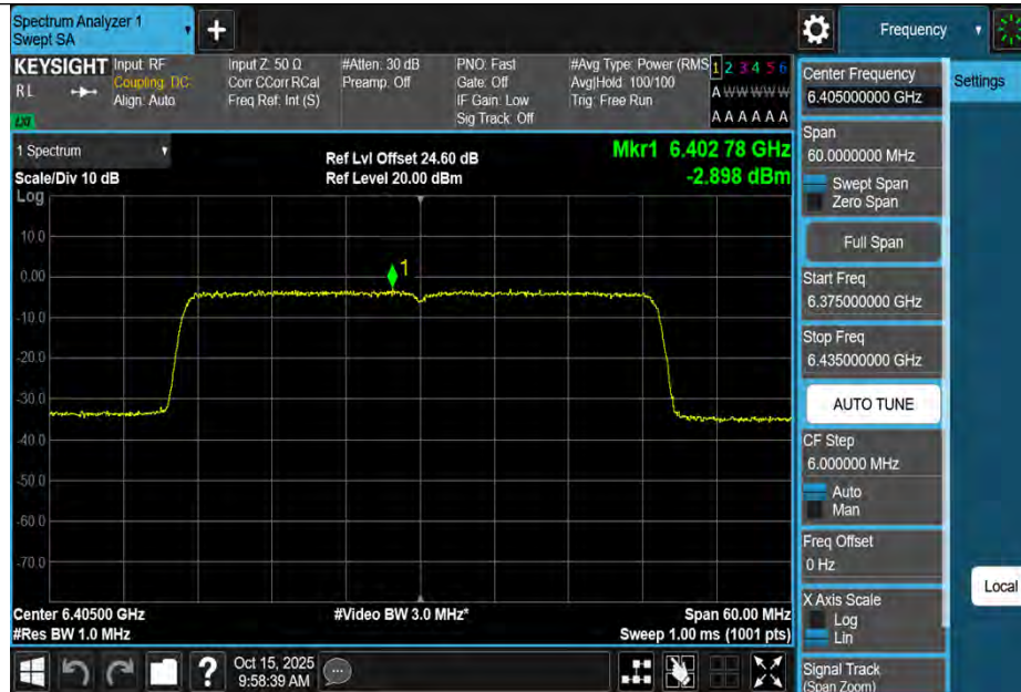
11AX40MIMO-Ant3-6405-PASS
