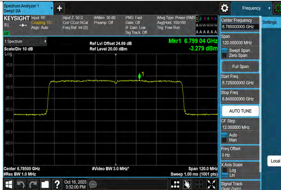
11AX80MIMO-Ant1-6785-PASS
