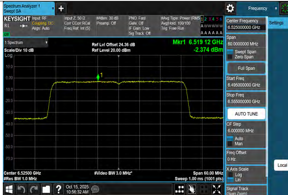
11AX40MIMO-Ant3-6525-PASS
