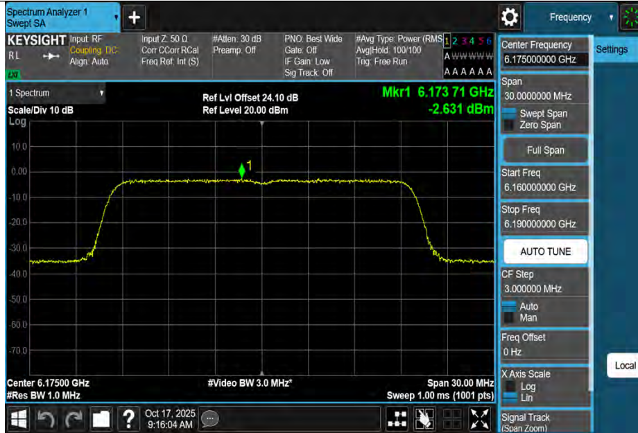
11BE20MIMO-Ant3-6175-PASS
