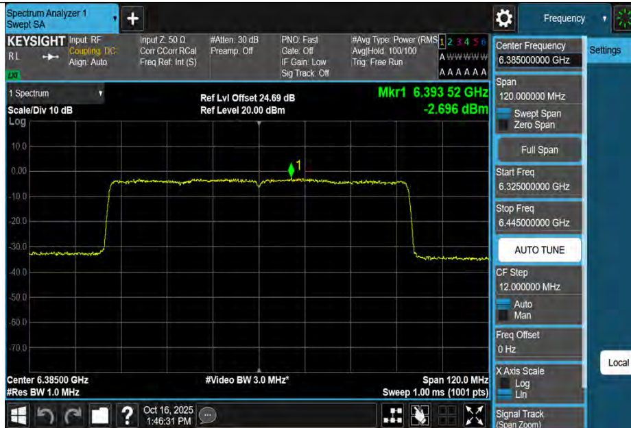
11AX80MIMO-Ant3-6385-PASS
