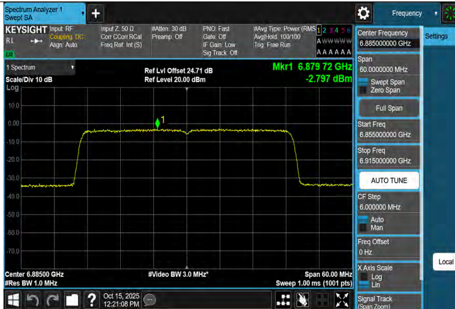
11AX40MIMO-Ant3-6885-PASS
