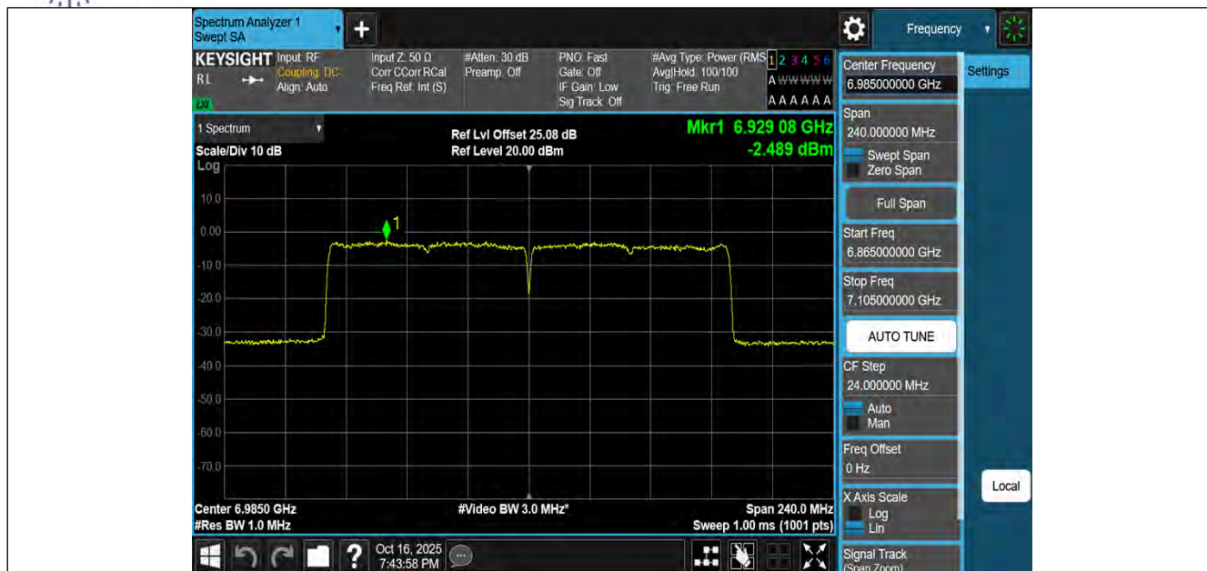
11AX160MIMO-Ant1-6985-PASS
