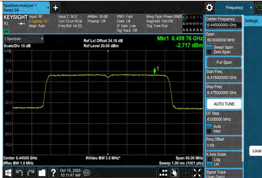
11AX40MIMO-Ant1-6445-PASS
