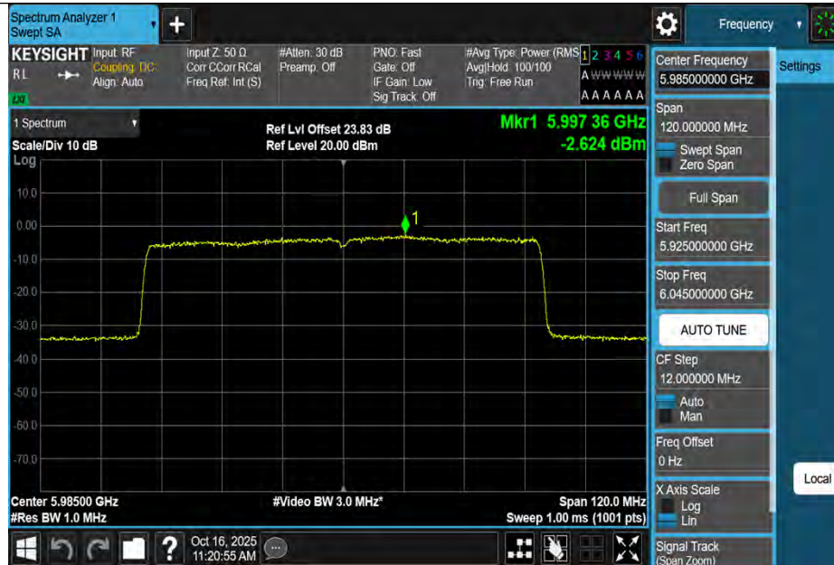
11AX80MIMO-Ant1-5985-PASS
