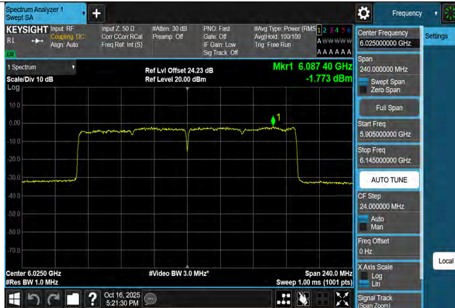
11AX160MIMO-Ant3-6025-PASS
