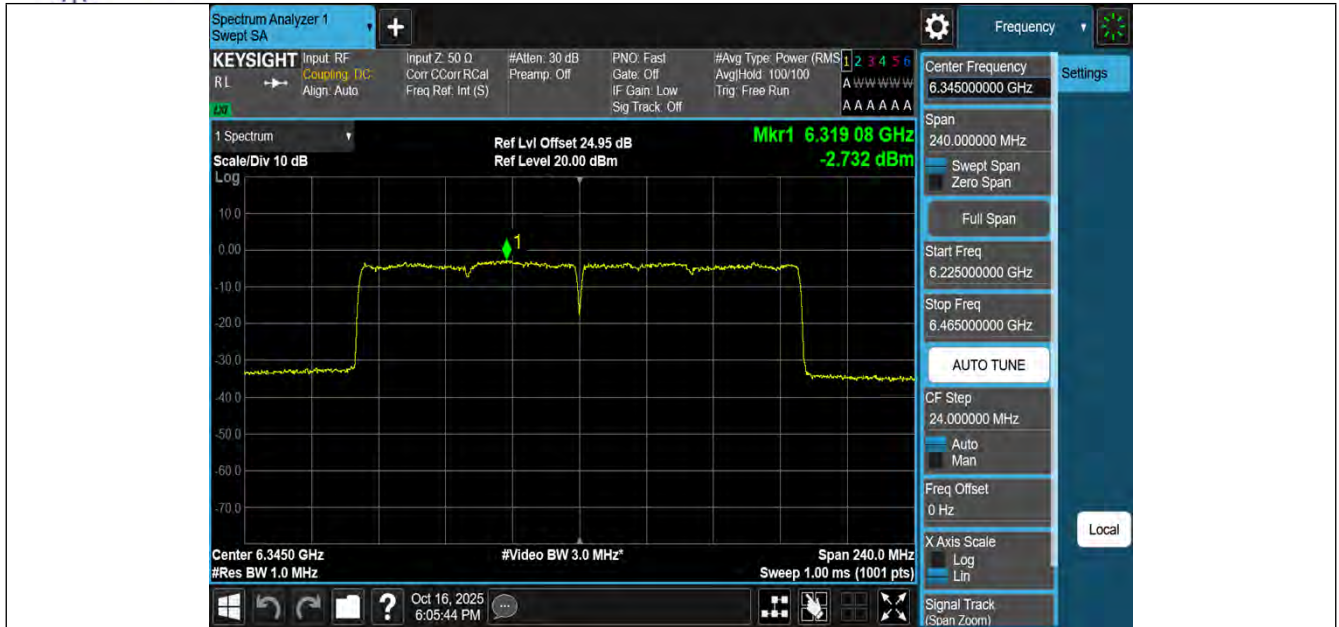
11AX160MIMO-Ant3-6345-PASS
