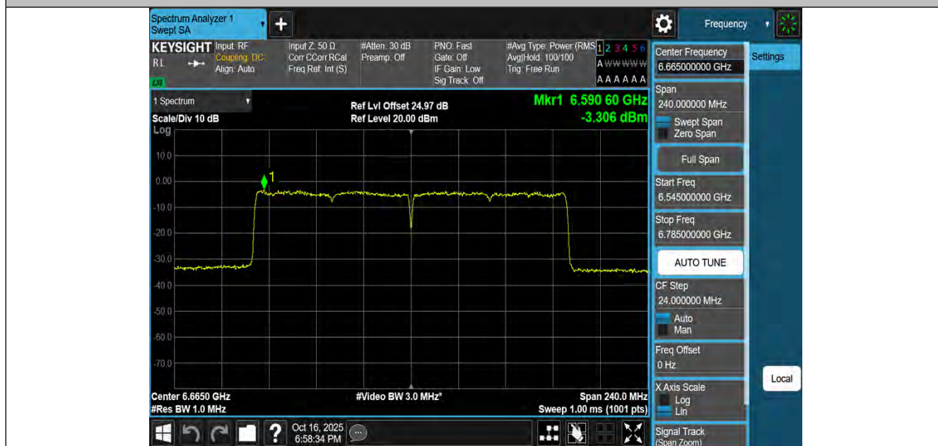
11AX160MIMO-Ant4-6665-PASS
