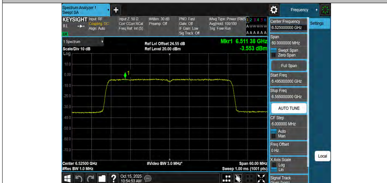
11AX40MIMO-Ant2-6525-PASS
