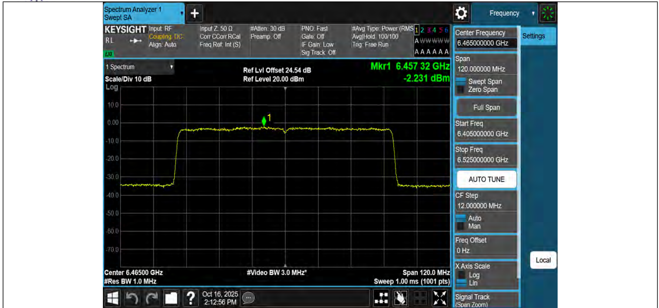
11AX80MIMO-Ant1-6465-PASS
