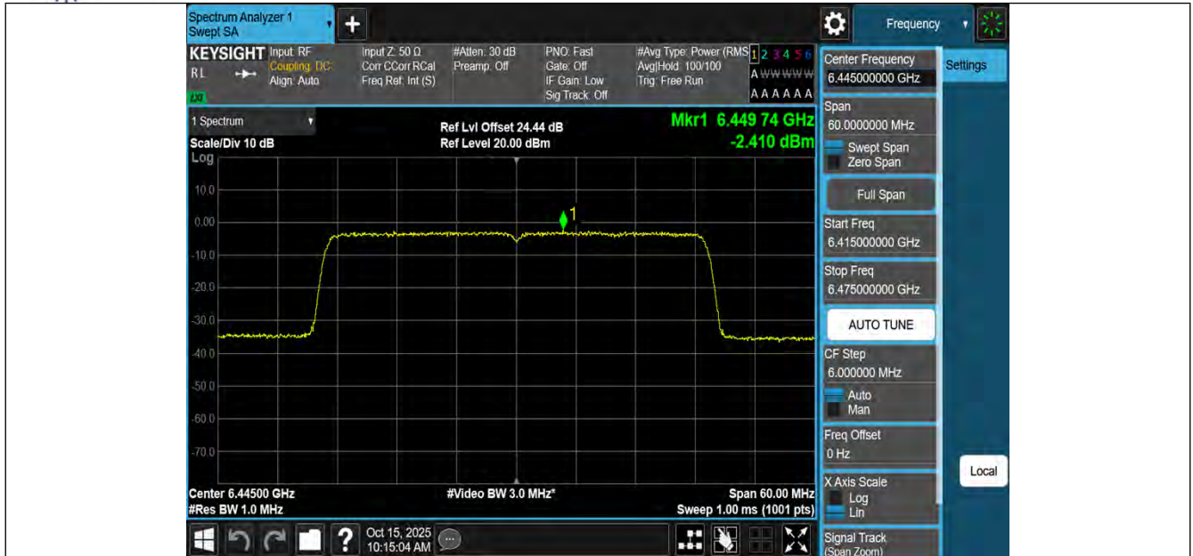
11AX40MIMO-Ant3-6445-PASS
