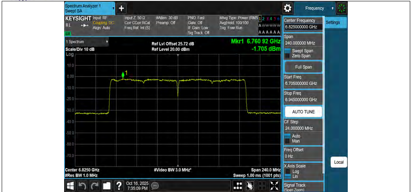
11AX160MIMO-Ant3-6825-PASS
