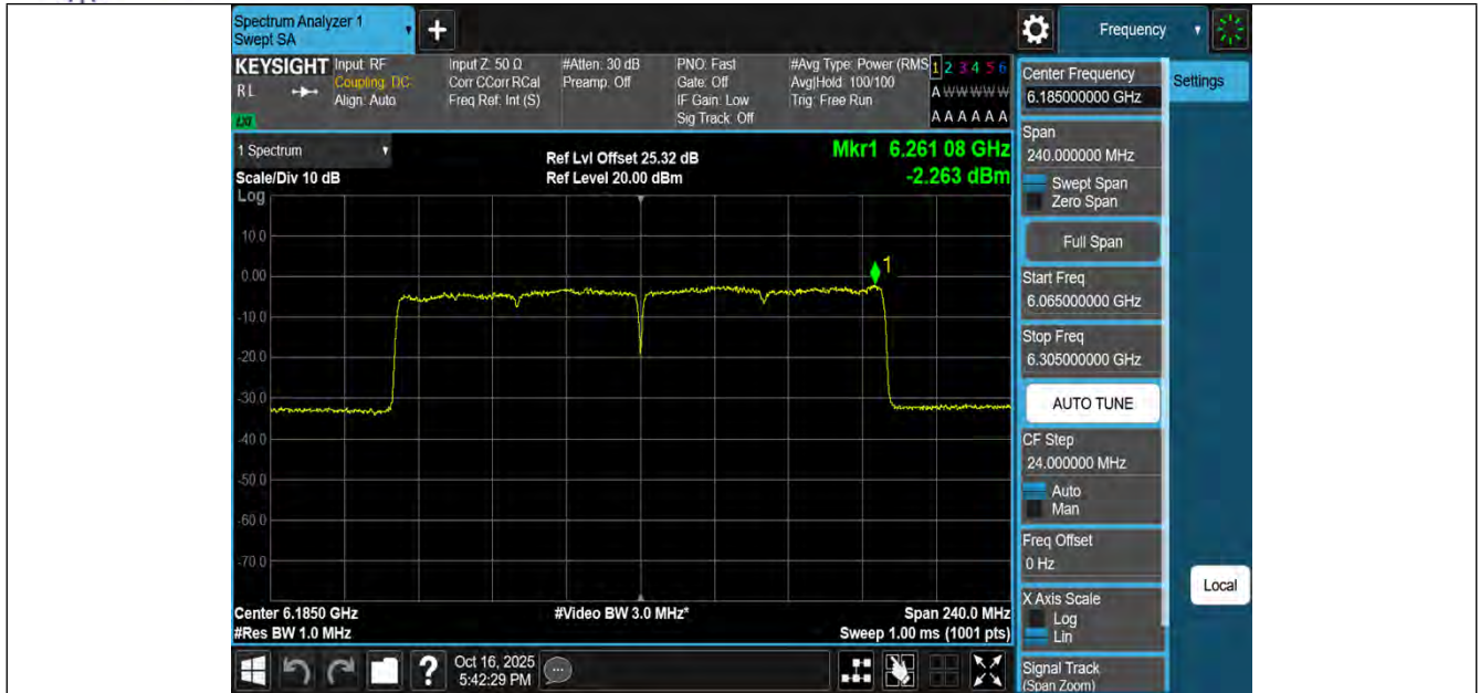
11AX160MIMO-Ant3-6185-PASS
