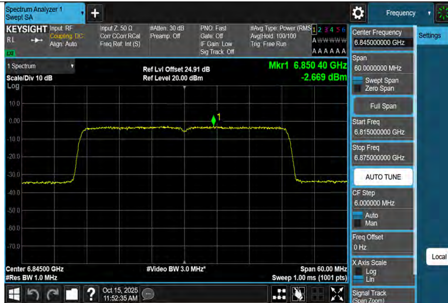
11AX40MIMO-Ant3-6845-PASS
