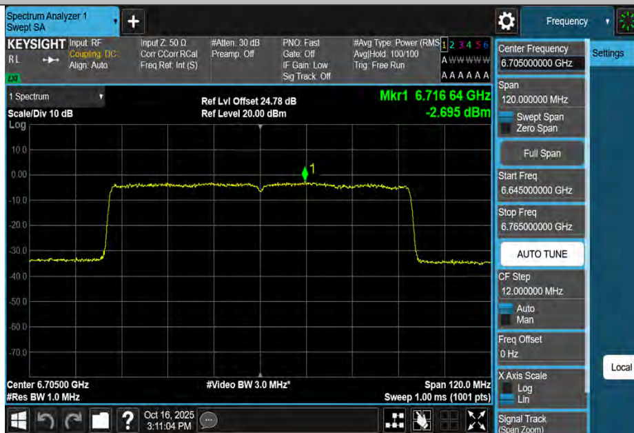
11AX80MIMO-Ant4-6705-PASS
