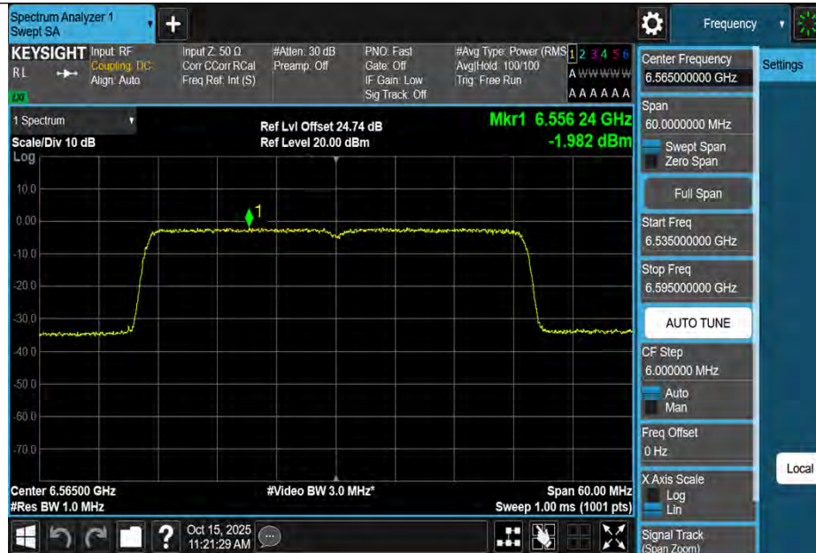
11AX40MIMO-Ant3-6565-PASS
