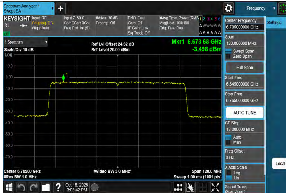
11AX80MIMO-Ant1-6705-PASS
