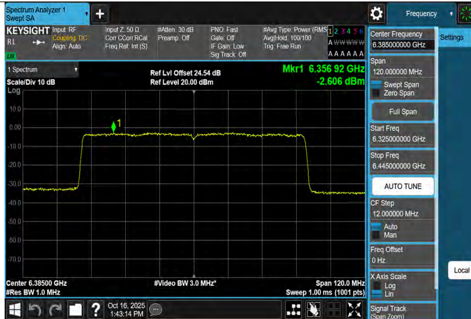
11AX80MIMO-Ant1-6385-PASS
