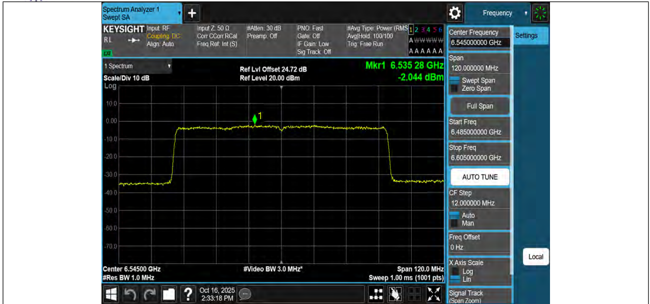
11AX80MIMO-Ant1-6545-PASS
