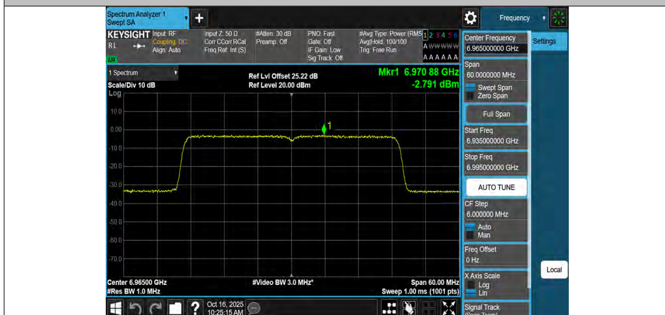
11AX40MIMO-Ant4-6965-PASS
