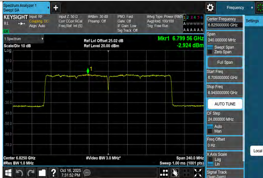
11AX160MIMO-Ant1-6825-PASS
