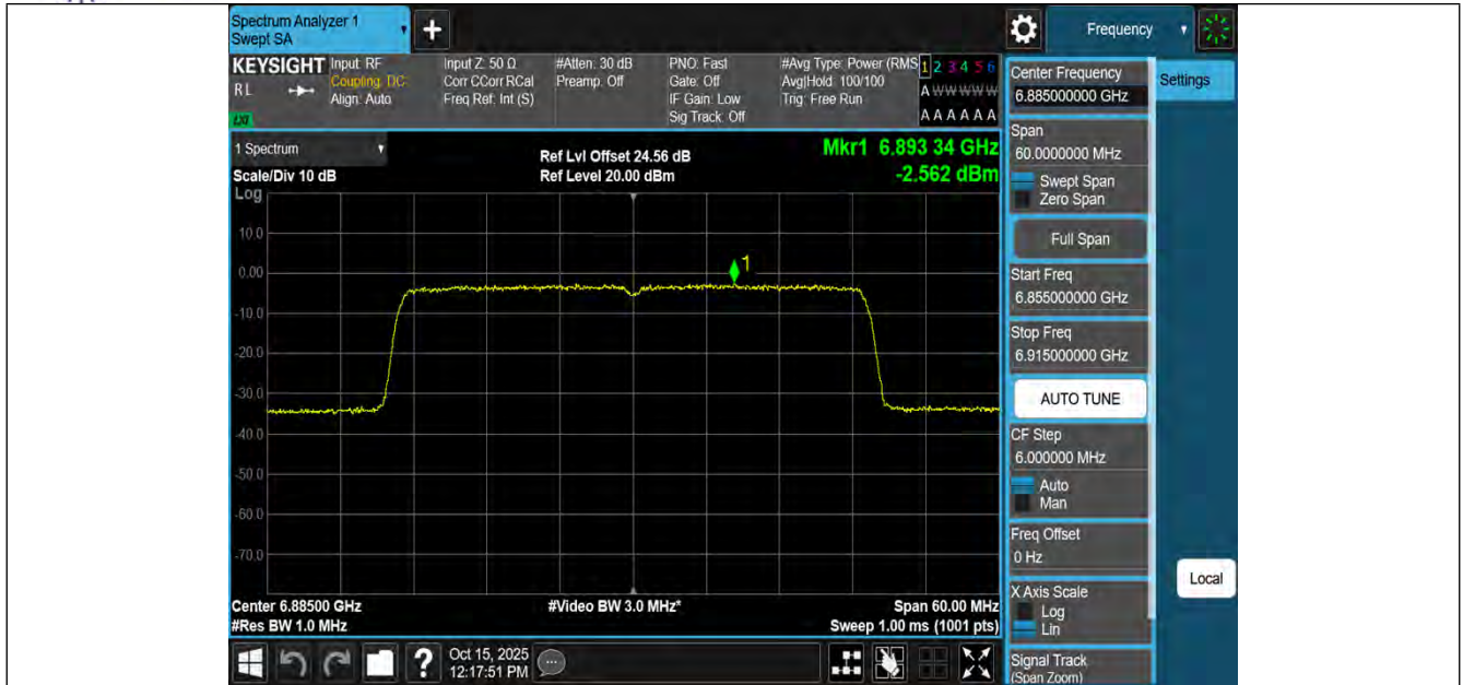
11AX40MIMO-Ant1-6885-PASS
