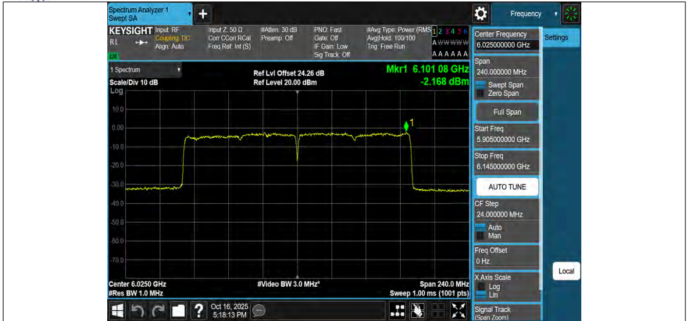
11AX160MIMO-Ant1-6025-PASS
