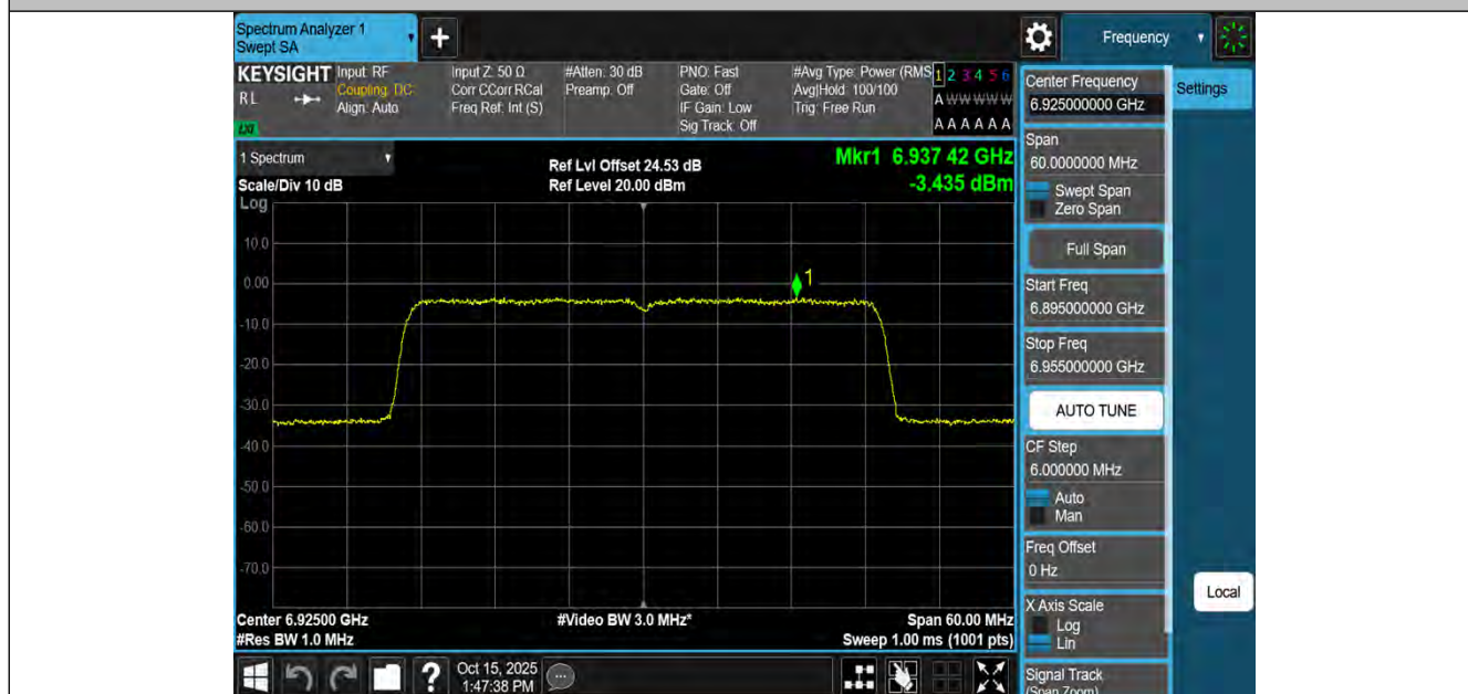
11AX40MIMO-Ant2-6925-PASS
