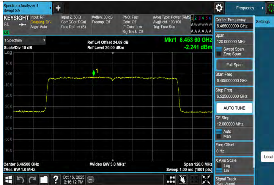
11AX80MIMO-Ant3-6465-PASS
