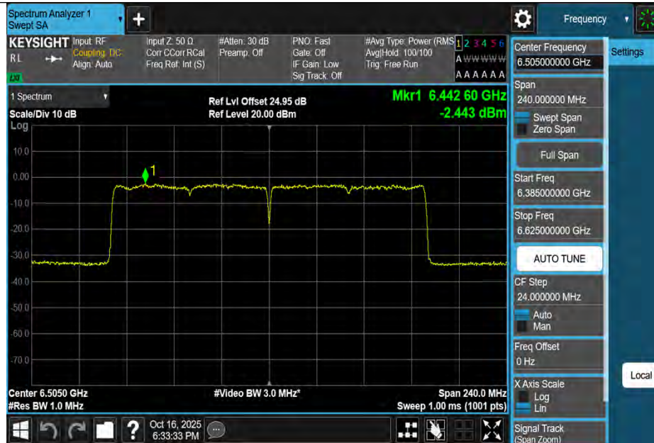
11AX160MIMO-Ant1-6505-PASS
