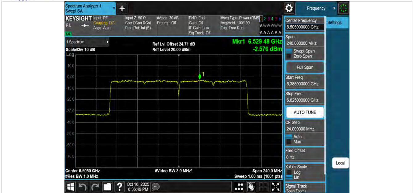
11AX160MIMO-Ant3-6505-PASS
