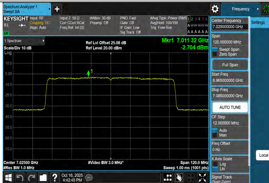
11AX80MIMO-Ant4-7025-PASS
