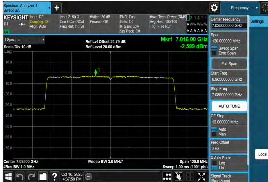
11AX80MIMO-Ant1-7025-PASS
