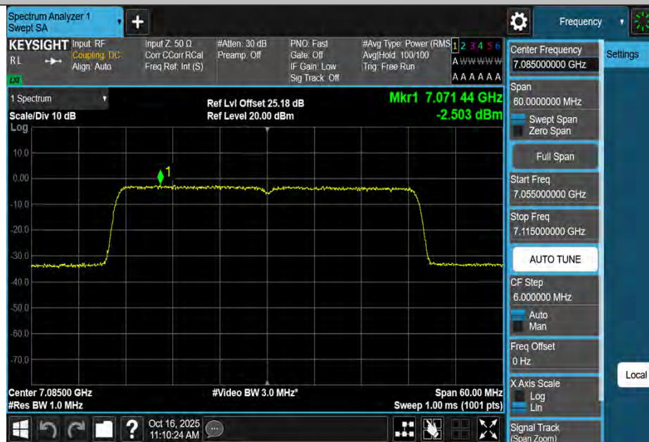
11AX40MIMO-Ant4-7085-PASS
