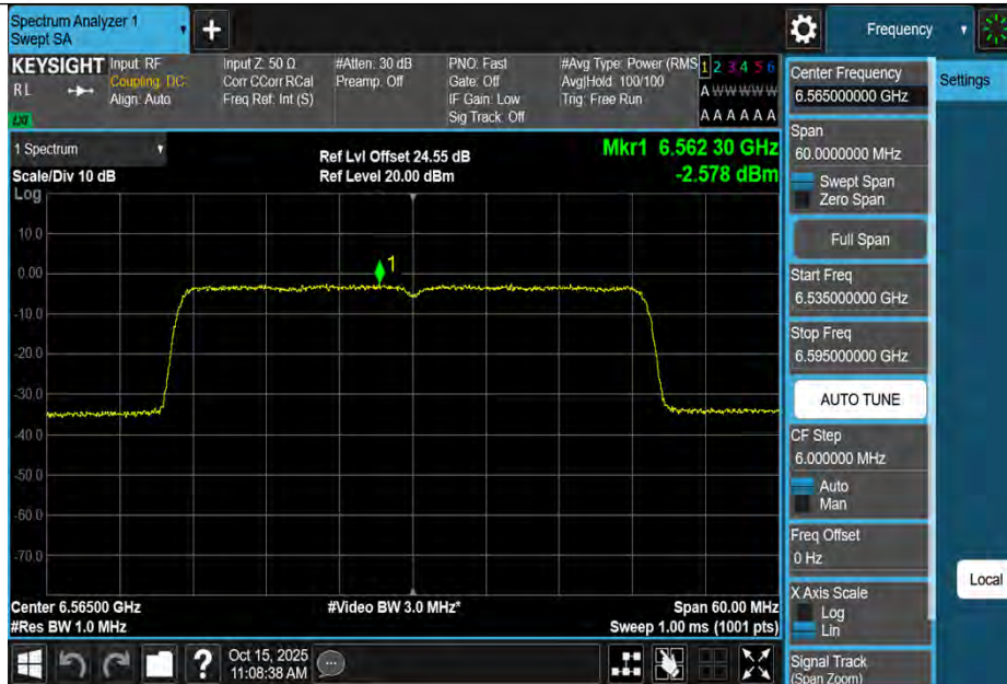
11AX40MIMO-Ant1-6565-PASS
