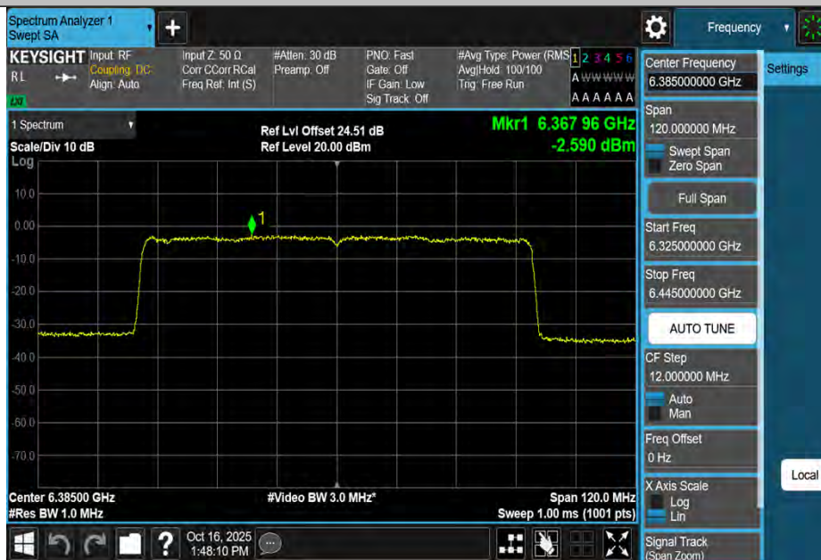
11AX80MIMO-Ant4-6385-PASS
