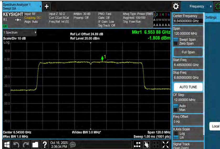
11AX80MIMO-Ant3-6545-PASS
