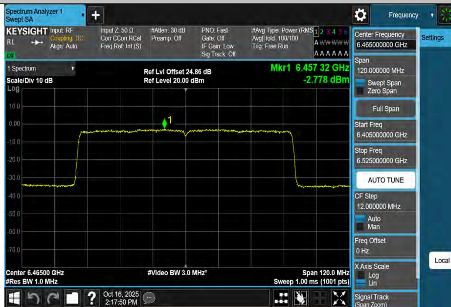
11AX80MIMO-Ant4-6465-PASS
