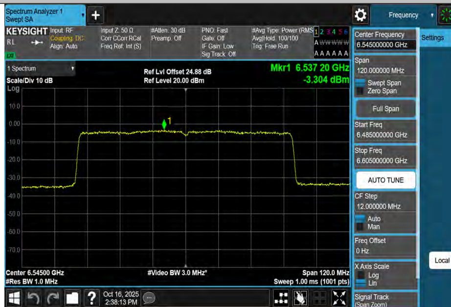
11AX80MIMO-Ant4-6545-PASS
