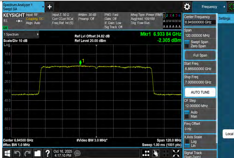
11AX80MIMO-Ant1-6945-PASS
