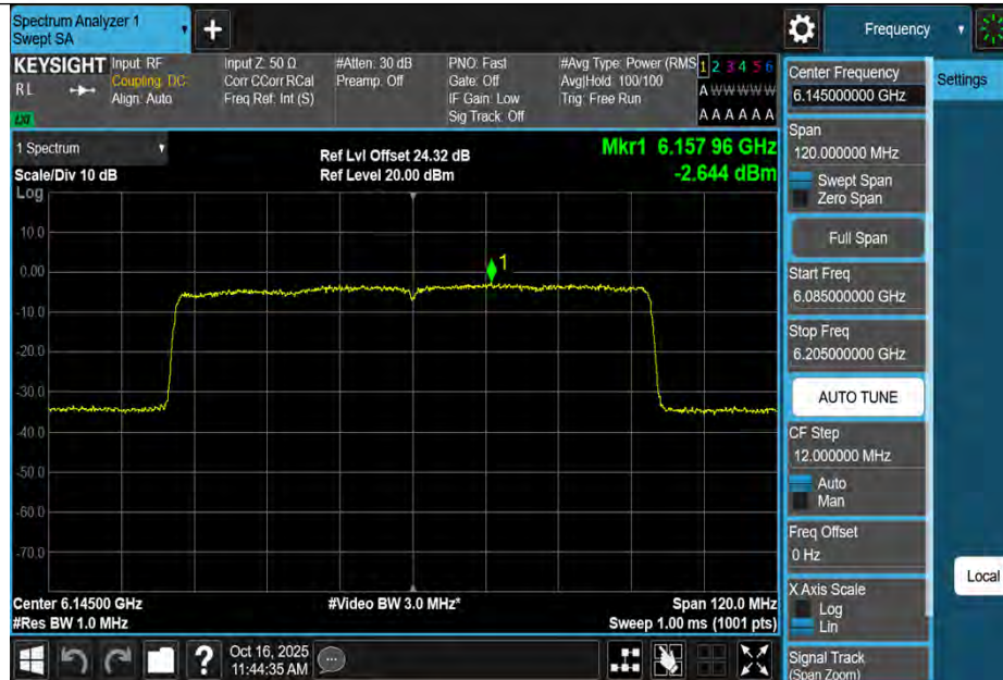
11AX80MIMO-Ant3-6145-PASS
