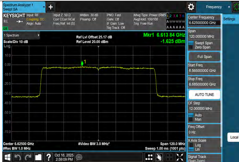
11AX80MIMO-Ant3-6625-PASS
