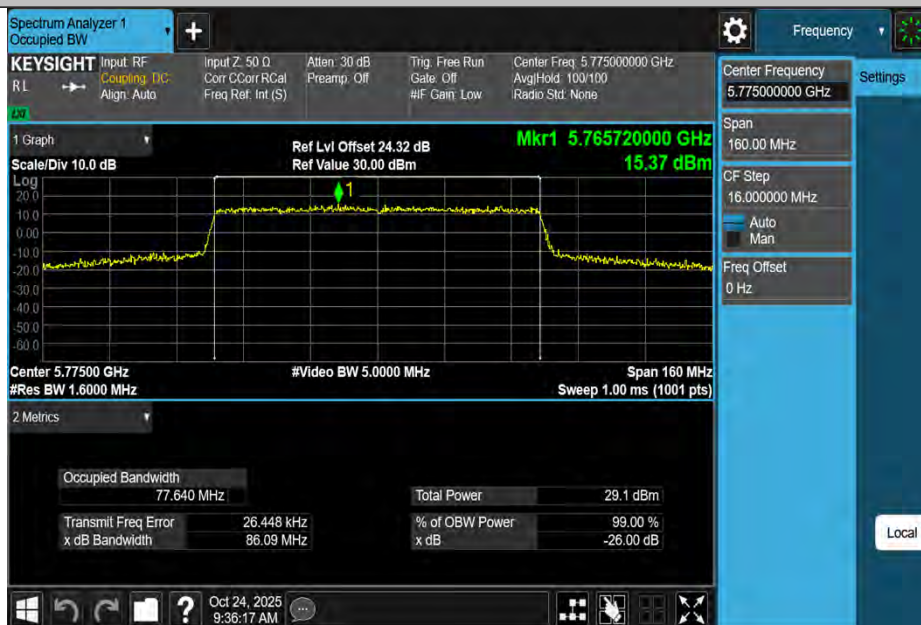
11AX80MIMO-Ant4-5775
