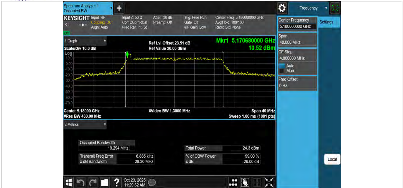
11AX20MIMO-Ant3-5180
