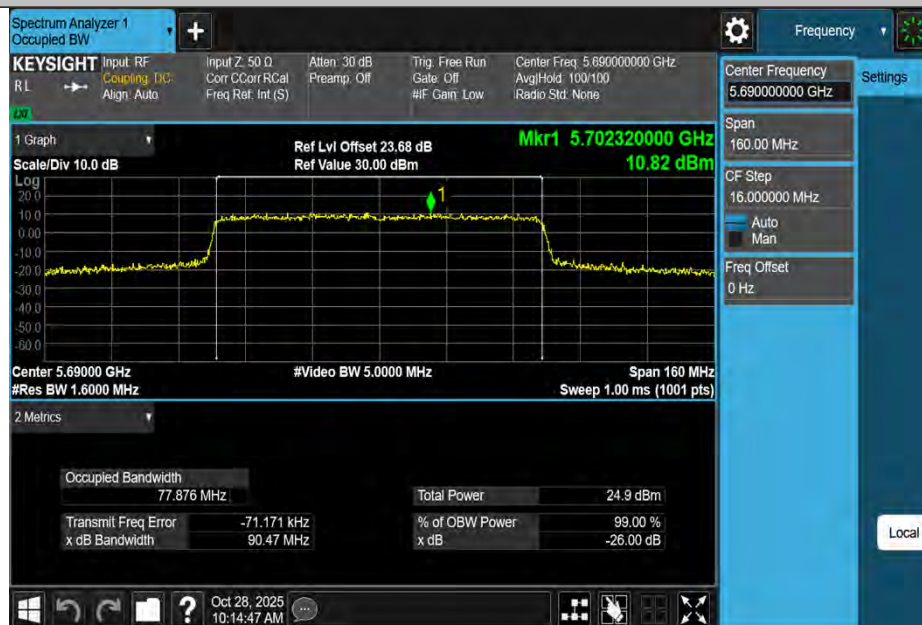
11AX80MIMO-Ant2-5690
