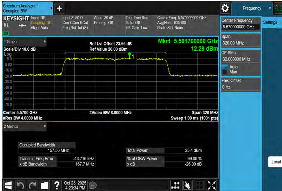
11AX160MIMO-Ant1-5570
