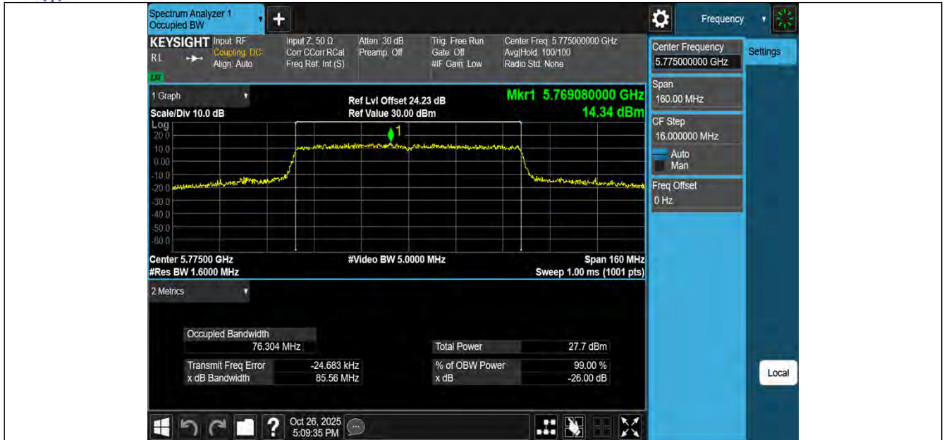
11AC80MIMO-Ant3-5775
