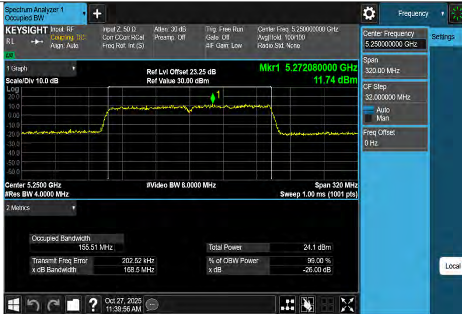
11AC160MIMO-Ant3-5250
