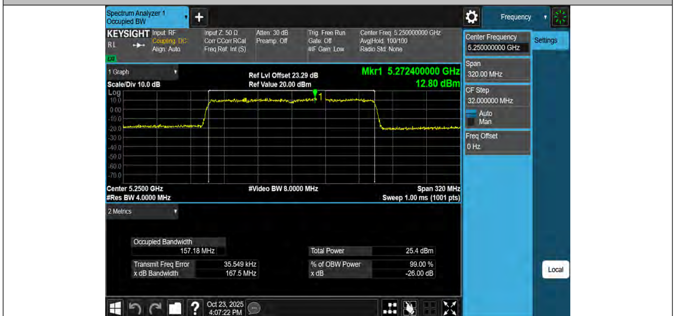
11AX160MIMO-Ant4-5250
