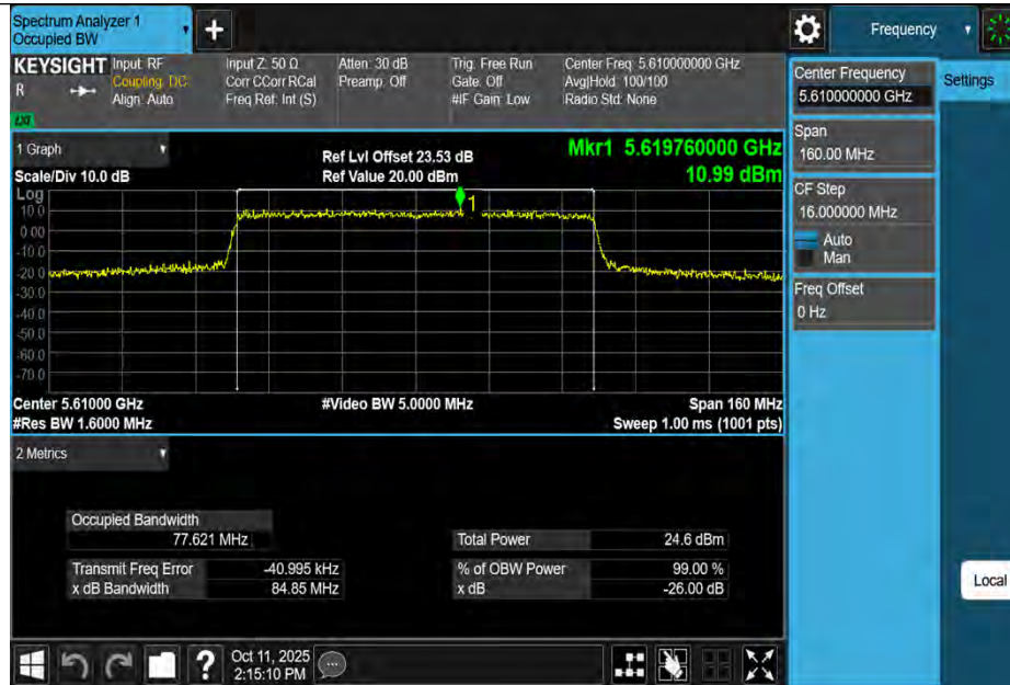
11AX80MIMO-Ant3-5610
