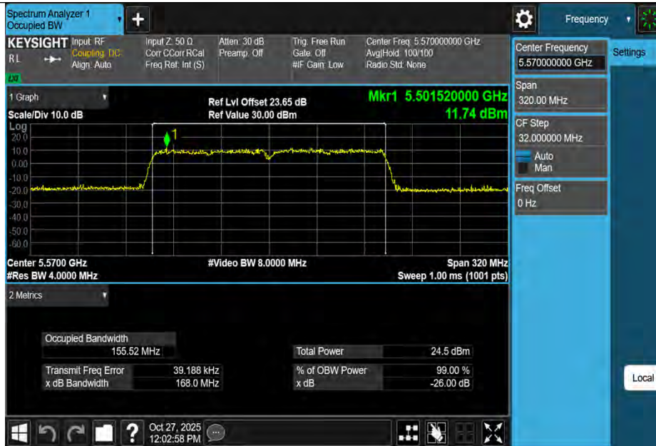
11AC160MIMO-Ant3-5570
