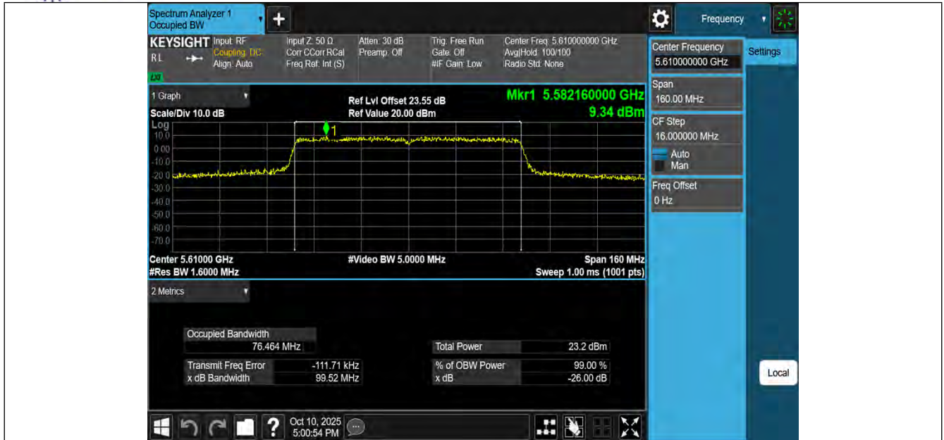
11AC80MIMO-Ant1-5610
