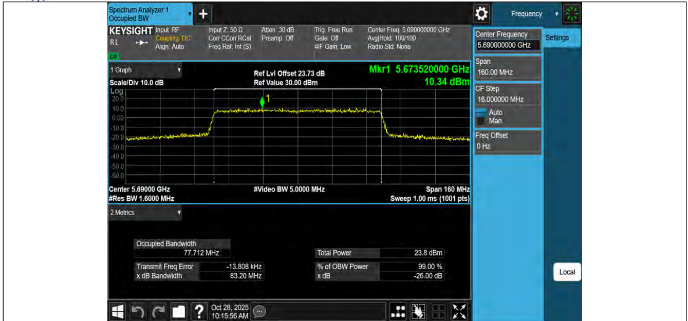
11AX80MIMO-Ant3-5690
