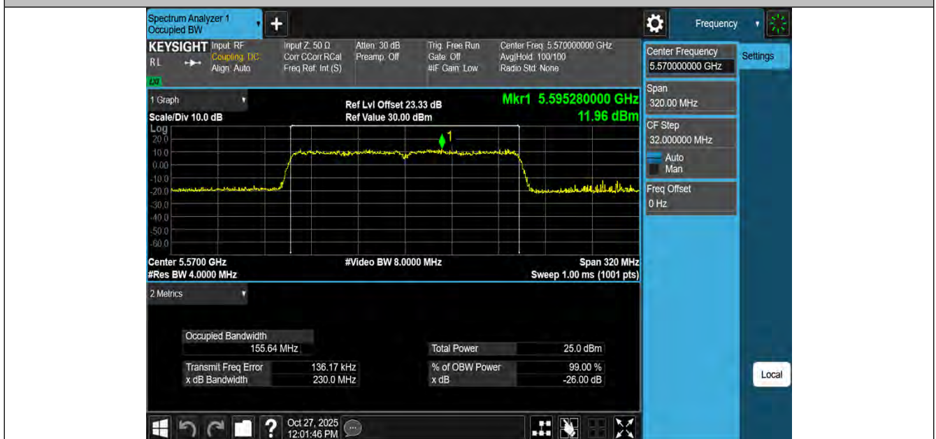
11AC160MIMO-Ant2-5570
