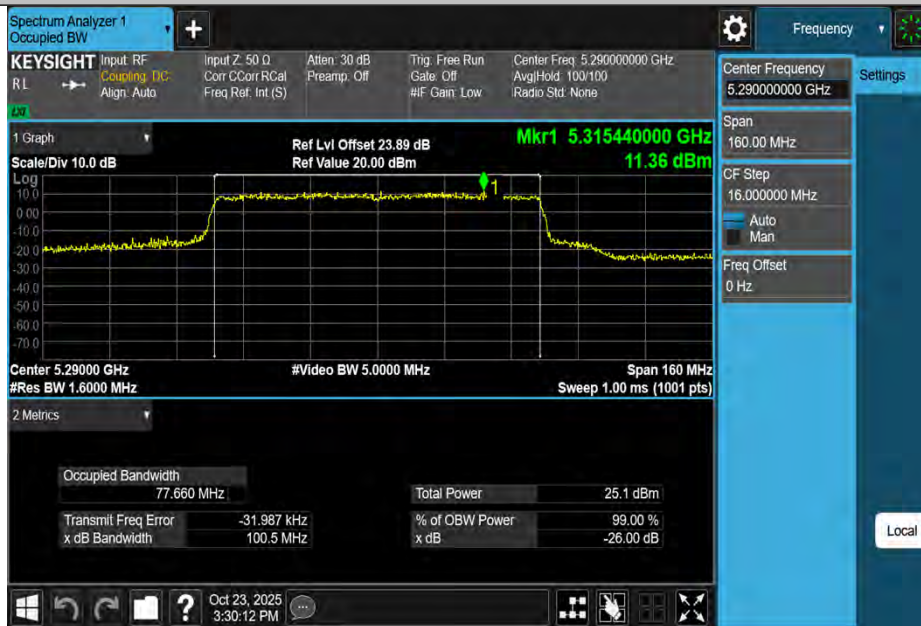
11AX80MIMO-Ant4-5290
