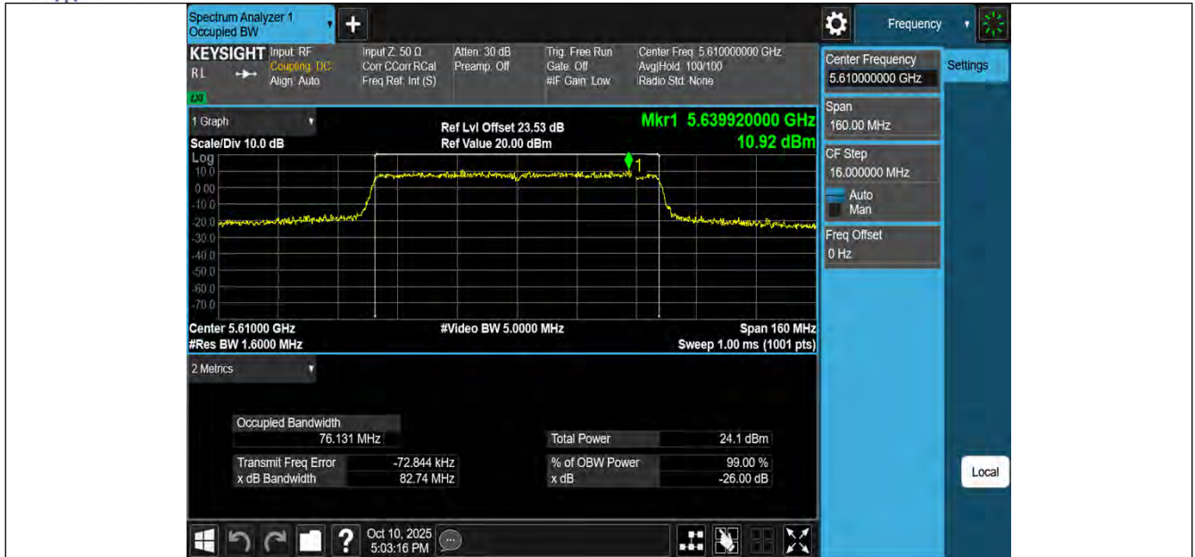
11AC80MIMO-Ant3-5610
