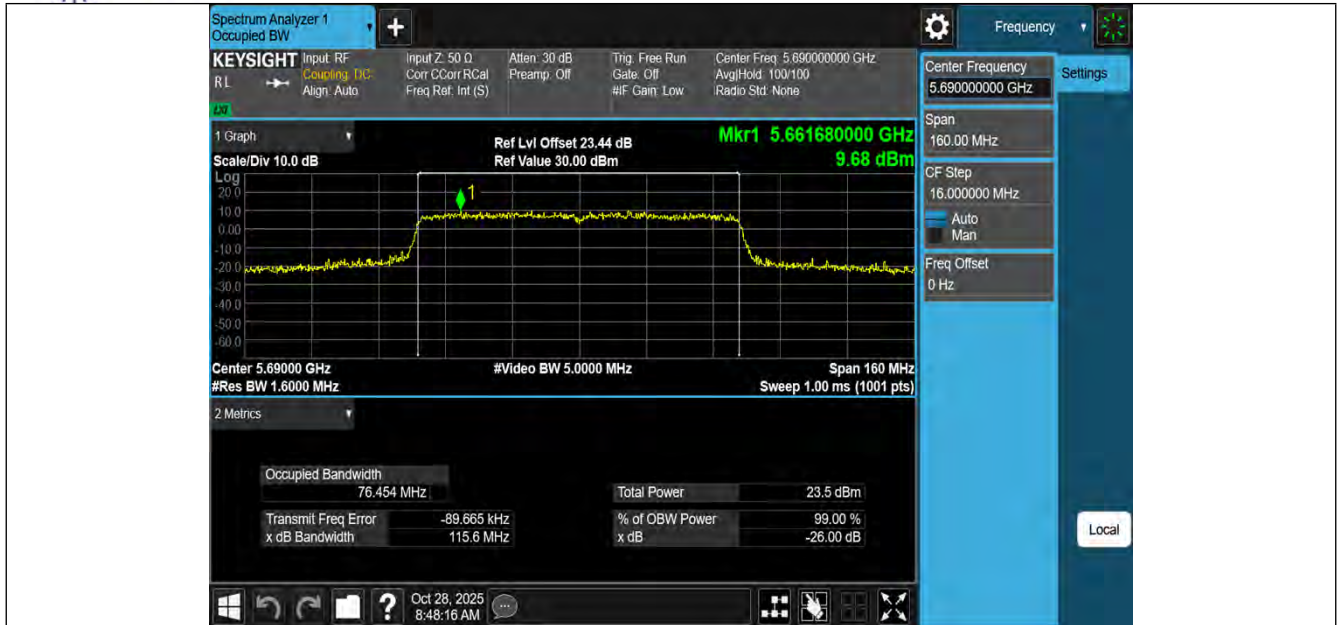
11AC80MIMO-Ant1-5690
