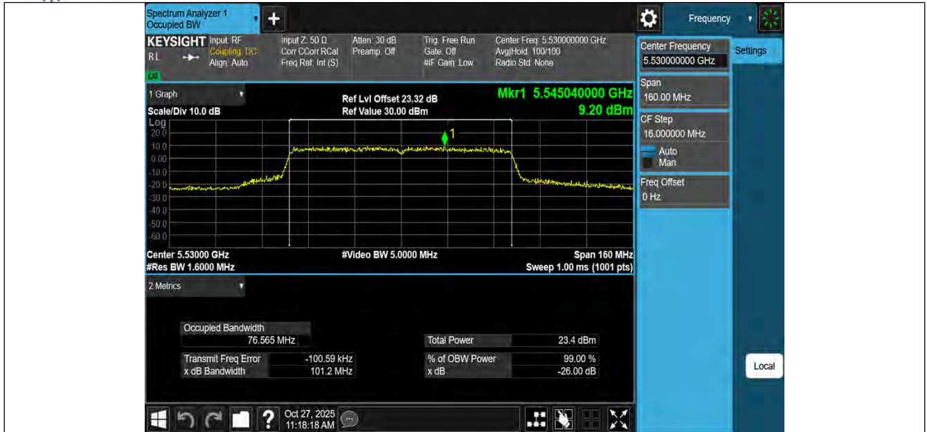
11AC80MIMO-Ant1-5530
