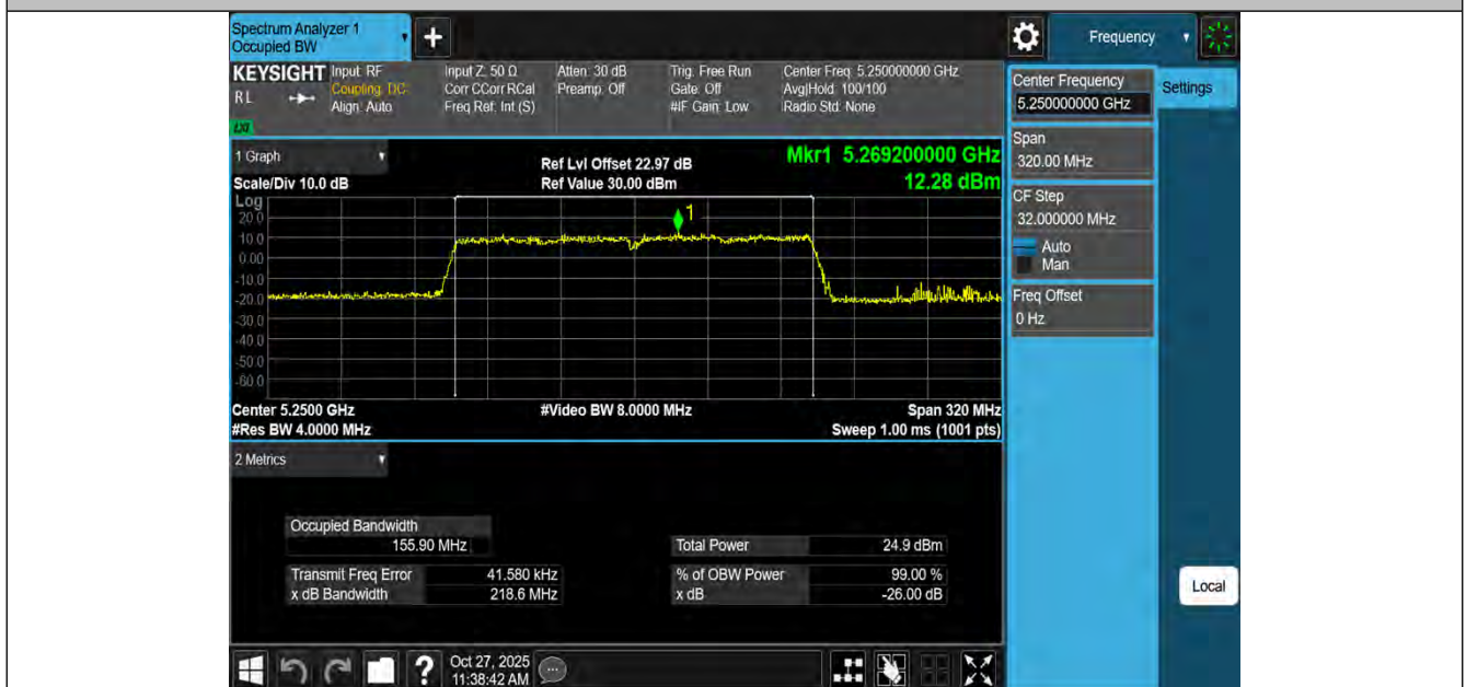
11AC160MIMO-Ant2-5250
