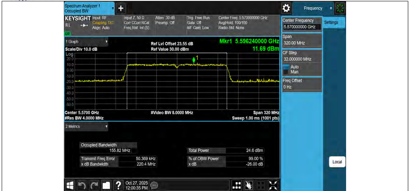
11AC160MIMO-Ant1-5570
