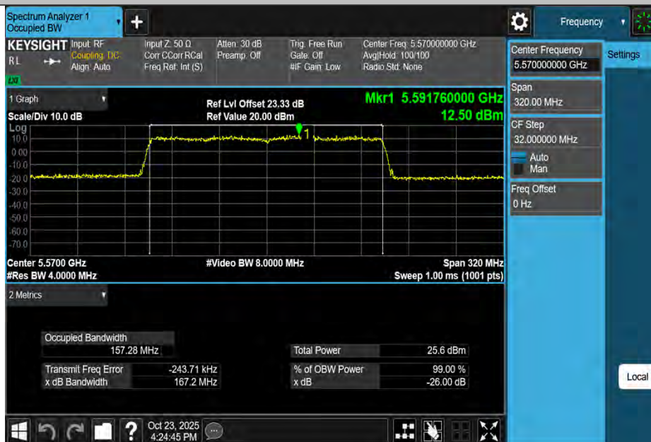
11AX160MIMO-Ant2-5570
