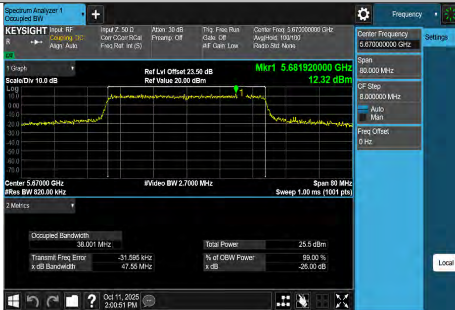
11AX40MIMO-Ant2-5670
