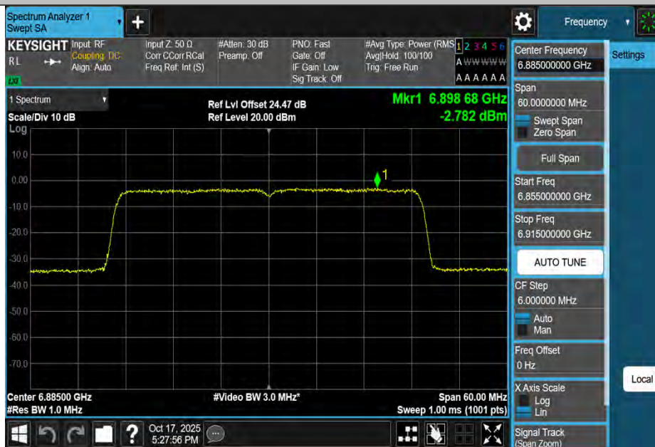
11BE40MIMO-Ant2-6885-PASS
