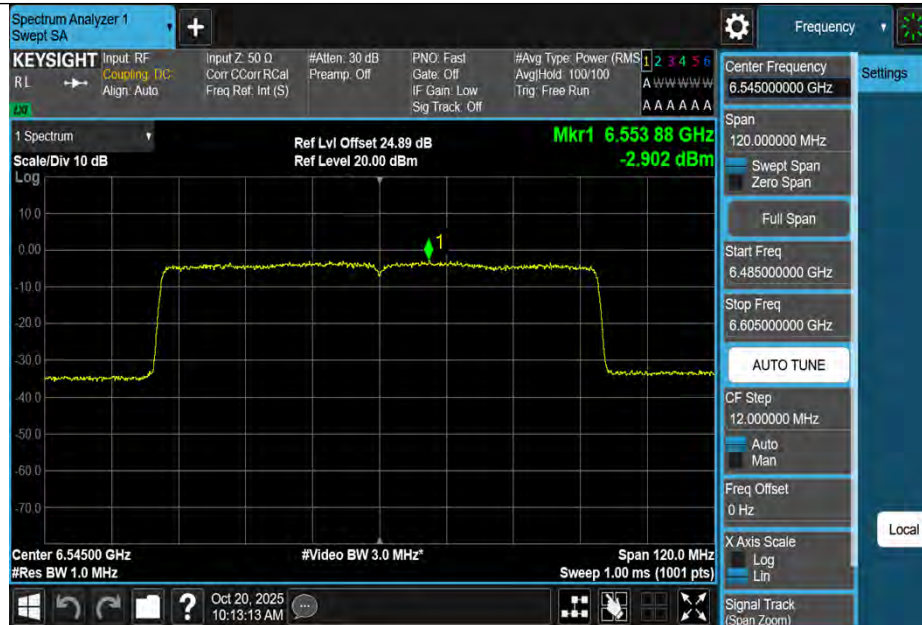
11BE80MIMO-Ant3-6545-PASS
