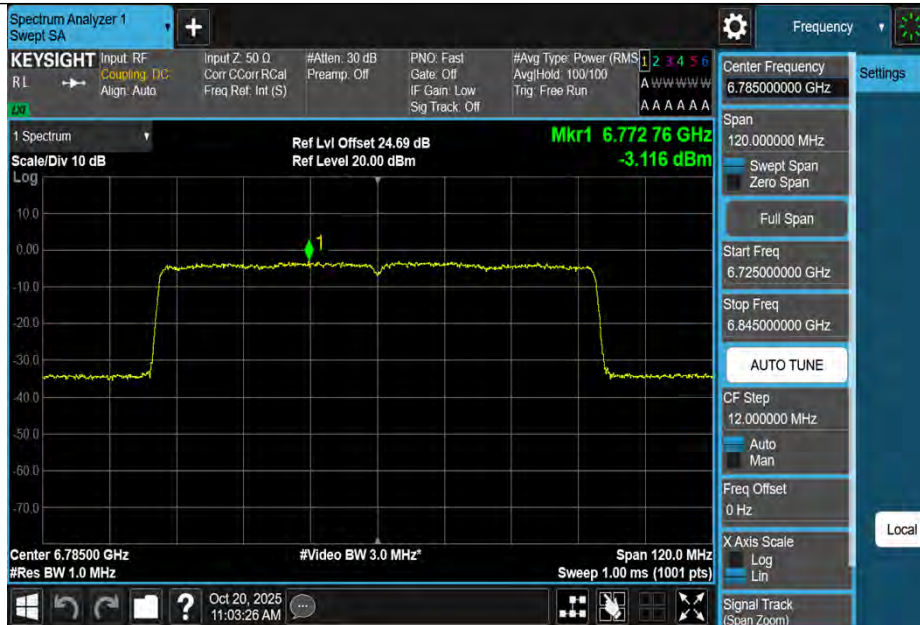
11BE80MIMO-Ant1-6785-PASS
