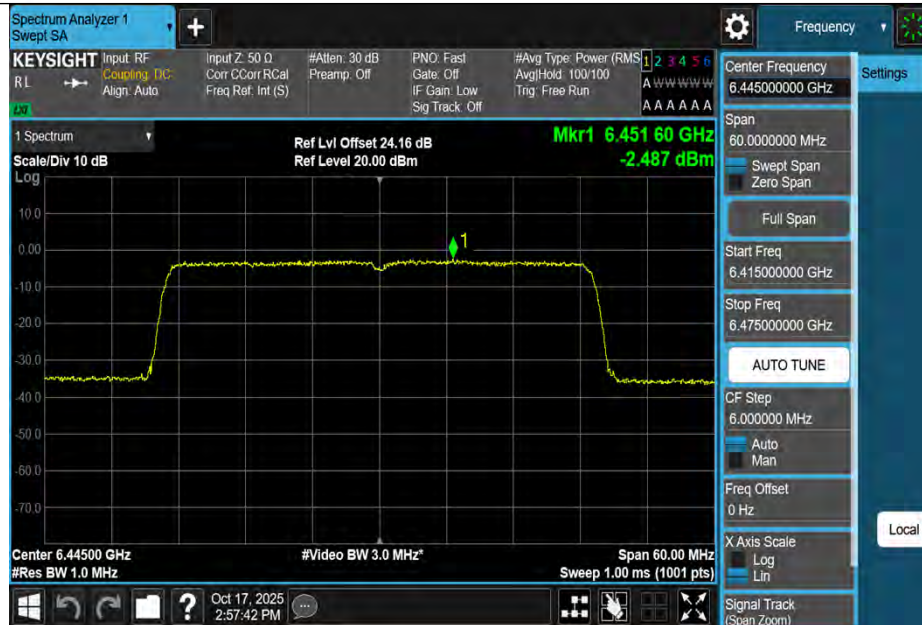
11BE40MIMO-Ant1-6445-PASS
