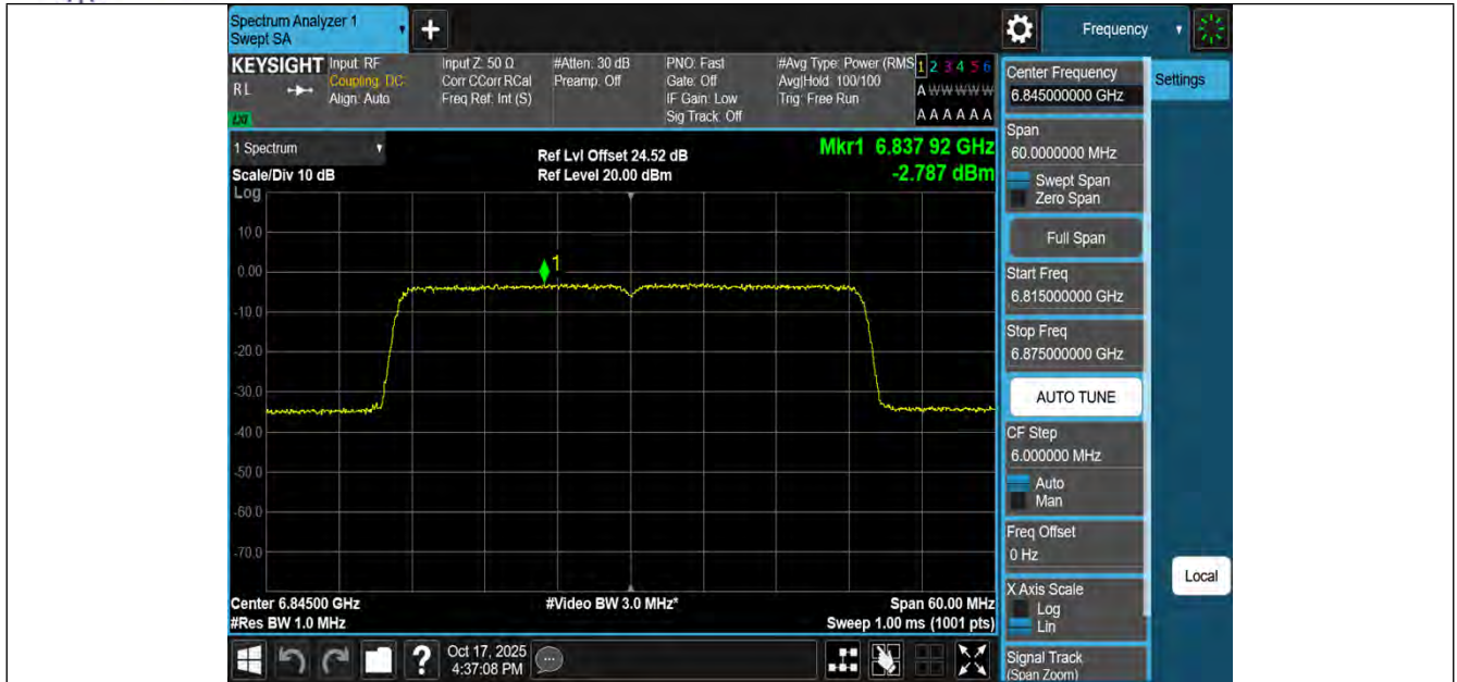
11BE40MIMO-Ant1-6845-PASS
