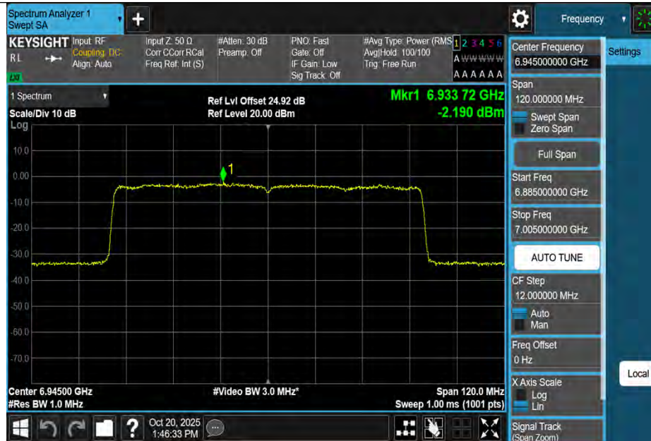
11BE80MIMO-Ant1-6945-PASS
