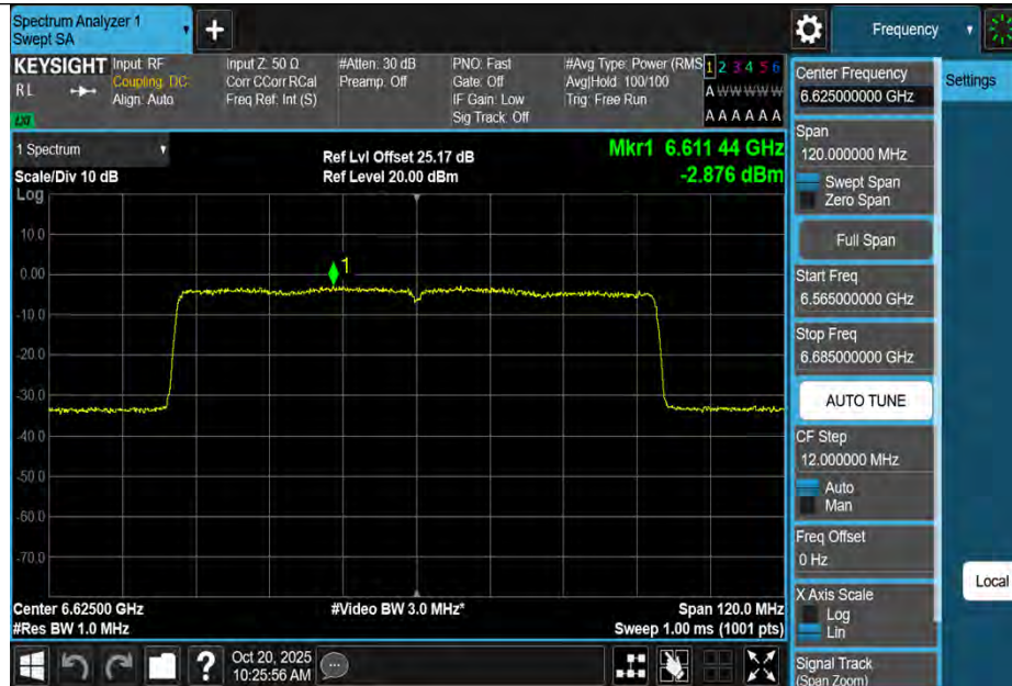
11BE80MIMO-Ant3-6625-PASS
