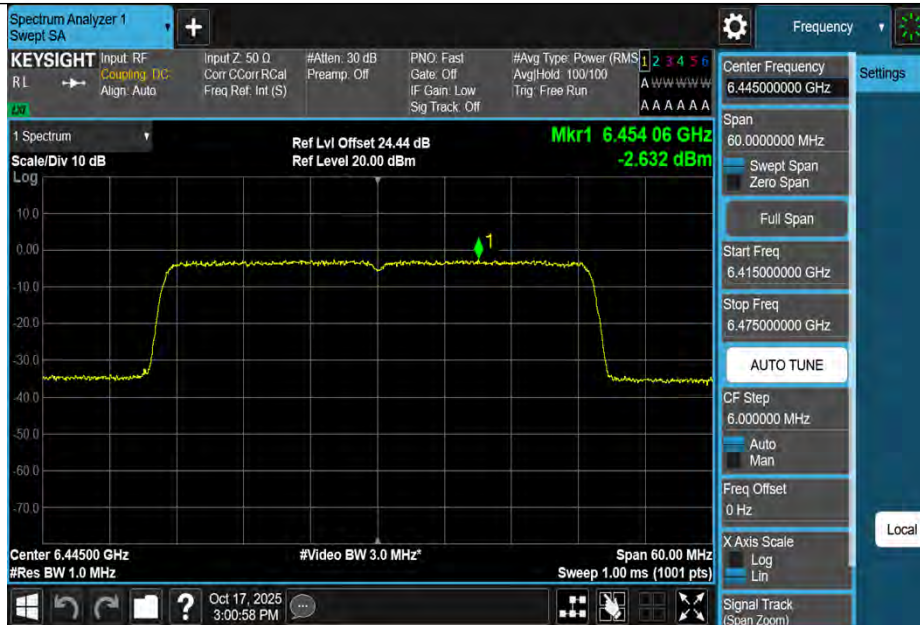
11BE40MIMO-Ant3-6445-PASS
