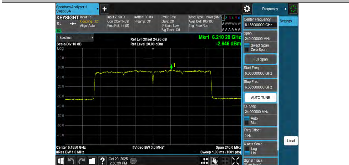
11BE160MIMO-Ant4-6185-PASS
