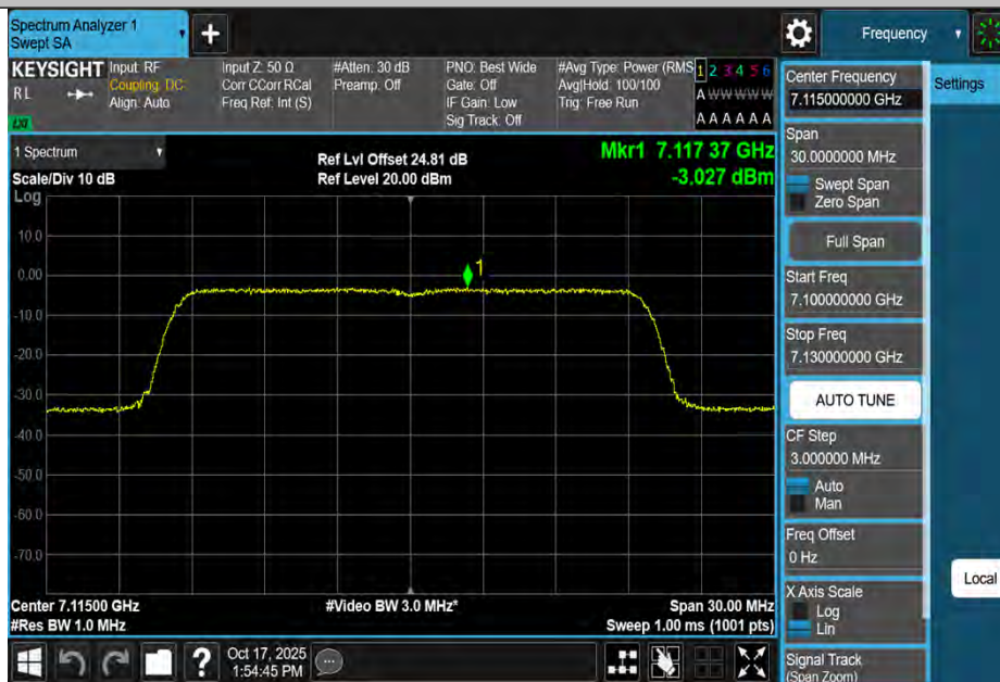
11BE20MIMO-Ant2-7115-PASS
