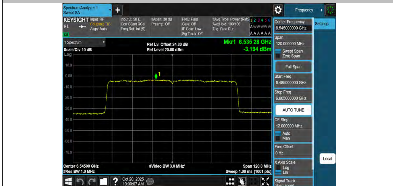
11BE80MIMO-Ant2-6545-PASS
