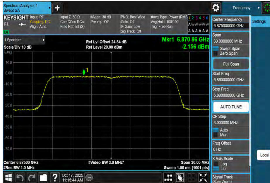
11BE20MIMO-Ant3-6875-PASS
