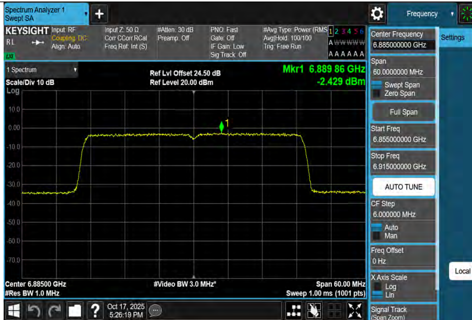
11BE40MIMO-Ant1-6885-PASS
