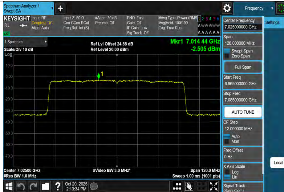
11BE80MIMO-Ant1-7025-PASS
