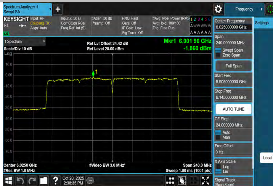
11BE160MIMO-Ant4-6025-PASS
