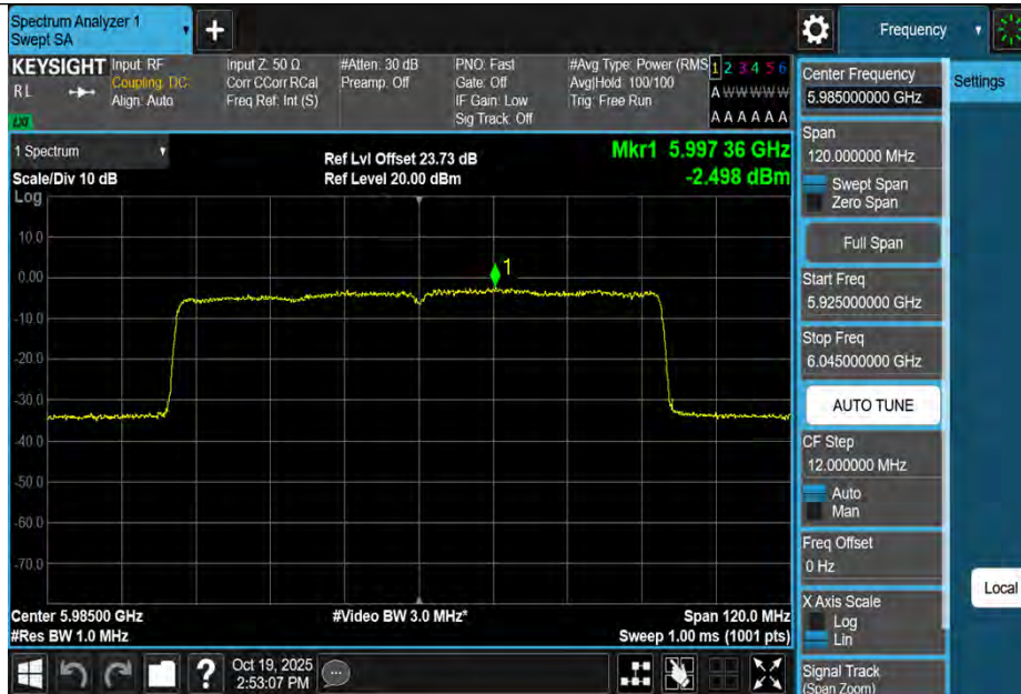
11BE80MIMO-Ant1-5985-PASS
