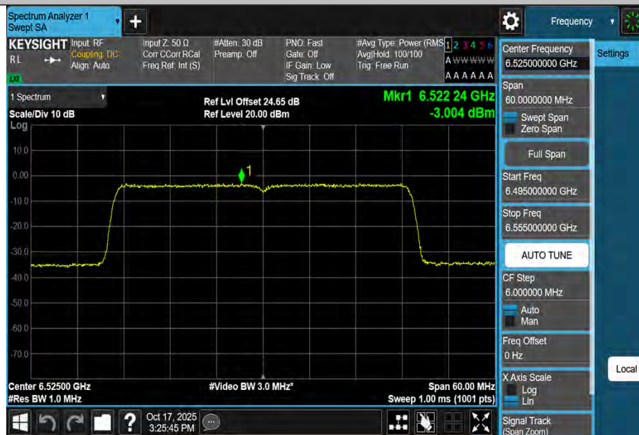
11BE40MIMO-Ant4-6525-PASS
