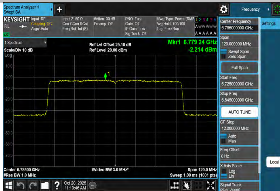
11BE80MIMO-Ant4-6785-PASS
