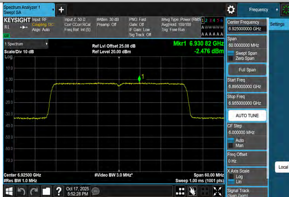
11BE40MIMO-Ant4-6925-PASS
