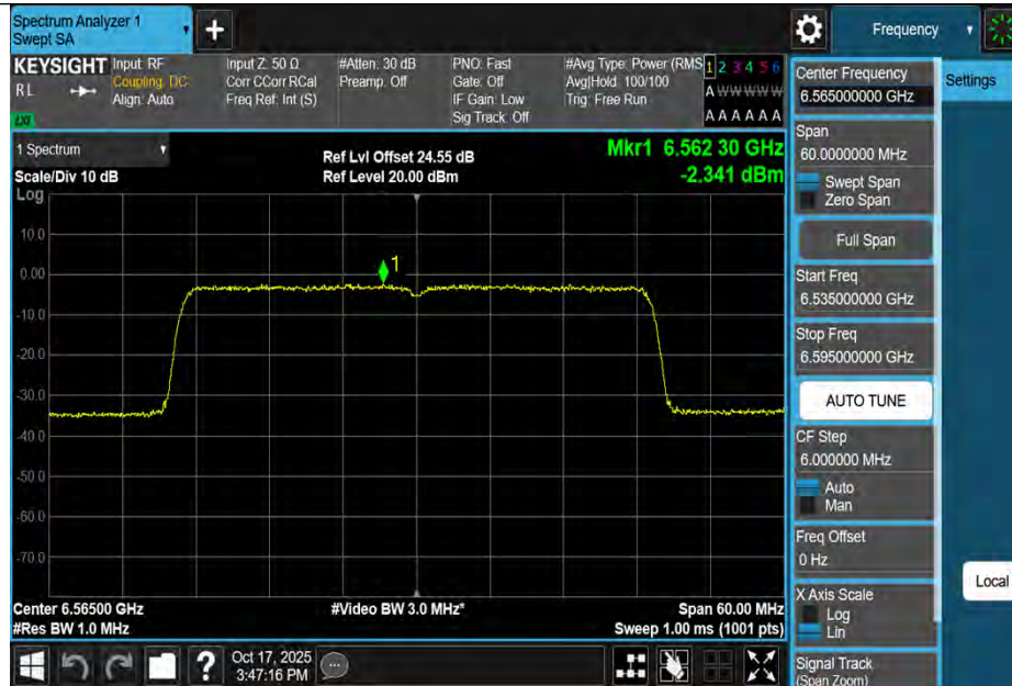
11BE40MIMO-Ant1-6565-PASS
