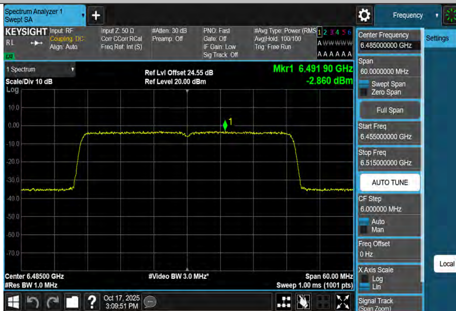
11BE40MIMO-Ant2-6485-PASS
