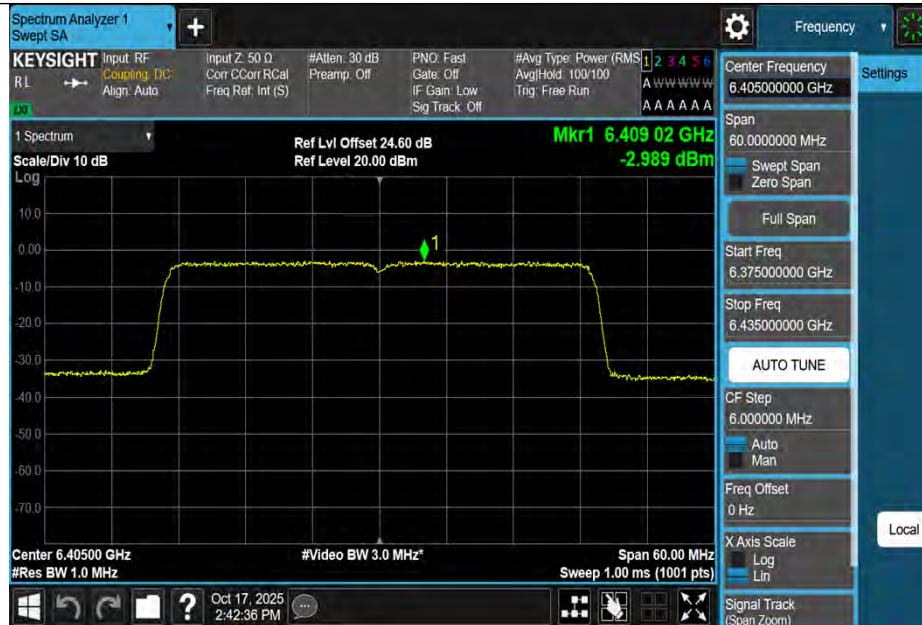
11BE40MIMO-Ant3-6405-PASS
