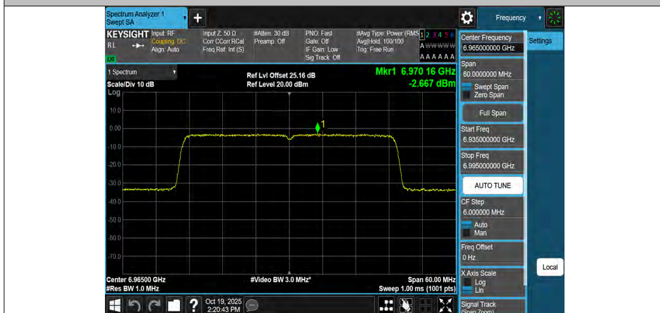
11BE40MIMO-Ant4-6965-PASS
