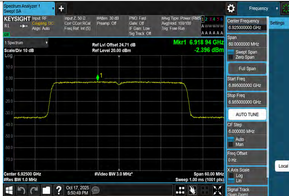
11BE40MIMO-Ant3-6925-PASS
