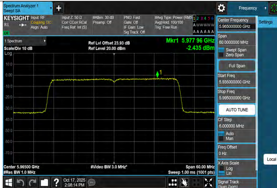
11BE40MIMO-Ant3-5965-PASS
