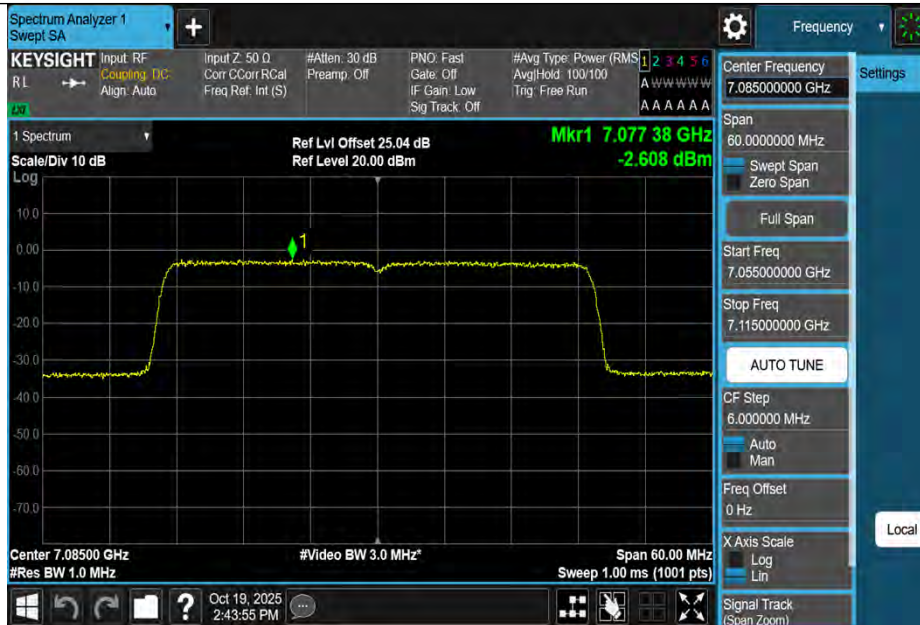
11BE40MIMO-Ant3-7085-PASS
