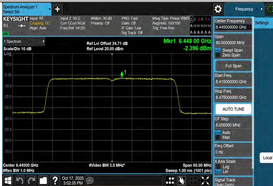
11BE40MIMO-Ant4-6445-PASS
