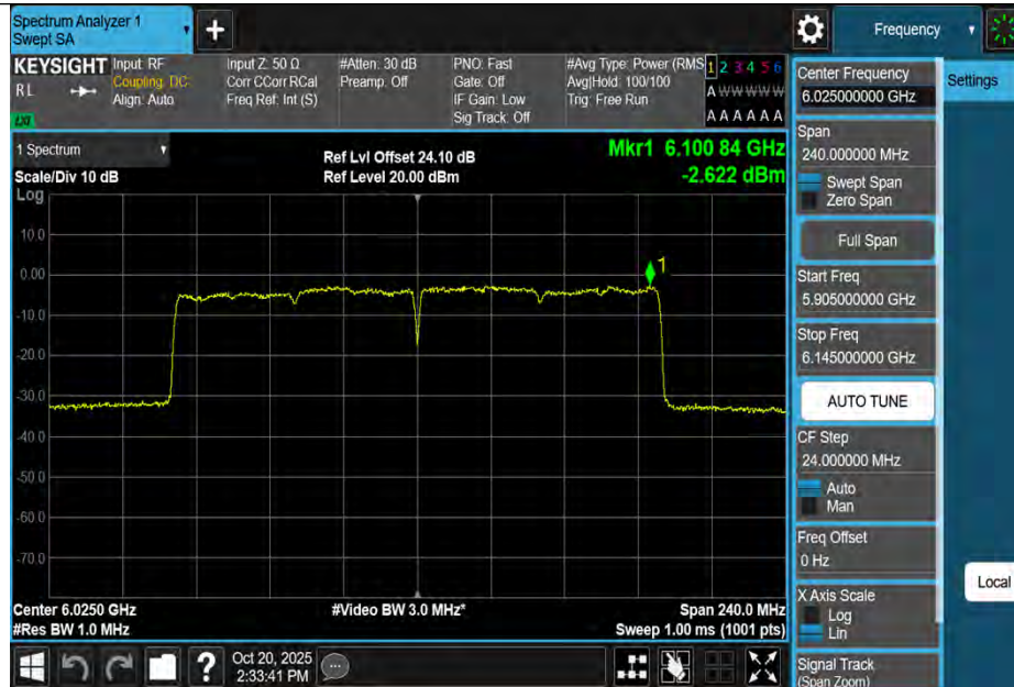
11BE160MIMO-Ant1-6025-PASS
