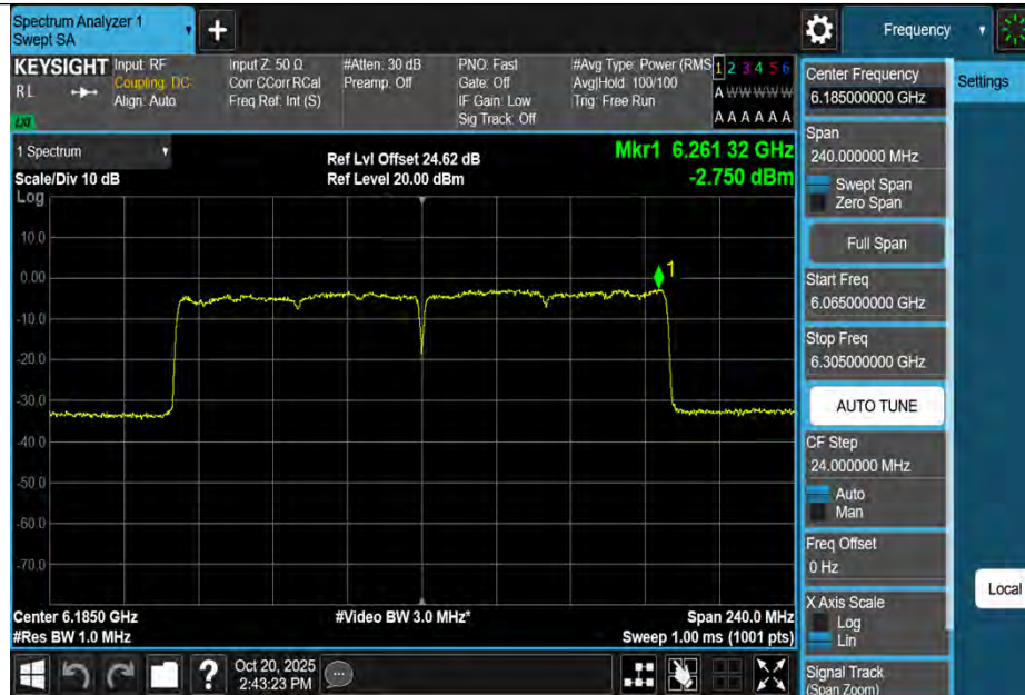
11BE160MIMO-Ant1-6185-PASS
