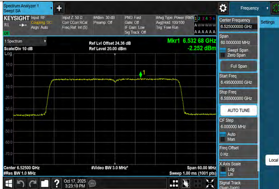
11BE40MIMO-Ant3-6525-PASS
