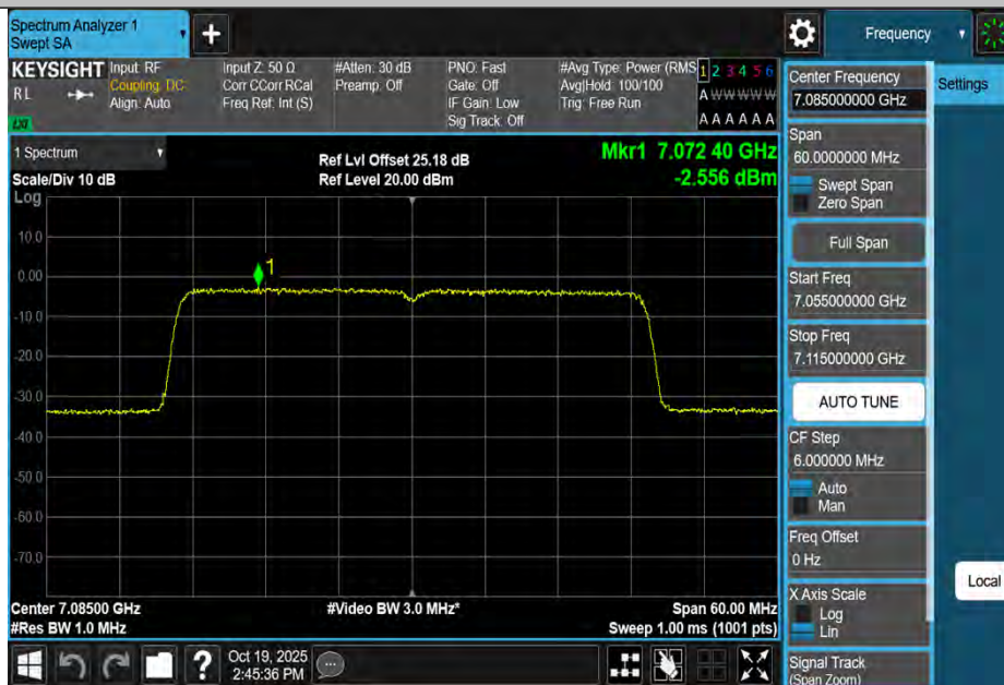
11BE40MIMO-Ant4-7085-PASS
