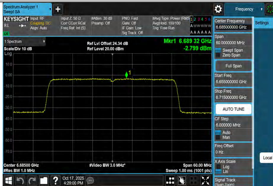
11BE40MIMO-Ant2-6685-PASS
