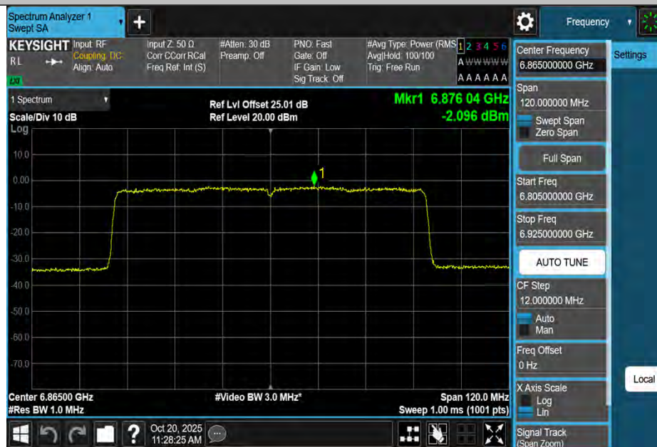
11BE80MIMO-Ant4-6865-PASS
