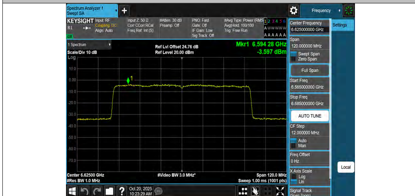
11BE80MIMO-Ant2-6625-PASS
