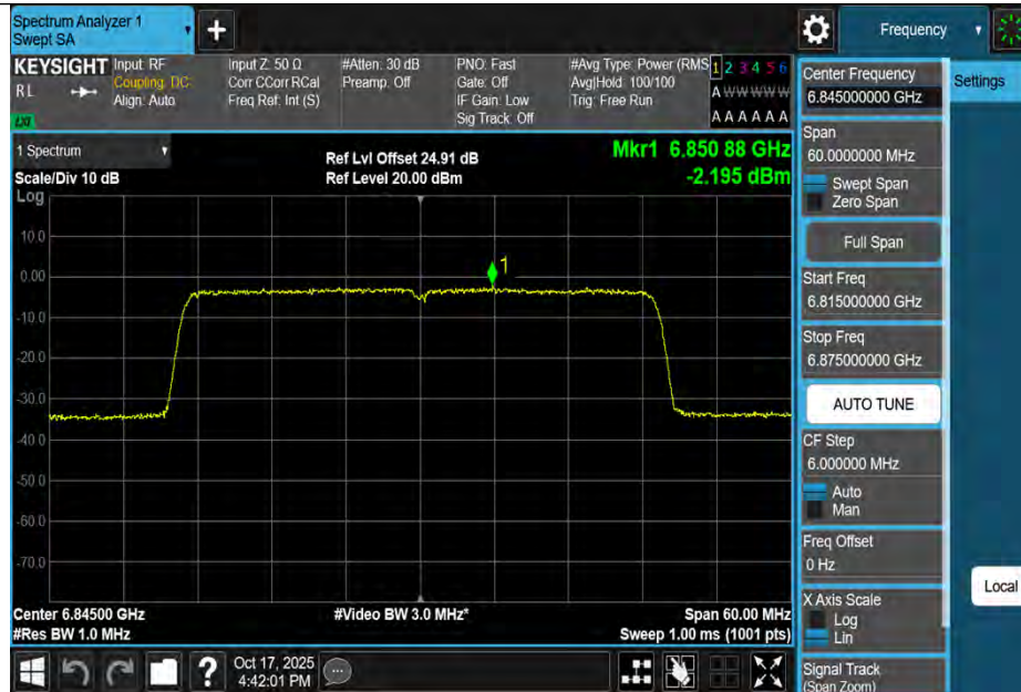
11BE40MIMO-Ant3-6845-PASS
