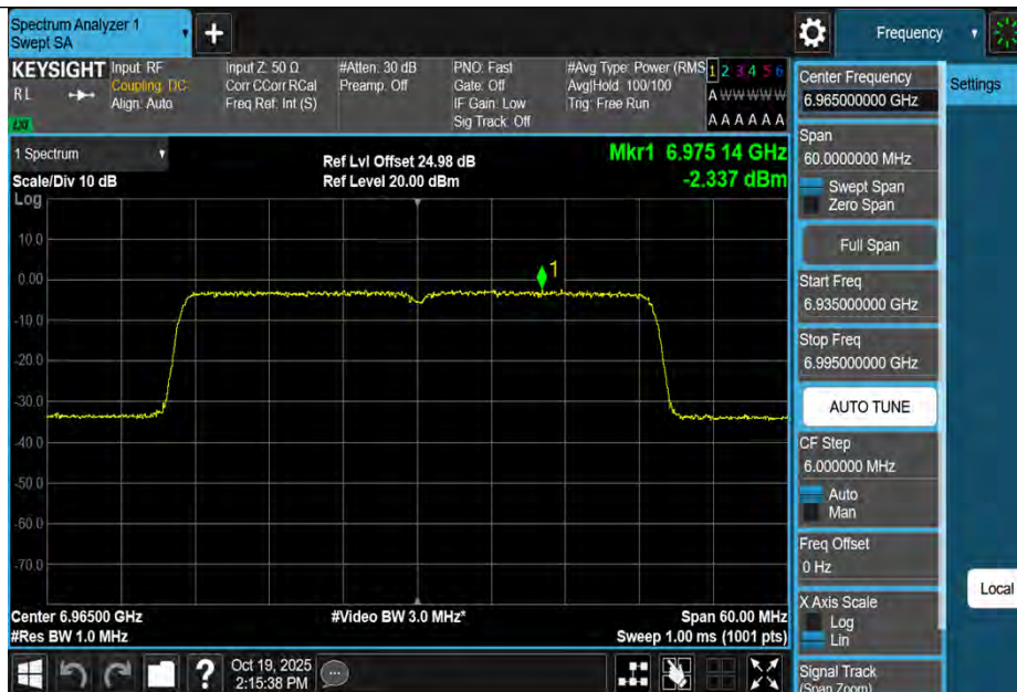
11BE40MIMO-Ant1-6965-PASS
