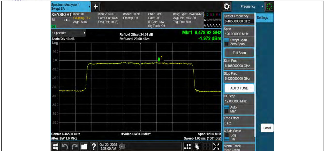
11BE80MIMO-Ant1-6465-PASS
