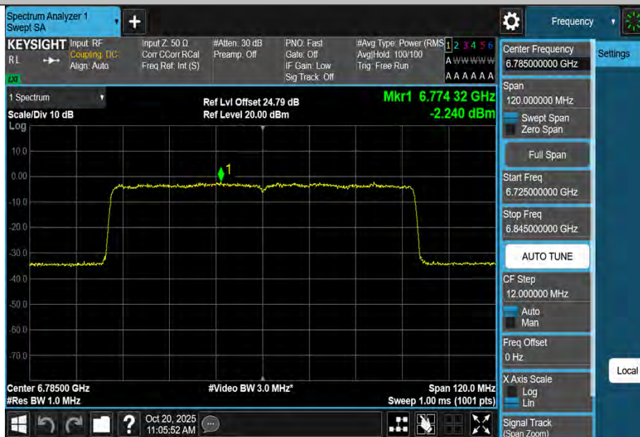
11BE80MIMO-Ant2-6785-PASS
