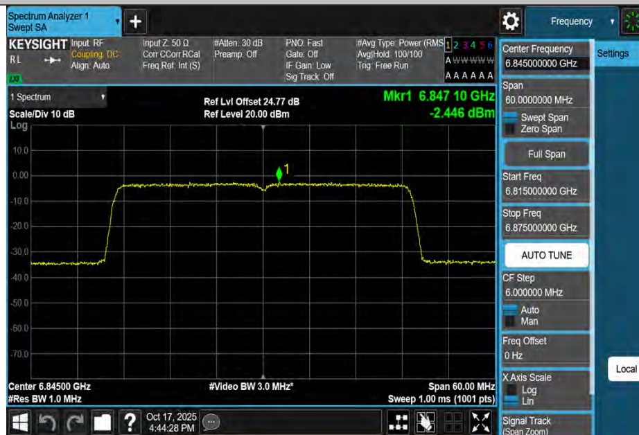
11BE40MIMO-Ant4-6845-PASS
