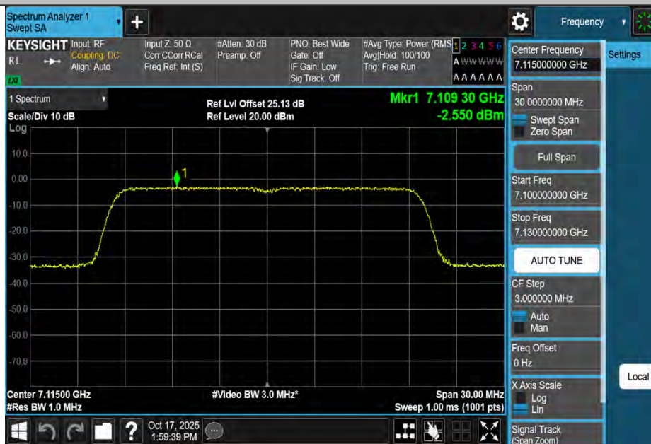
11BE20MIMO-Ant4-7115-PASS
