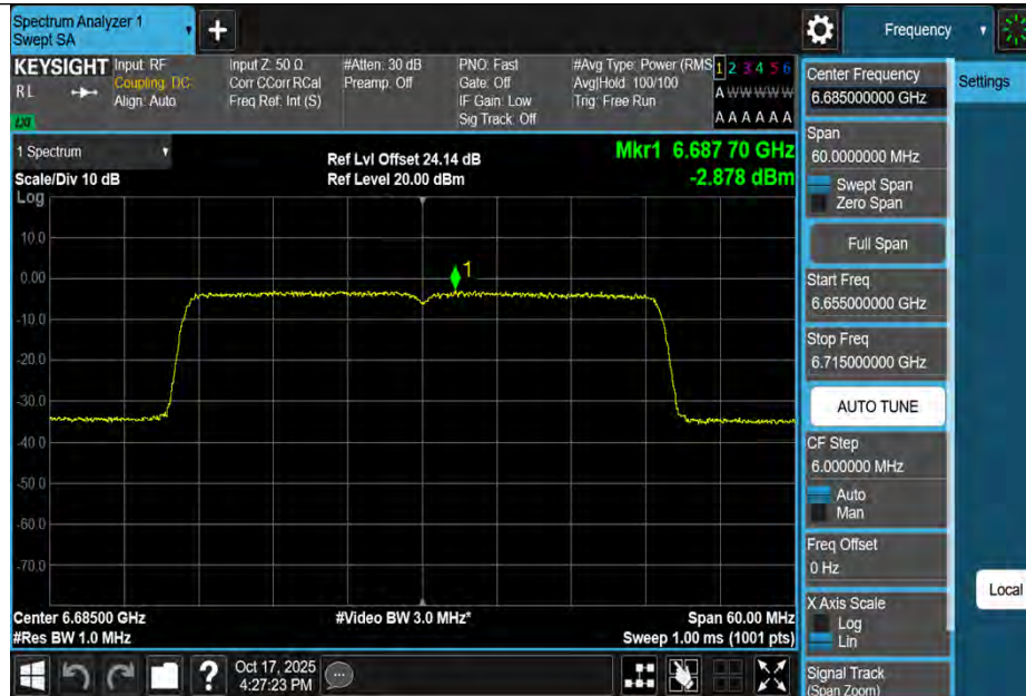
11BE40MIMO-Ant1-6685-PASS
