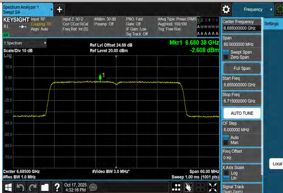
11BE40MIMO-Ant4-6685-PASS
