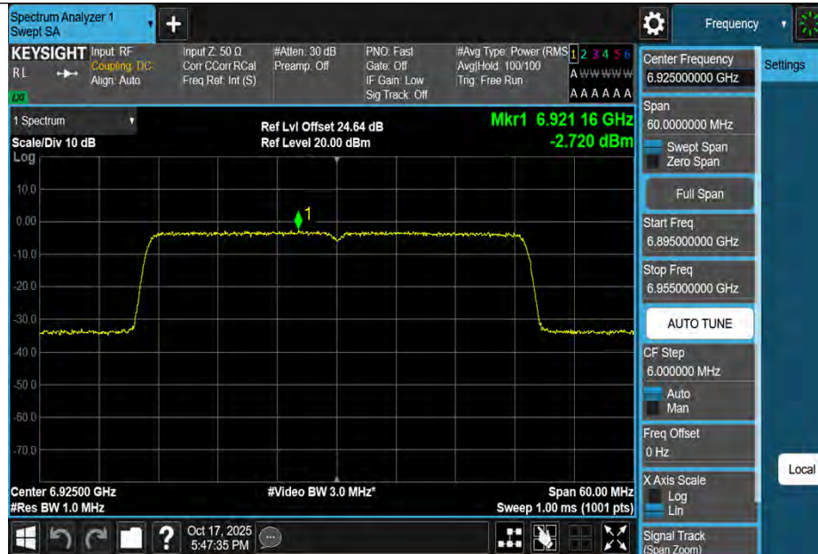
11BE40MIMO-Ant1-6925-PASS
