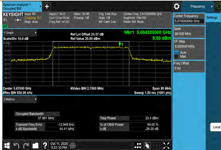
11BE40MIMO-Ant3-5670
