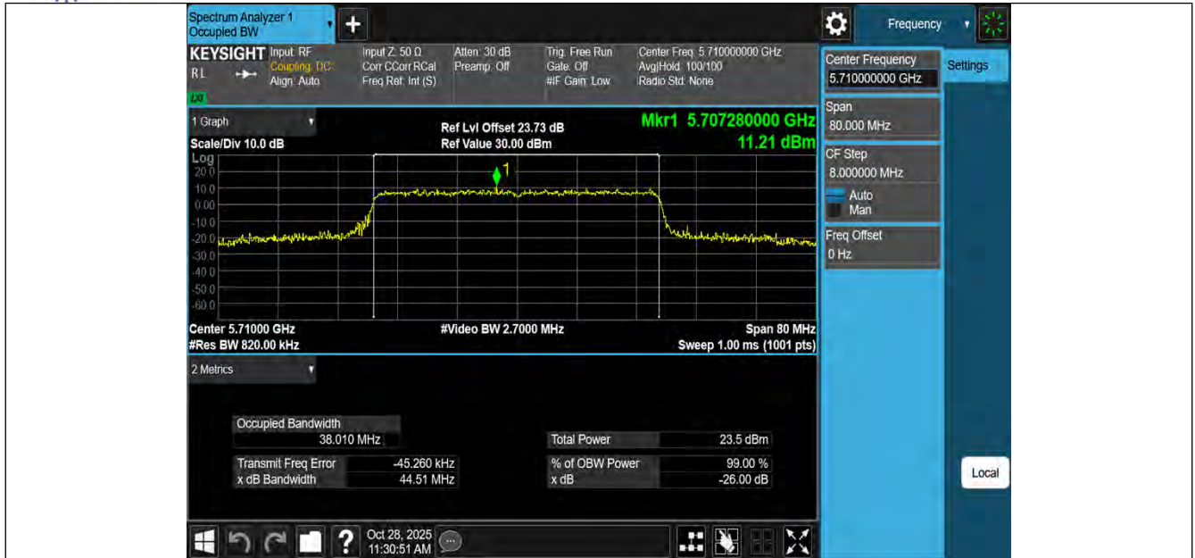
11BE40MIMO-Ant3-5710
