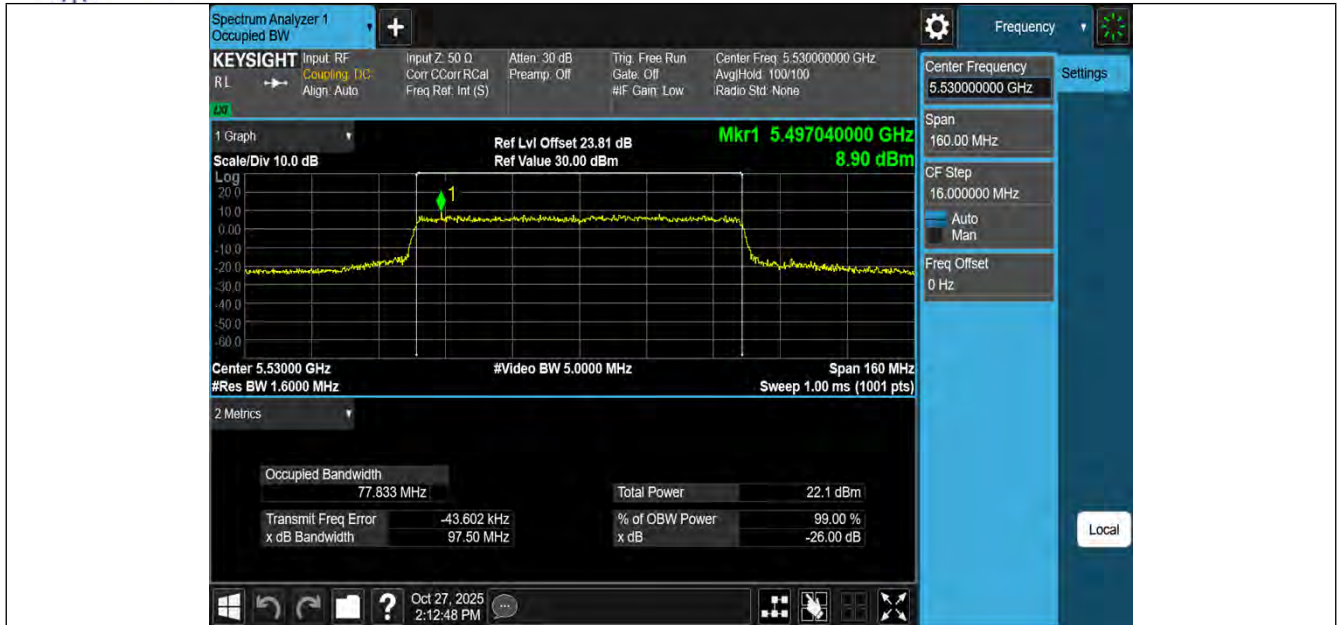
11BE80MIMO-Ant3-5530
