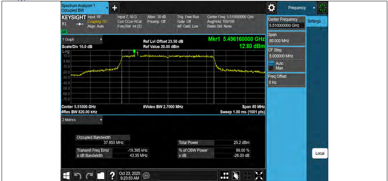
11BE40MIMO-Ant1-5510
