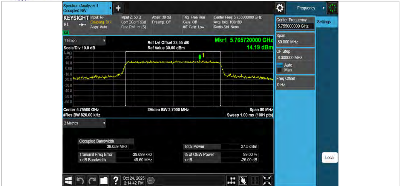
11BE40MIMO-Ant1-5755
