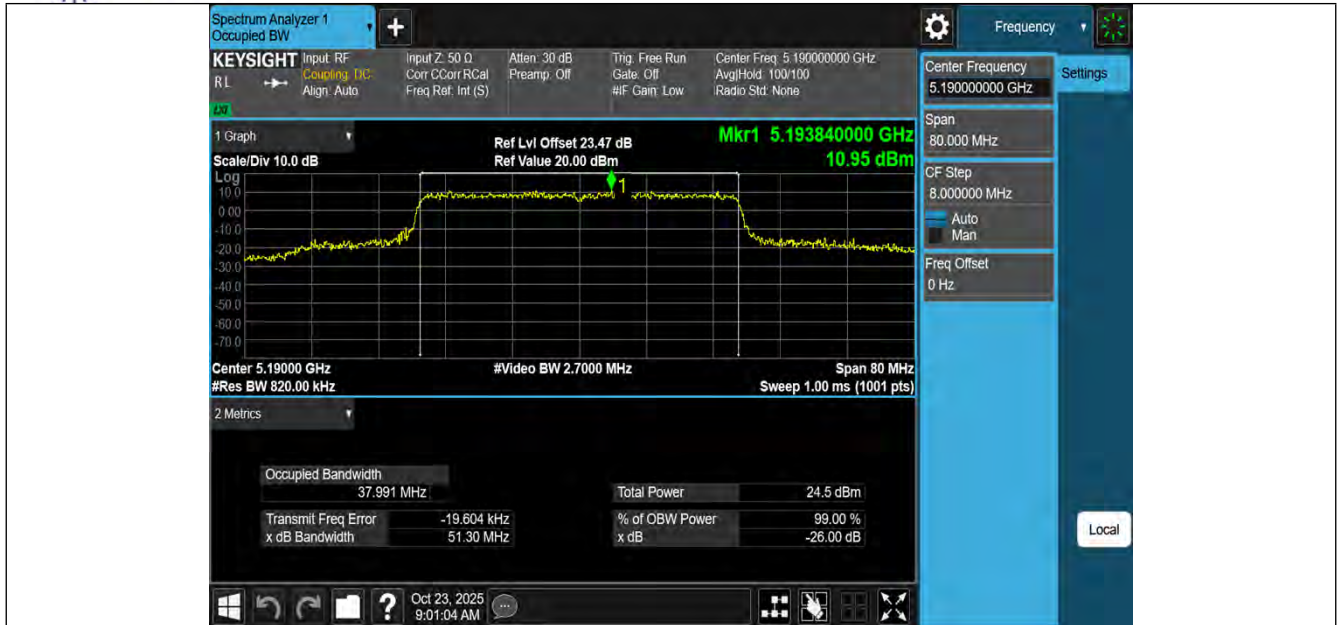
11BE40MIMO-Ant3-5190
