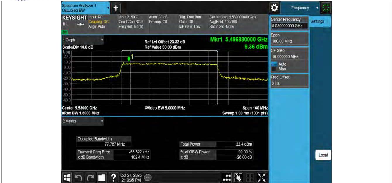
11BE80MIMO-Ant1-5530
