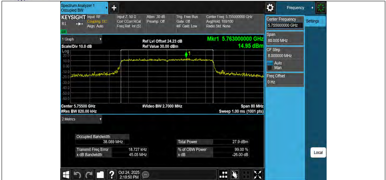
11BE40MIMO-Ant3-5755
