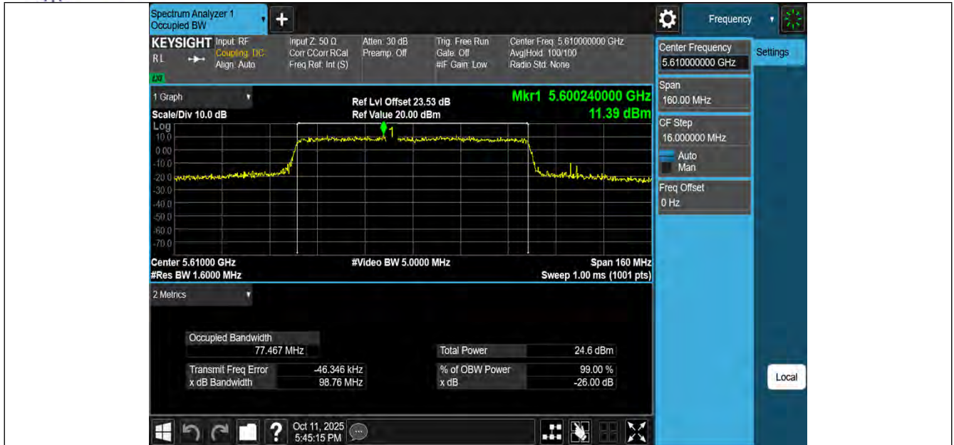
11BE80MIMO-Ant3-5610
