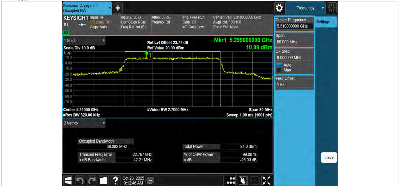
11BE40MIMO-Ant3-5310
