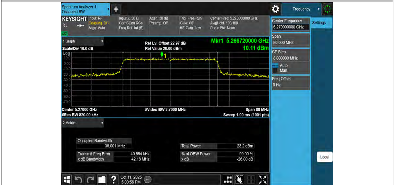
11BE40MIMO-Ant2-5270
