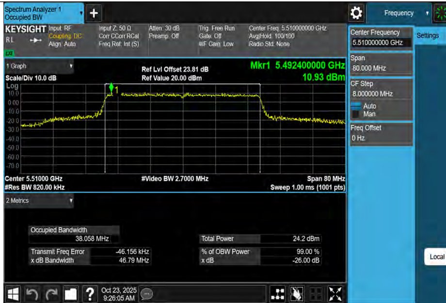
11BE40MIMO-Ant3-5510
