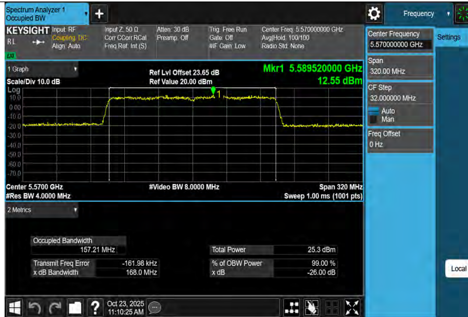
11BE160MIMO-Ant3-5570
