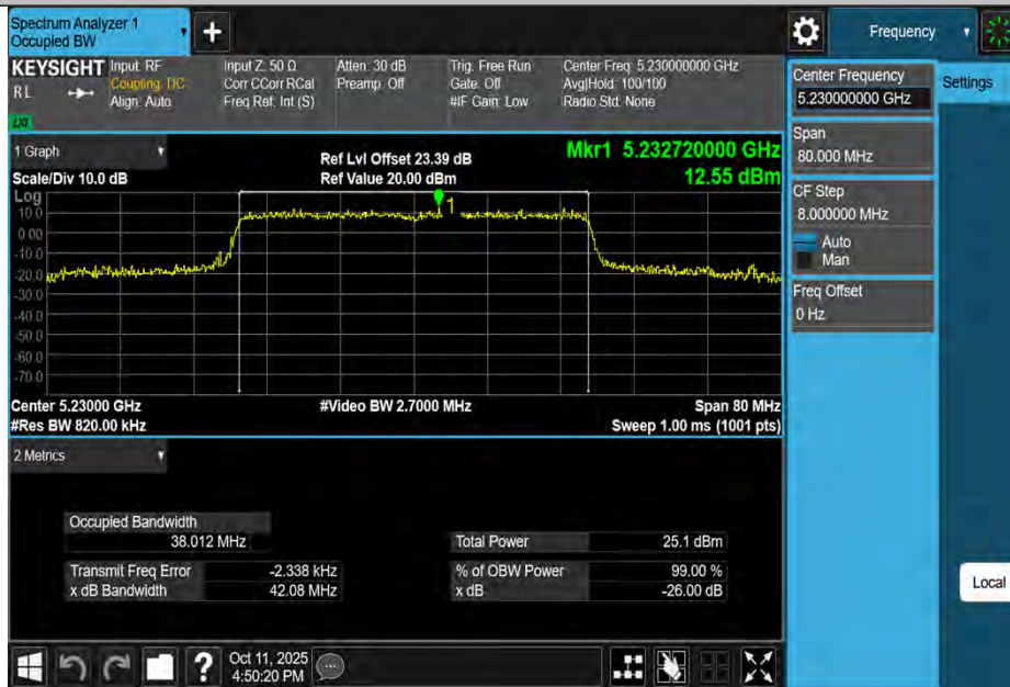
11BE40MIMO-Ant4-5230
