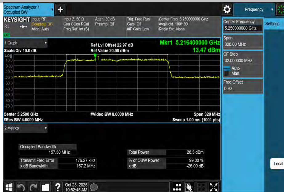
11BE160MIMO-Ant2-5250
