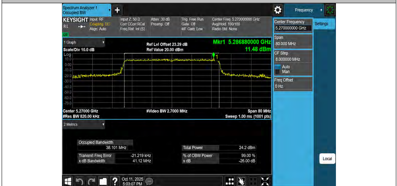
11BE40MIMO-Ant4-5270
