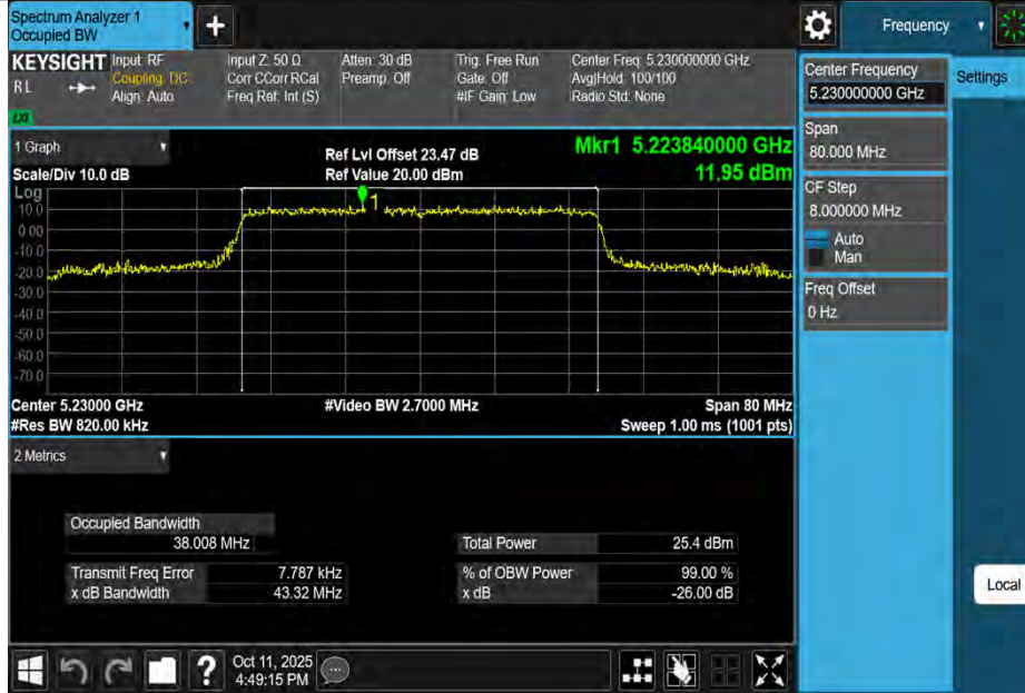
11BE40MIMO-Ant3-5230
