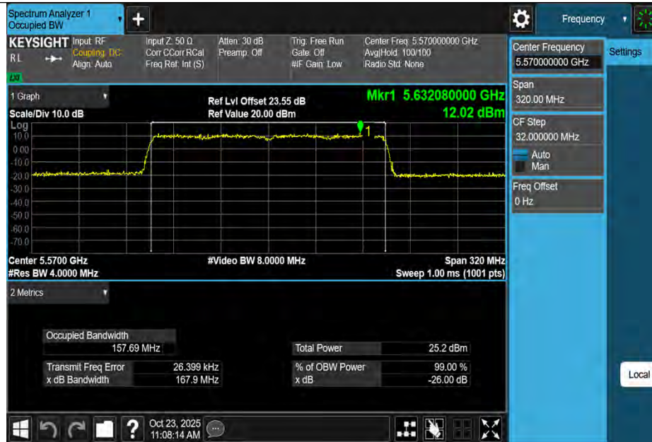
11BE160MIMO-Ant1-5570
