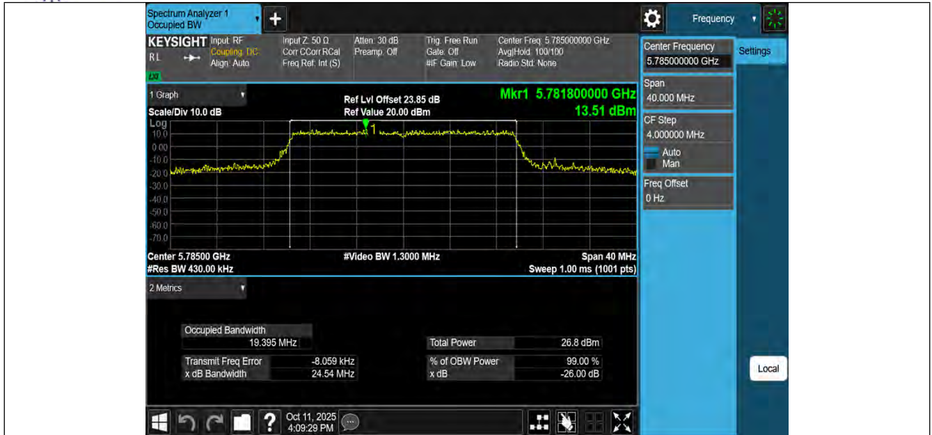
11BE20MIMO-Ant3-5785
