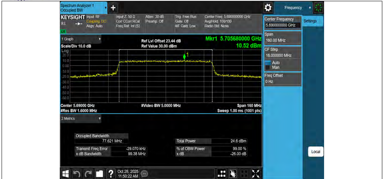
11BE80MIMO-Ant1-5690
