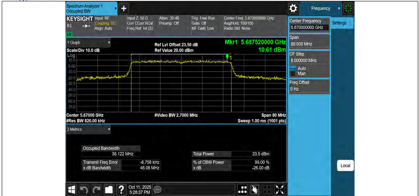
11BE40MIMO-Ant1-5670
