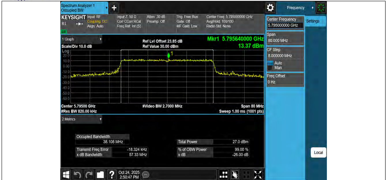
11BE40MIMO-Ant3-5795
