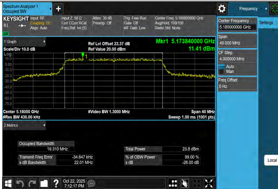
11BE20MIMO-Ant2-5180
