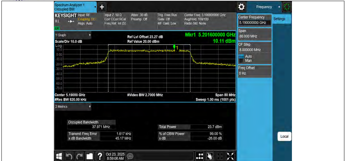
11BE40MIMO-Ant1-5190
