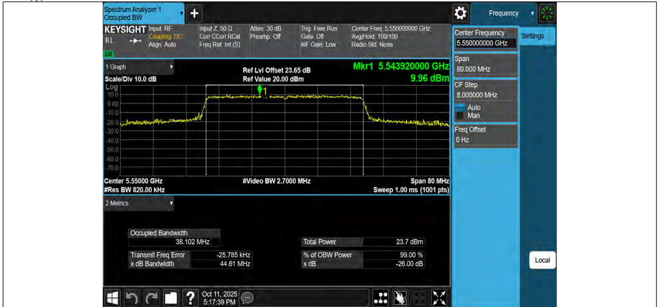
11BE40MIMO-Ant3-5550
