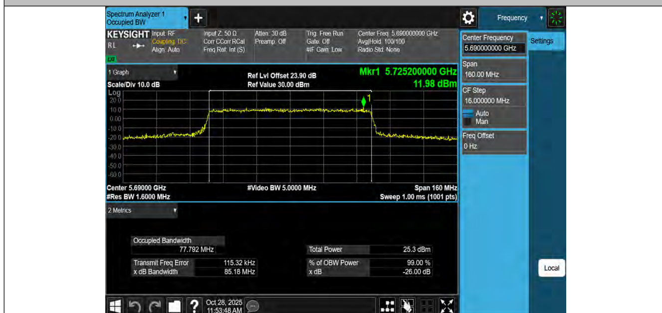
11BE80MIMO-Ant4-5690
