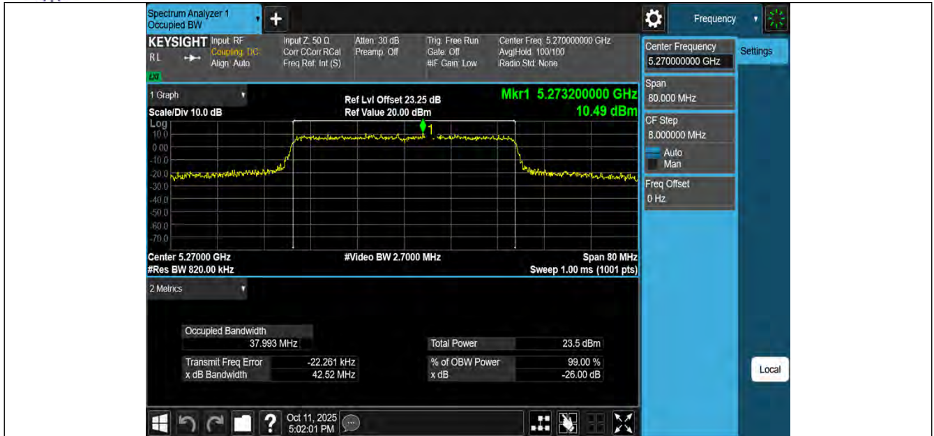
11BE40MIMO-Ant3-5270
