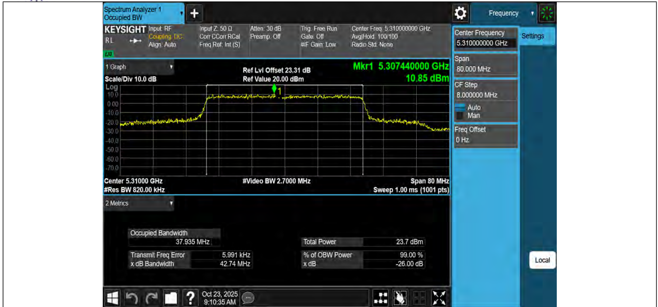
11BE40MIMO-Ant1-5310
