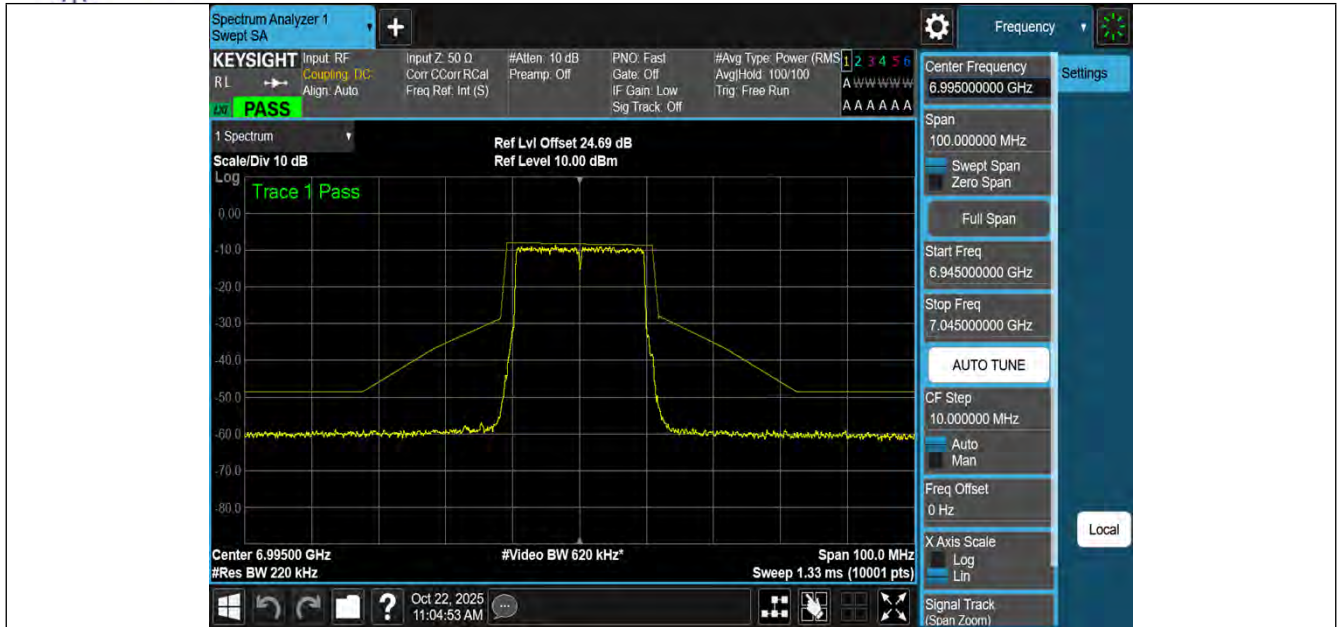
NTNV-11AX20MIMO-Ant1-6995-PASS
