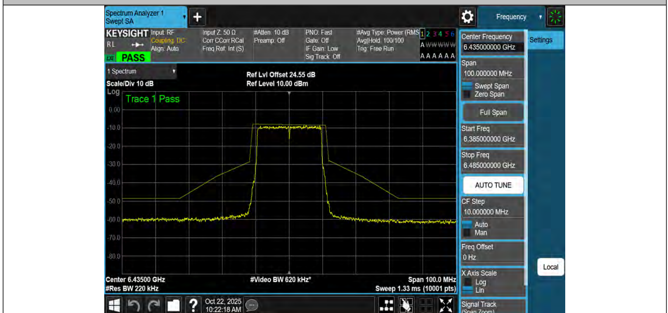
NTNV-11AX20MIMO-Ant4-6435-PASS
