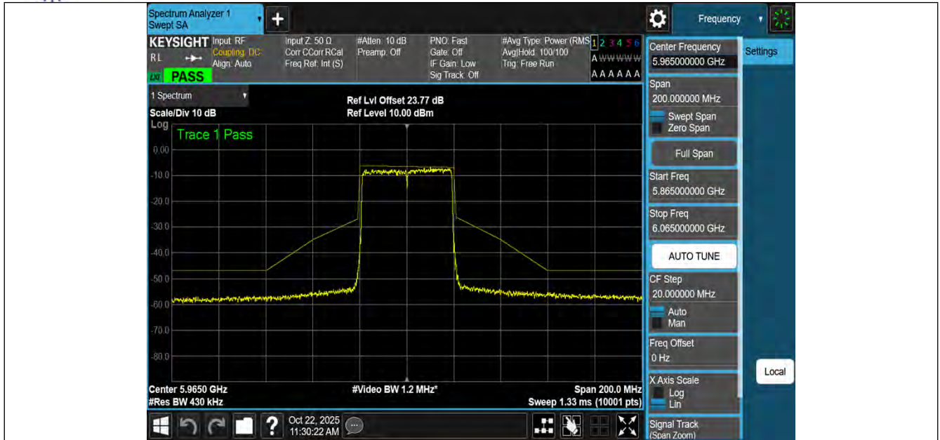
NTNV-11AX40MIMO-Ant3-5965-PASS
