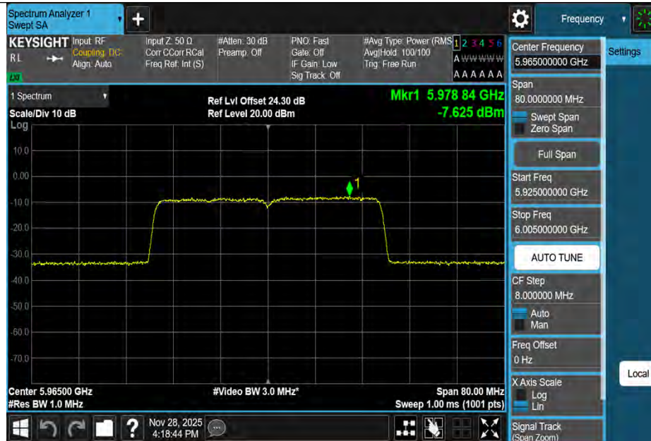
11AX40MIMO-Ant3-5965-PASS
