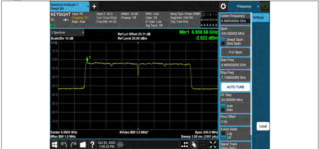
11BE160MIMO-Ant3-6985-PASS
