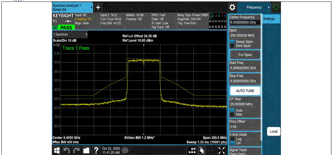
NTNV-11AX40MIMO-Ant3-6405-PASS
