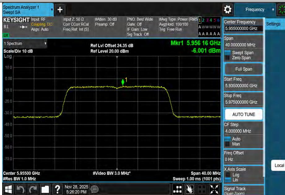
11BE20MIMO-Ant4-5955-PASS
