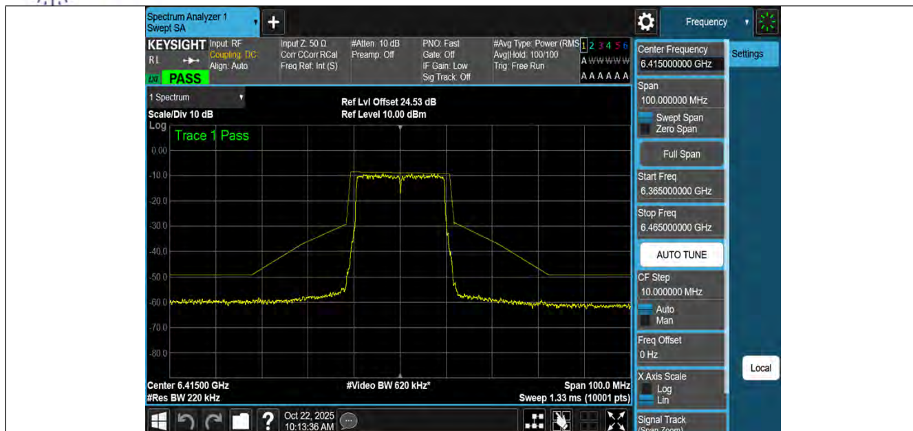
NTNV-11AX20MIMO-Ant1-6415-PASS
