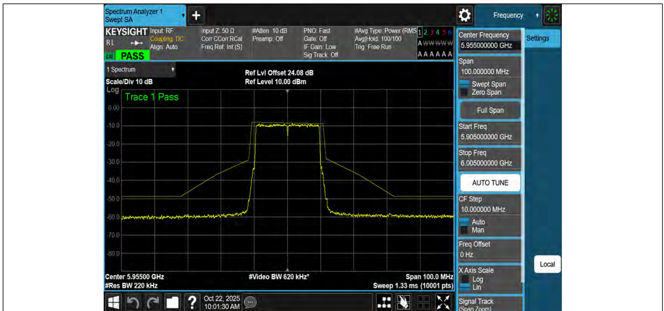
NTNV-11AX20MIMO-Ant1-5955-PASS
