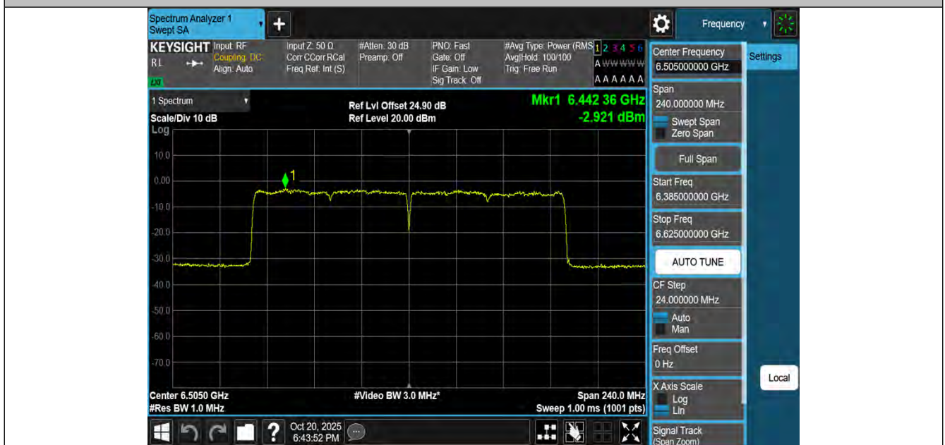
11BE160MIMO-Ant2-6505-PASS
