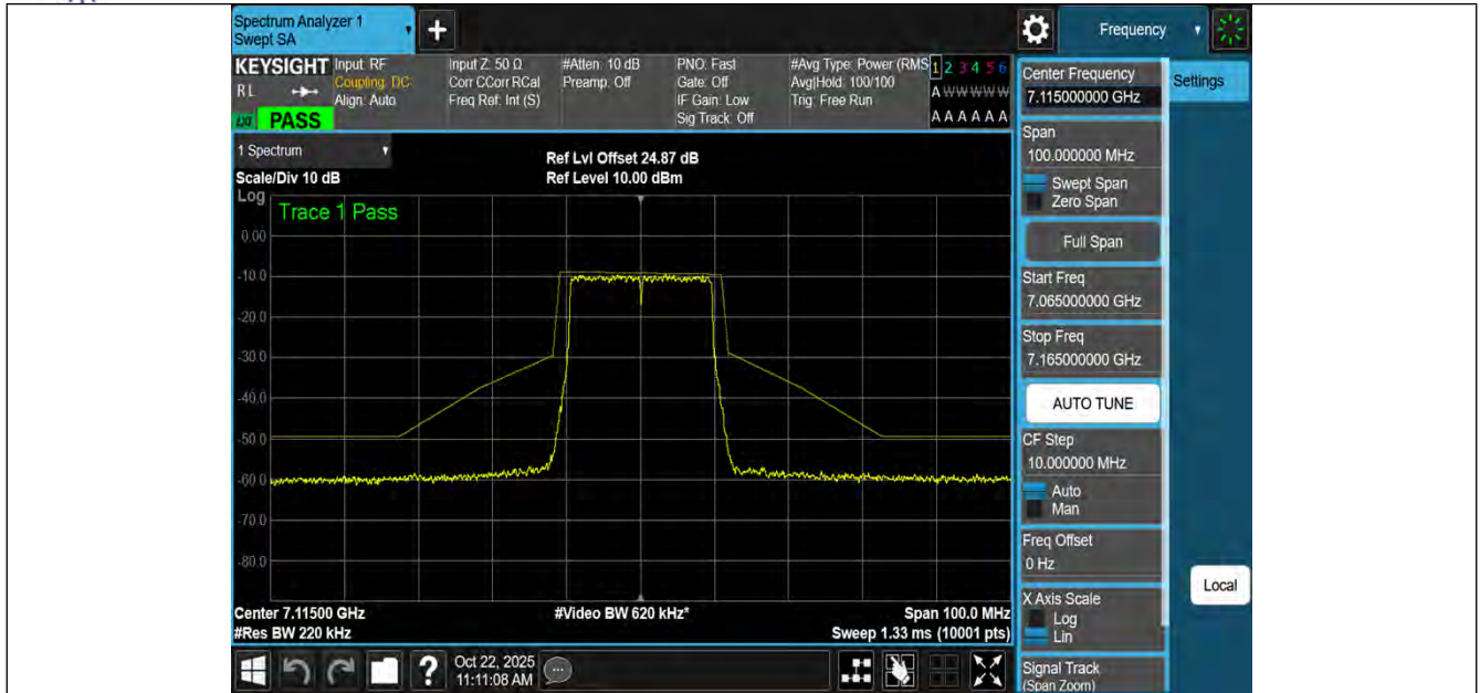
NTNV-11AX20MIMO-Ant1-7115-PASS
