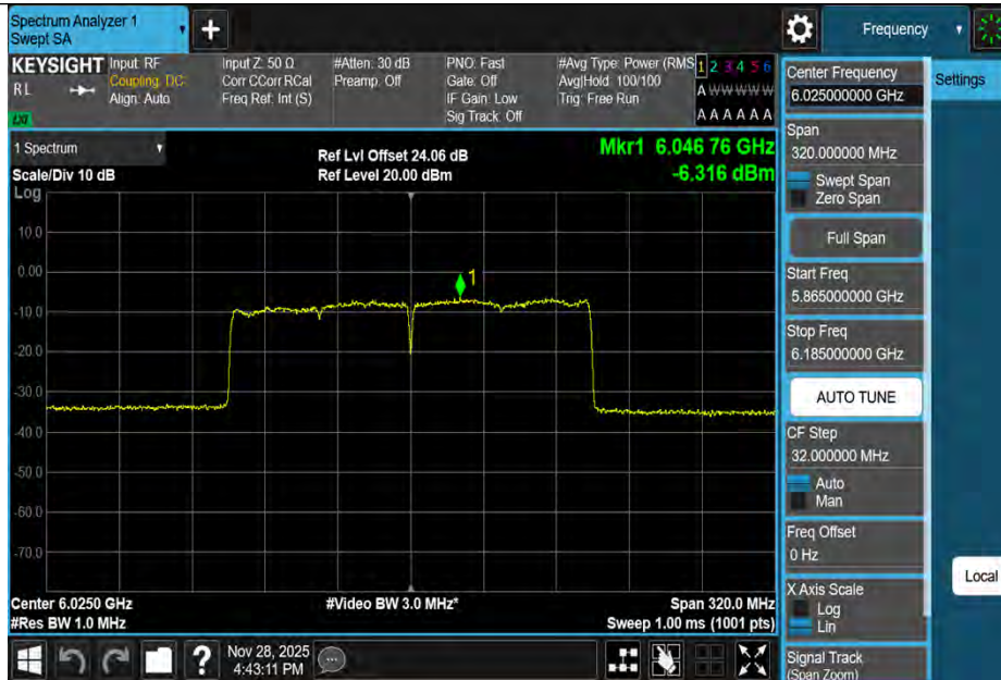
11AX160MIMO-Ant3-6025-PASS
