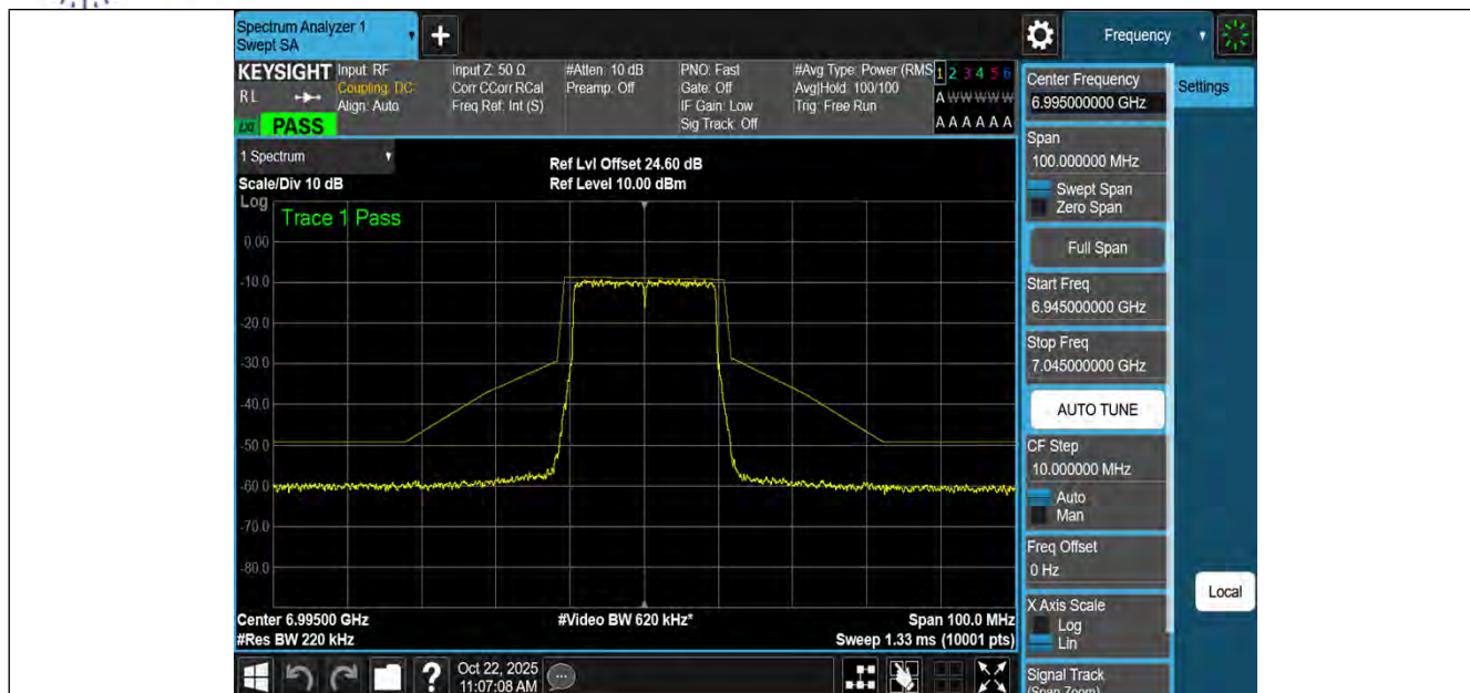
NTNV-11AX20MIMO-Ant3-6995-PASS
