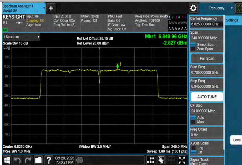
11BE160MIMO-Ant2-6825-PASS
