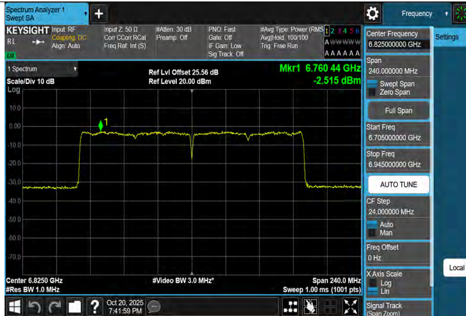
11BE160MIMO-Ant3-6825-PASS
