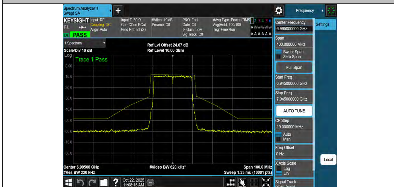
NTNV-11AX20MIMO-Ant4-6995-PASS
