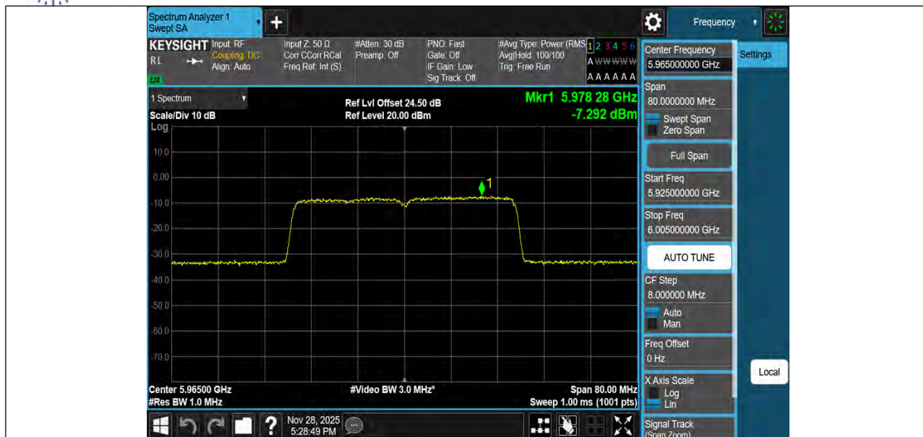
11BE40MIMO-Ant1-5965-PASS
