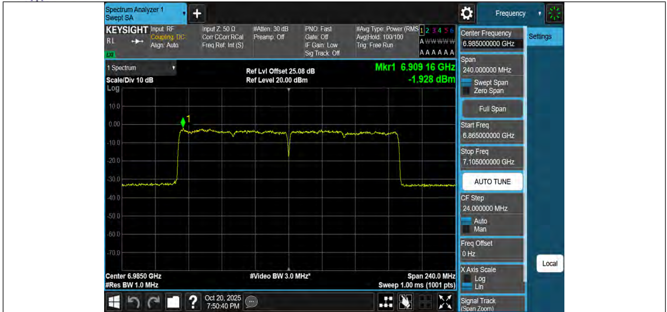
11BE160MIMO-Ant1-6985-PASS
