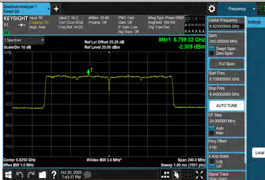
11BE160MIMO-Ant4-6825-PASS
