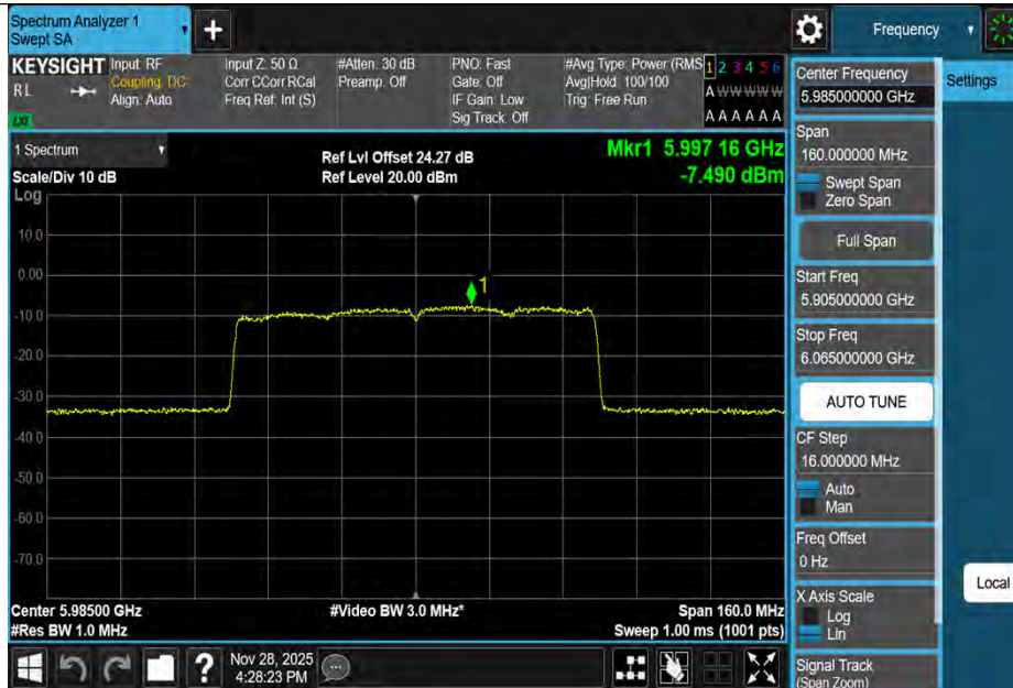
11AX80MIMO-Ant3-5985-PASS
