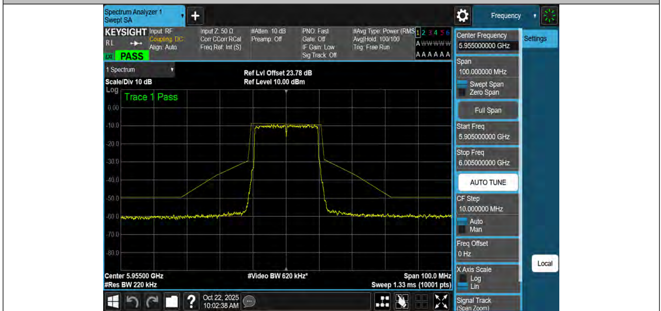
NTNV-11AX20MIMO-Ant2-5955-PASS
