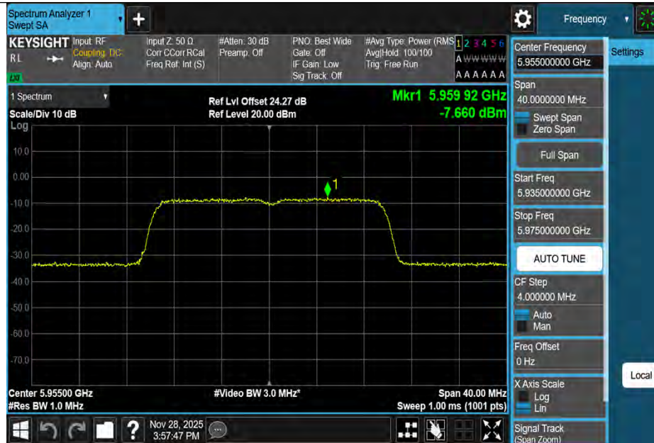
11AX20MIMO-Ant3-5955-PASS
