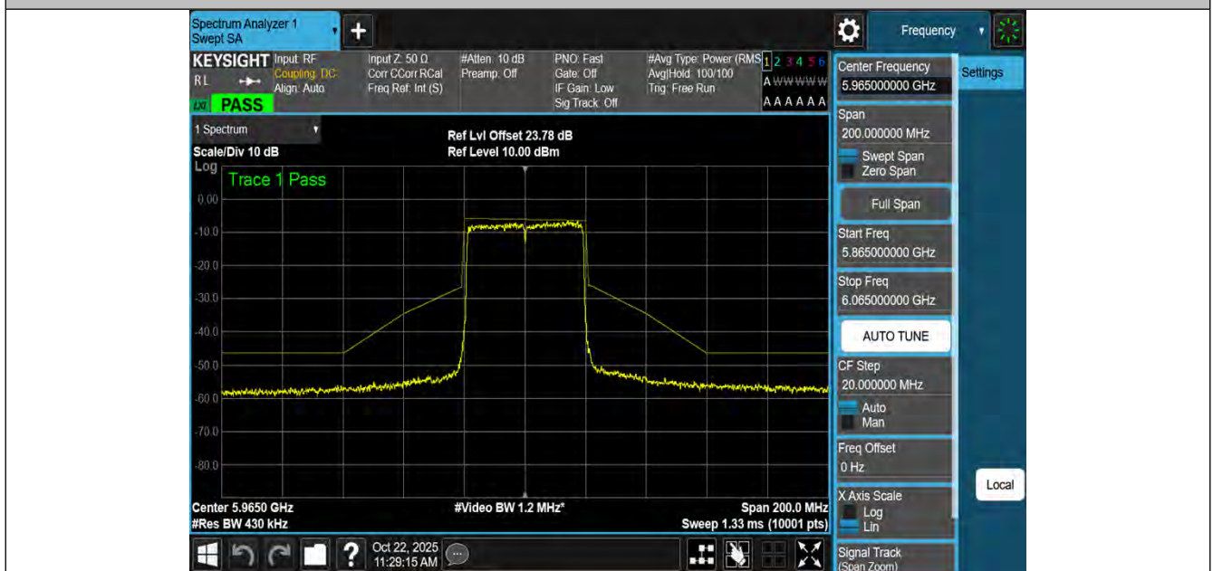
NTNV-11AX40MIMO-Ant2-5965-PASS
