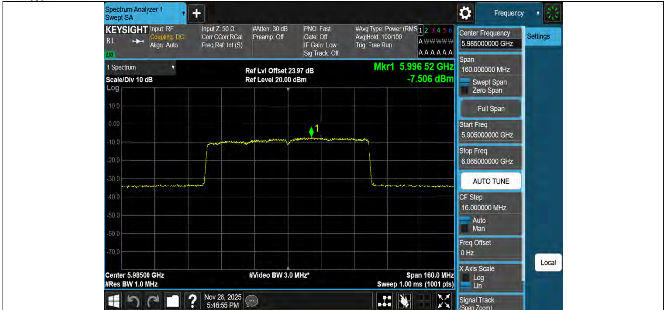
11BE80MIMO-Ant1-5985-PASS
