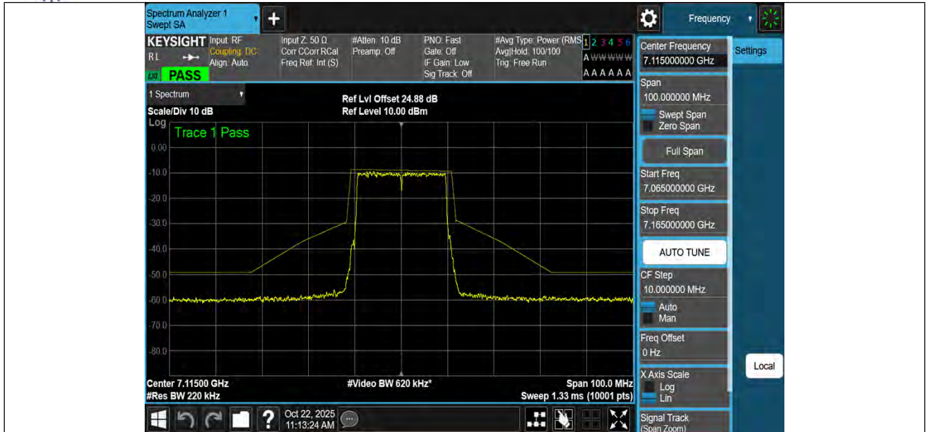
NTNV-11AX20MIMO-Ant3-7115-PASS
