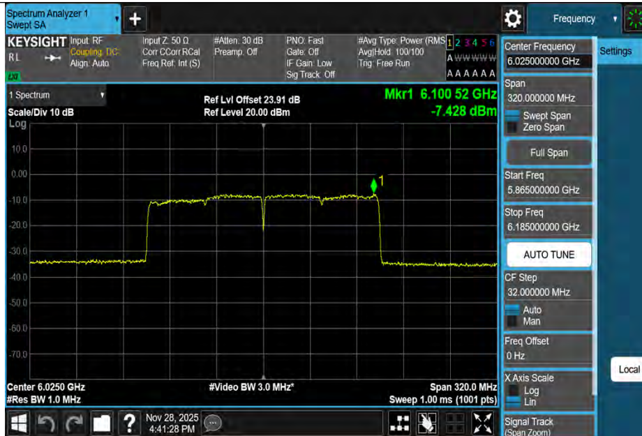
11AX160MIMO-Ant1-6025-PASS
