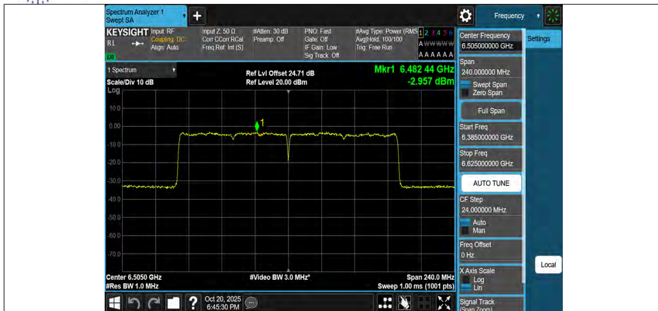
11BE160MIMO-Ant3-6505-PASS
