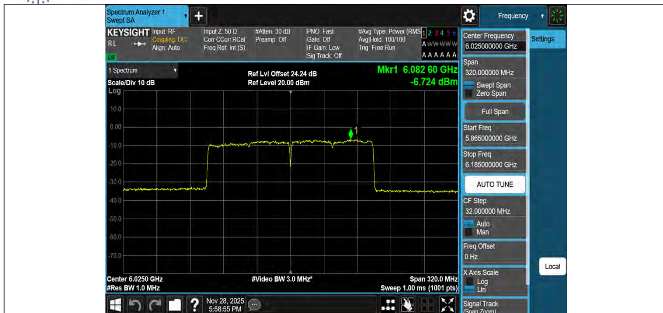
11BE160MIMO-Ant3-6025-PASS
