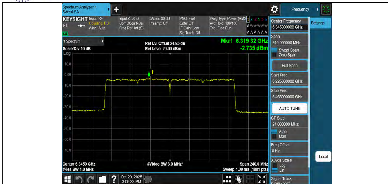
11BE160MIMO-Ant3-6345-PASS
