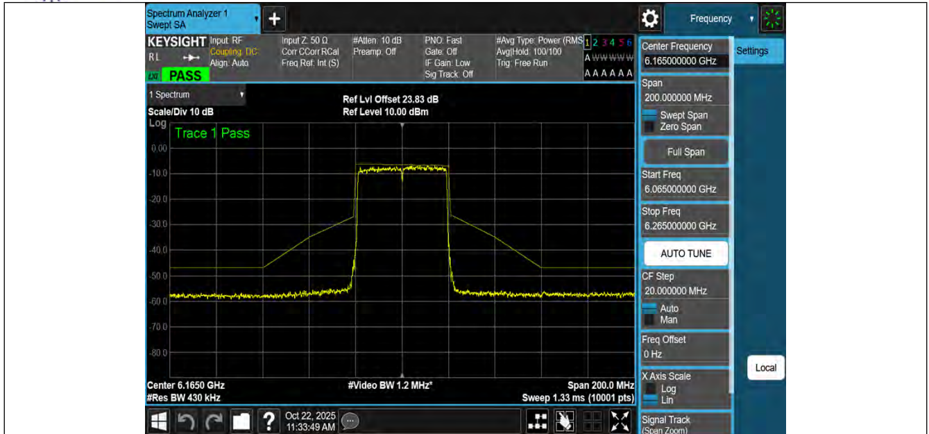
NTNV-11AX40MIMO-Ant1-6165-PASS
