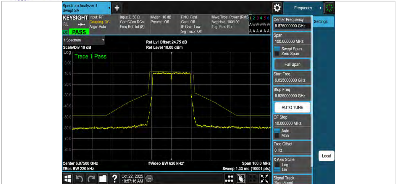
NTNV-11AX20MIMO-Ant3-6875-PASS
