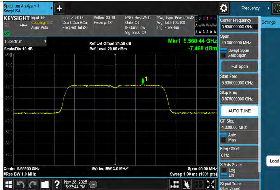
11BE20MIMO-Ant1-5955-PASS
