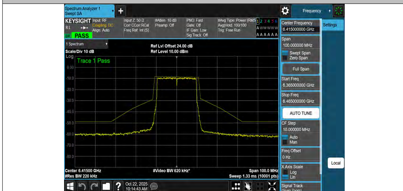
NTNV-11AX20MIMO-Ant2-6415-PASS
