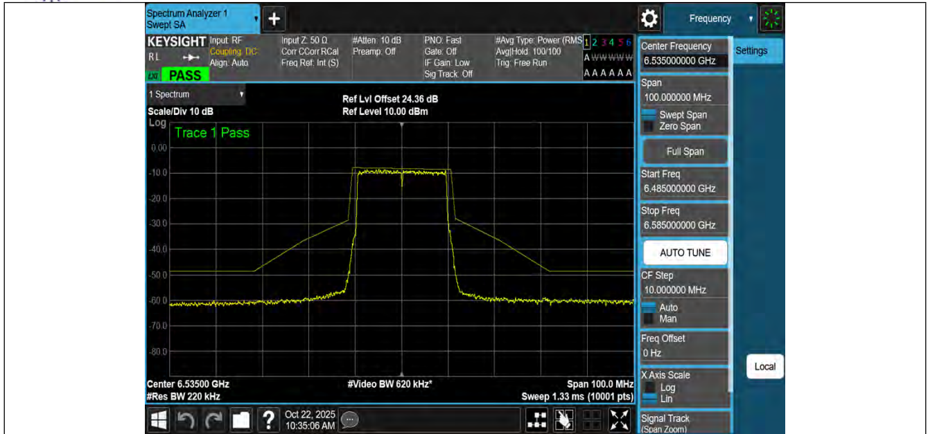
NTNV-11AX20MIMO-Ant1-6535-PASS
