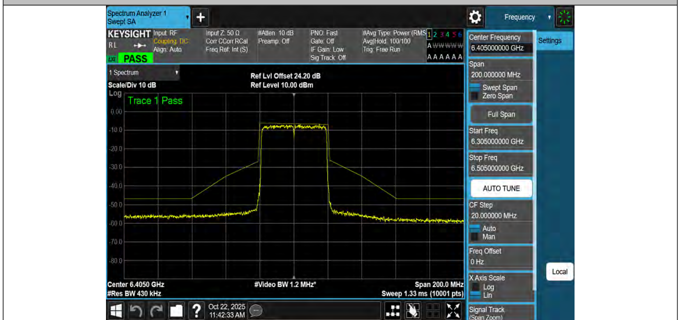
NTNV-11AX40MIMO-Ant4-6405-PASS
