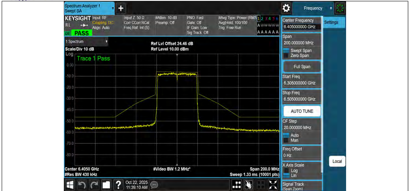
NTNV-11AX40MIMO-Ant1-6405-PASS
