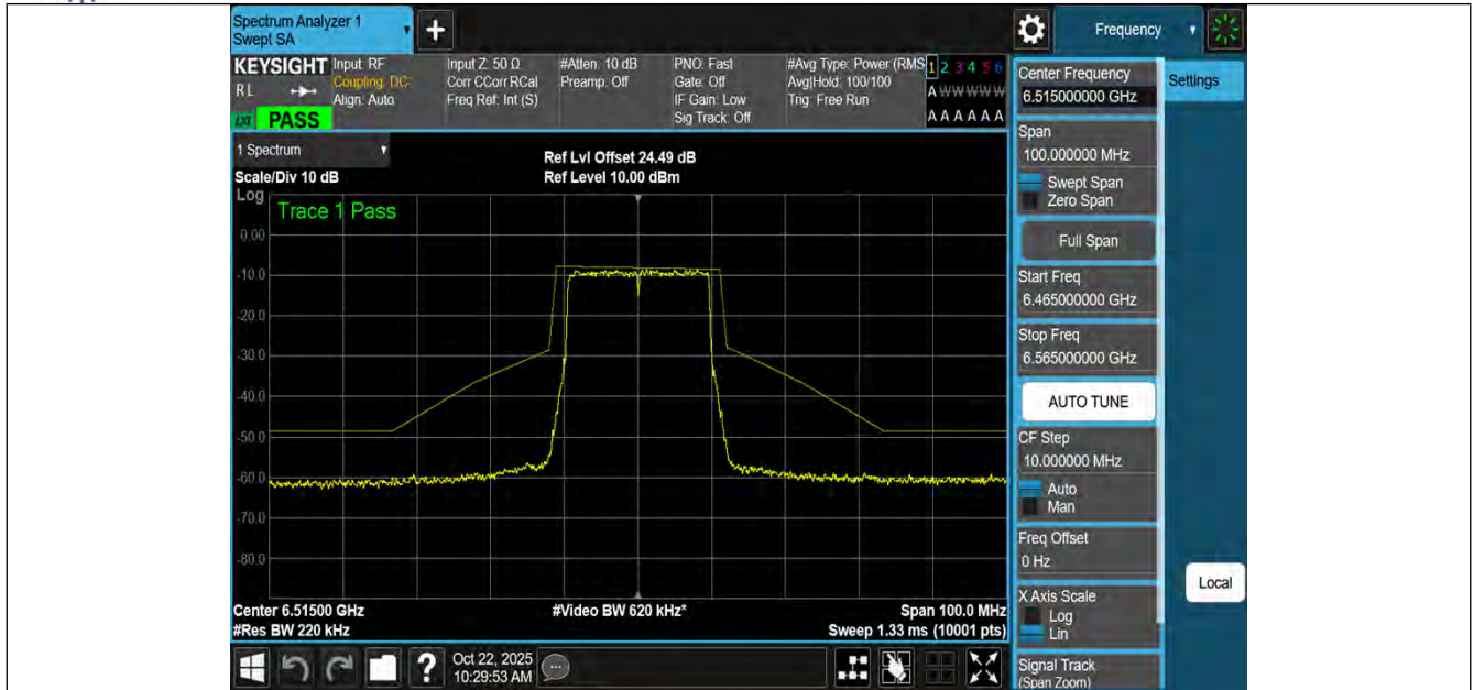
NTNV-11AX20MIMO-Ant1-6515-PASS
