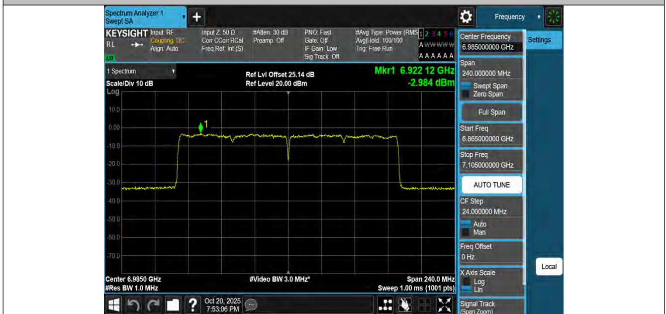
11BE160MIMO-Ant2-6985-PASS
