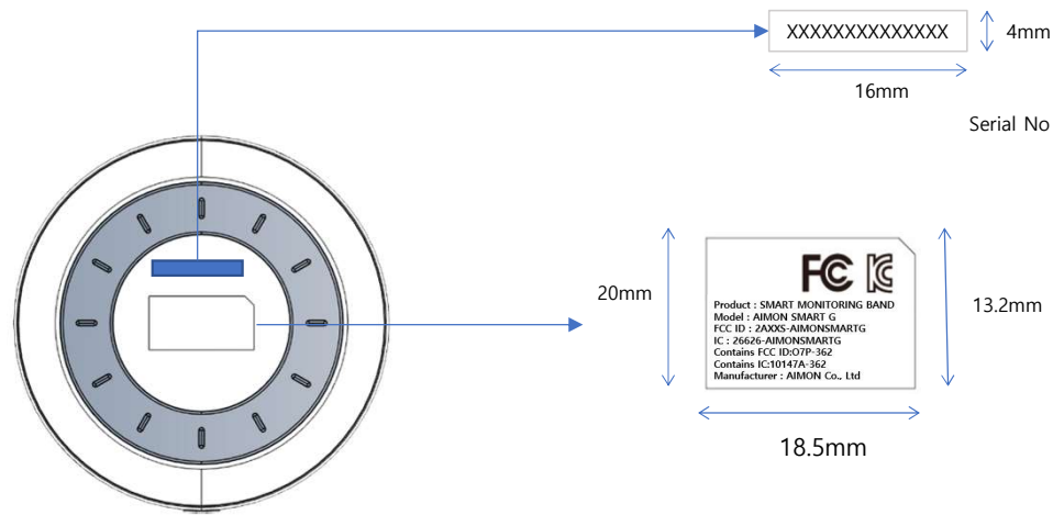
[ Rear of the device ]
